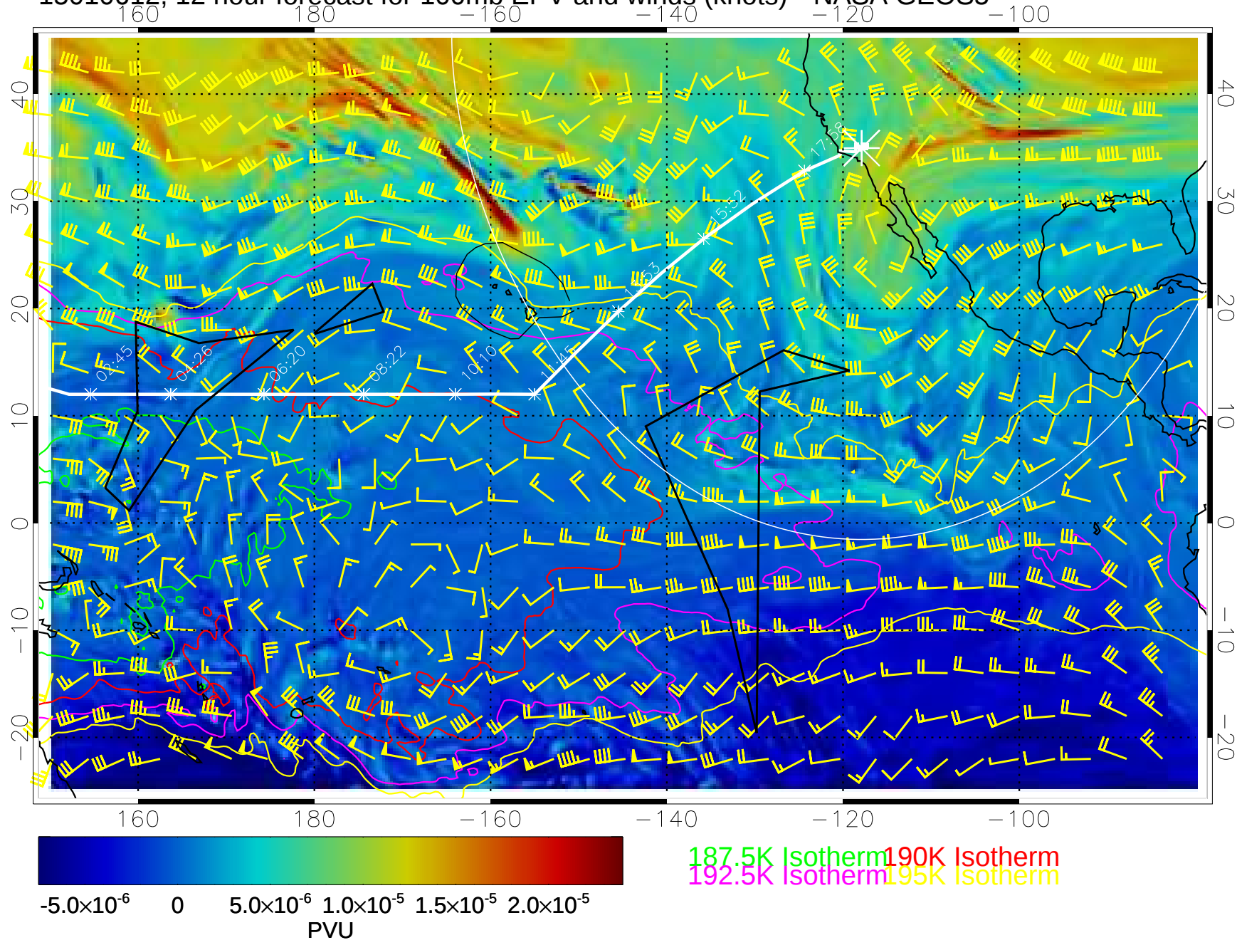
15010612, 12 hour forecast for 100mb EPV and winds (knots)-- NASA GEOS5
