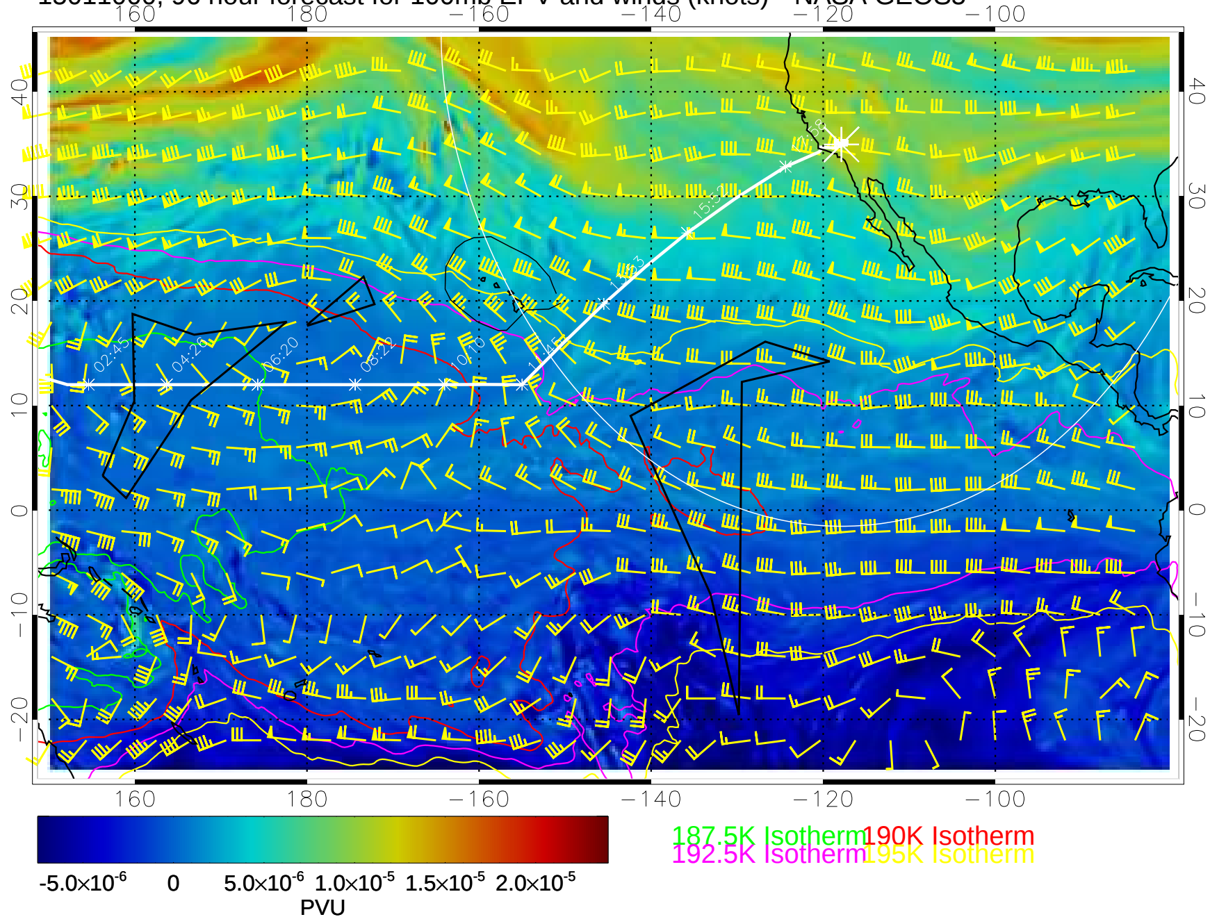
15011000, 96 hour forecast for 100mb EPV and winds (knots)-- NASA GEOS5
