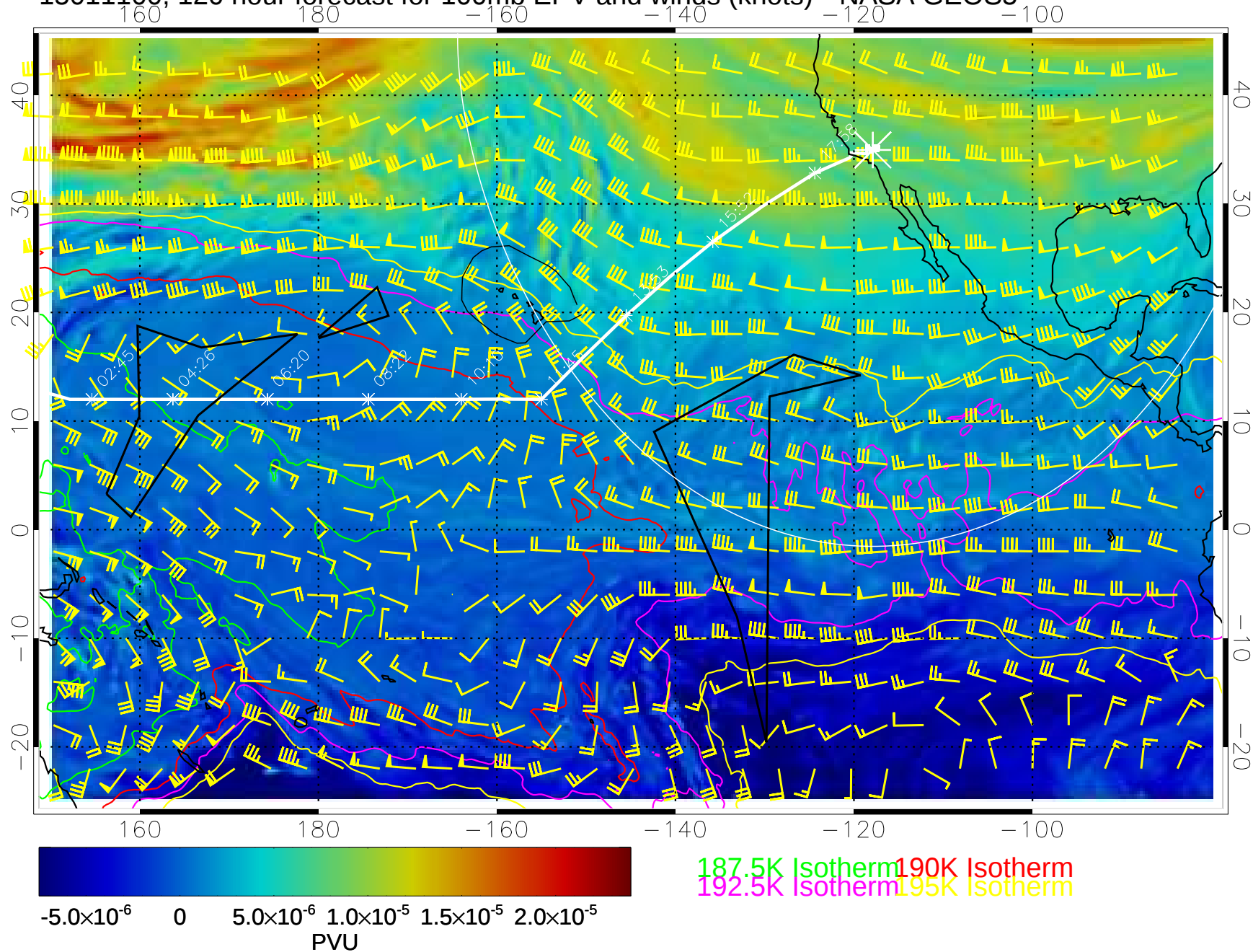
15011100, 120 hour forecast for 100mb EPV and winds (knots)-- NASA GEOS5
