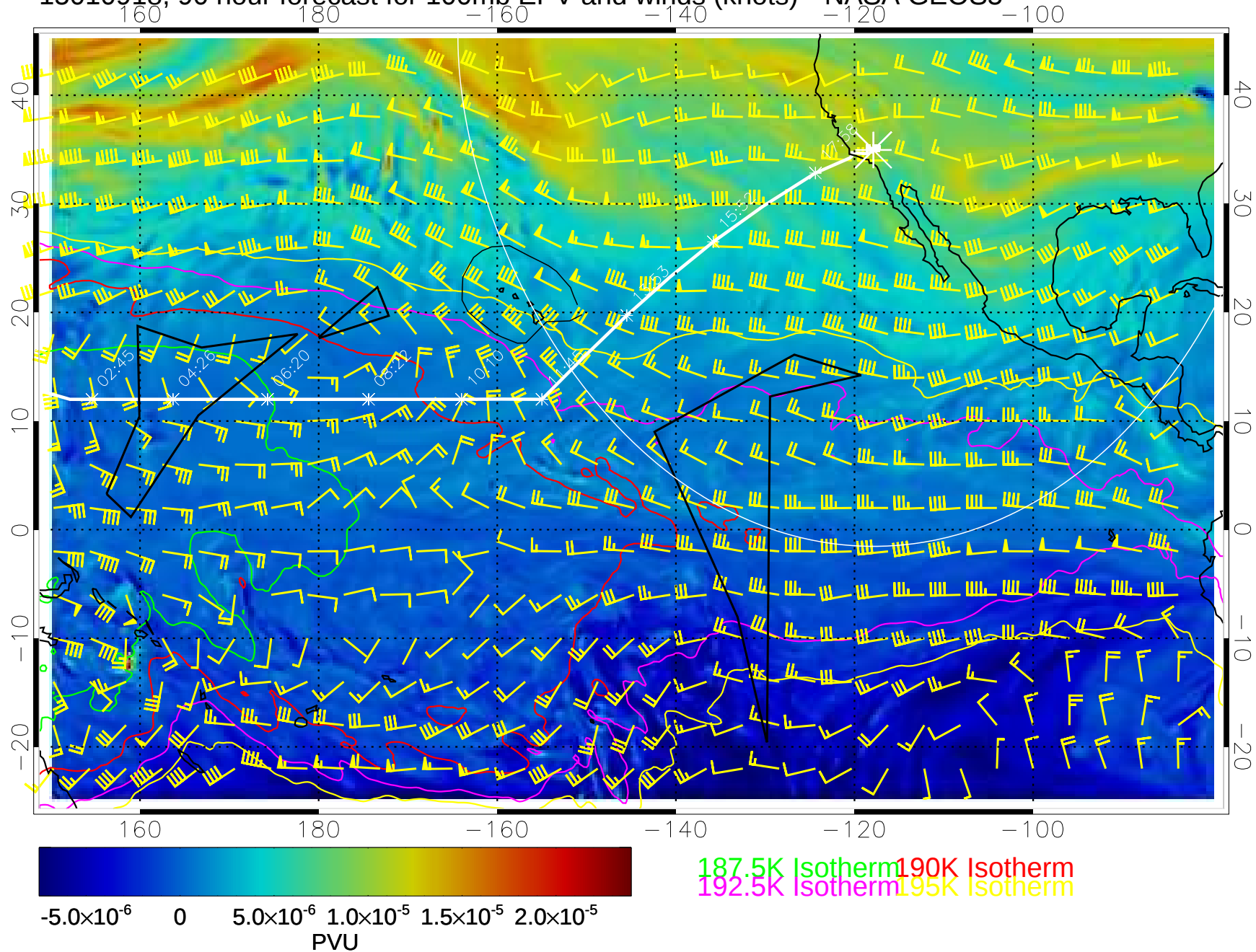
15010918, 90 hour forecast for 100mb EPV and winds (knots)-- NASA GEOS5
