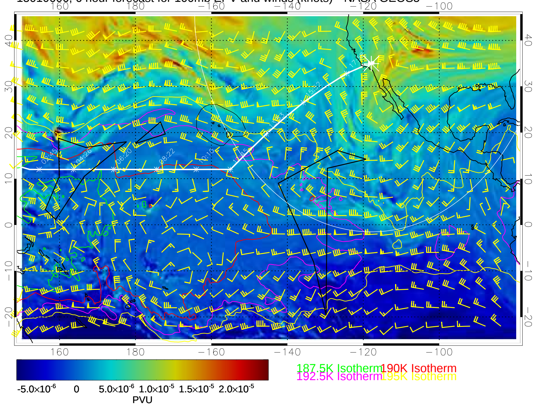
15010606, 6 hour forecast for 100mb EPV and winds (knots)-- NASA GEOS5
