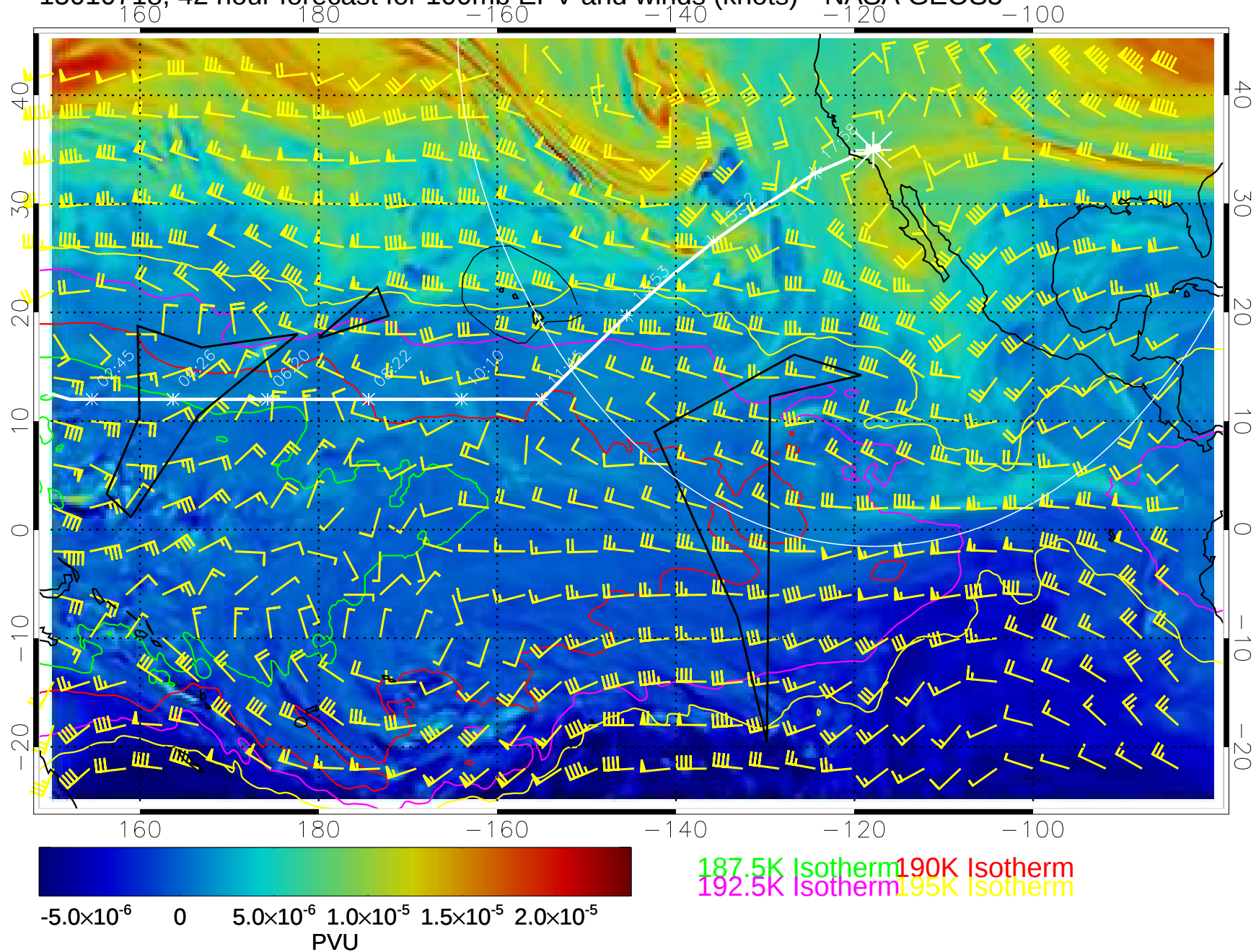
15010718, 42 hour forecast for 100mb EPV and winds (knots)-- NASA GEOS5
