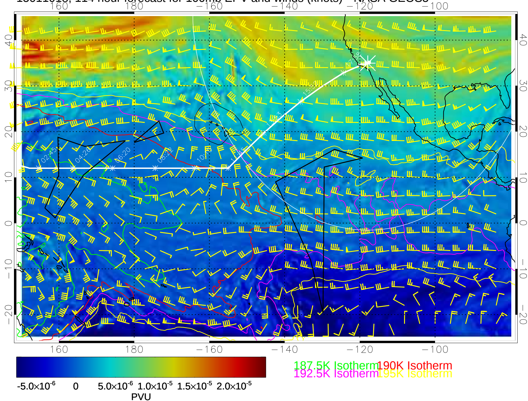
15011018, 114 hour forecast for 100mb EPV and winds (knots)-- NASA GEOS5
