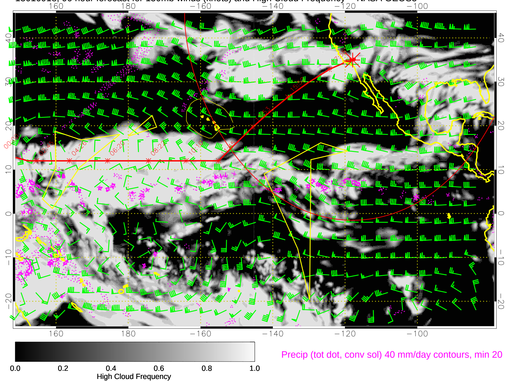
15010918, 90 hour forecast for 150mb winds (knots) and High Cloud Frequency -- NASA GEOS5
