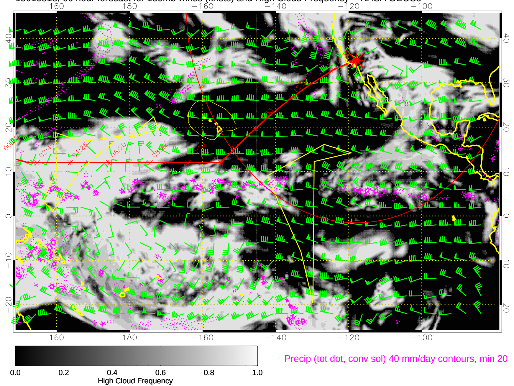
15010818, 66 hour forecast for 150mb winds (knots) and High Cloud Frequency -- NASA GEOS5
