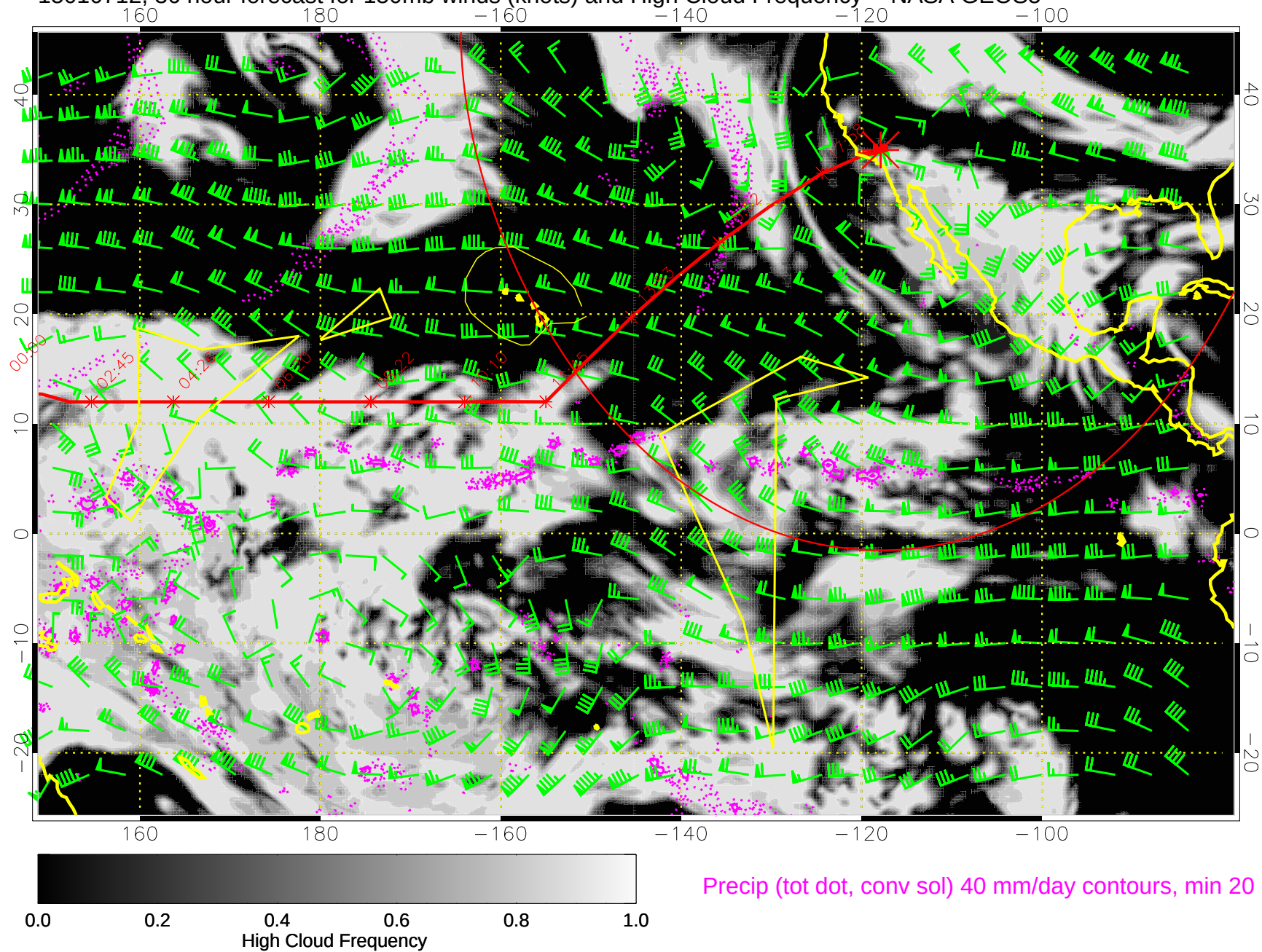
15010712, 36 hour forecast for 150mb winds (knots) and High Cloud Frequency -- NASA GEOS5
