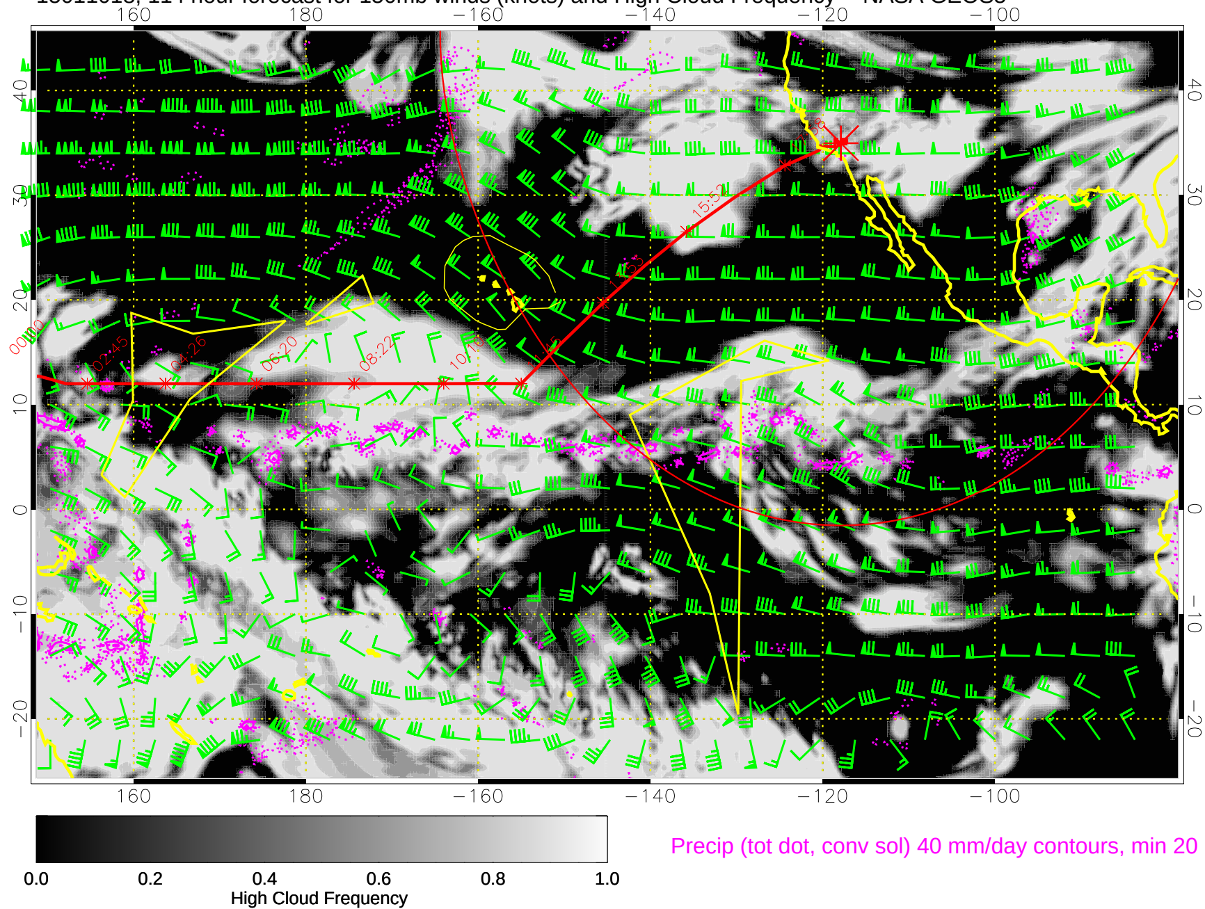
15011018, 114 hour forecast for 150mb winds (knots) and High Cloud Frequency -- NASA GEOS5
