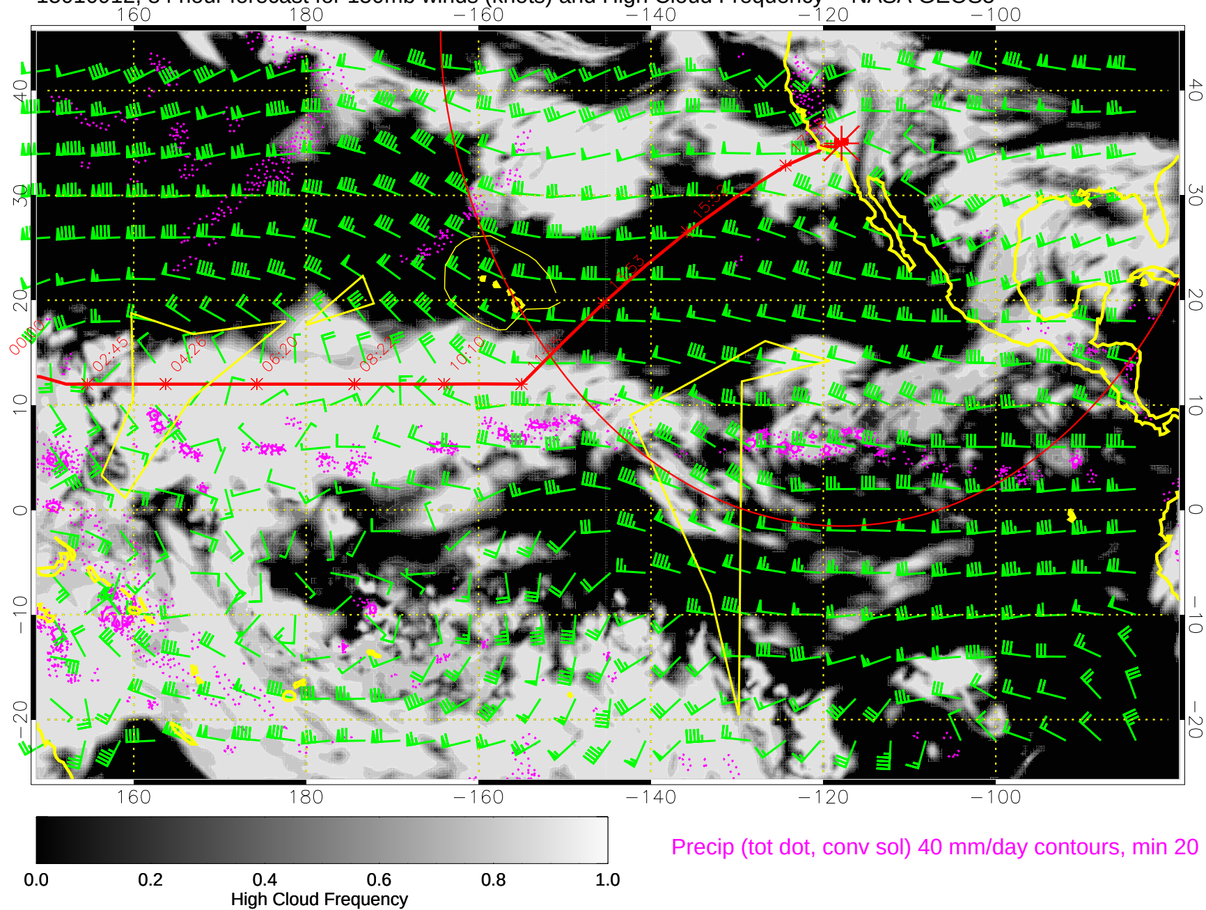
15010912, 84 hour forecast for 150mb winds (knots) and High Cloud Frequency -- NASA GEOS5
