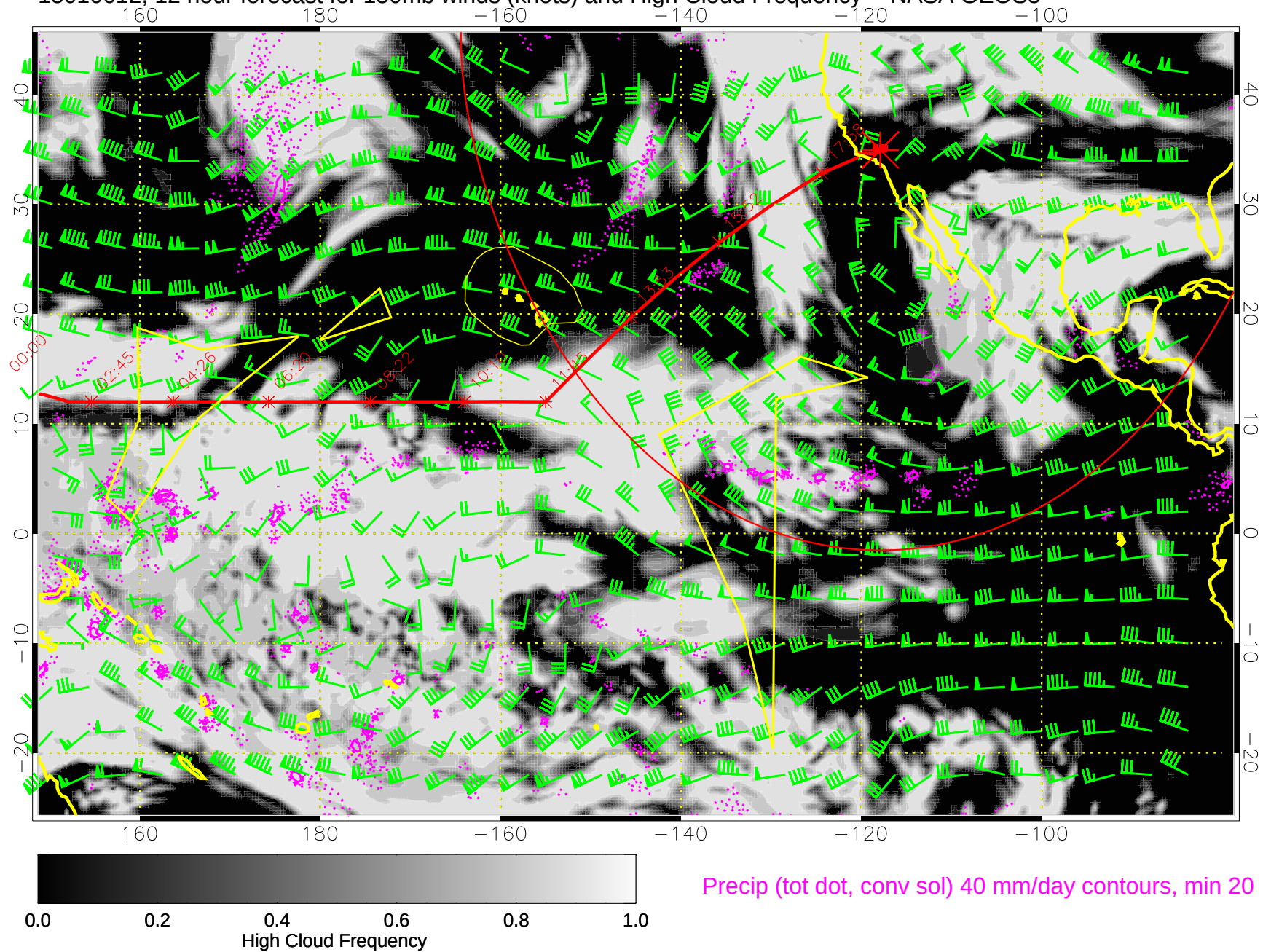
15010612, 12 hour forecast for 150mb winds (knots) and High Cloud Frequency -- NASA GEOS5
