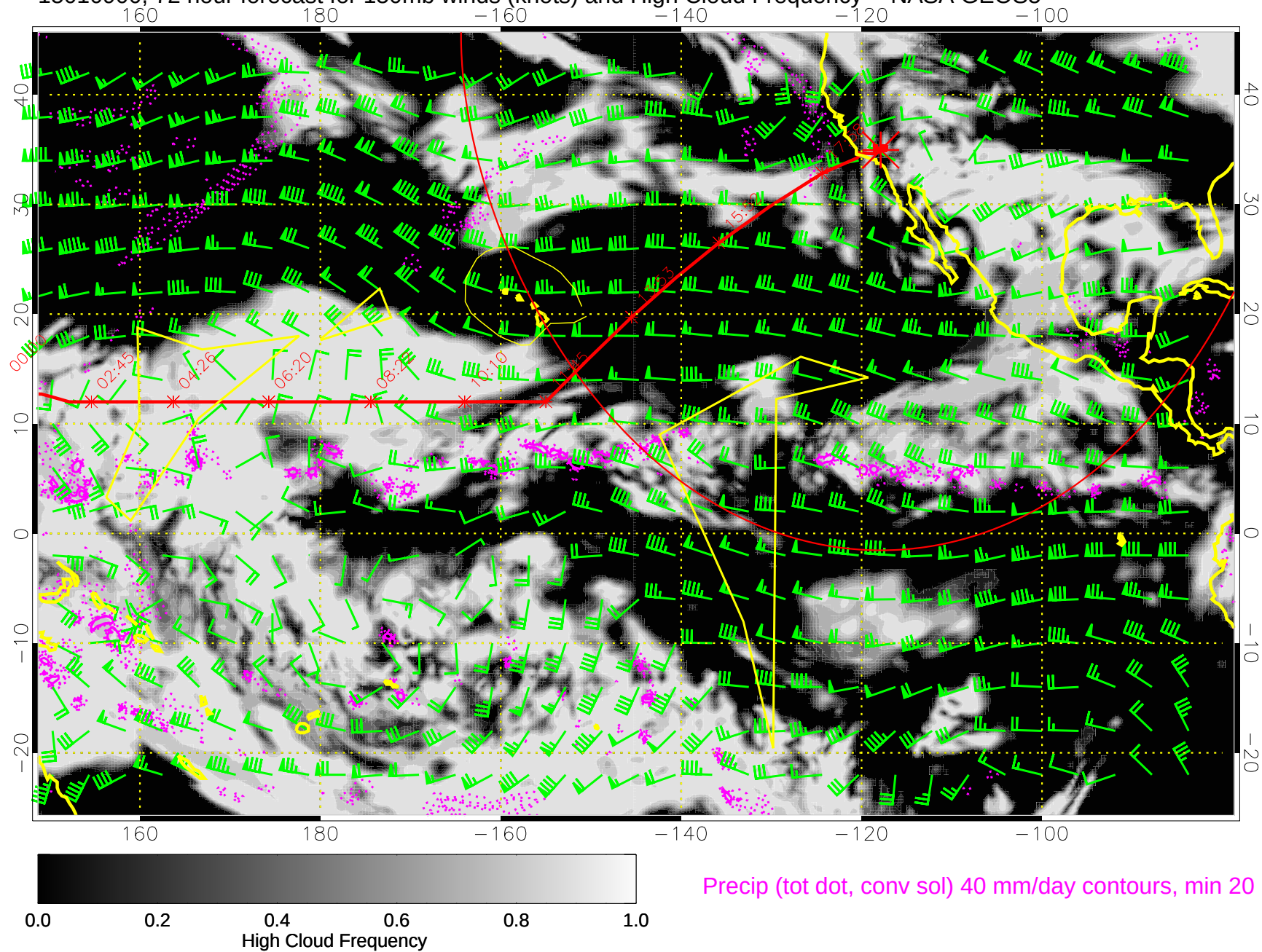
15010900, 72 hour forecast for 150mb winds (knots) and High Cloud Frequency -- NASA GEOS5
