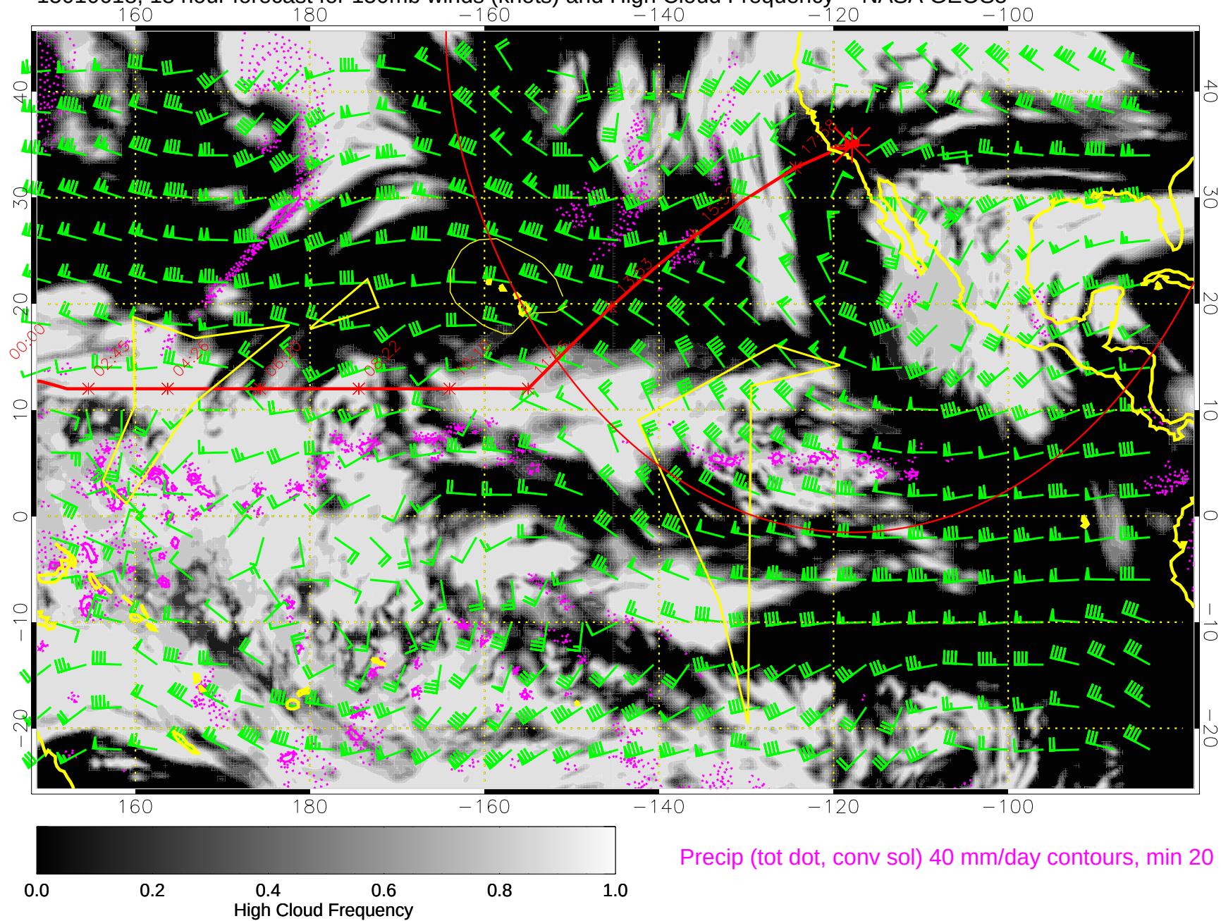
15010618, 18 hour forecast for 150mb winds (knots) and High Cloud Frequency -- NASA GEOS5
