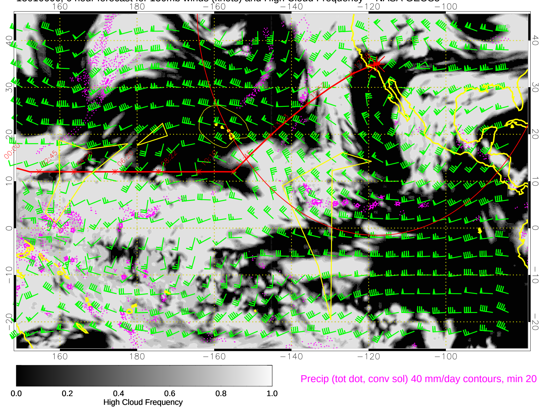
15010606, 6 hour forecast for 150mb winds (knots) and High Cloud Frequency -- NASA GEOS5
