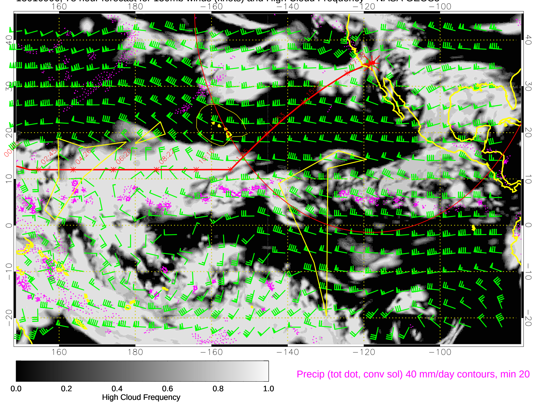
15010906, 78 hour forecast for 150mb winds (knots) and High Cloud Frequency -- NASA GEOS5
