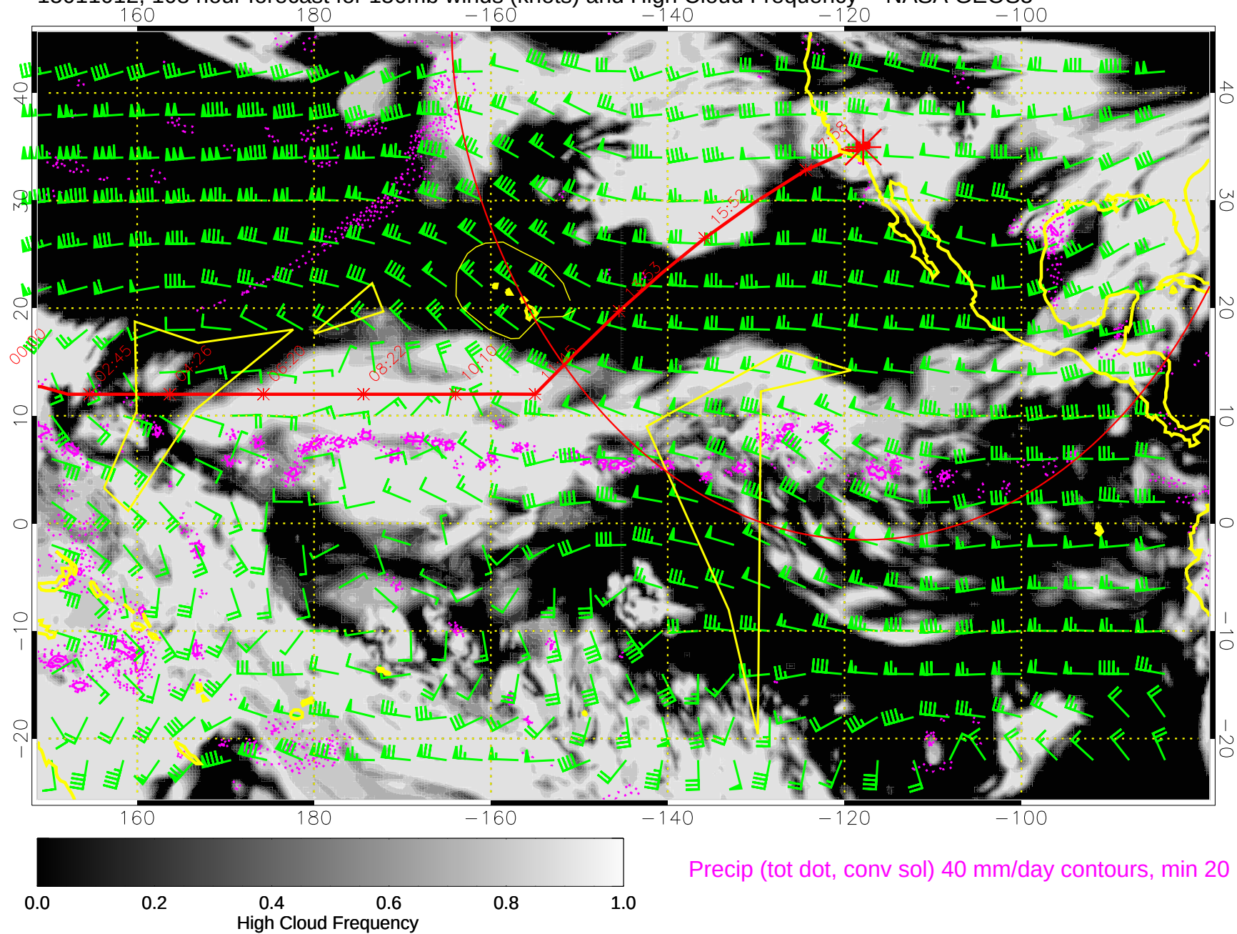
15011012, 108 hour forecast for 150mb winds (knots) and High Cloud Frequency -- NASA GEOS5
