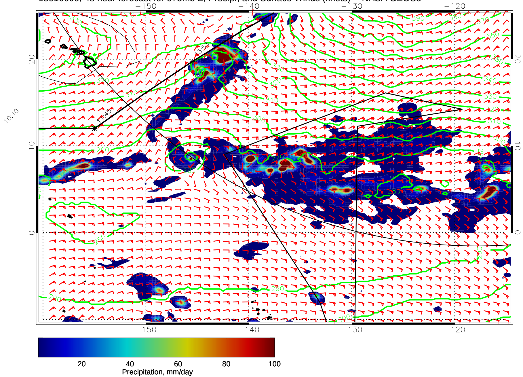
15010600, 48 hour forecast for 975mb Z, Precip., and Surface Winds (knots) -- NASA GEOS5
