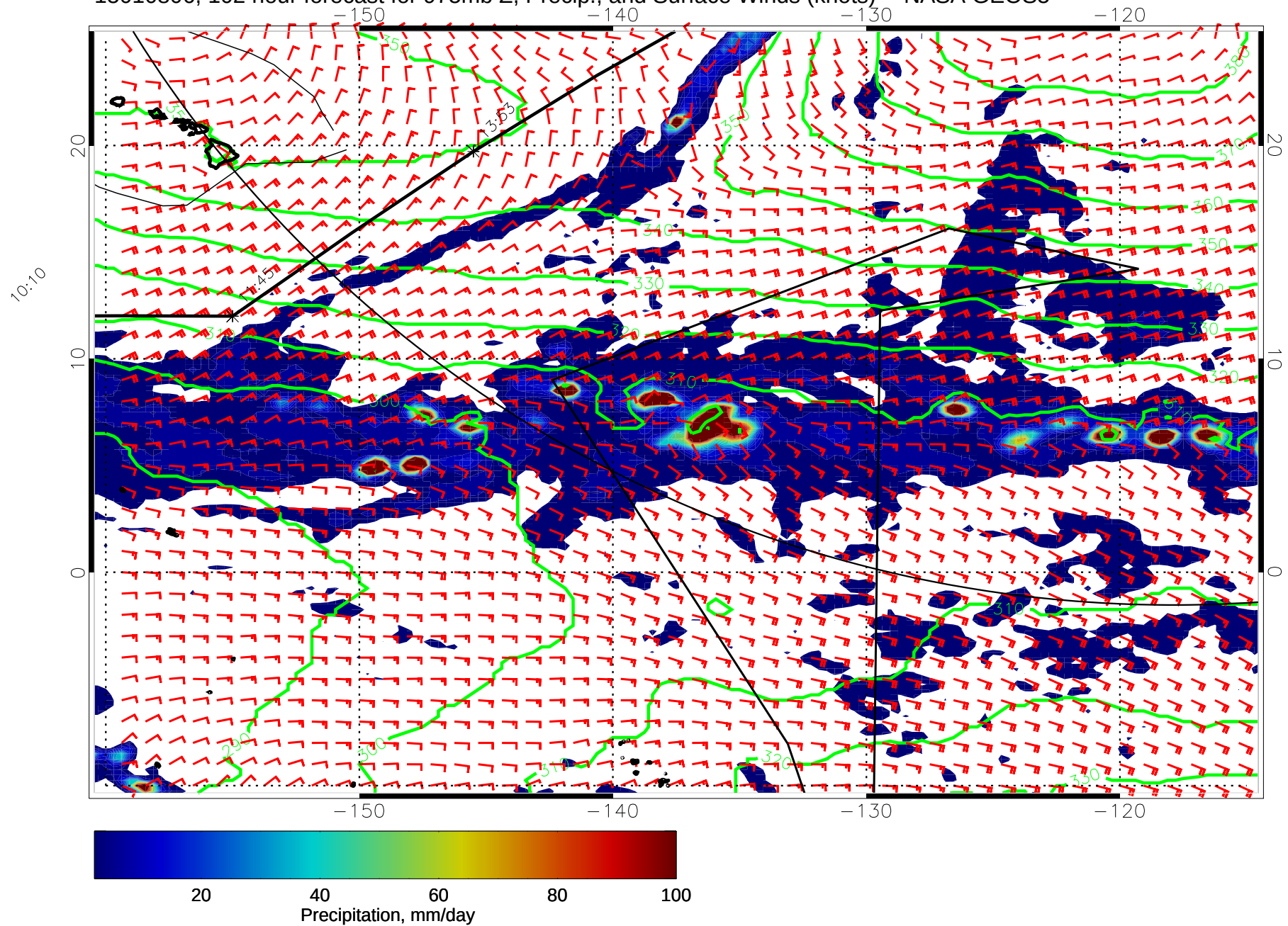
15010806, 102 hour forecast for 975mb Z, Precip., and Surface Winds (knots) -- NASA GEOS5
