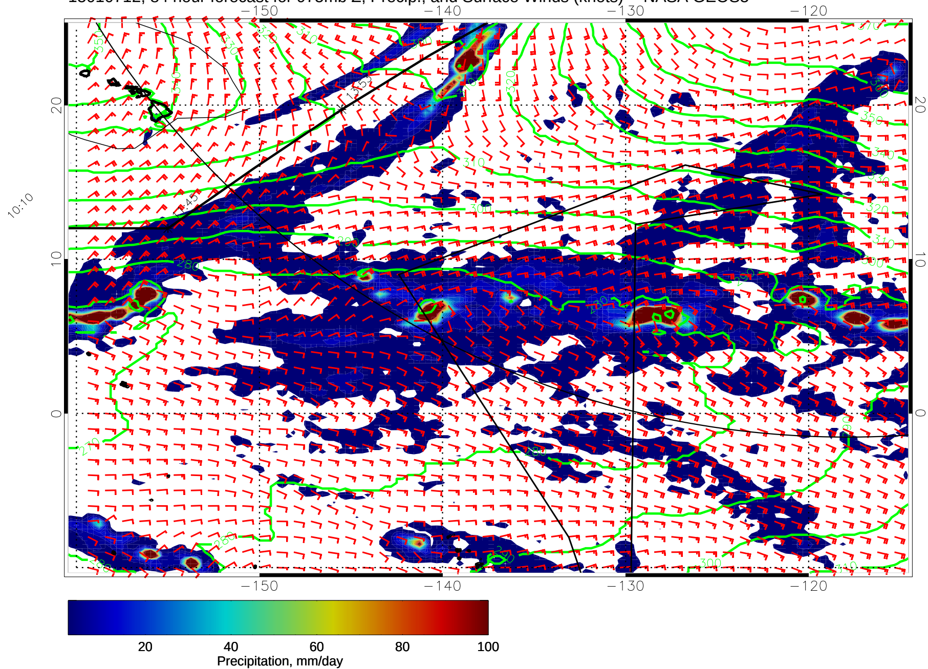
15010712, 84 hour forecast for 975mb Z, Precip., and Surface Winds (knots) -- NASA GEOS5
