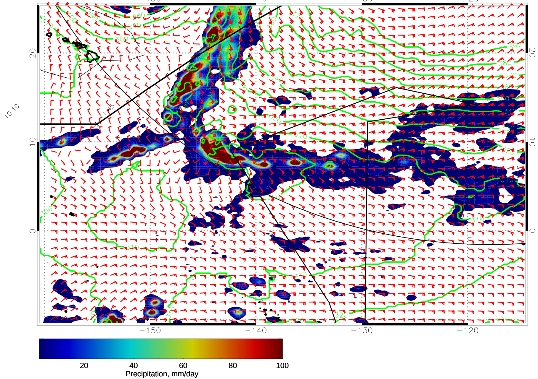
15010418, 18 hour forecast for 975mb Z, Precip., and Surface Winds (knots) -- NASA GEOS5
