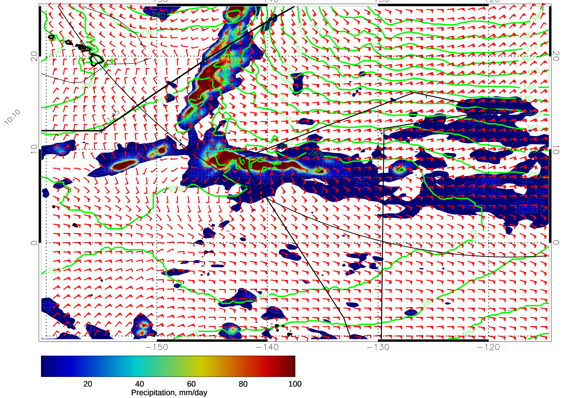
15010500, 24 hour forecast for 975mb Z, Precip., and Surface Winds (knots) -- NASA GEOS5
