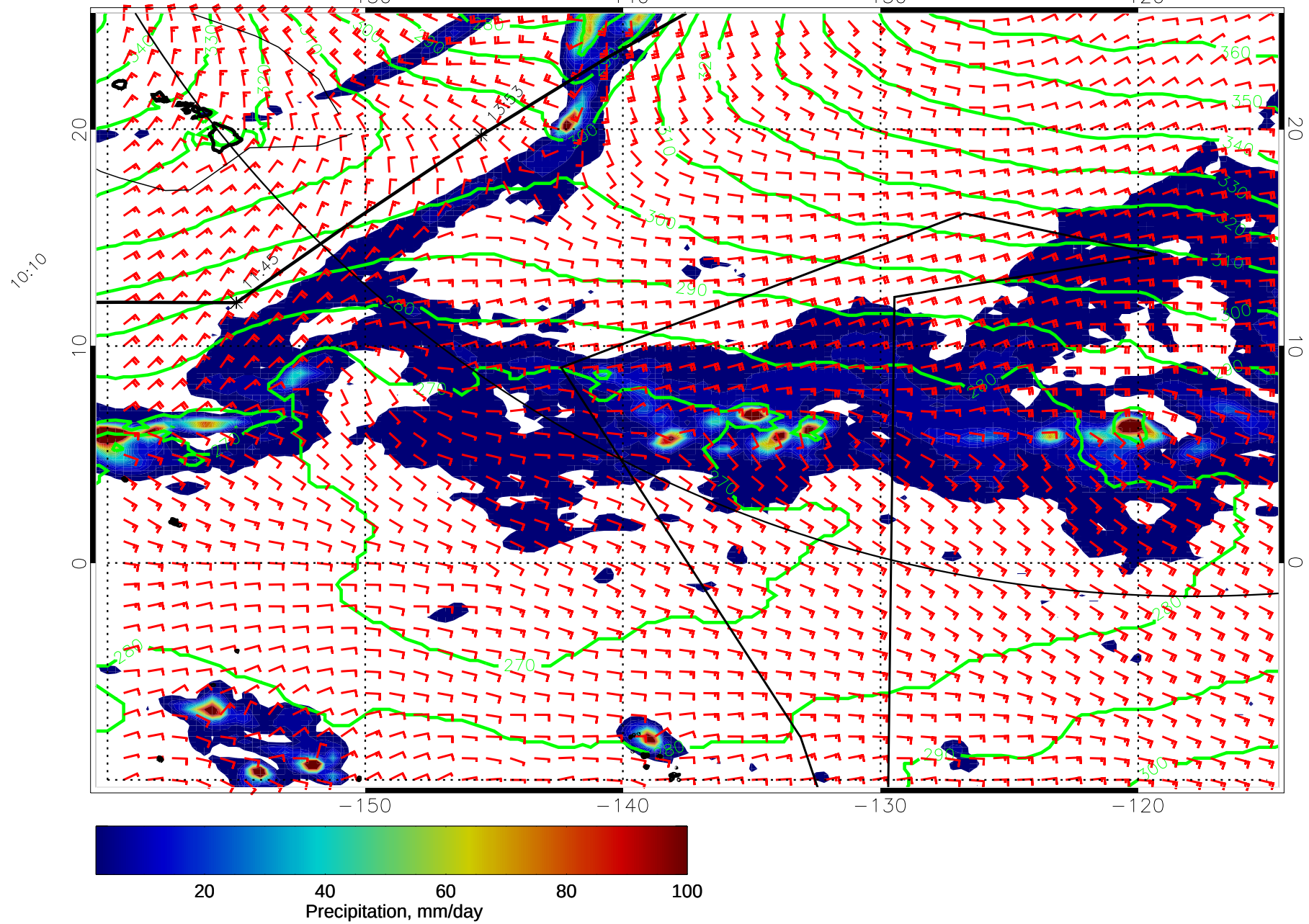
15010700, 72 hour forecast for 975mb Z, Precip., and Surface Winds (knots) -- NASA GEOS5
