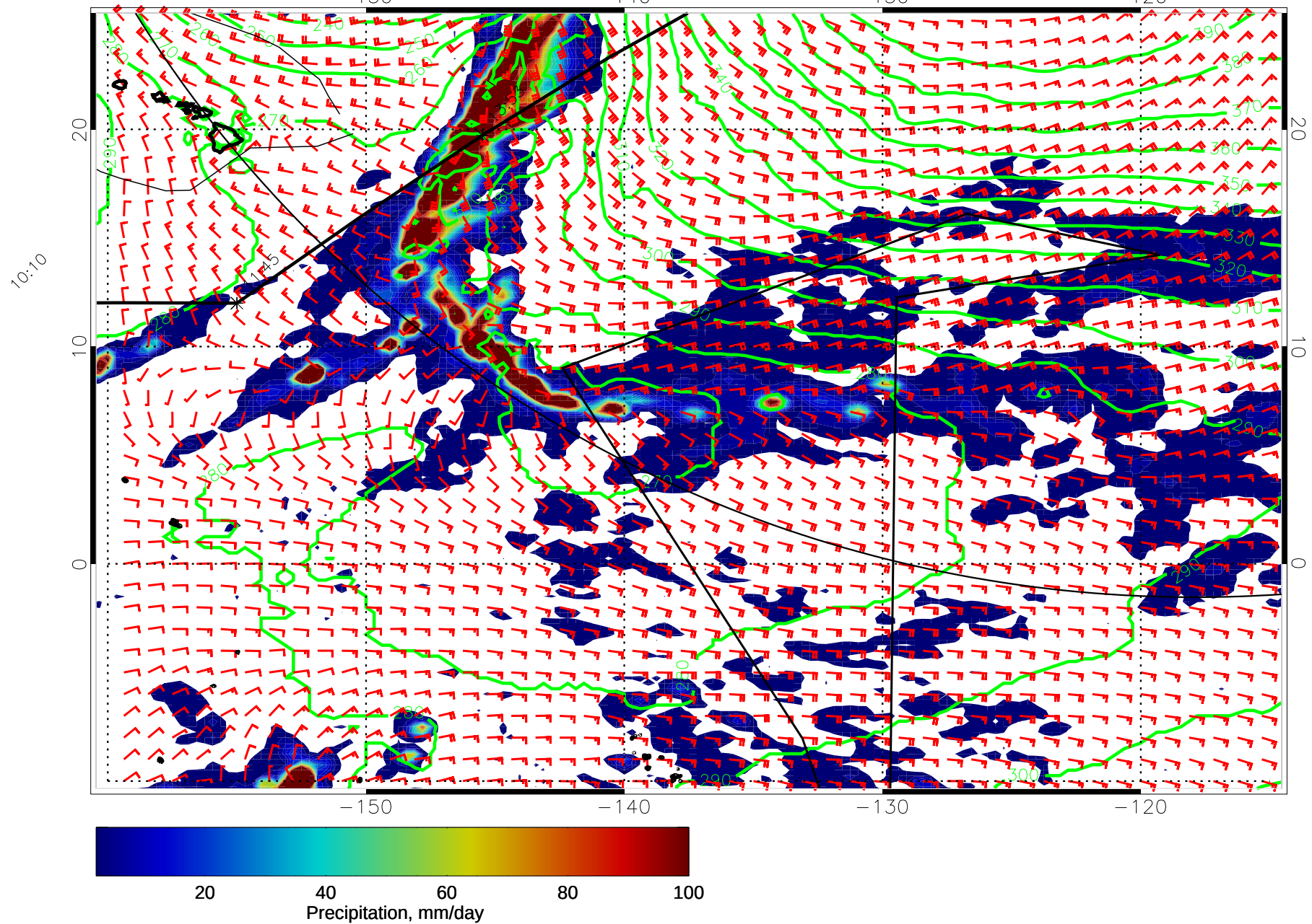
15010412, 12 hour forecast for 975mb Z, Precip., and Surface Winds (knots) -- NASA GEOS5
