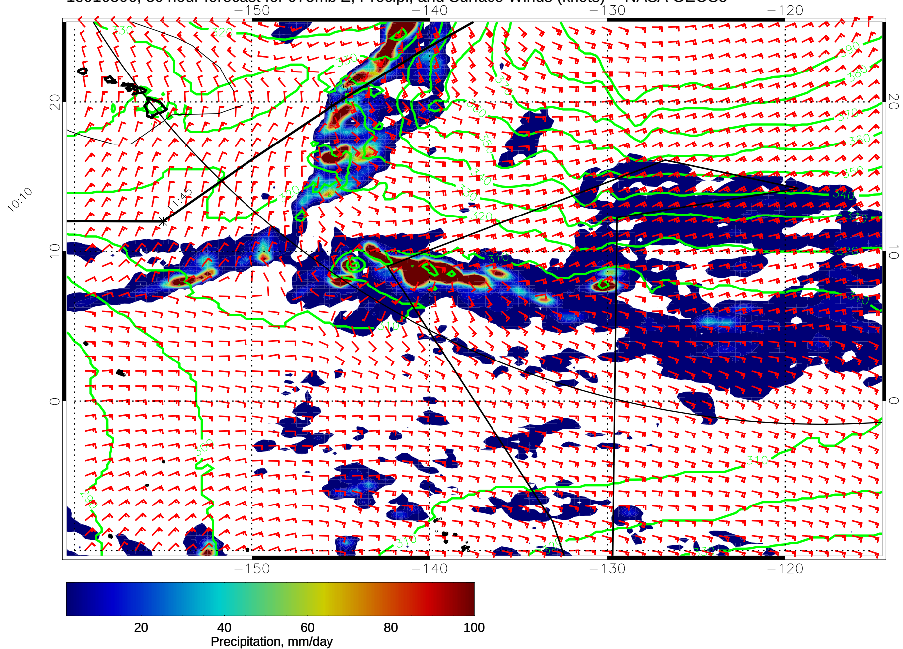
15010506, 30 hour forecast for 975mb Z, Precip., and Surface Winds (knots) -- NASA GEOS5
