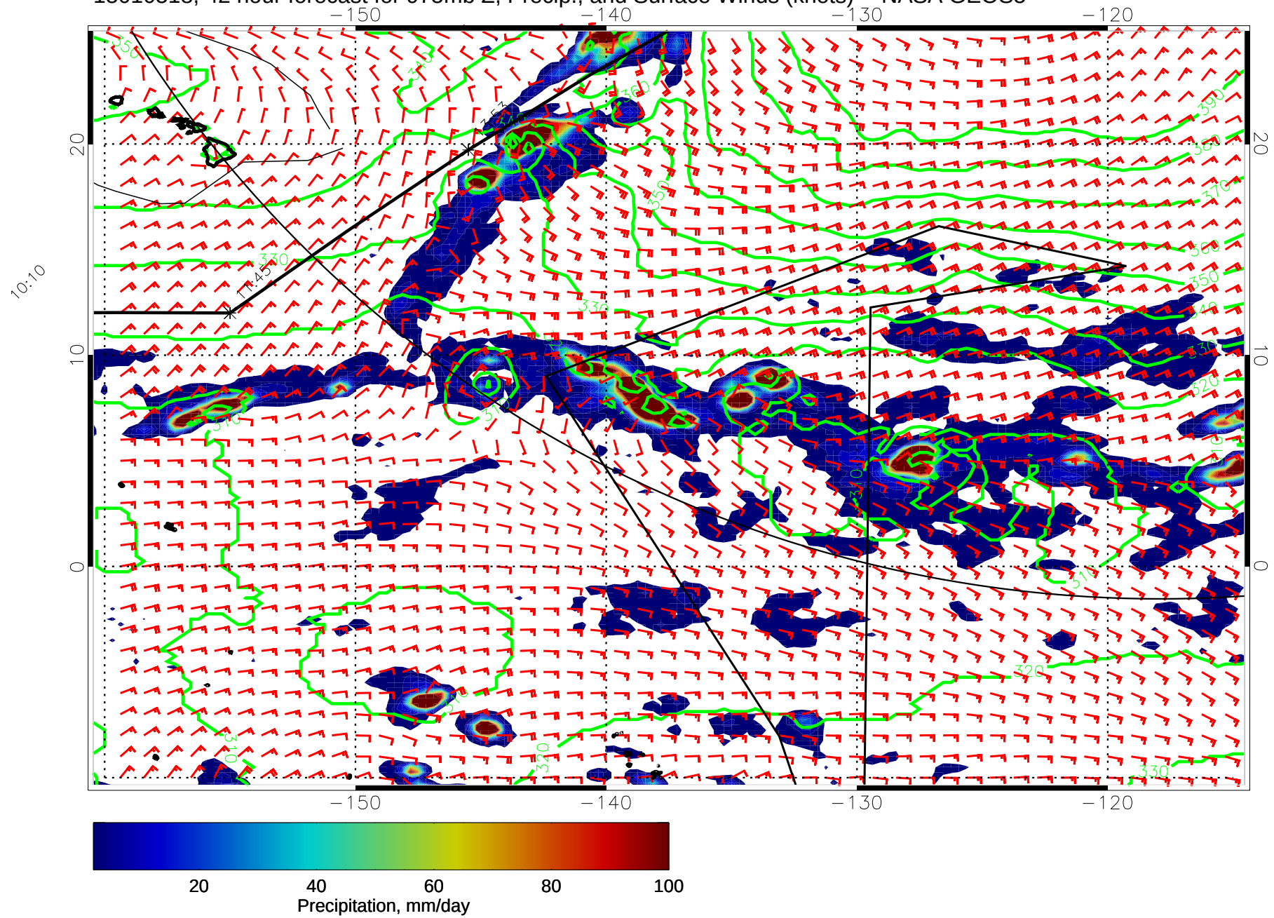
15010518, 42 hour forecast for 975mb Z, Precip., and Surface Winds (knots) -- NASA GEOS5
