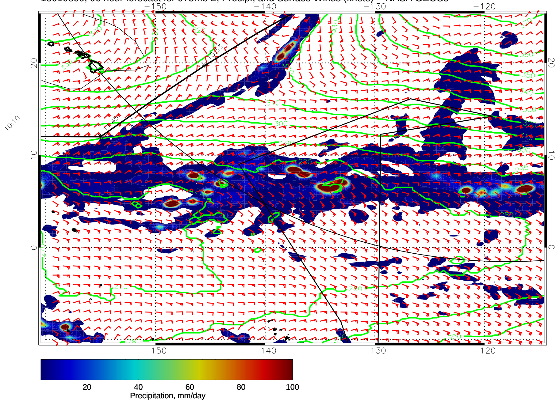
15010800, 96 hour forecast for 975mb Z, Precip., and Surface Winds (knots) -- NASA GEOS5
