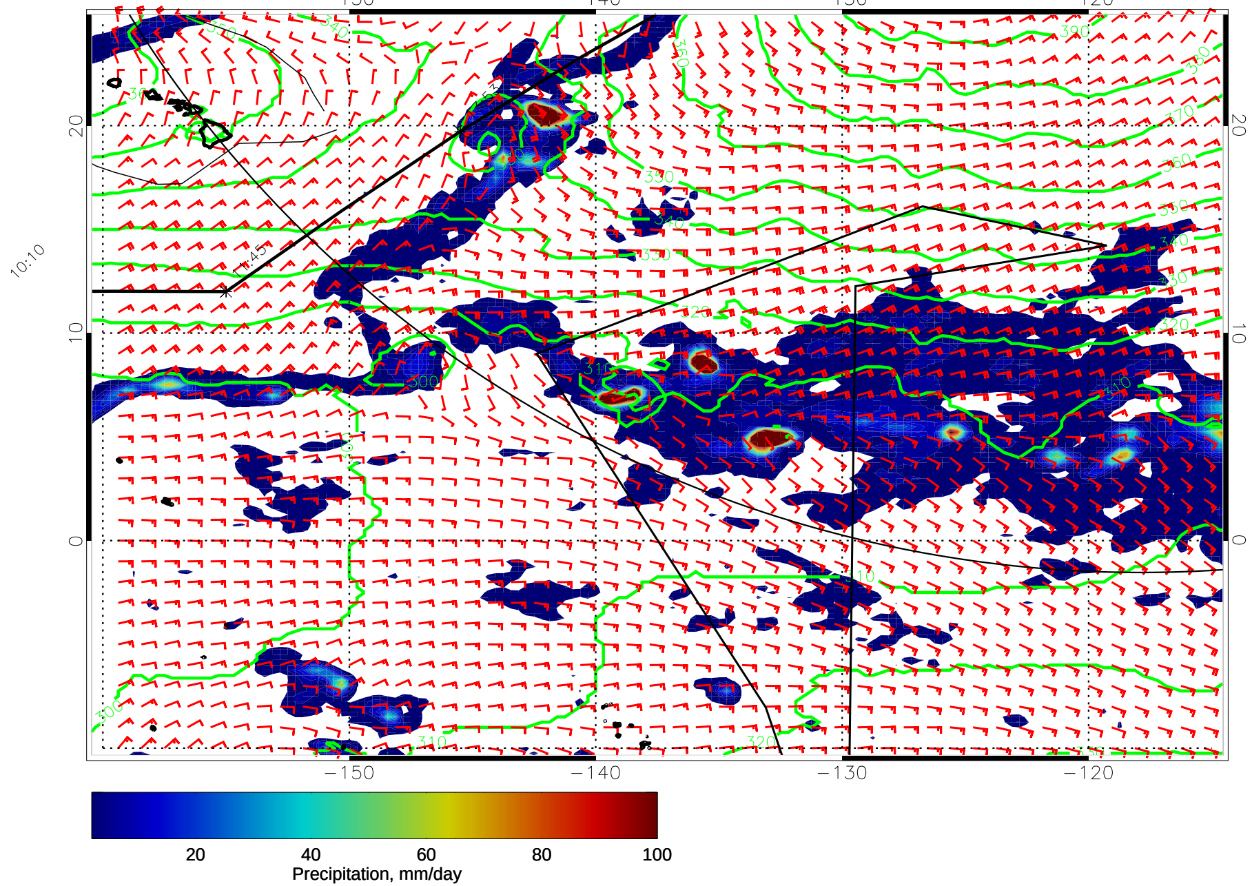
15010606, 54 hour forecast for 975mb Z, Precip., and Surface Winds (knots) -- NASA GEOS5
