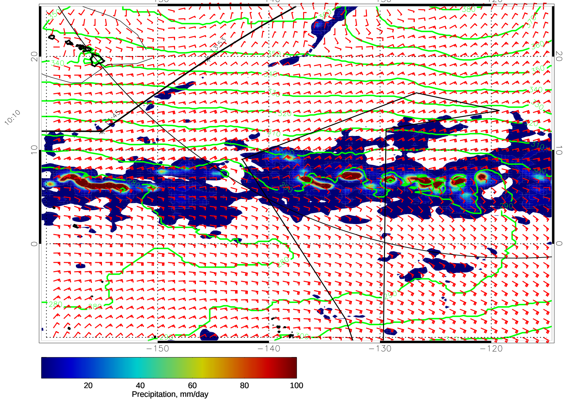
15010900, 120 hour forecast for 975mb Z, Precip., and Surface Winds (knots) -- NASA GEOS5
