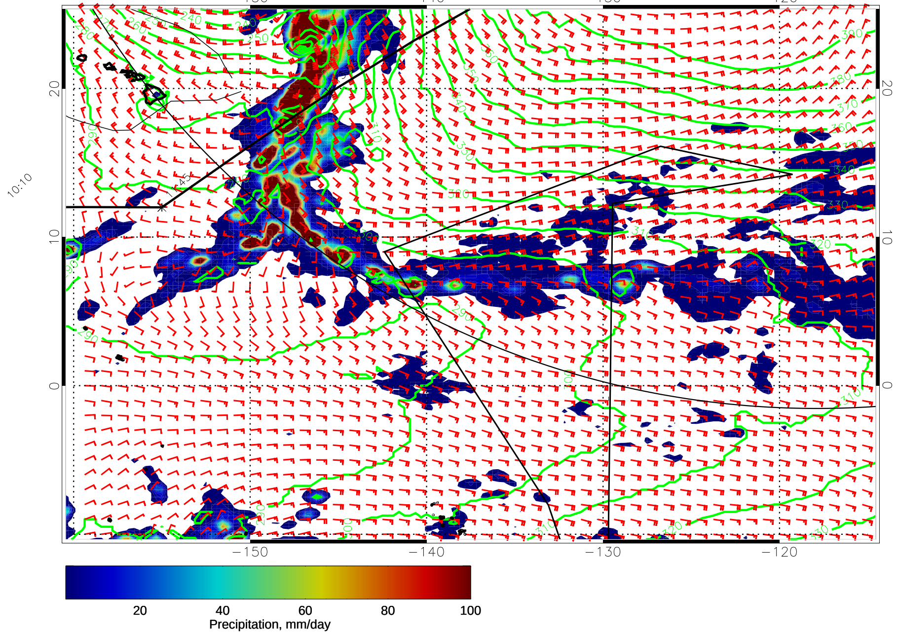
15010406, 6 hour forecast for 975mb Z, Precip., and Surface Winds (knots) -- NASA GEOS5
