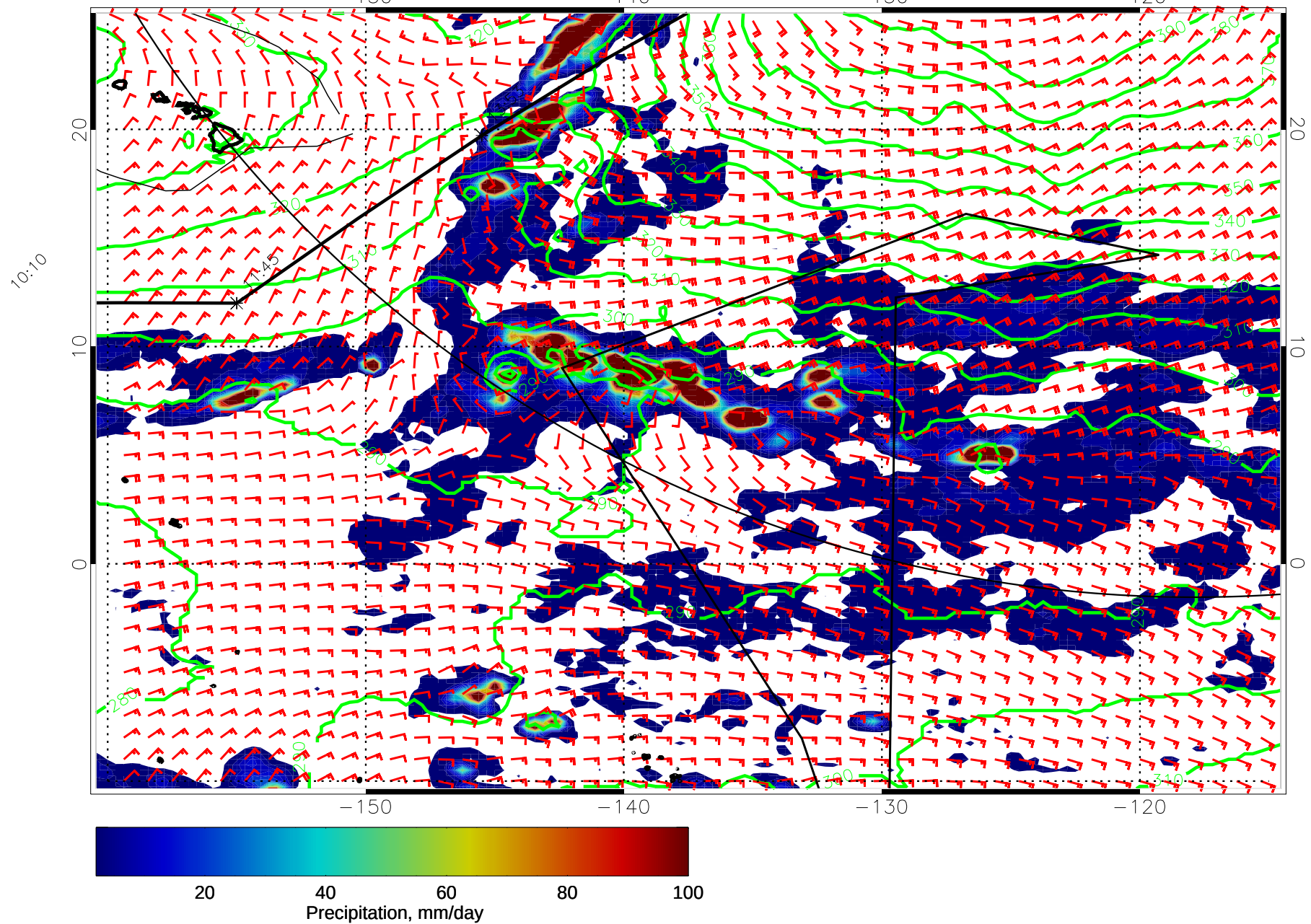
15010512, 36 hour forecast for 975mb Z, Precip., and Surface Winds (knots) -- NASA GEOS5
