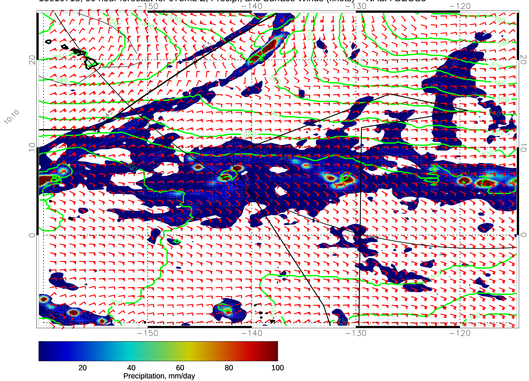
15010718, 90 hour forecast for 975mb Z, Precip., and Surface Winds (knots) -- NASA GEOS5
