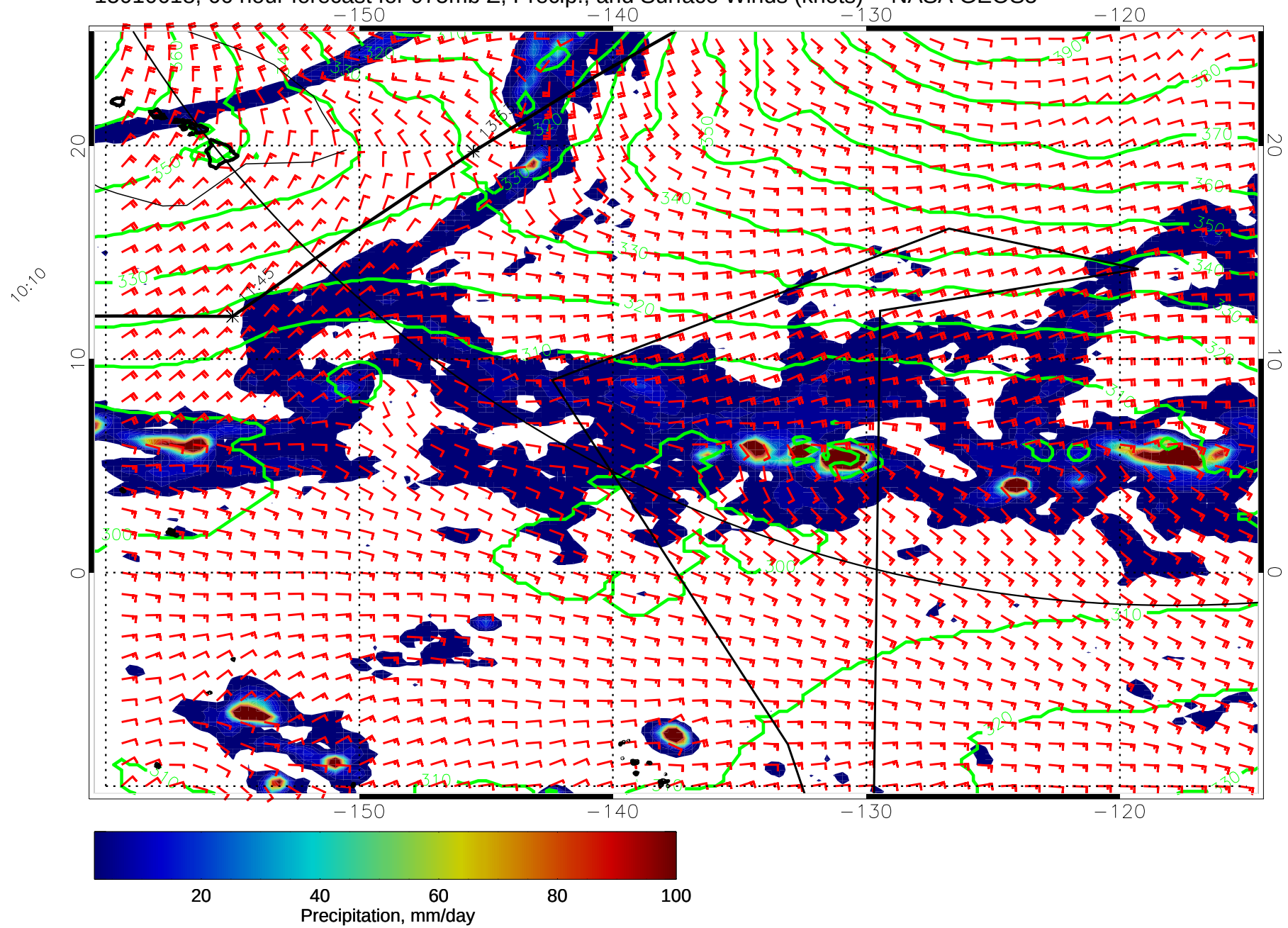
15010618, 66 hour forecast for 975mb Z, Precip., and Surface Winds (knots) -- NASA GEOS5
