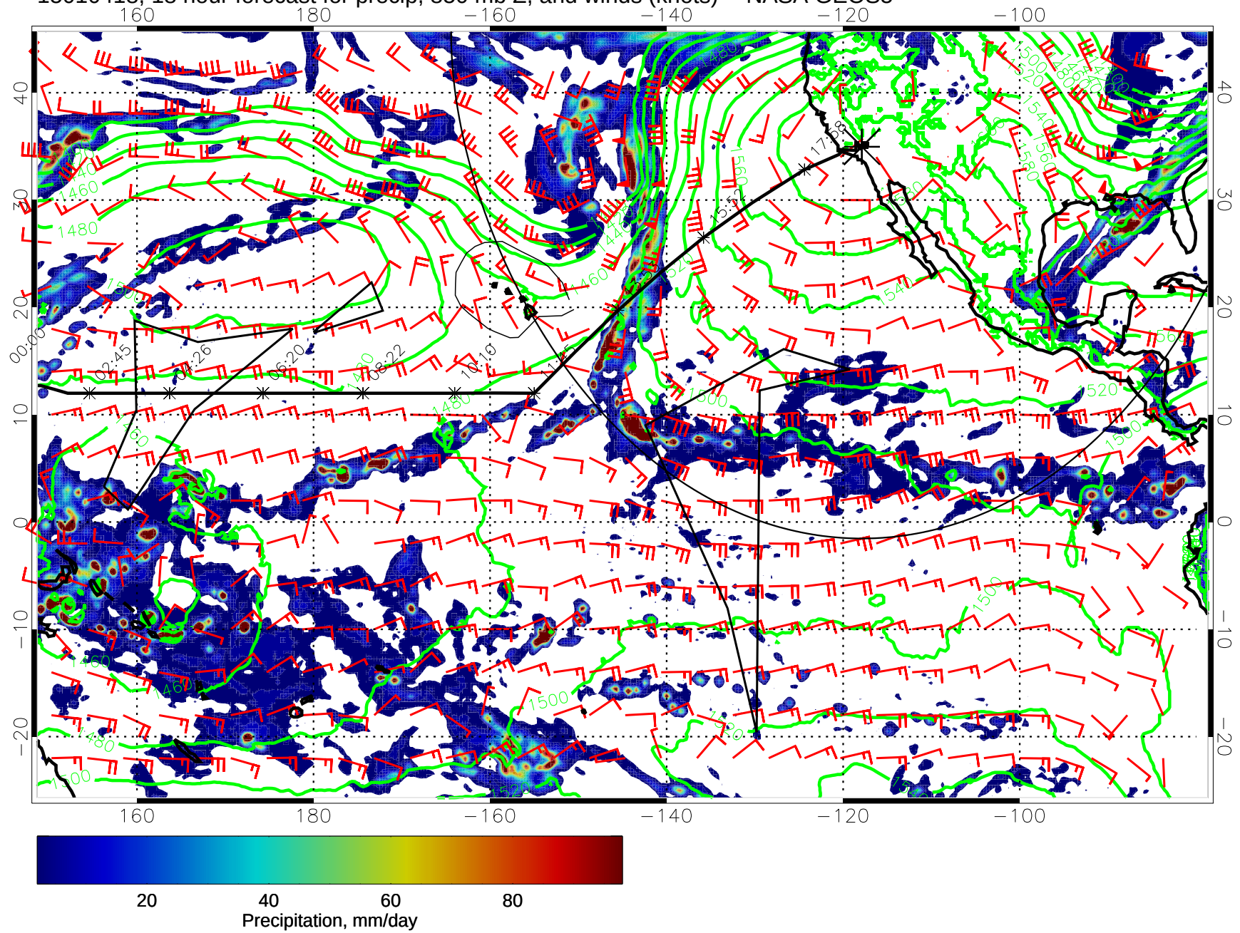
15010418, 18 hour forecast for precip, 850 mb Z, and winds (knots) -- NASA GEOS5
