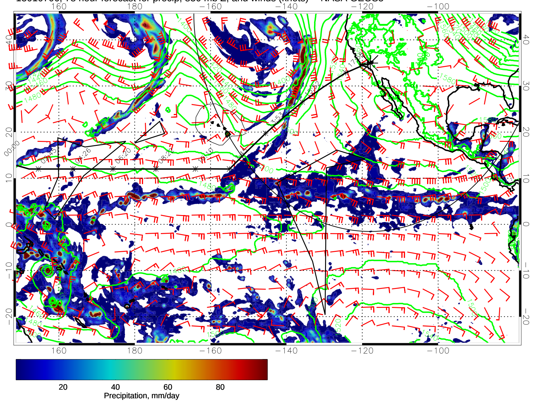
15010706, 78 hour forecast for precip, 850 mb Z, and winds (knots) -- NASA GEOS5
