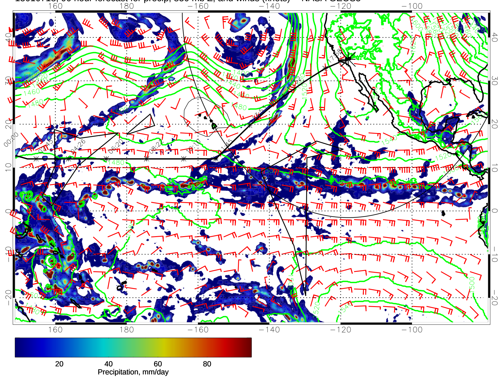
15010718, 90 hour forecast for precip, 850 mb Z, and winds (knots) -- NASA GEOS5
