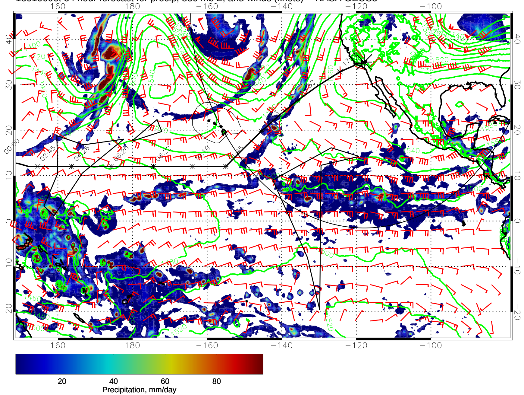
15010606, 54 hour forecast for precip, 850 mb Z, and winds (knots) -- NASA GEOS5
