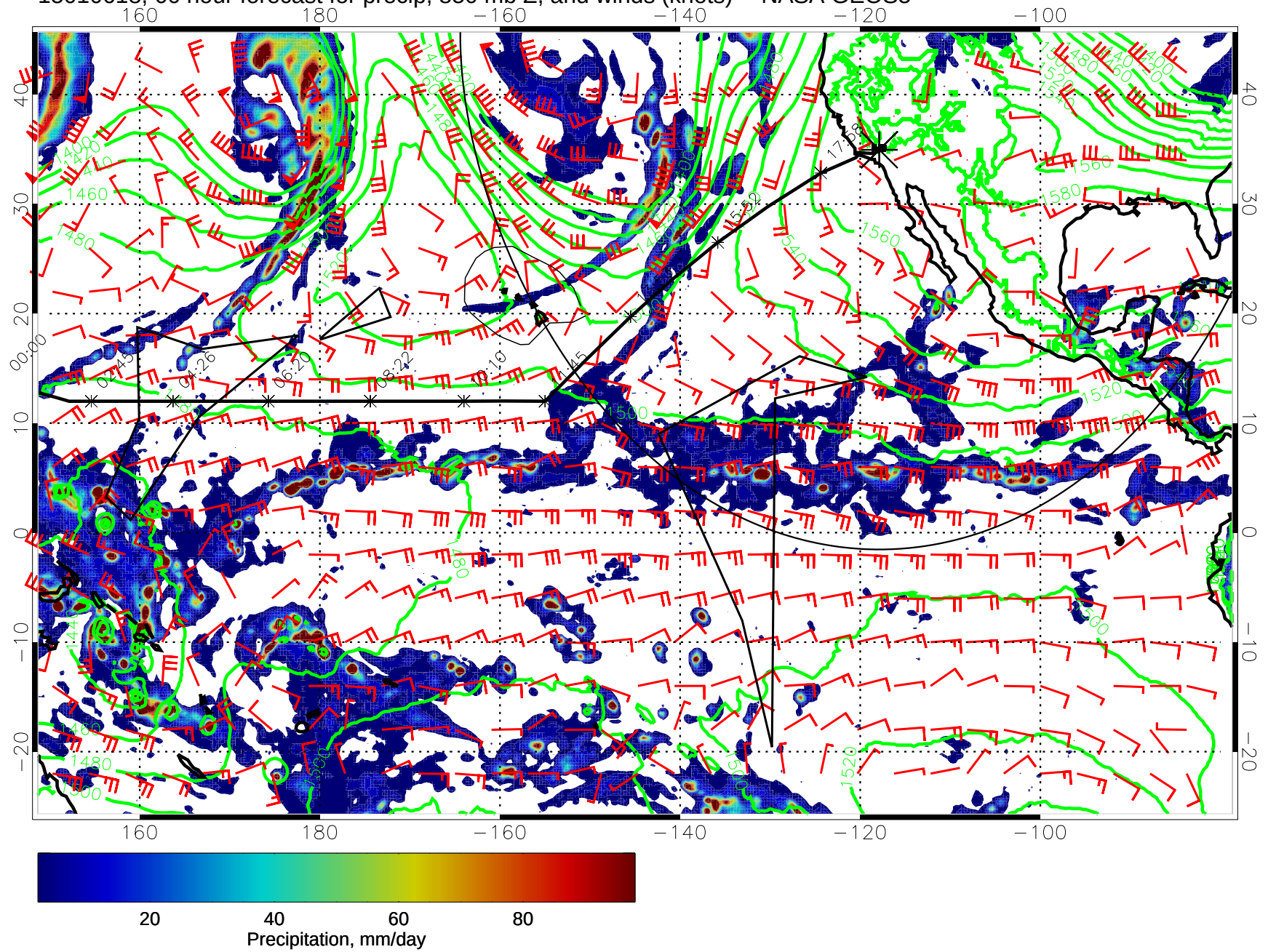
15010618, 66 hour forecast for precip, 850 mb Z, and winds (knots) -- NASA GEOS5
