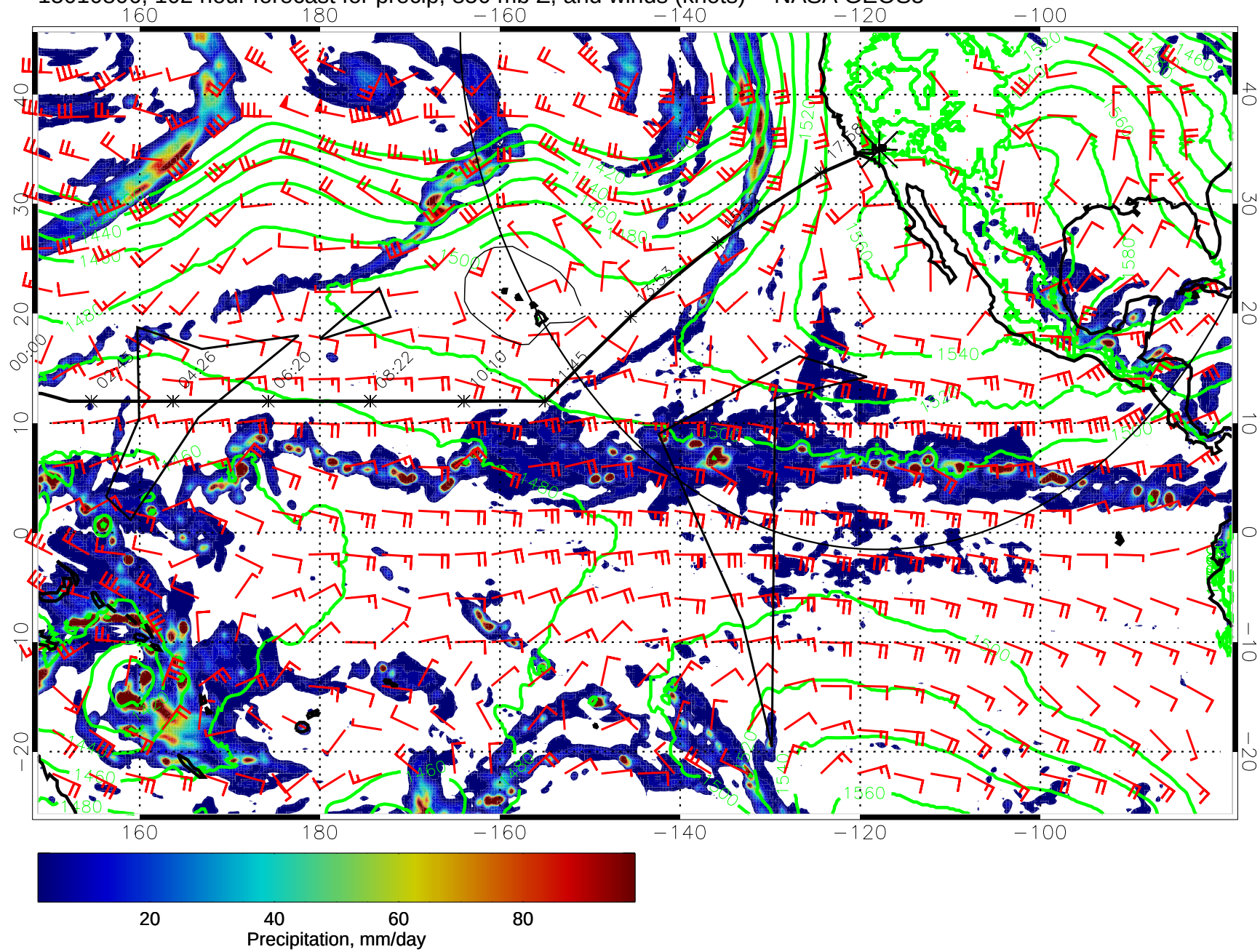
15010806, 102 hour forecast for precip, 850 mb Z, and winds (knots) -- NASA GEOS5
