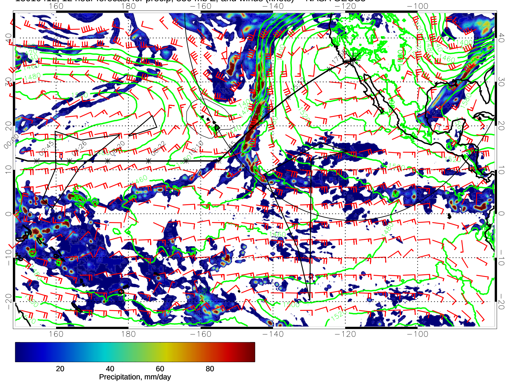
15010412, 12 hour forecast for precip, 850 mb Z, and winds (knots) -- NASA GEOS5
