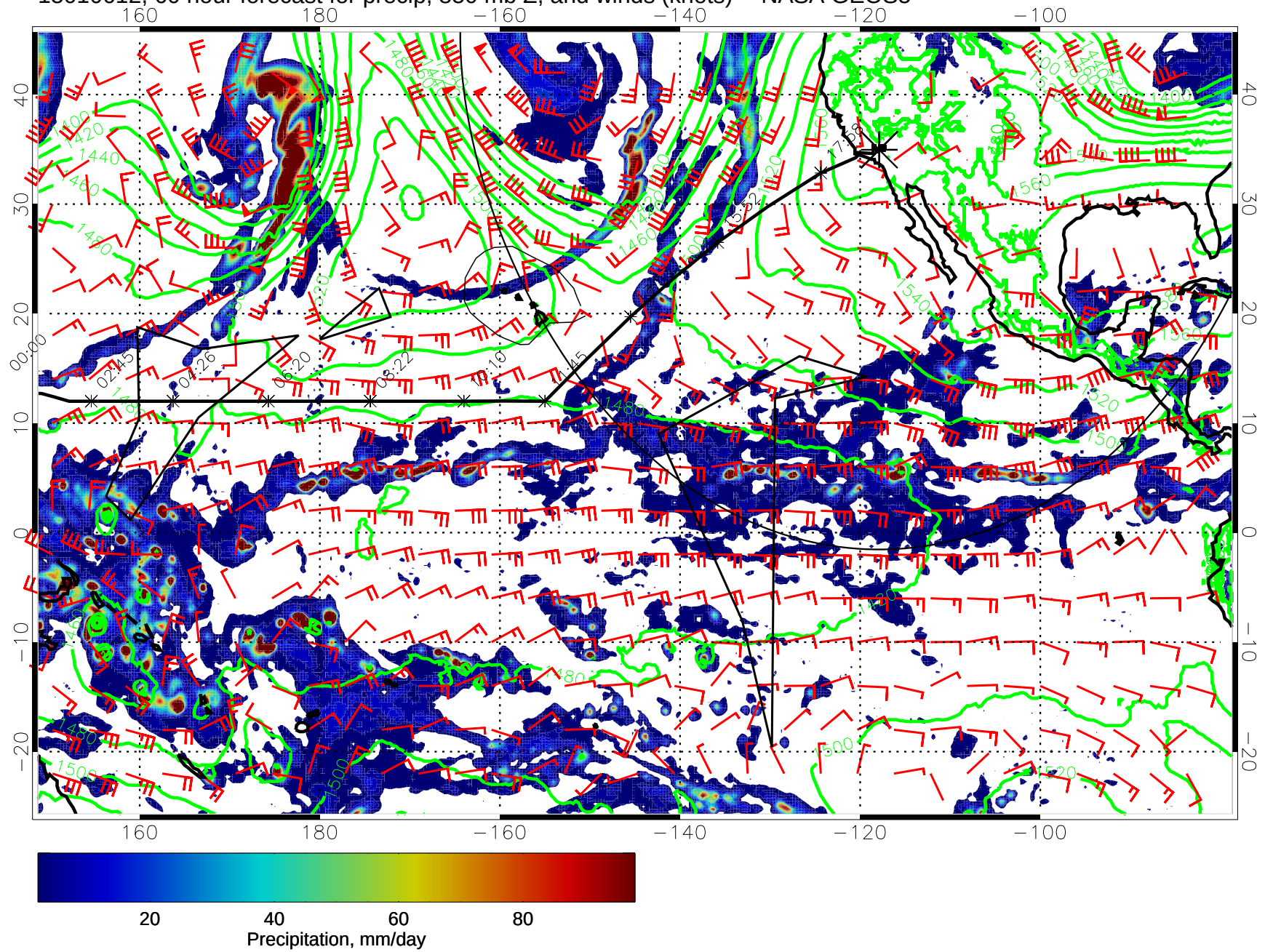
15010612, 60 hour forecast for precip, 850 mb Z, and winds (knots) -- NASA GEOS5
