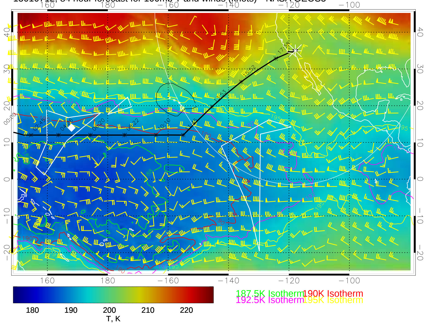
15010712, 84 hour forecast for 100mb T and winds (knots)-- NASA GEOS5
