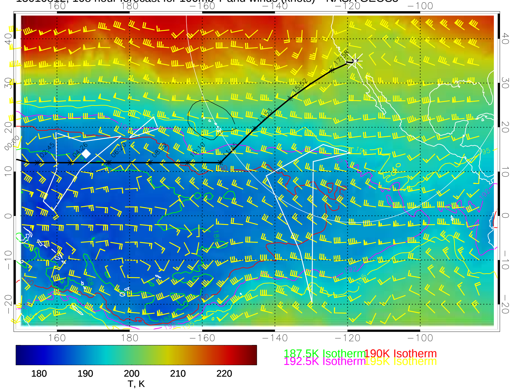
15010812, 108 hour forecast for 100mb T and winds (knots)-- NASA GEOS5
