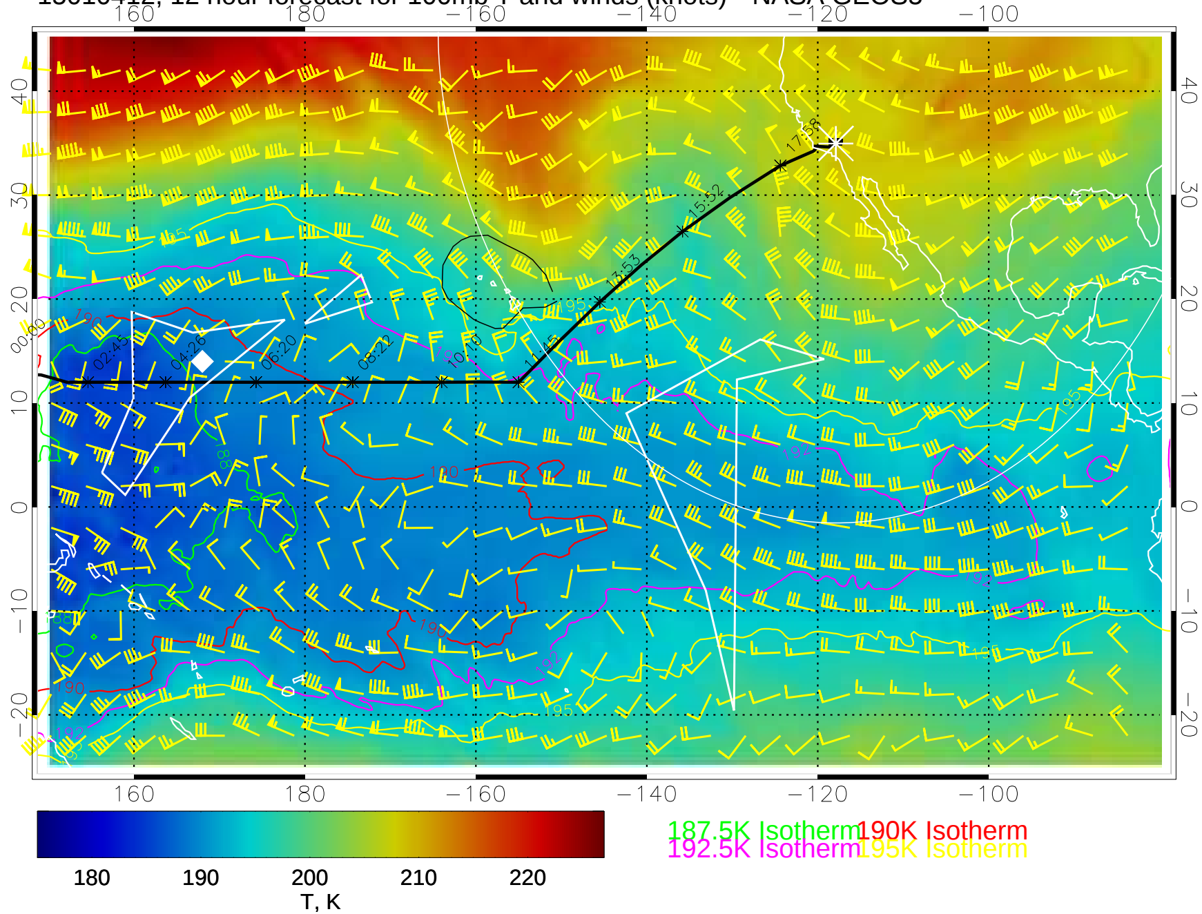
15010412, 12 hour forecast for 100mb T and winds (knots)-- NASA GEOS5
