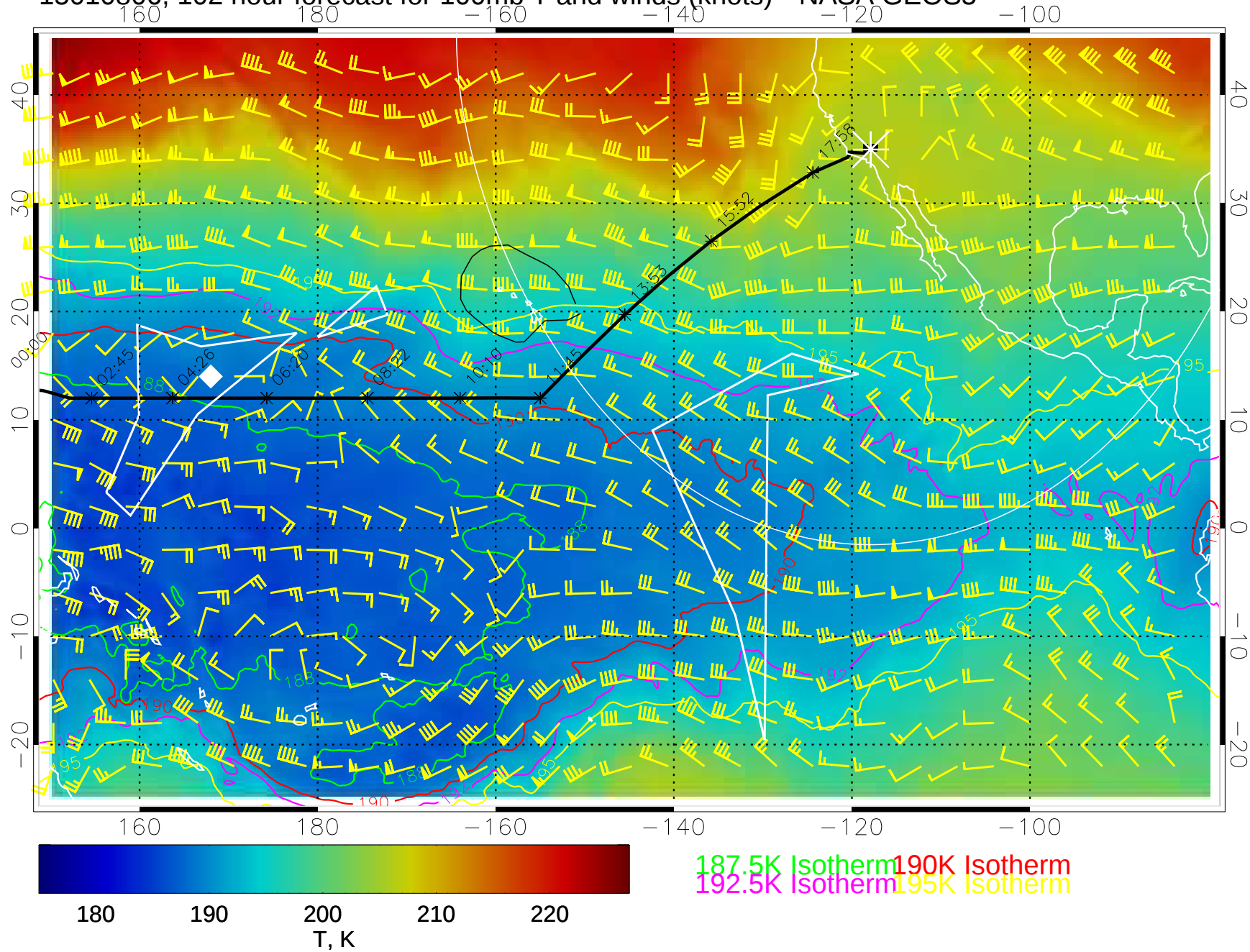
15010806, 102 hour forecast for 100mb T and winds (knots)-- NASA GEOS5
