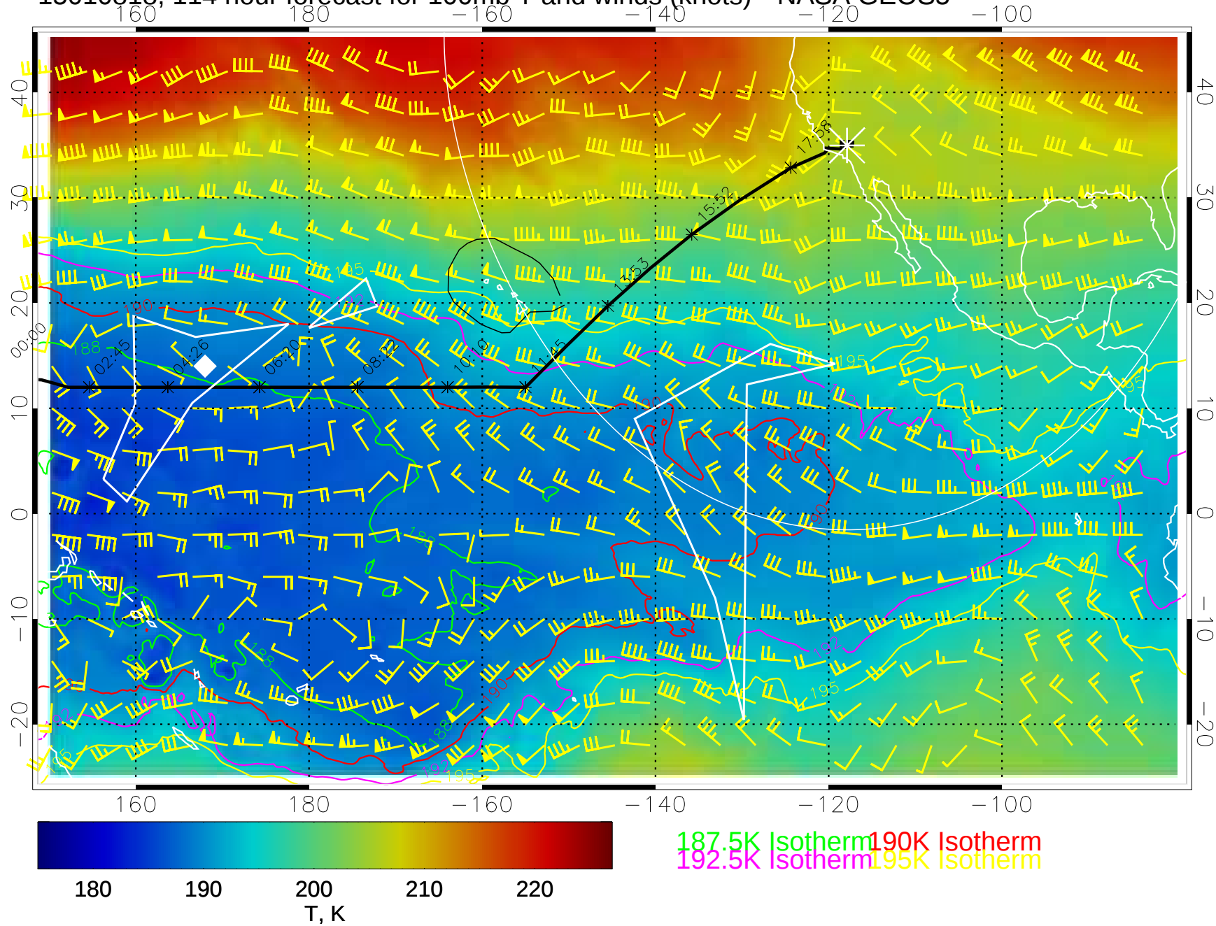
15010818, 114 hour forecast for 100mb T and winds (knots)-- NASA GEOS5
