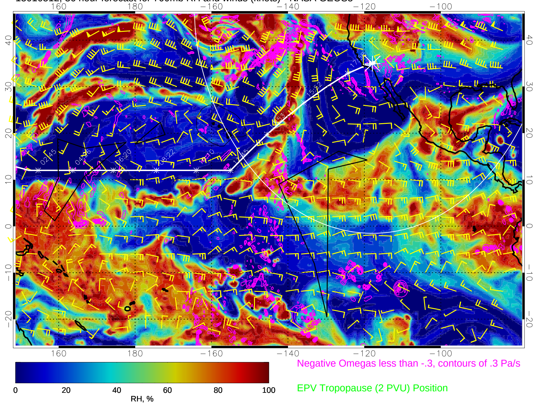
15010512, 36 hour forecast for 700mb RH and winds (knots) - NASA GEOS5
