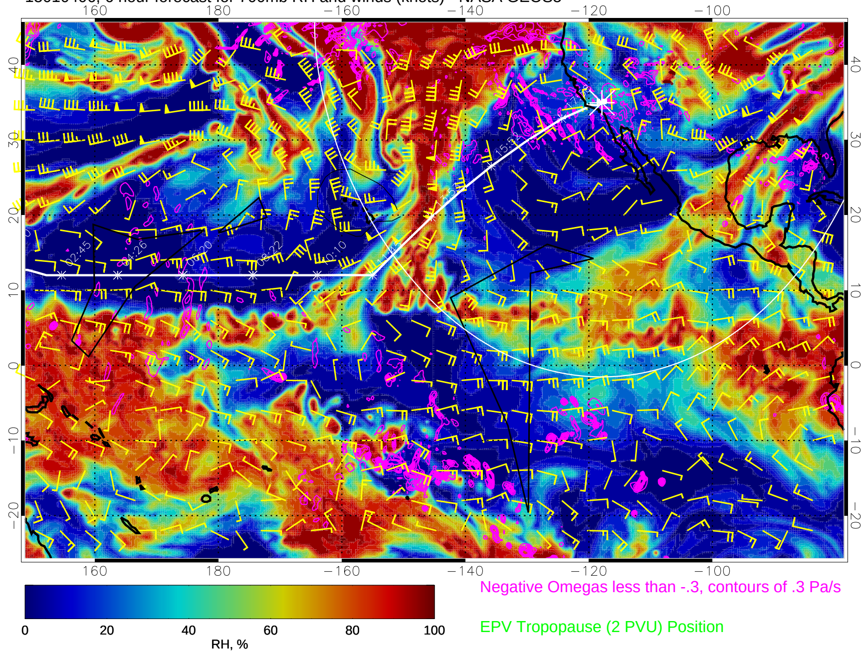
15010406, 6 hour forecast for 700mb RH and winds (knots) - NASA GEOS5
