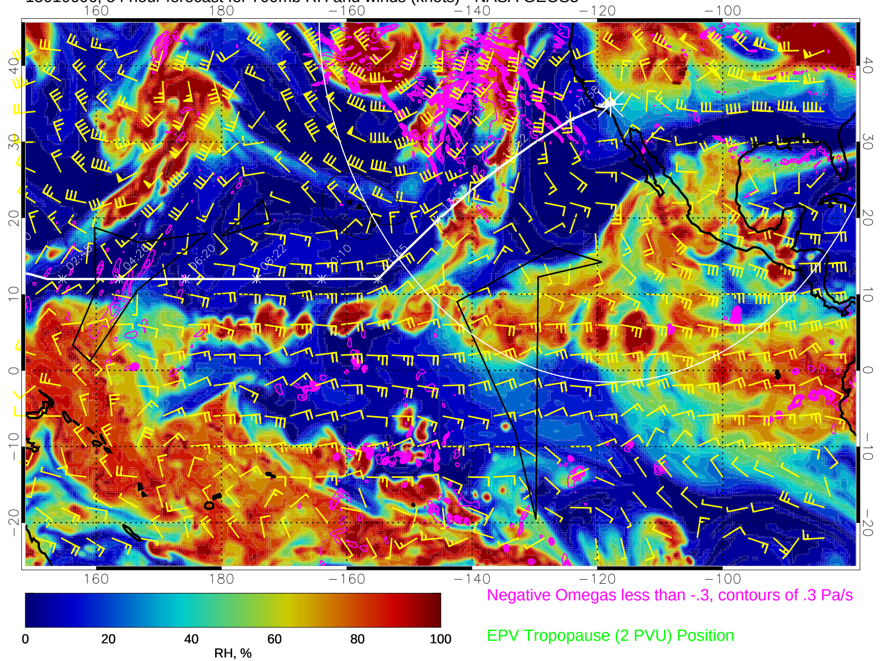
15010606, 54 hour forecast for 700mb RH and winds (knots) - NASA GEOS5
