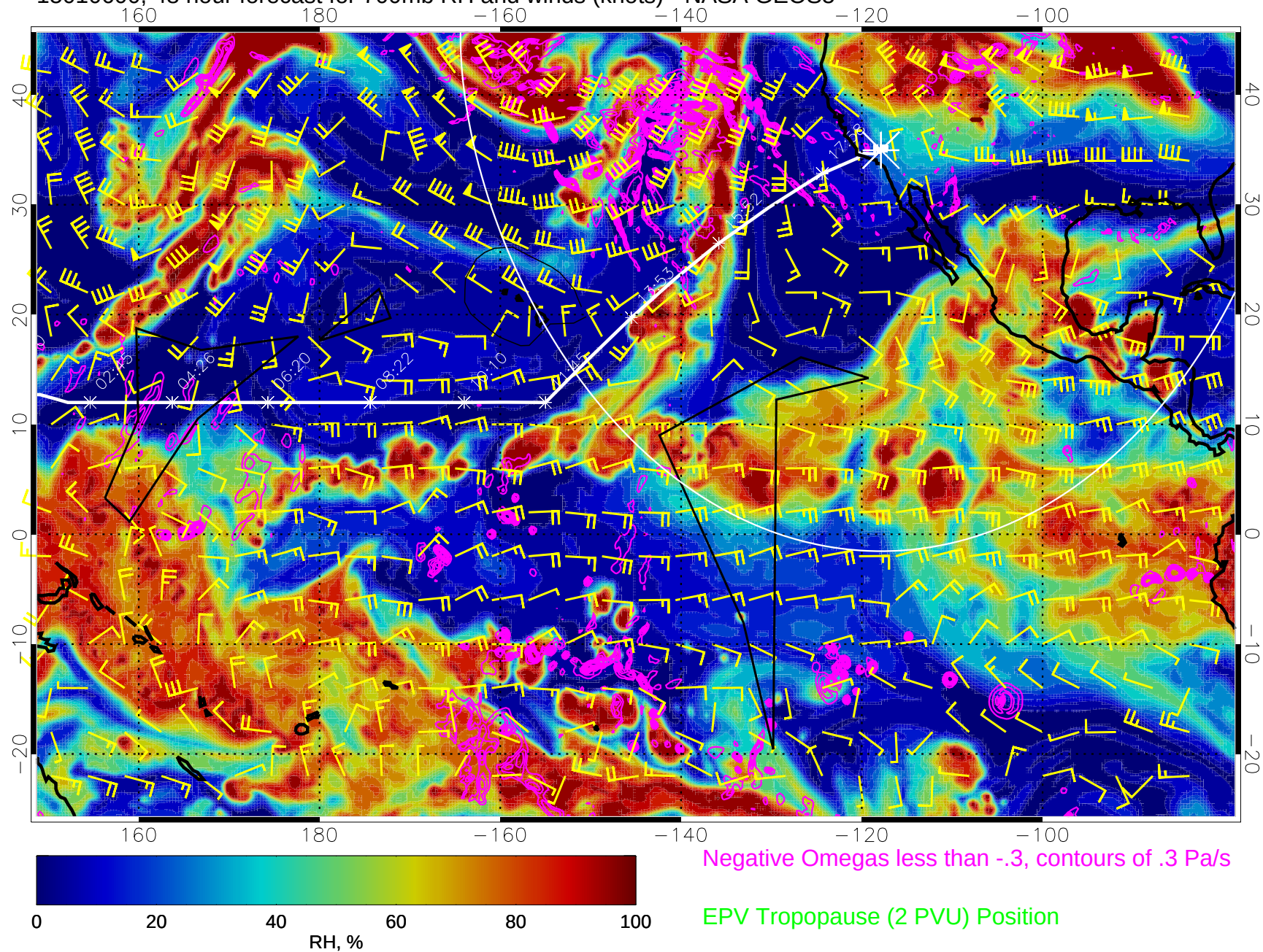
15010600, 48 hour forecast for 700mb RH and winds (knots) - NASA GEOS5
