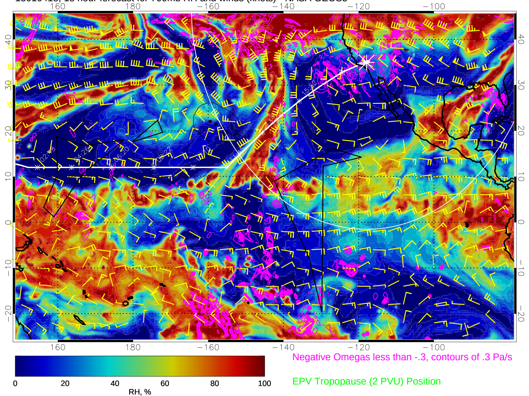
15010418, 18 hour forecast for 700mb RH and winds (knots) - NASA GEOS5
