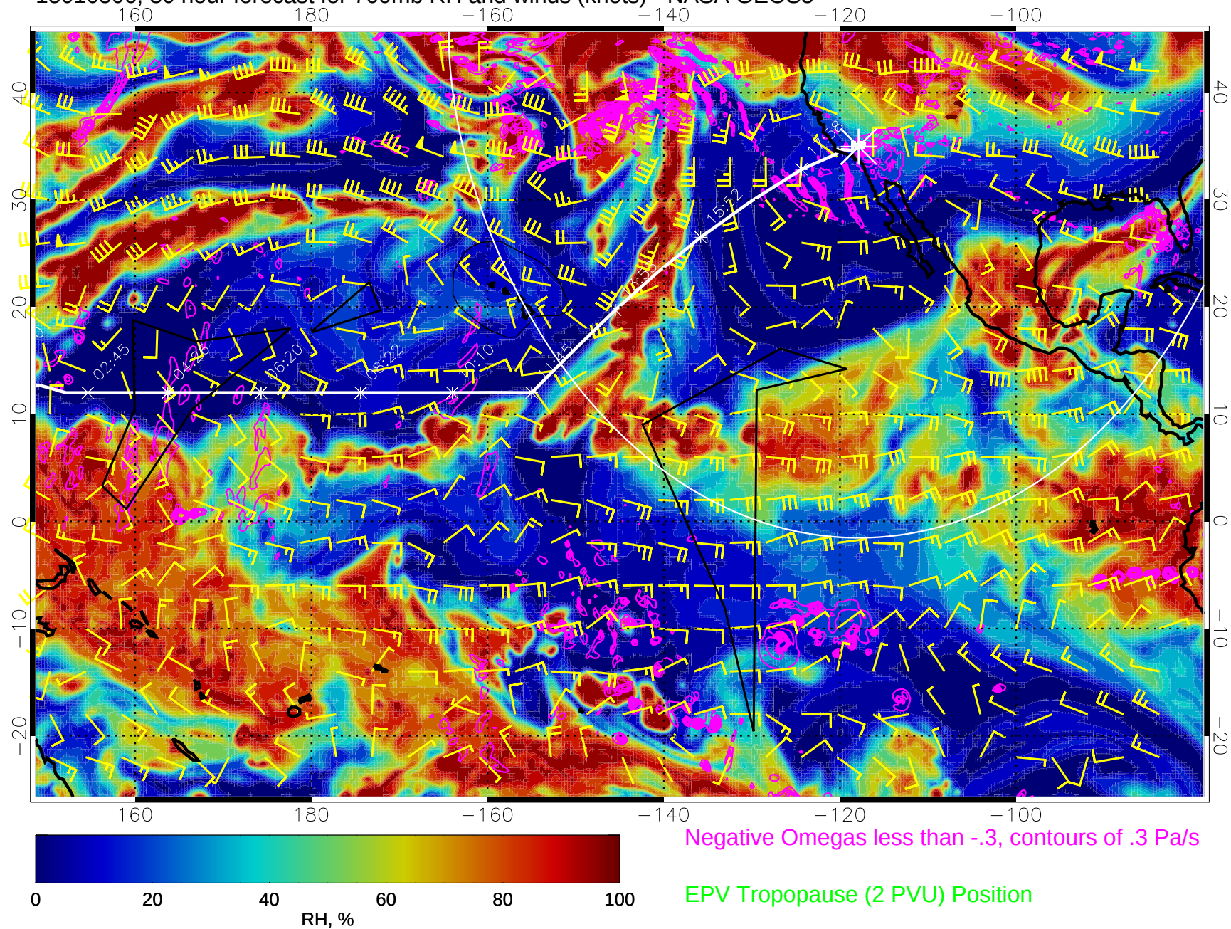
15010506, 30 hour forecast for 700mb RH and winds (knots) - NASA GEOS5
