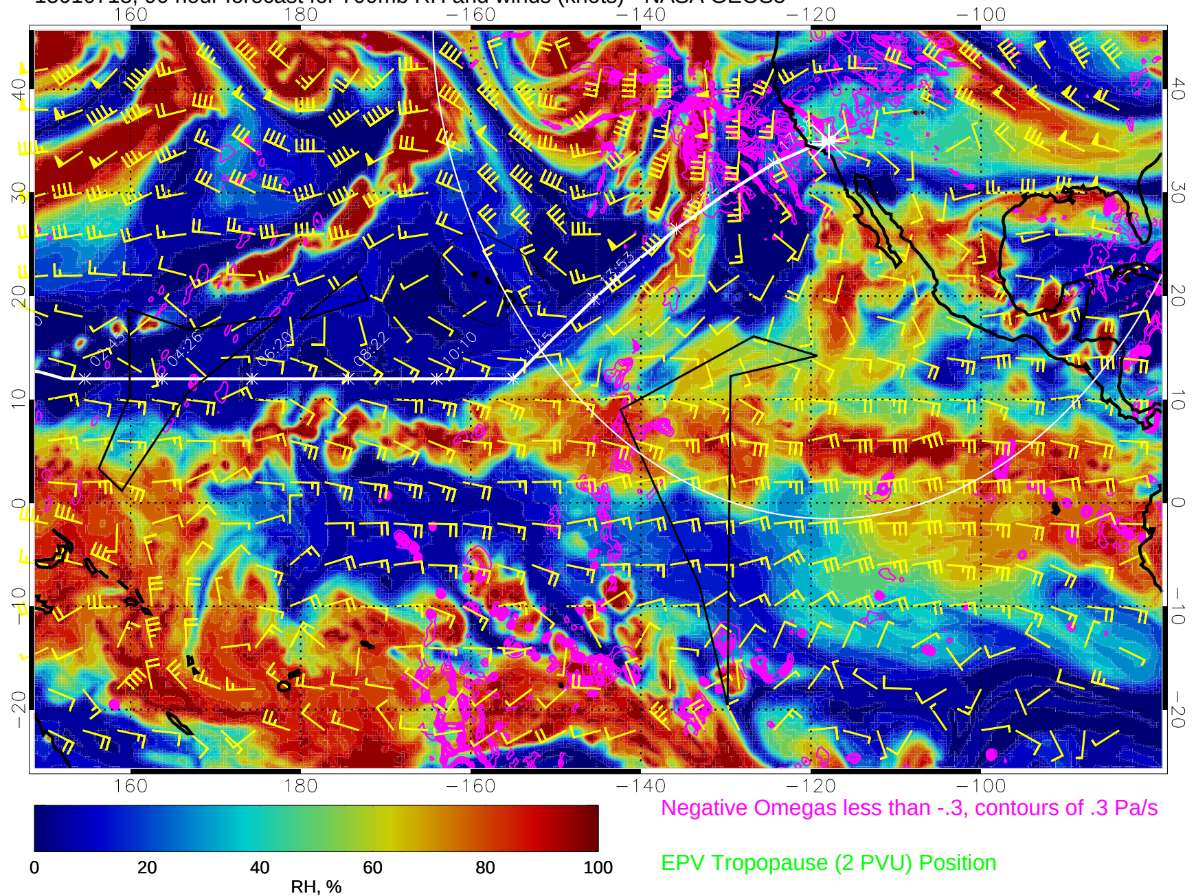
15010718, 90 hour forecast for 700mb RH and winds (knots) - NASA GEOS5
