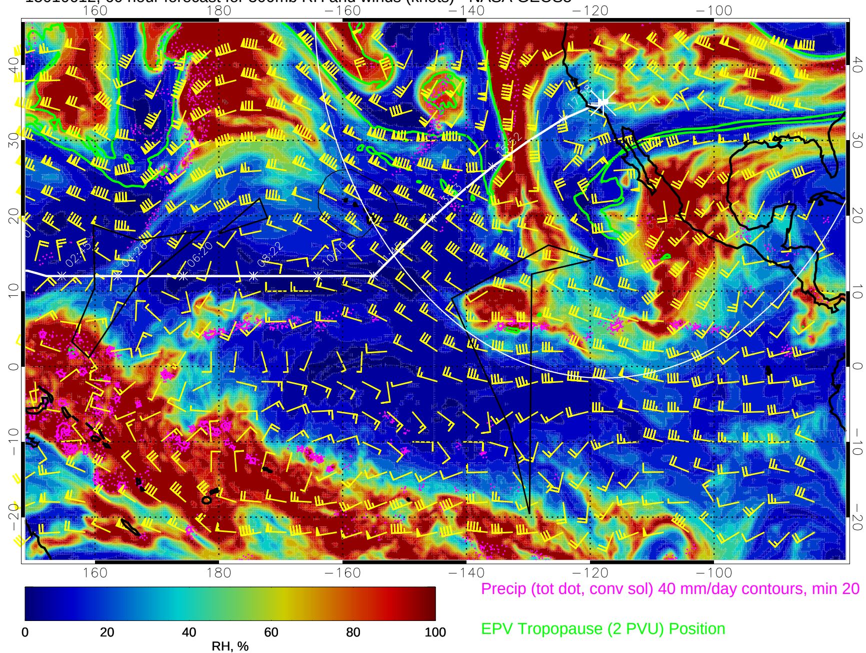
15010612, 60 hour forecast for 300mb RH and winds (knots) - NASA GEOS5
