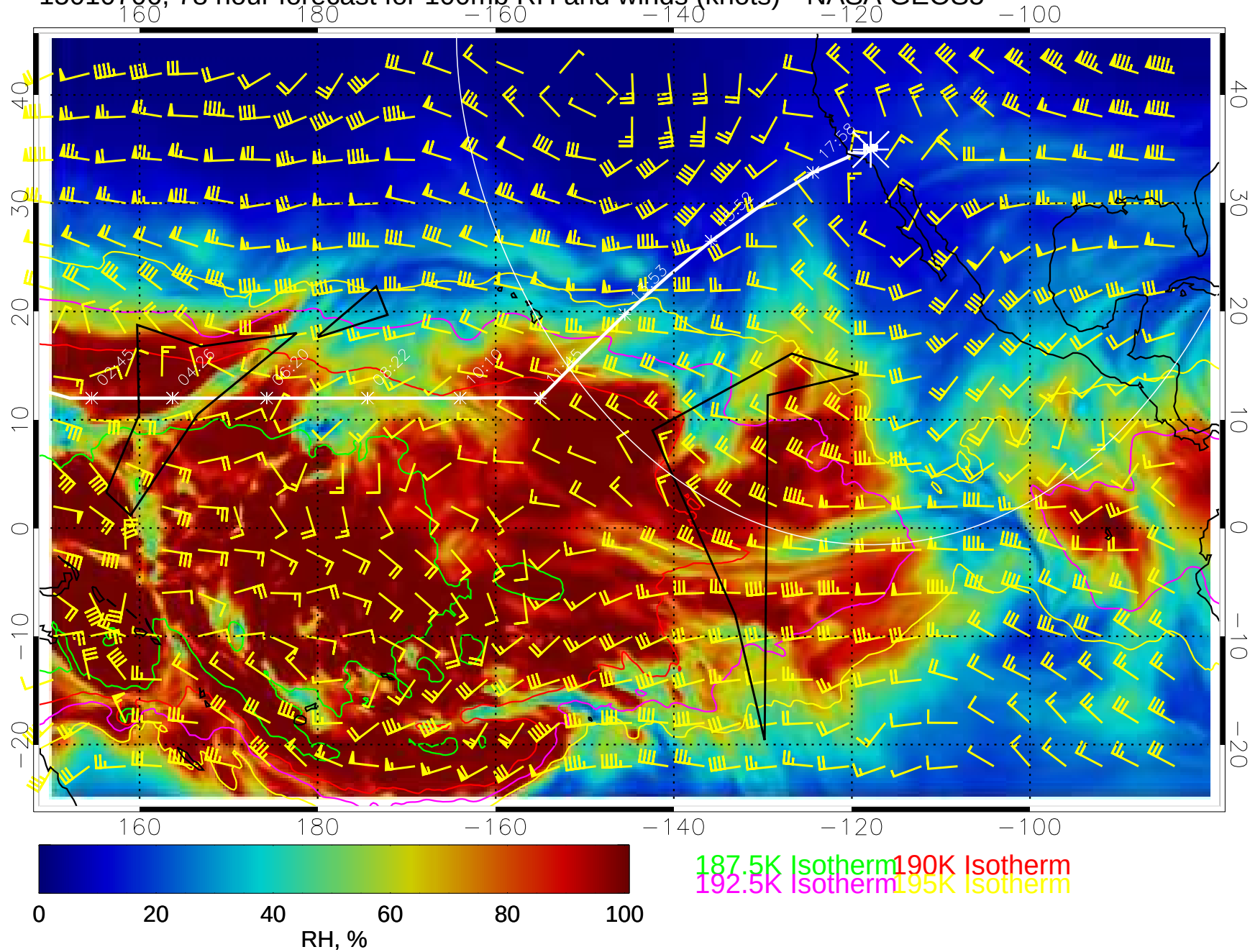
15010706, 78 hour forecast for 100mb RH and winds (knots)-- NASA GEOS5
