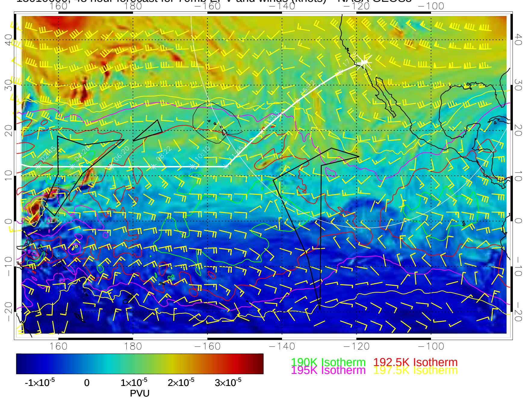
15010600, 48 hour forecast for 70mb EPV and winds (knots)-- NASA GEOS5
