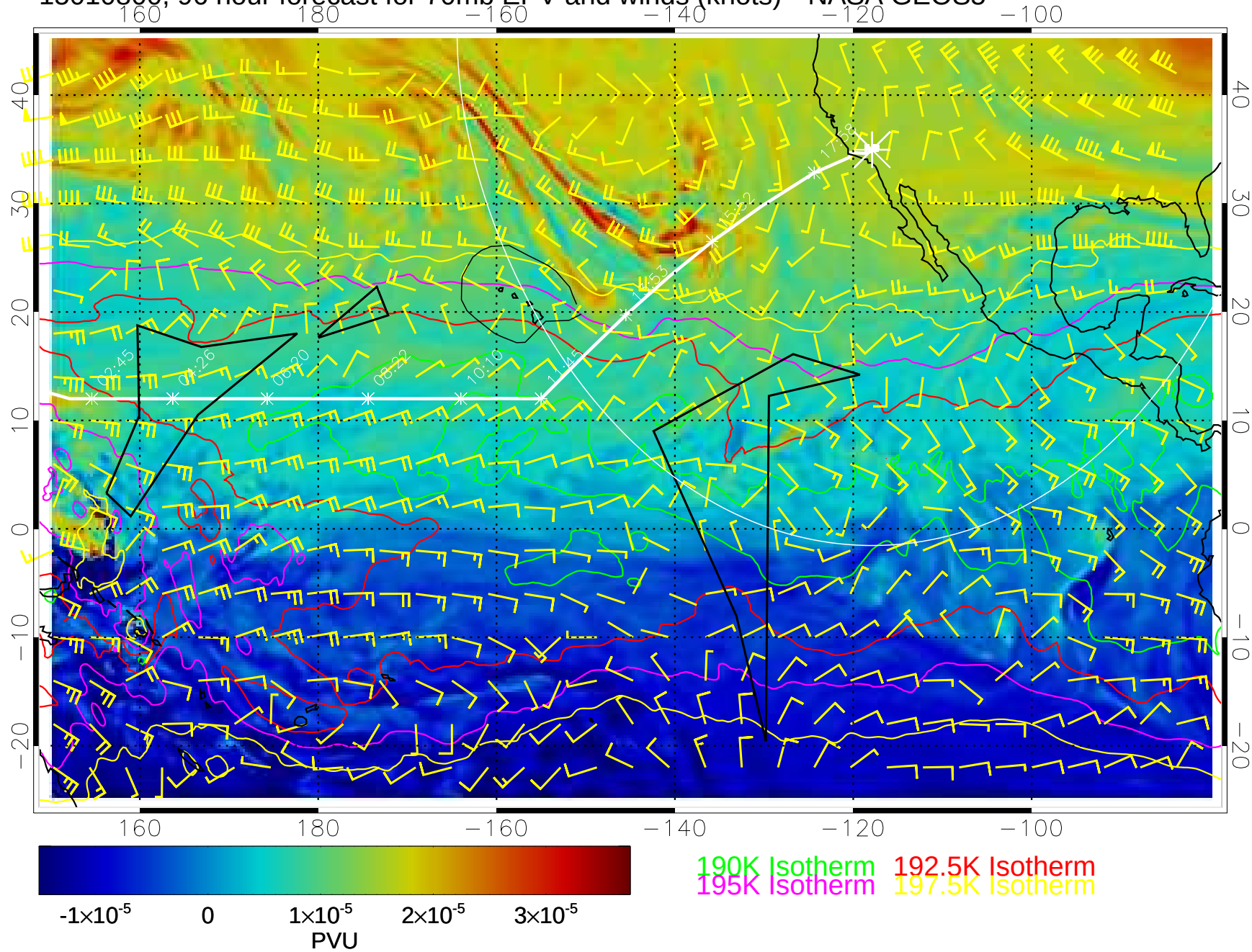
15010800, 96 hour forecast for 70mb EPV and winds (knots)-- NASA GEOS5
