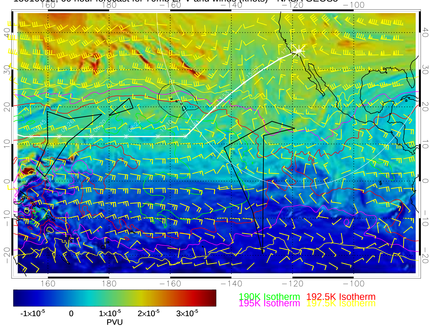
15010612, 60 hour forecast for 70mb EPV and winds (knots)-- NASA GEOS5
