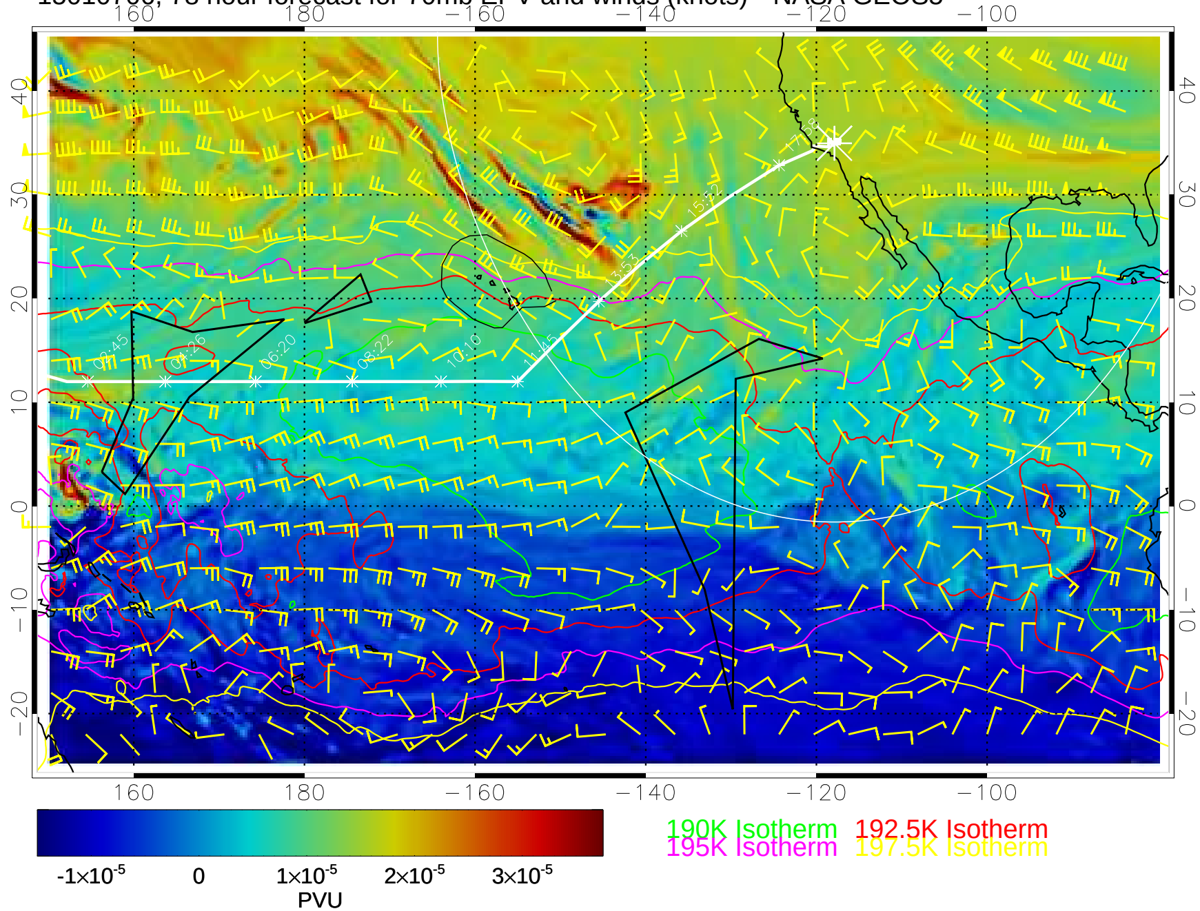
15010706, 78 hour forecast for 70mb EPV and winds (knots)-- NASA GEOS5
