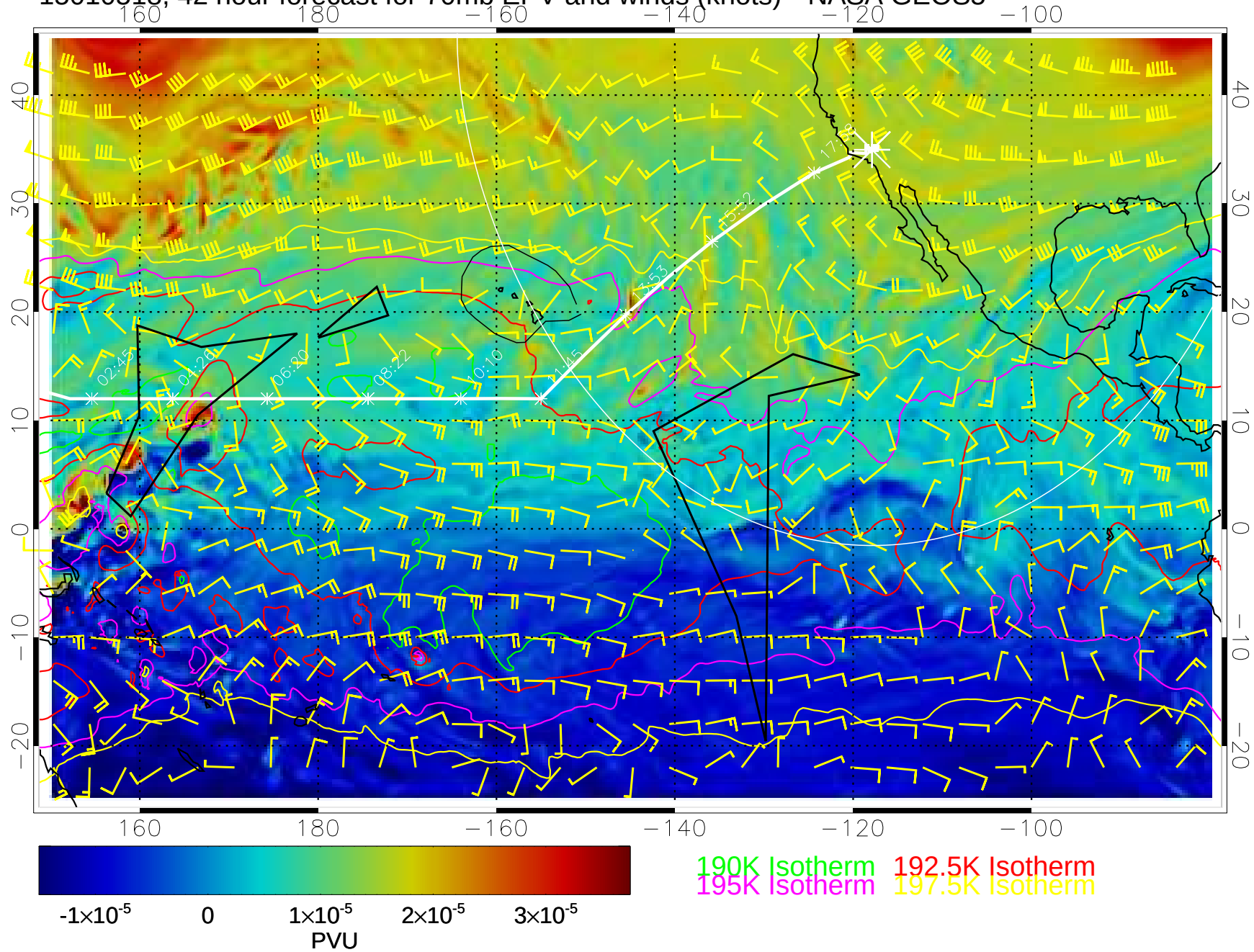
15010518, 42 hour forecast for 70mb EPV and winds (knots)-- NASA GEOS5
