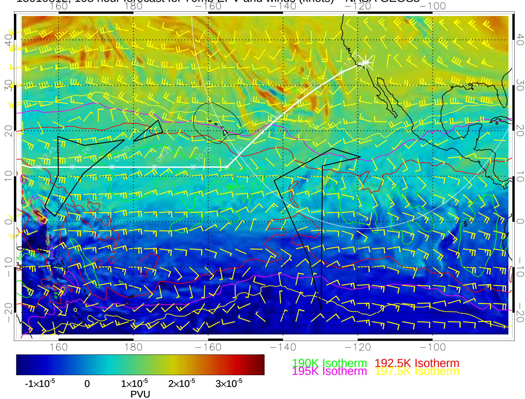
15010812, 108 hour forecast for 70mb EPV and winds (knots)-- NASA GEOS5
