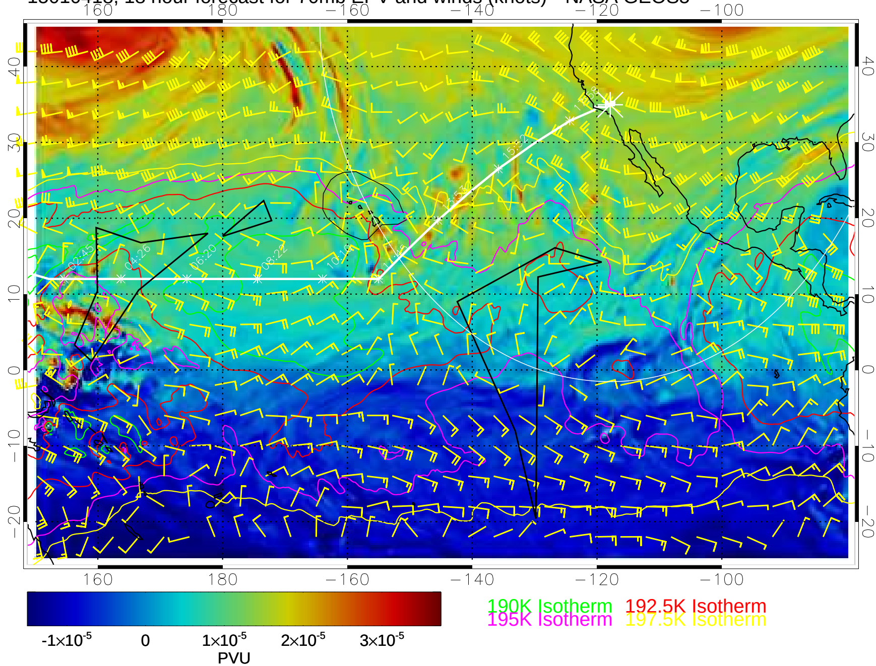
15010418, 18 hour forecast for 70mb EPV and winds (knots)-- NASA GEOS5
