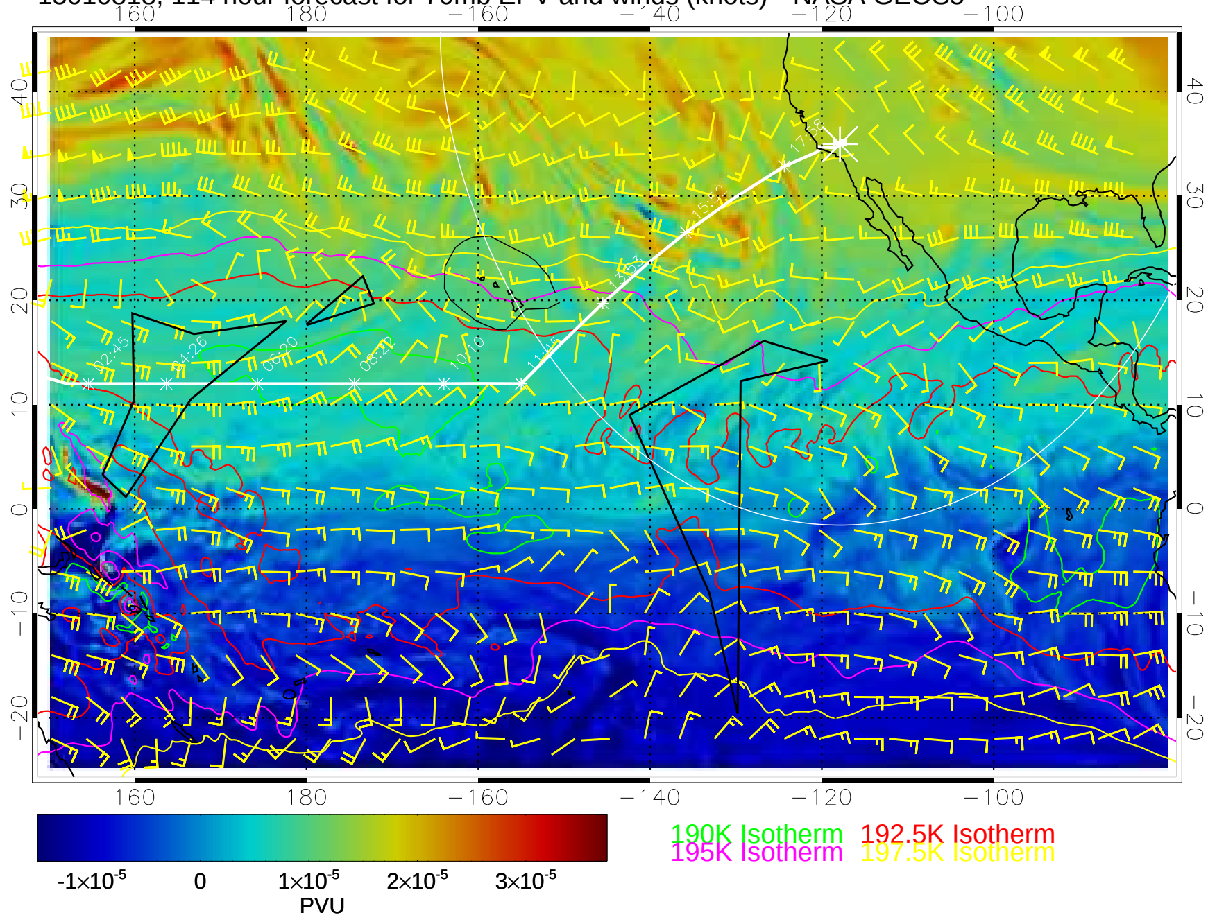
15010818, 114 hour forecast for 70mb EPV and winds (knots)-- NASA GEOS5
