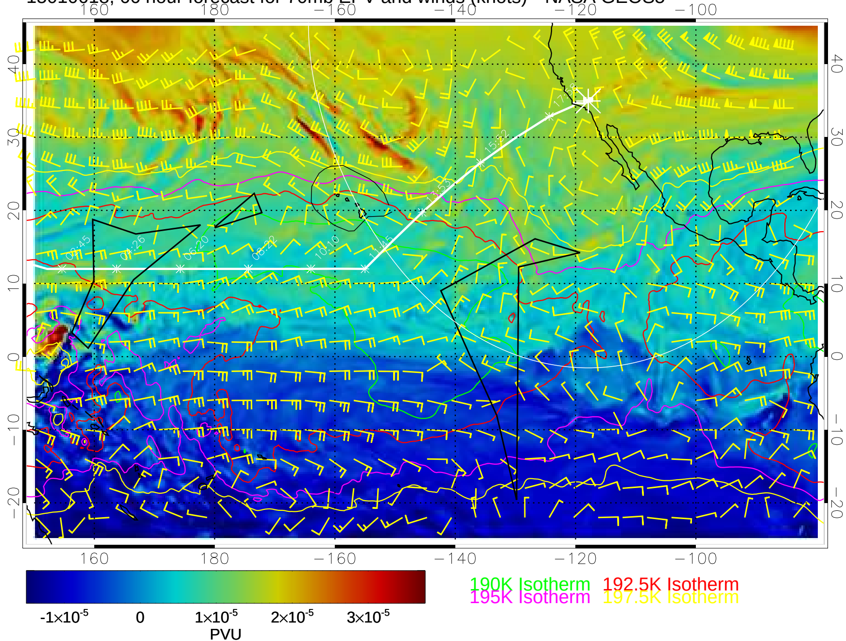
15010618, 66 hour forecast for 70mb EPV and winds (knots)-- NASA GEOS5
