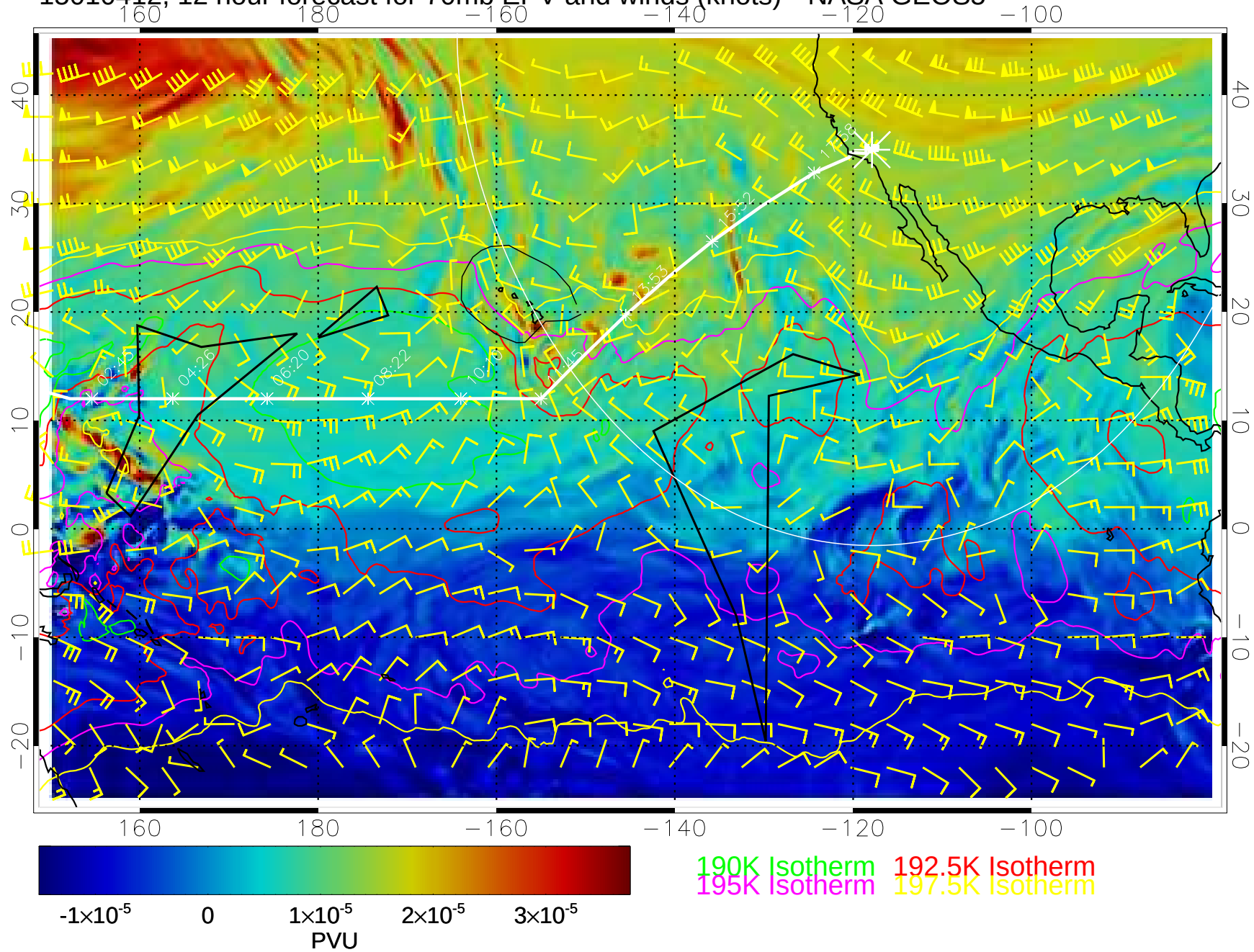
15010412, 12 hour forecast for 70mb EPV and winds (knots)-- NASA GEOS5
