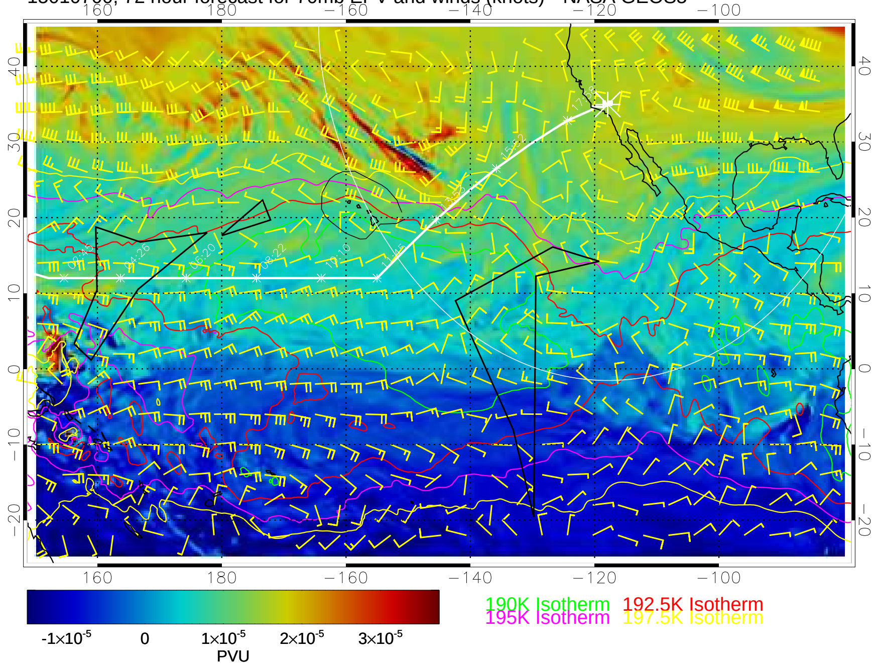
15010700, 72 hour forecast for 70mb EPV and winds (knots)-- NASA GEOS5
