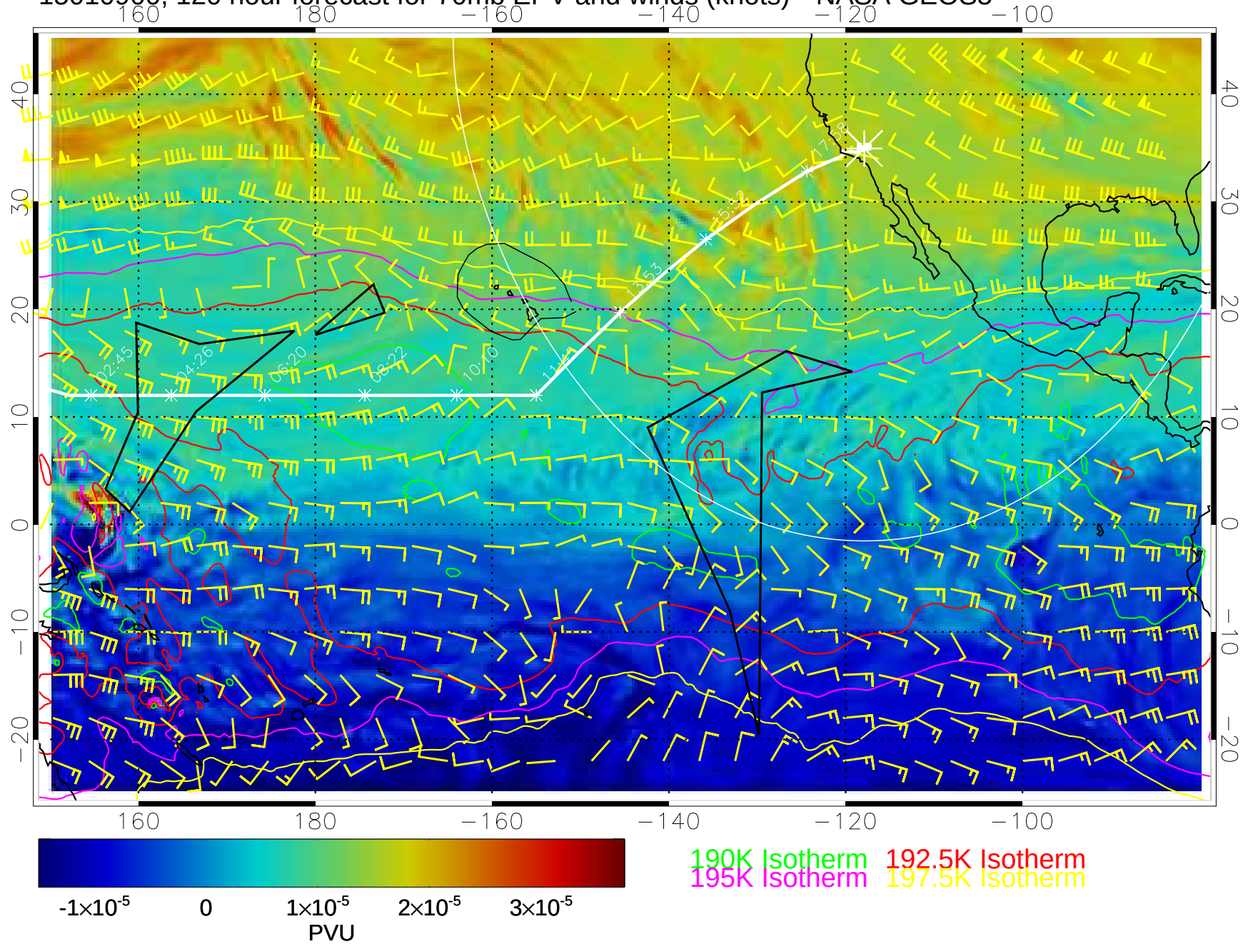
15010900, 120 hour forecast for 70mb EPV and winds (knots)-- NASA GEOS5
