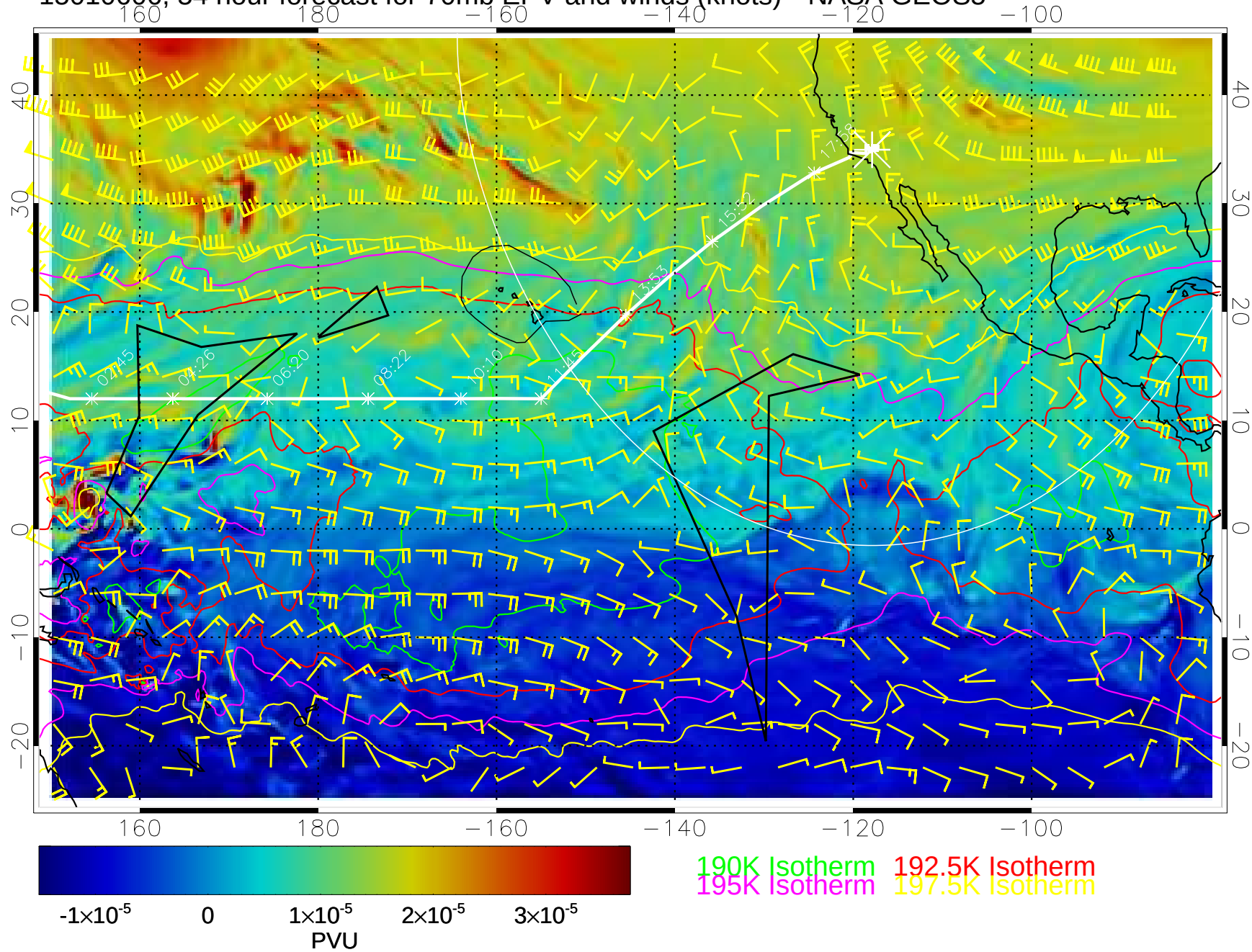
15010606, 54 hour forecast for 70mb EPV and winds (knots)-- NASA GEOS5
