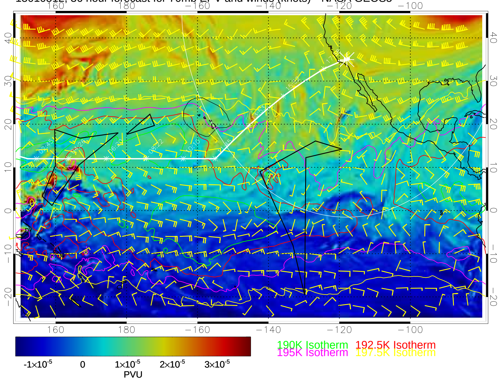
15010512, 36 hour forecast for 70mb EPV and winds (knots)-- NASA GEOS5
