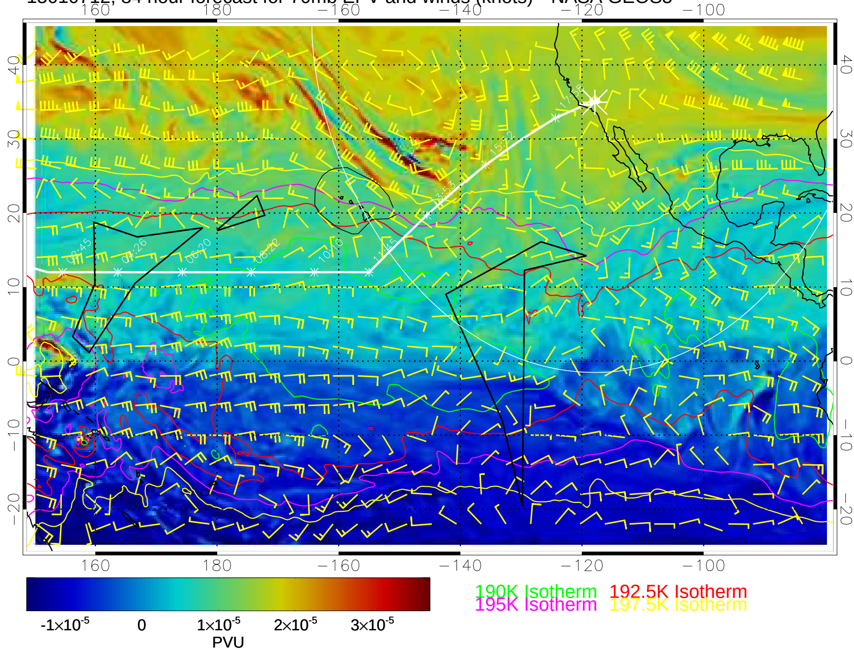
15010712, 84 hour forecast for 70mb EPV and winds (knots)-- NASA GEOS5
