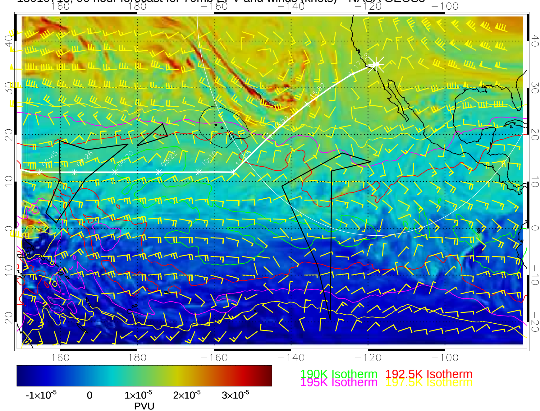
15010718, 90 hour forecast for 70mb EPV and winds (knots)-- NASA GEOS5
