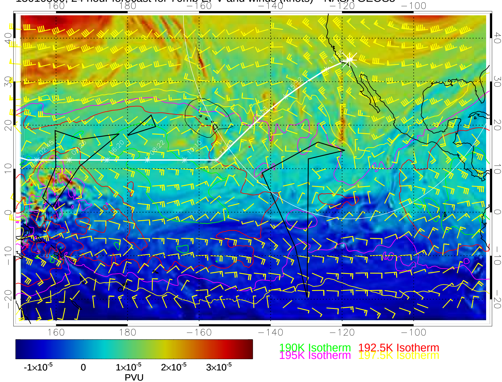
15010500, 24 hour forecast for 70mb EPV and winds (knots)-- NASA GEOS5
