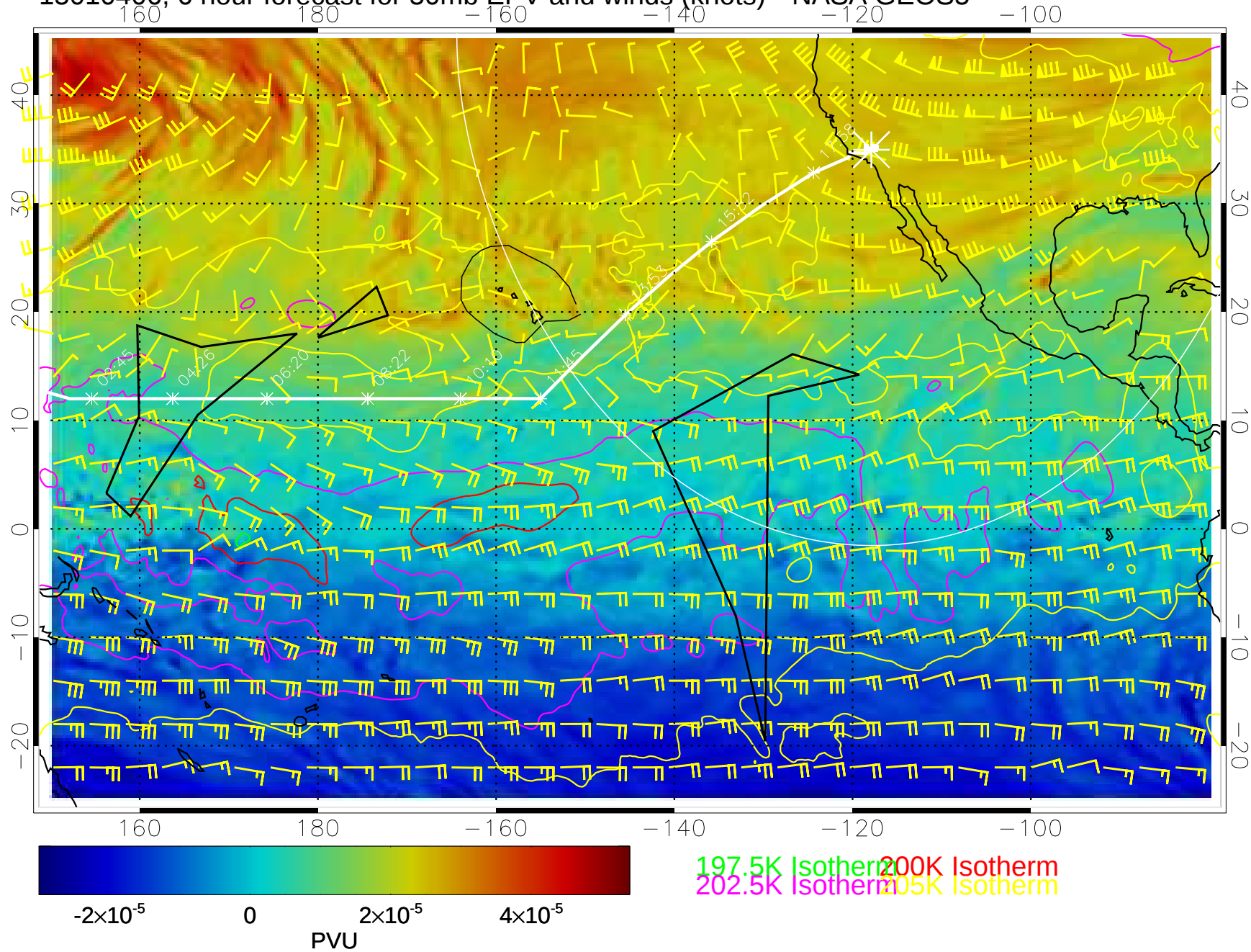
15010406, 6 hour forecast for 50mb EPV and winds (knots)-- NASA GEOS5
