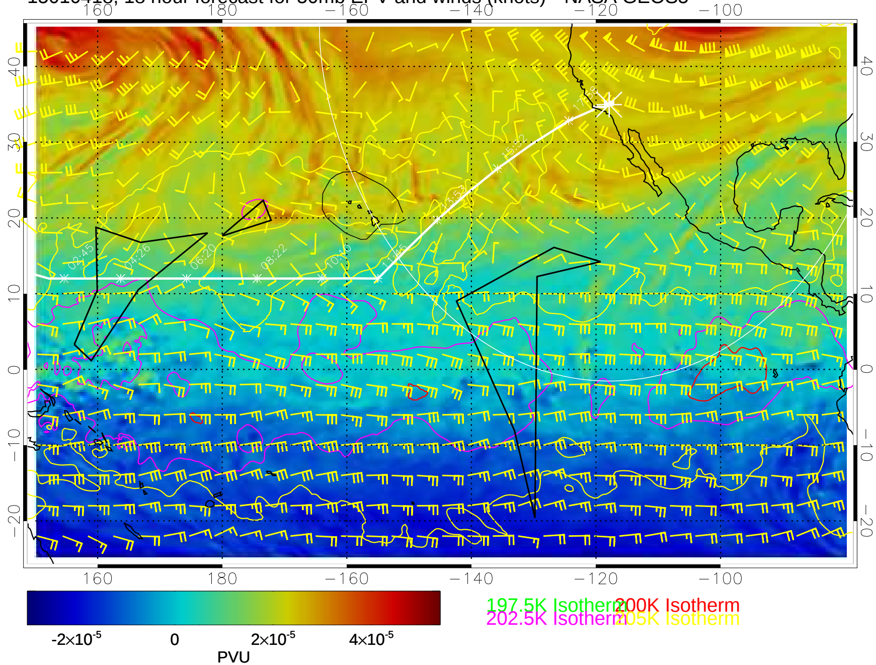
15010418, 18 hour forecast for 50mb EPV and winds (knots)-- NASA GEOS5
