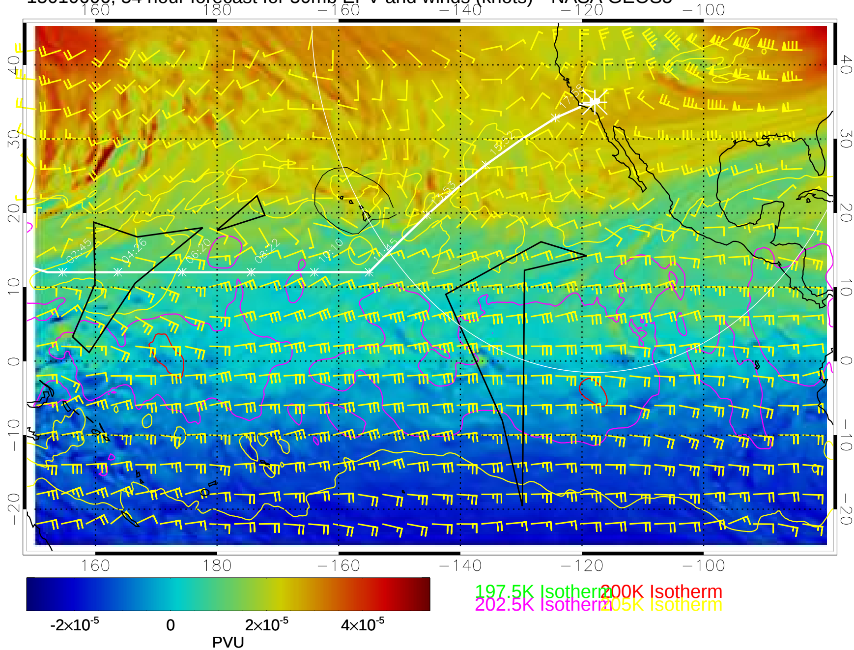
15010606, 54 hour forecast for 50mb EPV and winds (knots)-- NASA GEOS5
