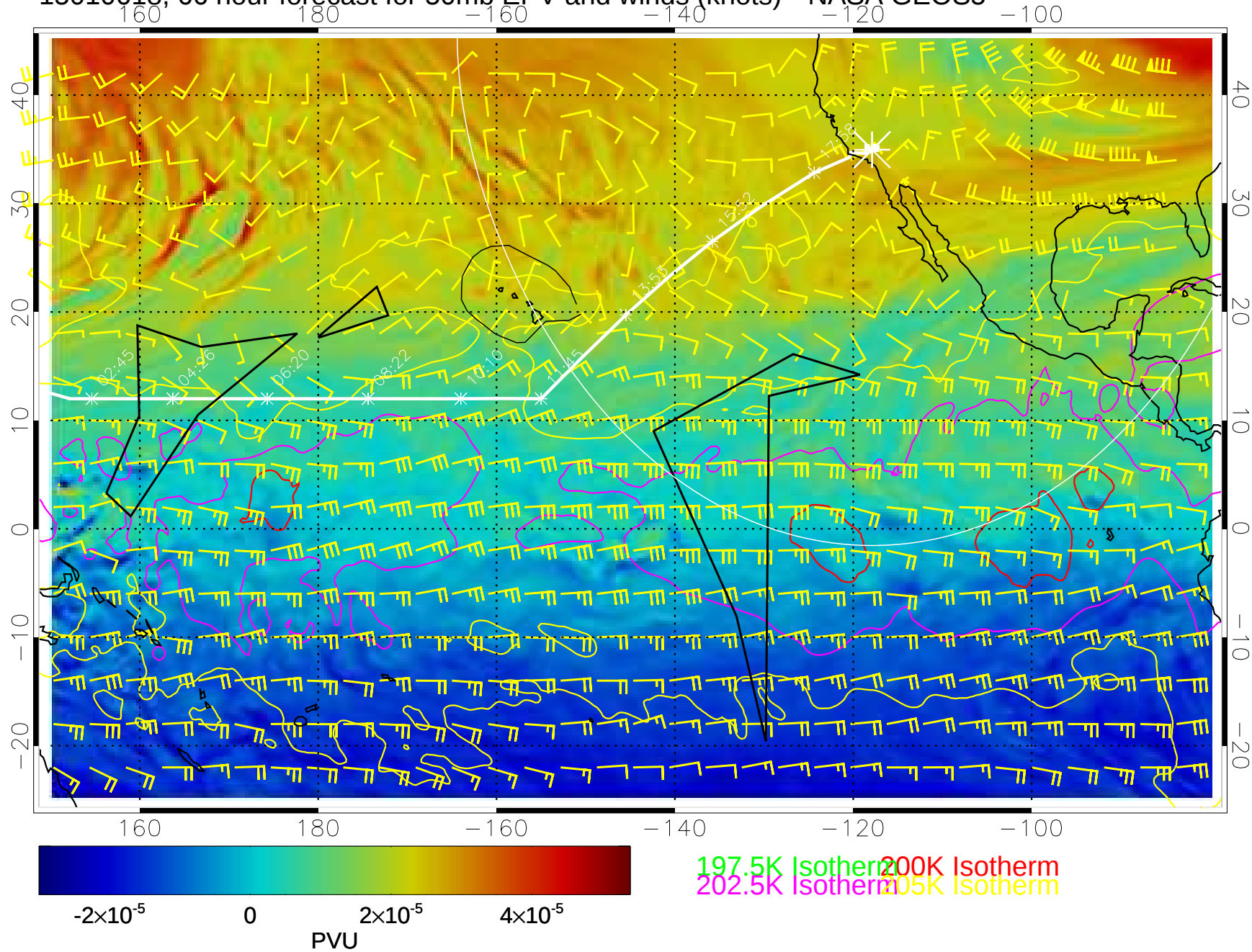
15010618, 66 hour forecast for 50mb EPV and winds (knots)-- NASA GEOS5
