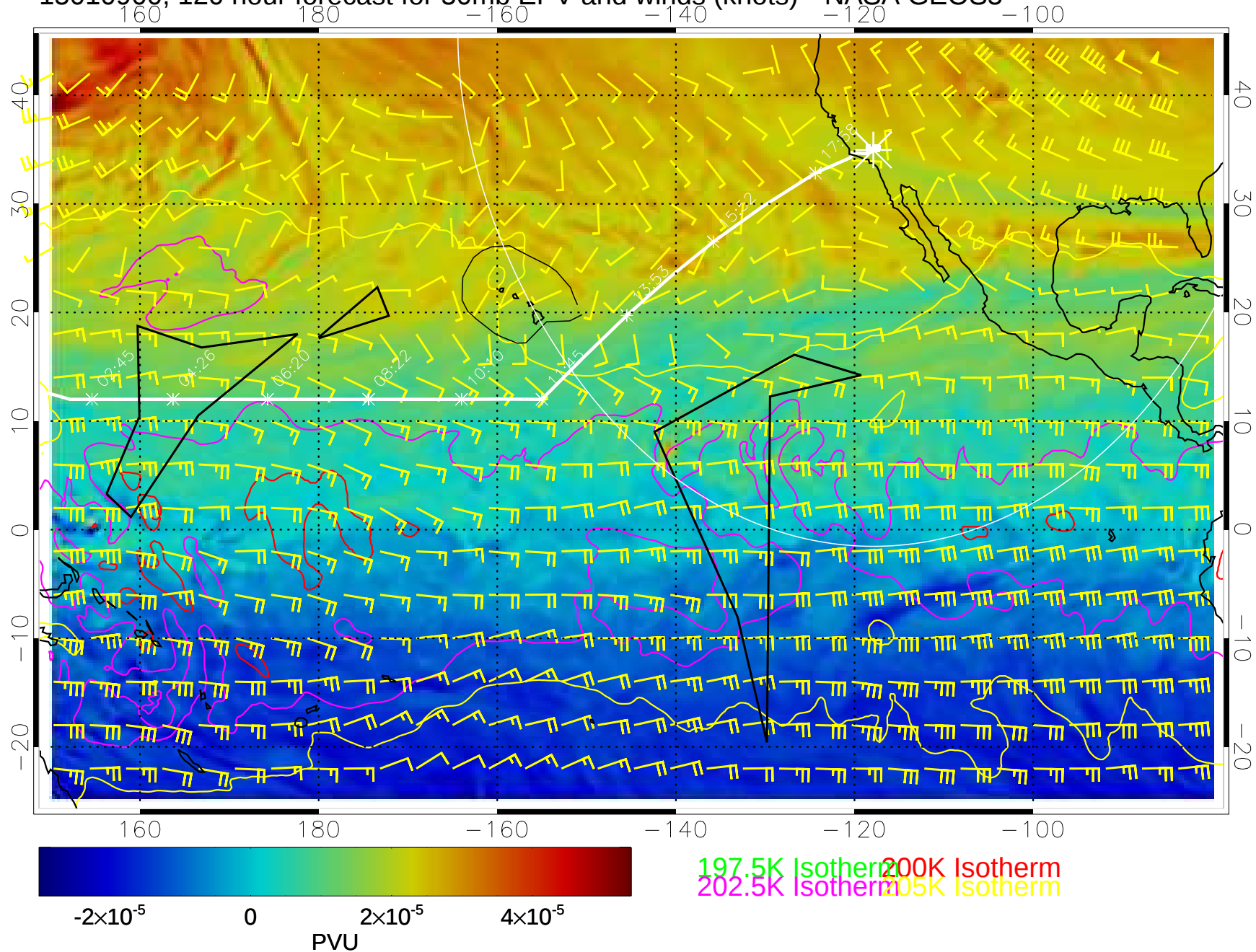
15010900, 120 hour forecast for 50mb EPV and winds (knots)-- NASA GEOS5
