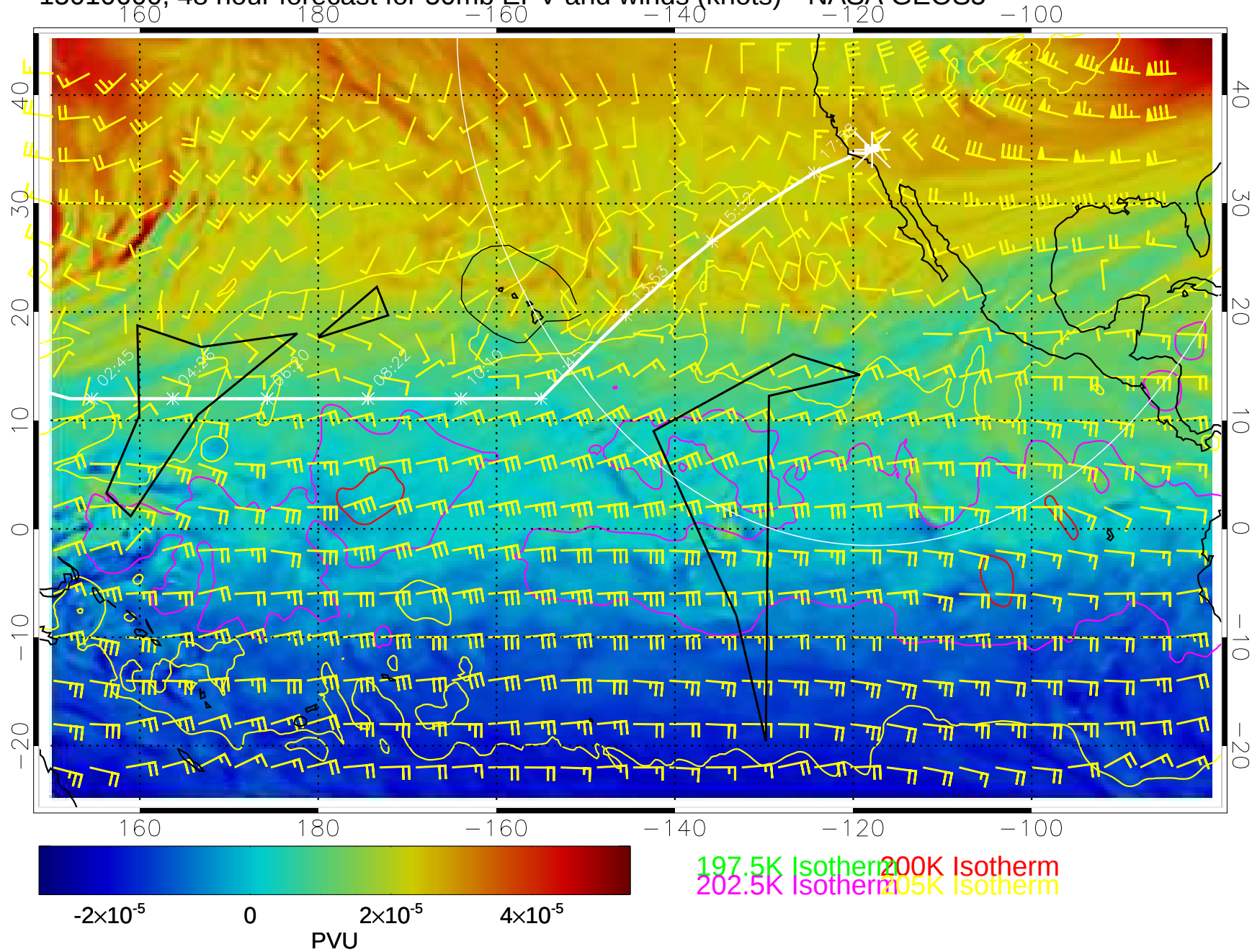
15010600, 48 hour forecast for 50mb EPV and winds (knots)-- NASA GEOS5
