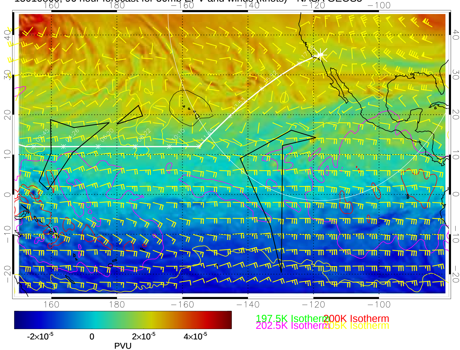
15010800, 96 hour forecast for 50mb EPV and winds (knots)-- NASA GEOS5
