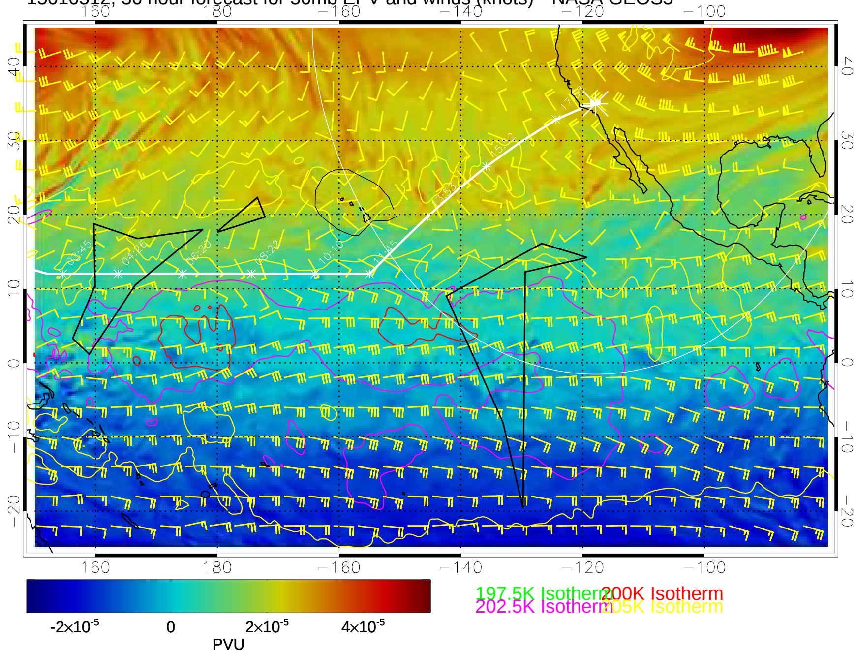
15010512, 36 hour forecast for 50mb EPV and winds (knots)-- NASA GEOS5
