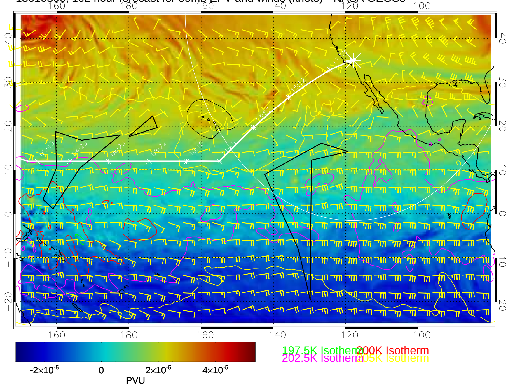
15010806, 102 hour forecast for 50mb EPV and winds (knots)-- NASA GEOS5
