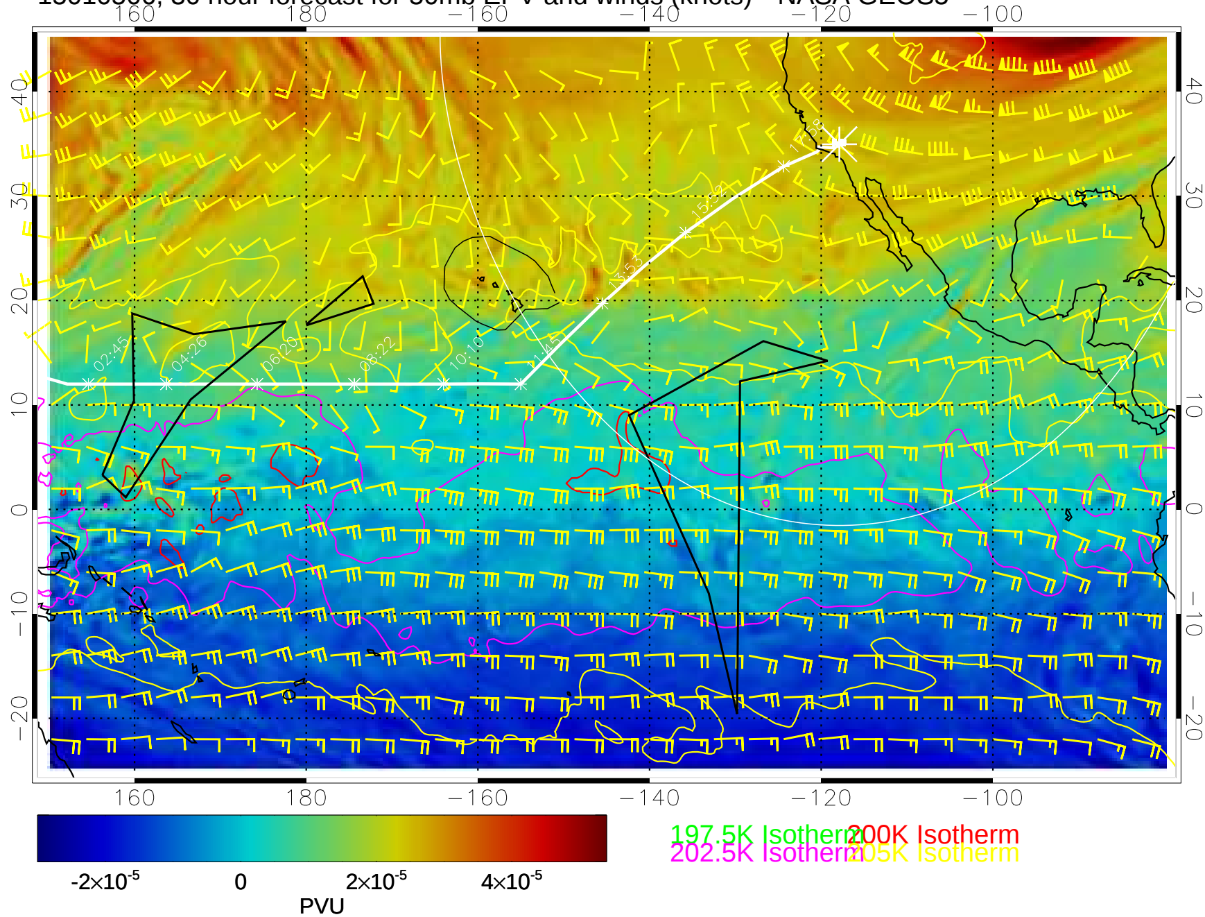
15010506, 30 hour forecast for 50mb EPV and winds (knots)-- NASA GEOS5
