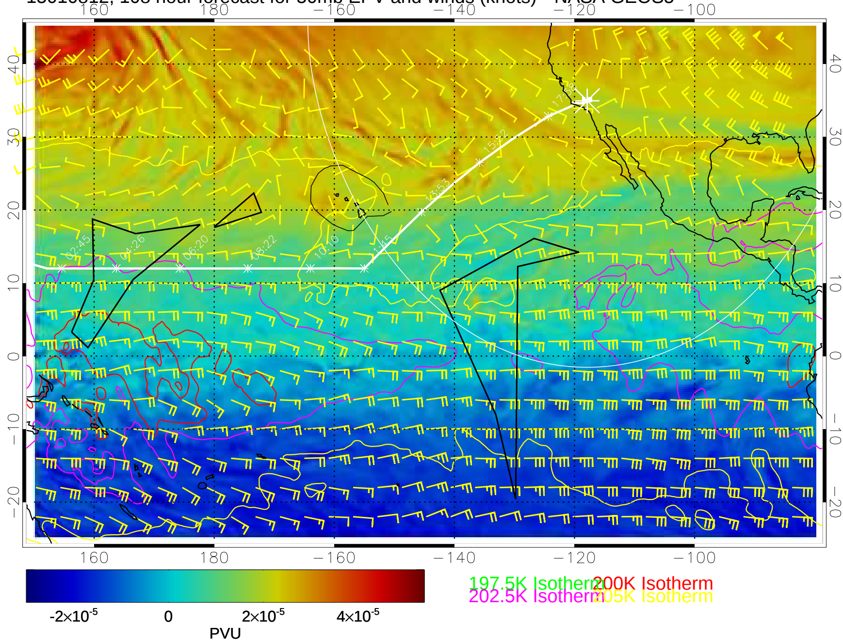
15010812, 108 hour forecast for 50mb EPV and winds (knots)-- NASA GEOS5
