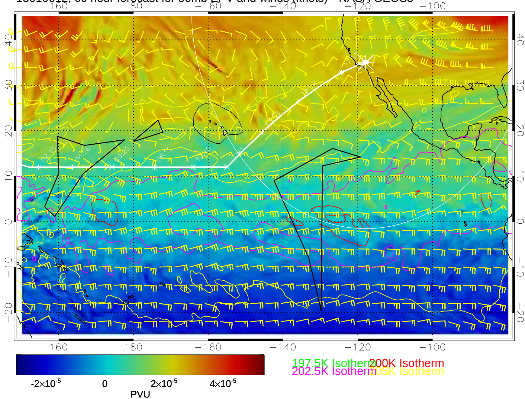
15010612, 60 hour forecast for 50mb EPV and winds (knots)-- NASA GEOS5
