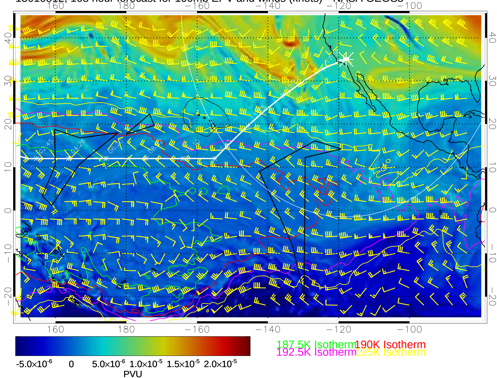
15010812, 108 hour forecast for 100mb EPV and winds (knots)-- NASA GEOS5
