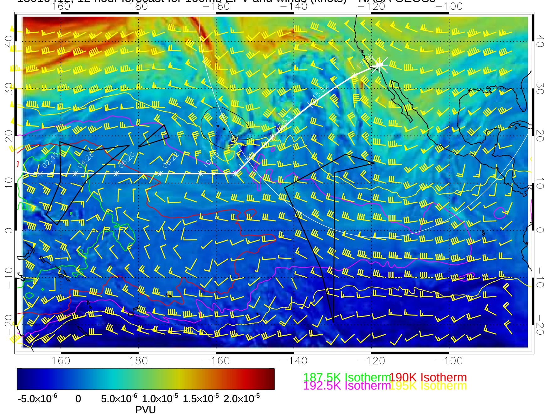
15010412, 12 hour forecast for 100mb EPV and winds (knots)-- NASA GEOS5
