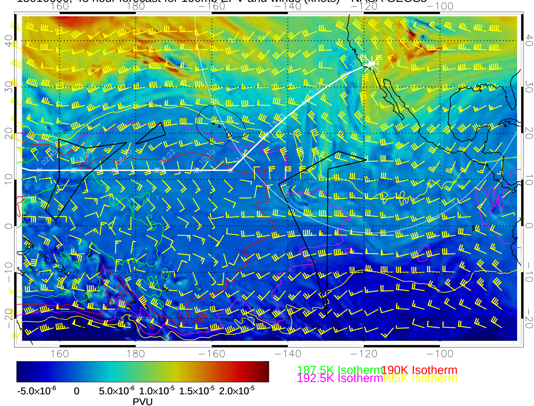
15010600, 48 hour forecast for 100mb EPV and winds (knots)-- NASA GEOS5
