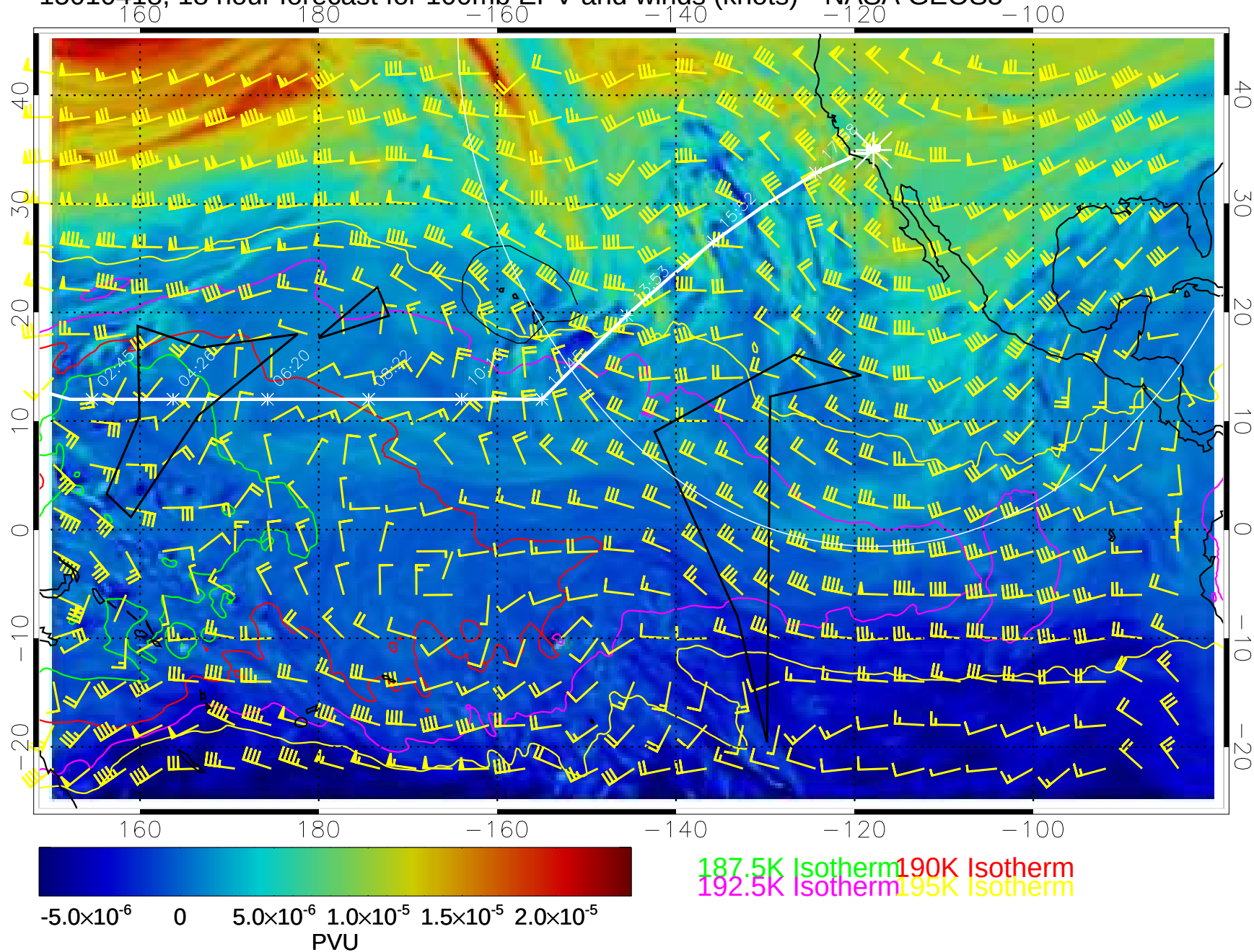
15010418, 18 hour forecast for 100mb EPV and winds (knots)-- NASA GEOS5
