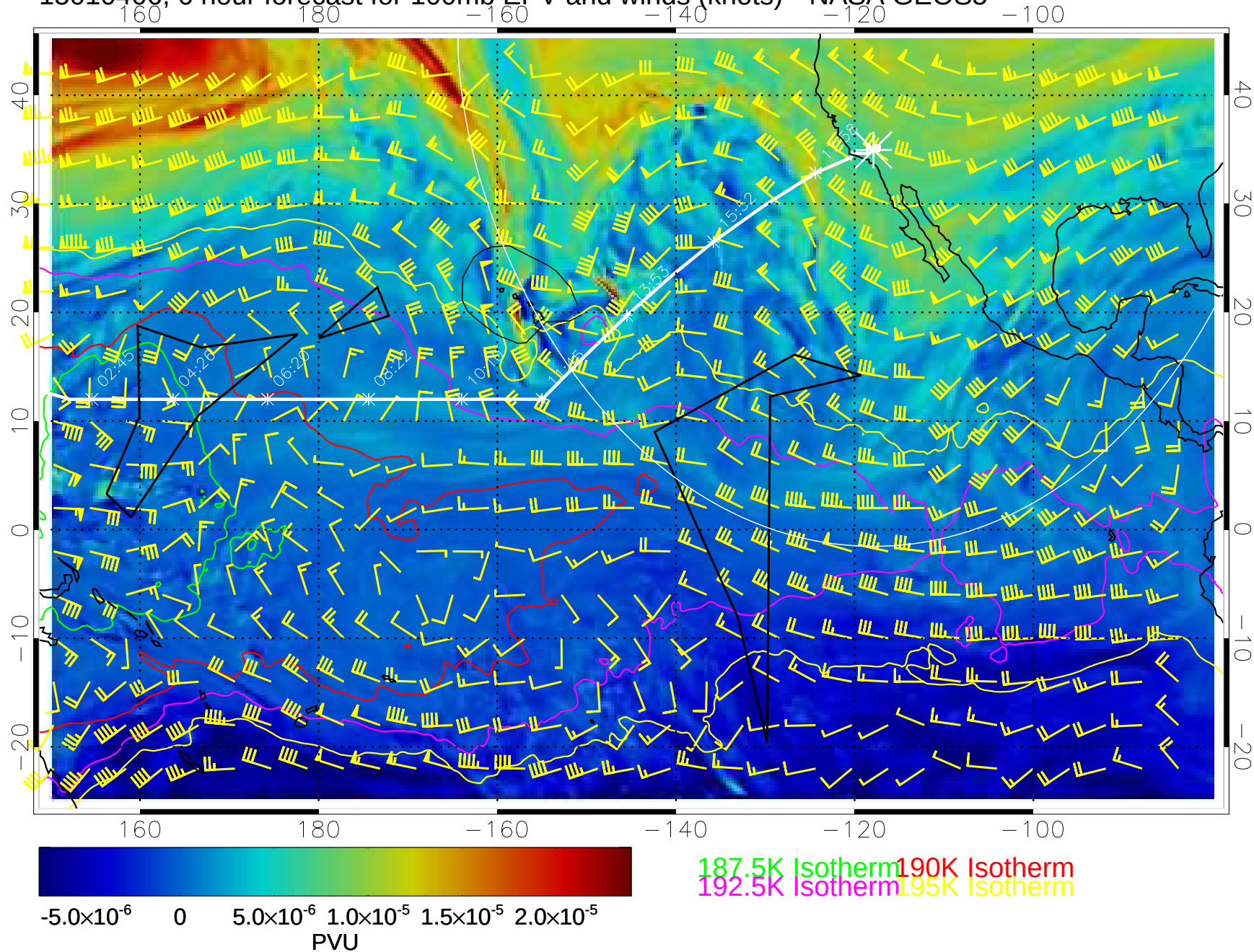
15010406, 6 hour forecast for 100mb EPV and winds (knots)-- NASA GEOS5
