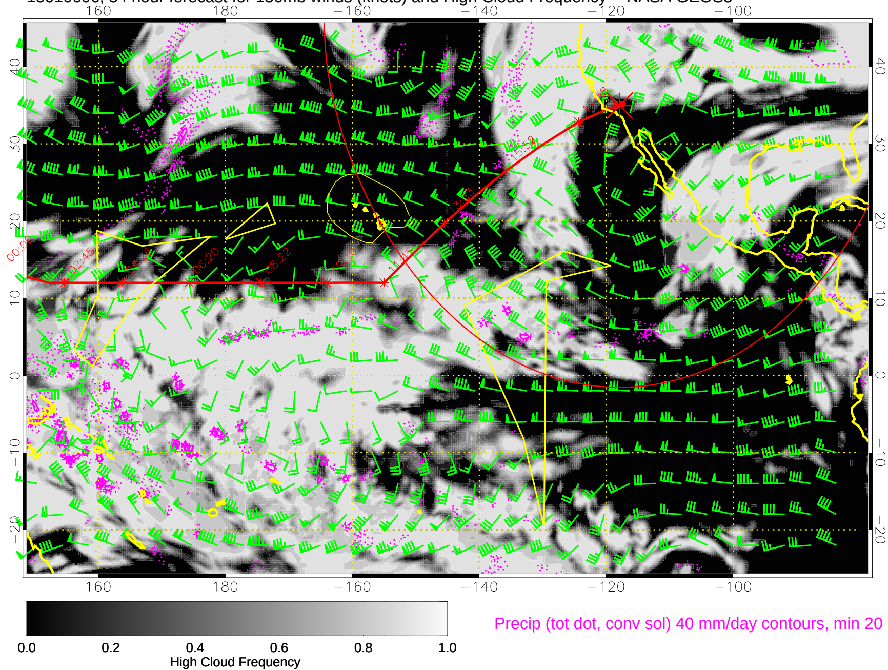
15010606, 54 hour forecast for 150mb winds (knots) and High Cloud Frequency -- NASA GEOS5
