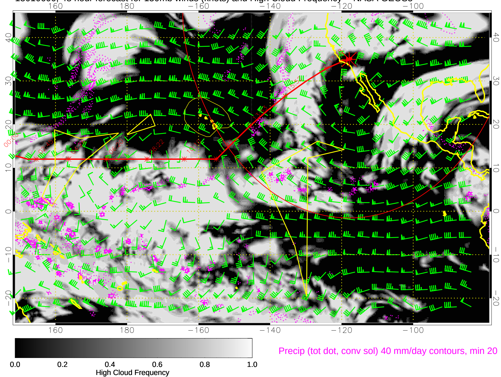
15010600, 48 hour forecast for 150mb winds (knots) and High Cloud Frequency -- NASA GEOS5
