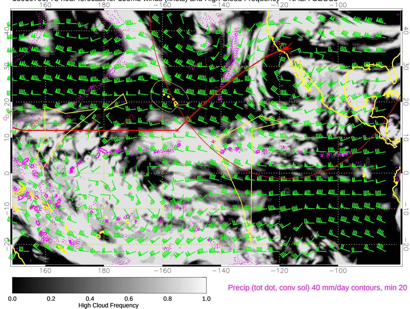
15010706, 78 hour forecast for 150mb winds (knots) and High Cloud Frequency -- NASA GEOS5
