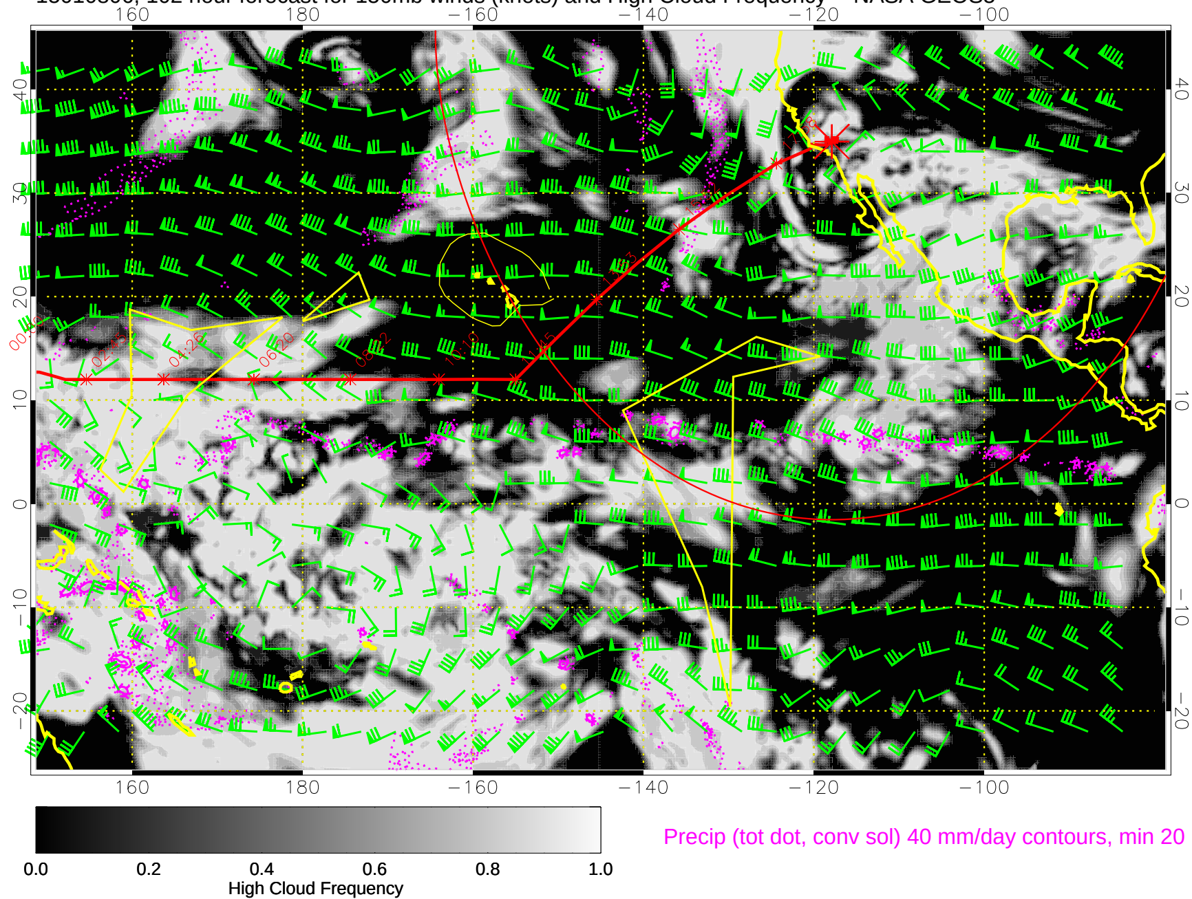
15010806, 102 hour forecast for 150mb winds (knots) and High Cloud Frequency -- NASA GEOS5
