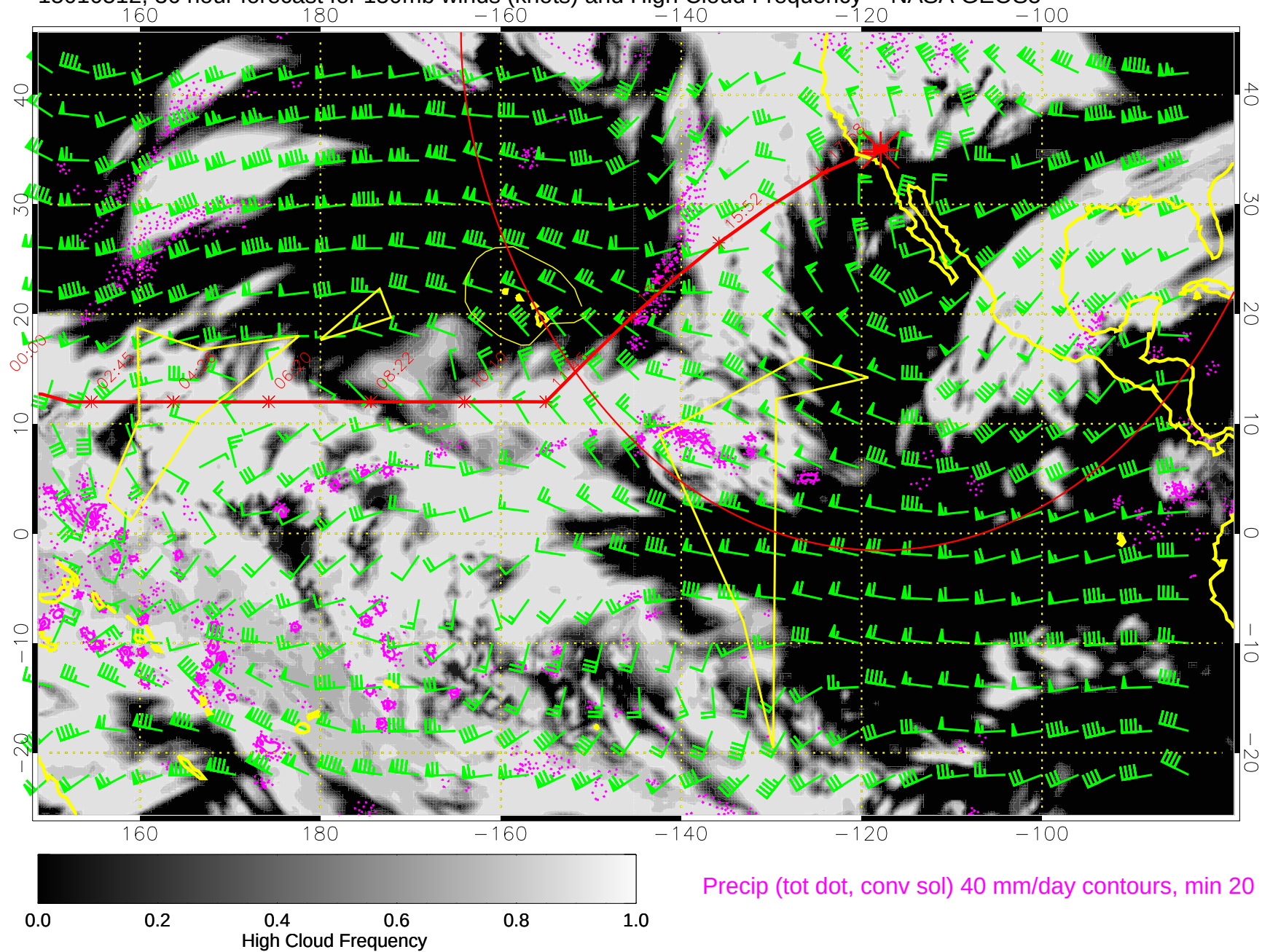
15010512, 36 hour forecast for 150mb winds (knots) and High Cloud Frequency -- NASA GEOS5
