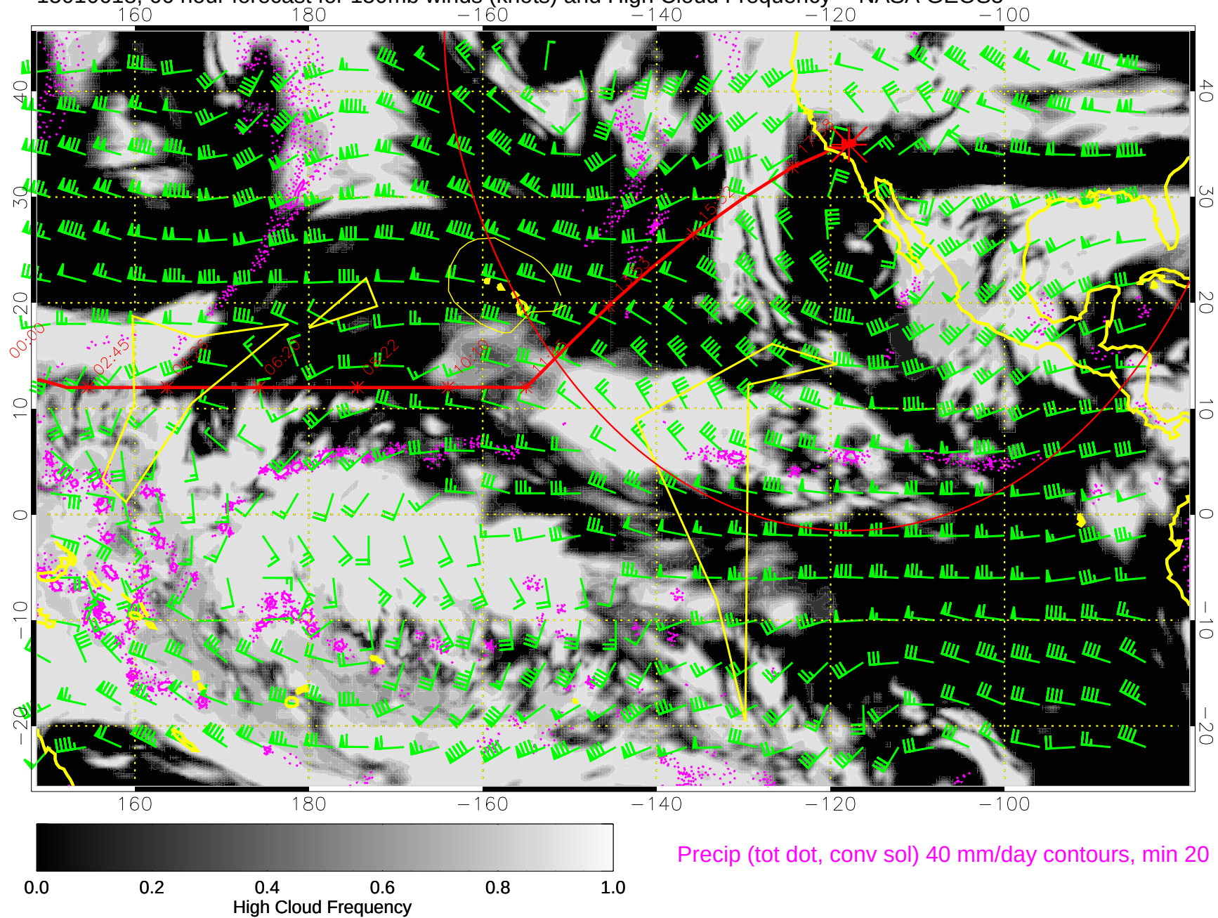
15010618, 66 hour forecast for 150mb winds (knots) and High Cloud Frequency -- NASA GEOS5
