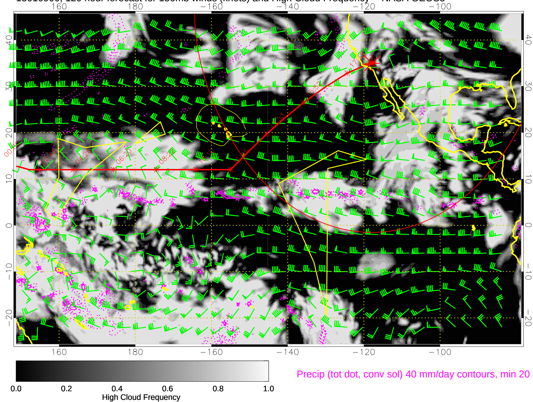
15010900, 120 hour forecast for 150mb winds (knots) and High Cloud Frequency -- NASA GEOS5
