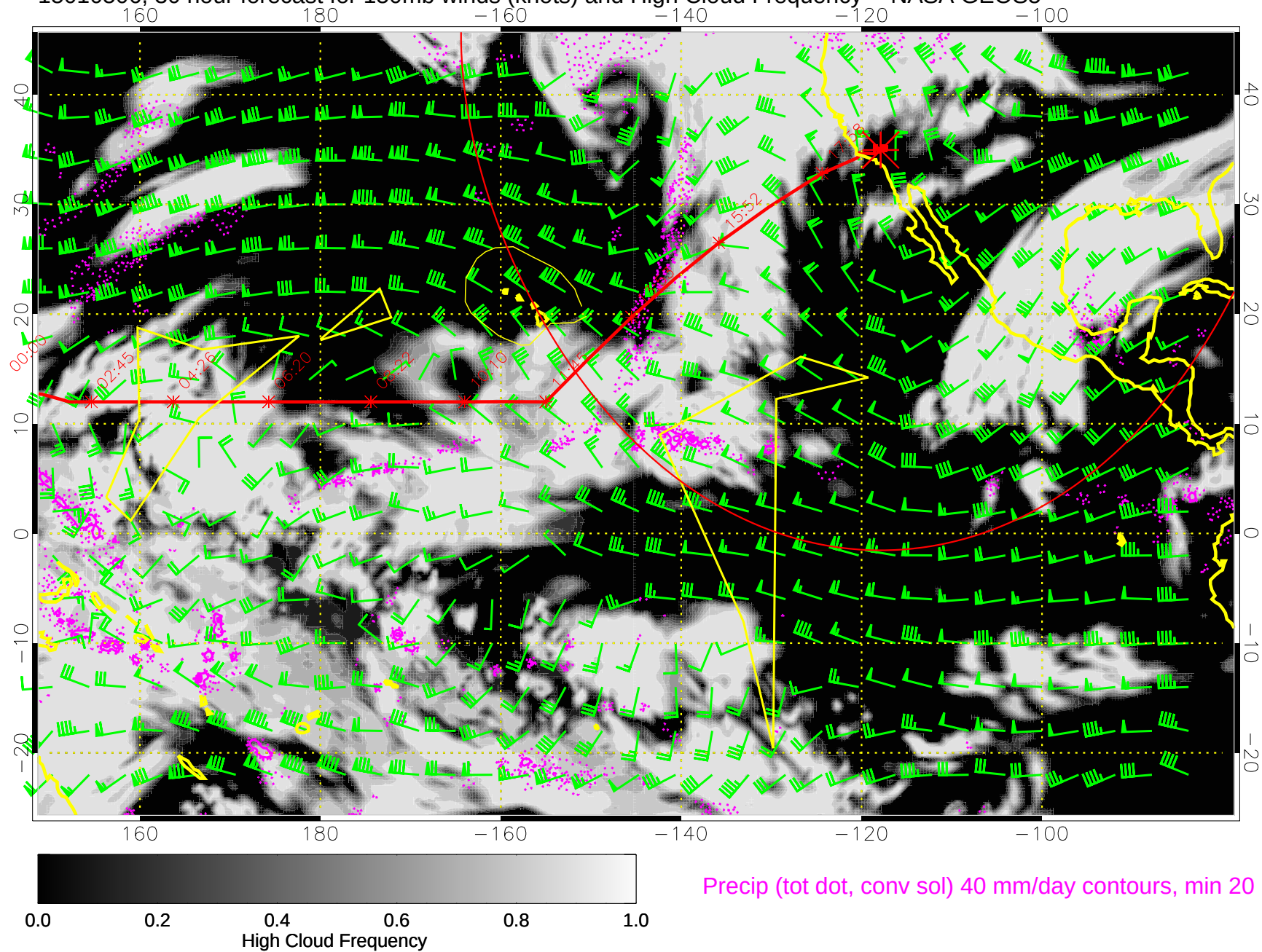
15010506, 30 hour forecast for 150mb winds (knots) and High Cloud Frequency -- NASA GEOS5
