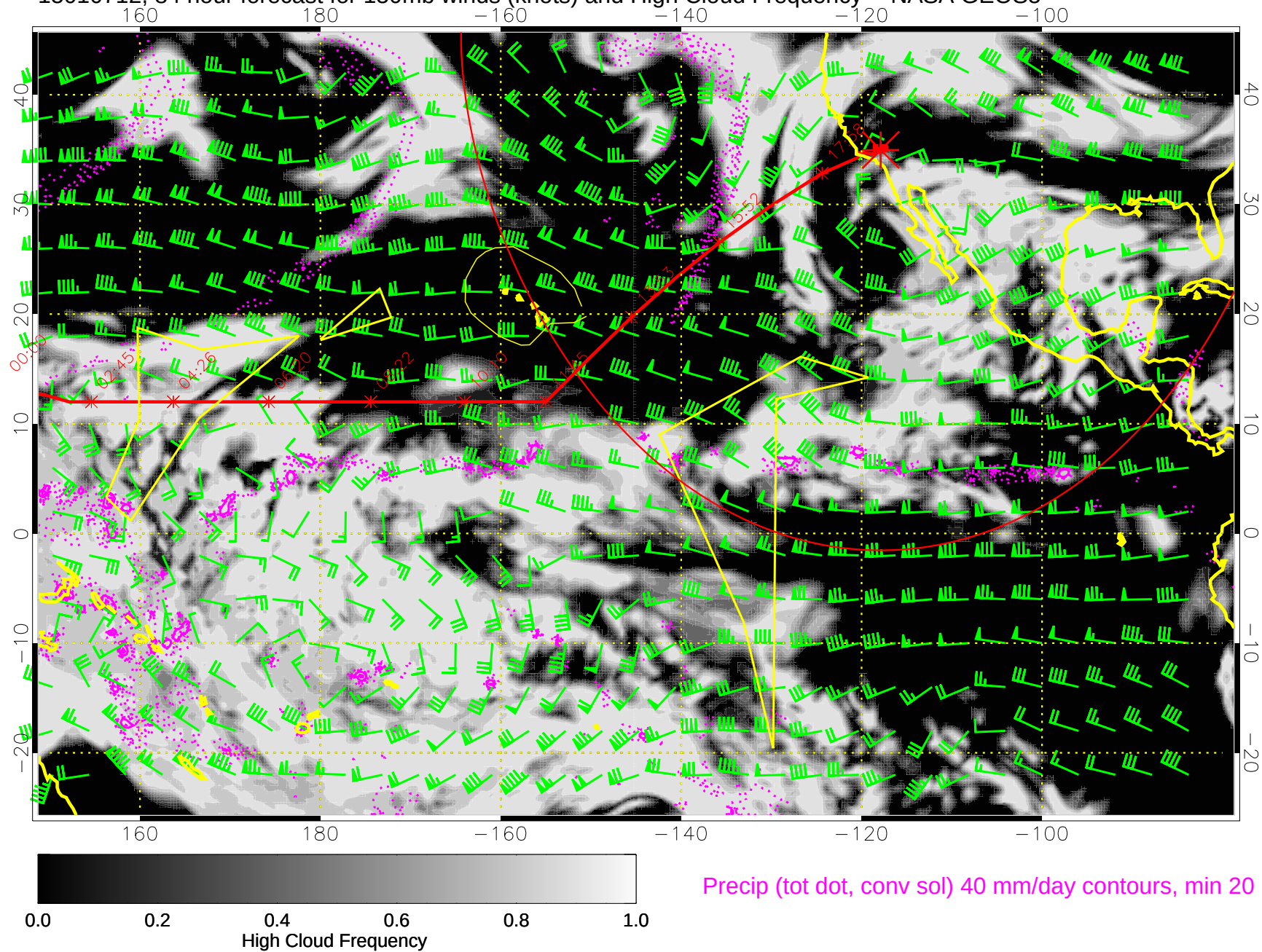
15010712, 84 hour forecast for 150mb winds (knots) and High Cloud Frequency -- NASA GEOS5
