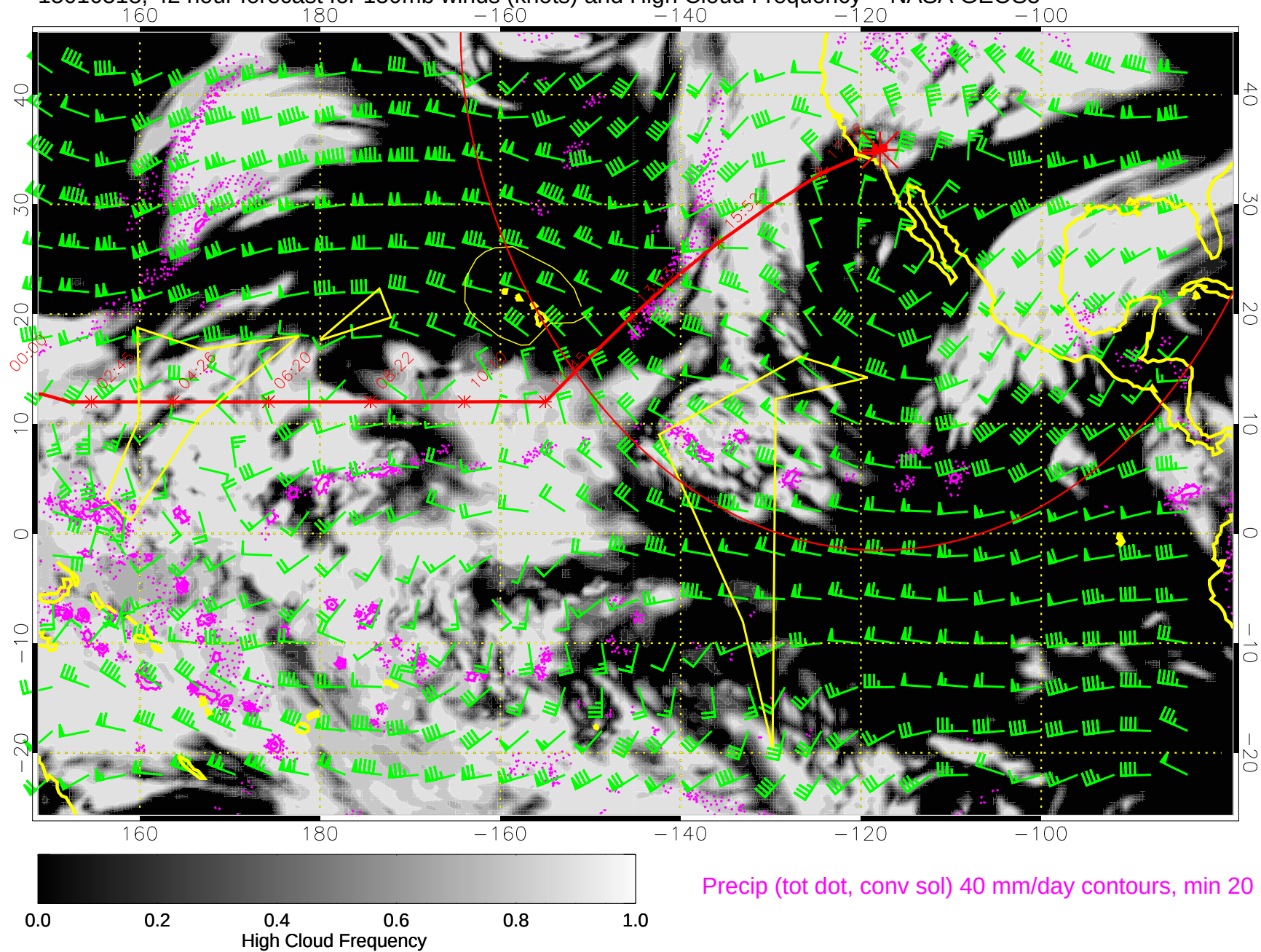
15010518, 42 hour forecast for 150mb winds (knots) and High Cloud Frequency -- NASA GEOS5
