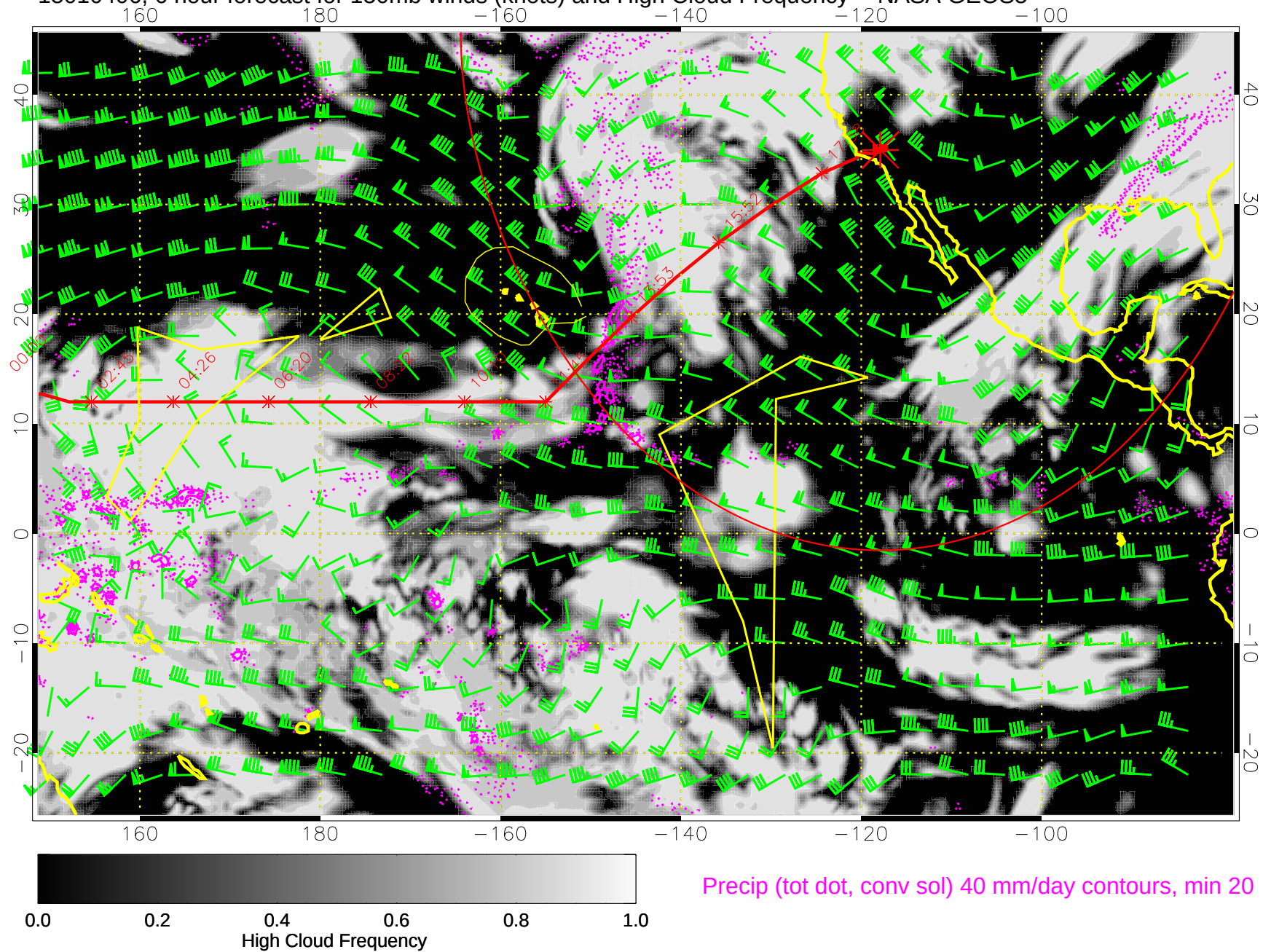
15010406, 6 hour forecast for 150mb winds (knots) and High Cloud Frequency -- NASA GEOS5
