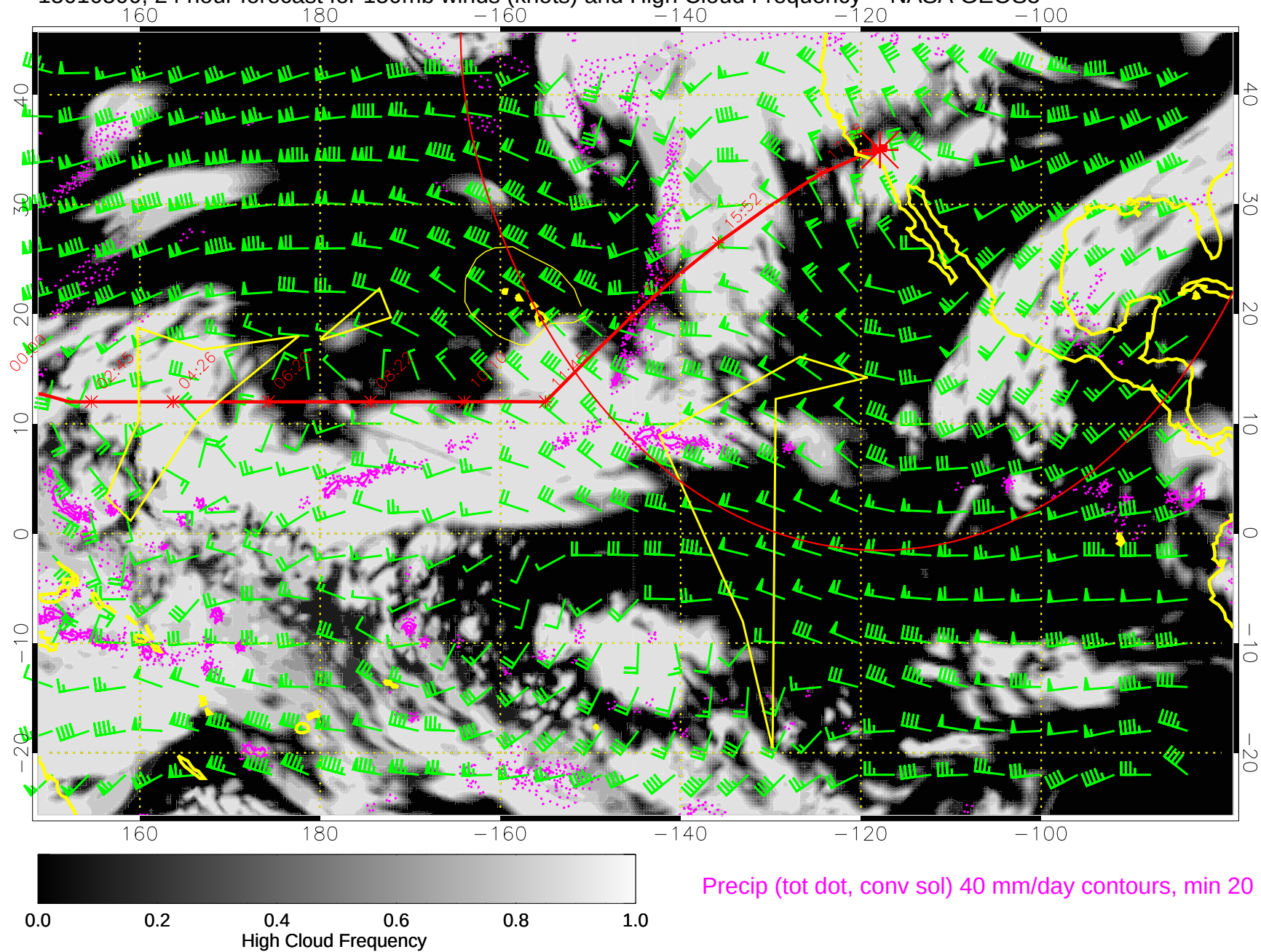
15010500, 24 hour forecast for 150mb winds (knots) and High Cloud Frequency -- NASA GEOS5
