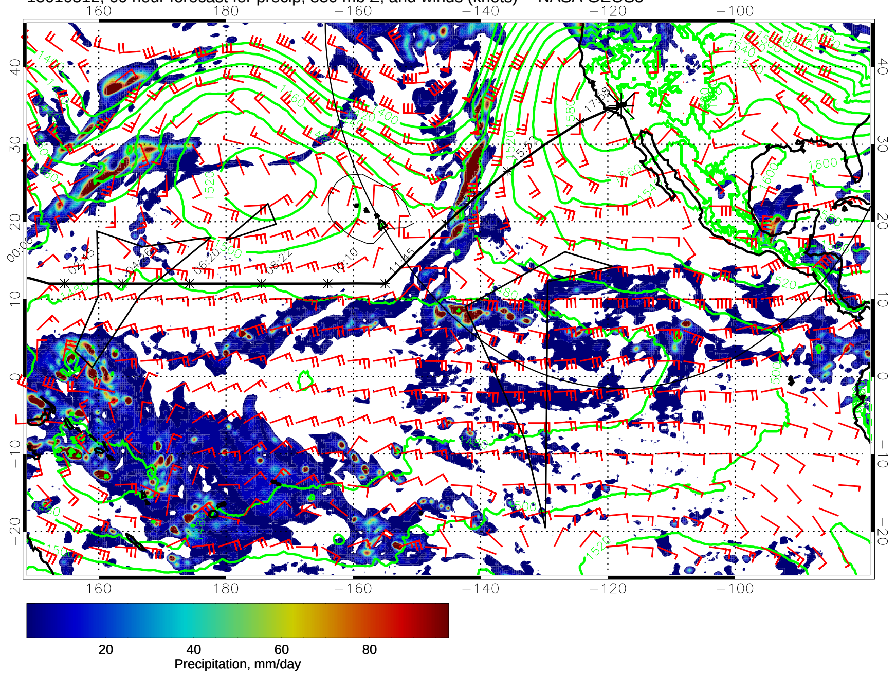
15010512, 60 hour forecast for precip, 850 mb Z, and winds (knots) -- NASA GEOS5
