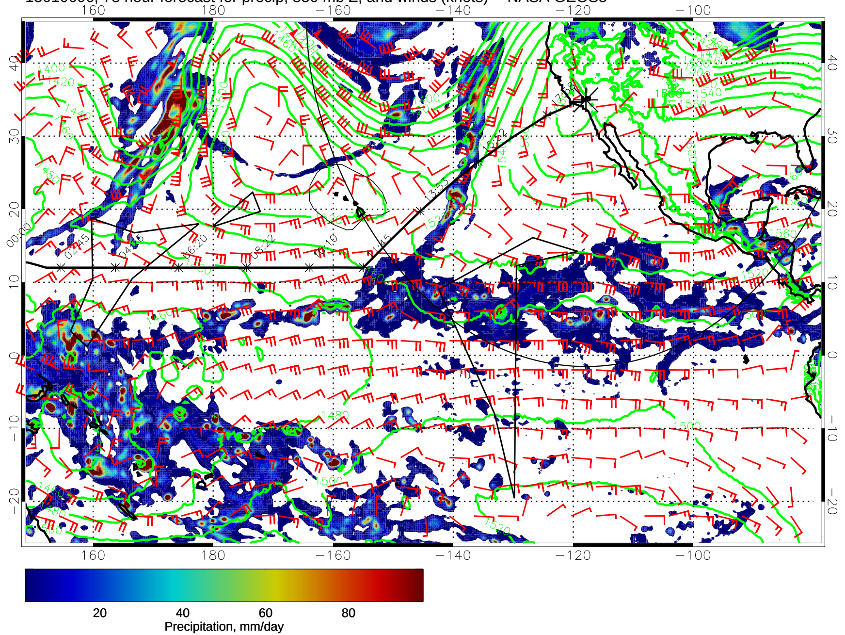
15010606, 78 hour forecast for precip, 850 mb Z, and winds (knots) -- NASA GEOS5
