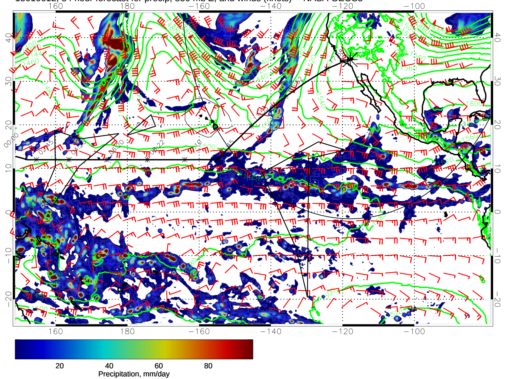
15010612, 84 hour forecast for precip, 850 mb Z, and winds (knots) -- NASA GEOS5
