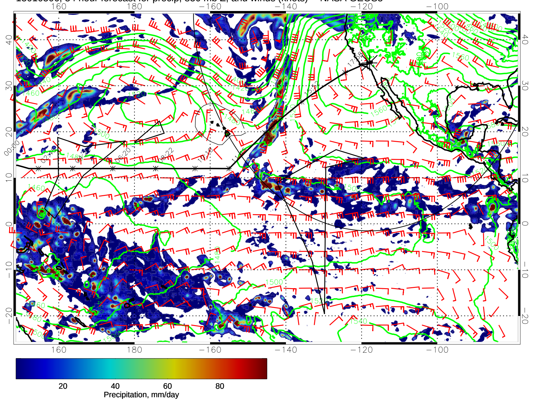
15010506, 54 hour forecast for precip, 850 mb Z, and winds (knots) -- NASA GEOS5
