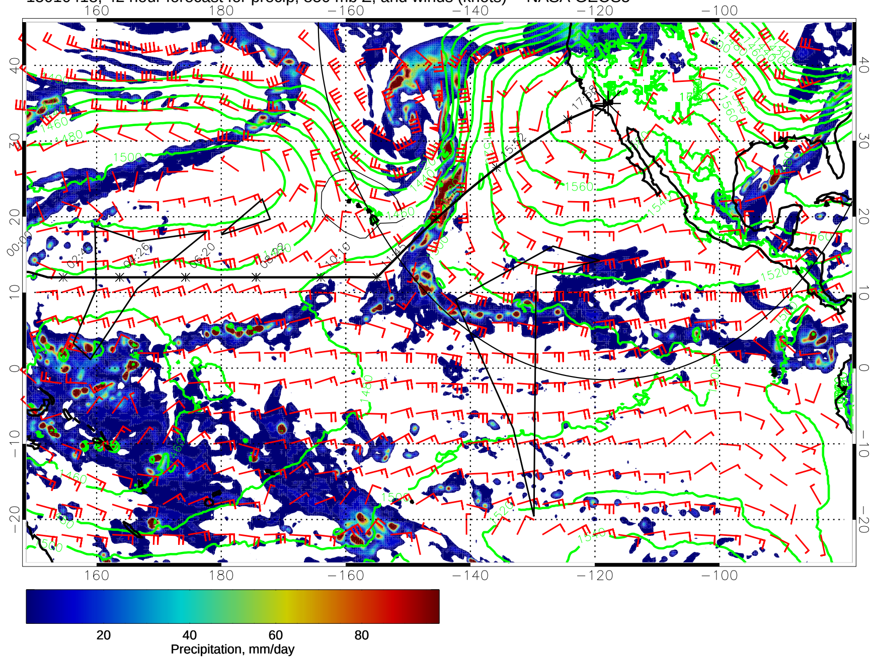
15010418, 42 hour forecast for precip, 850 mb Z, and winds (knots) -- NASA GEOS5
