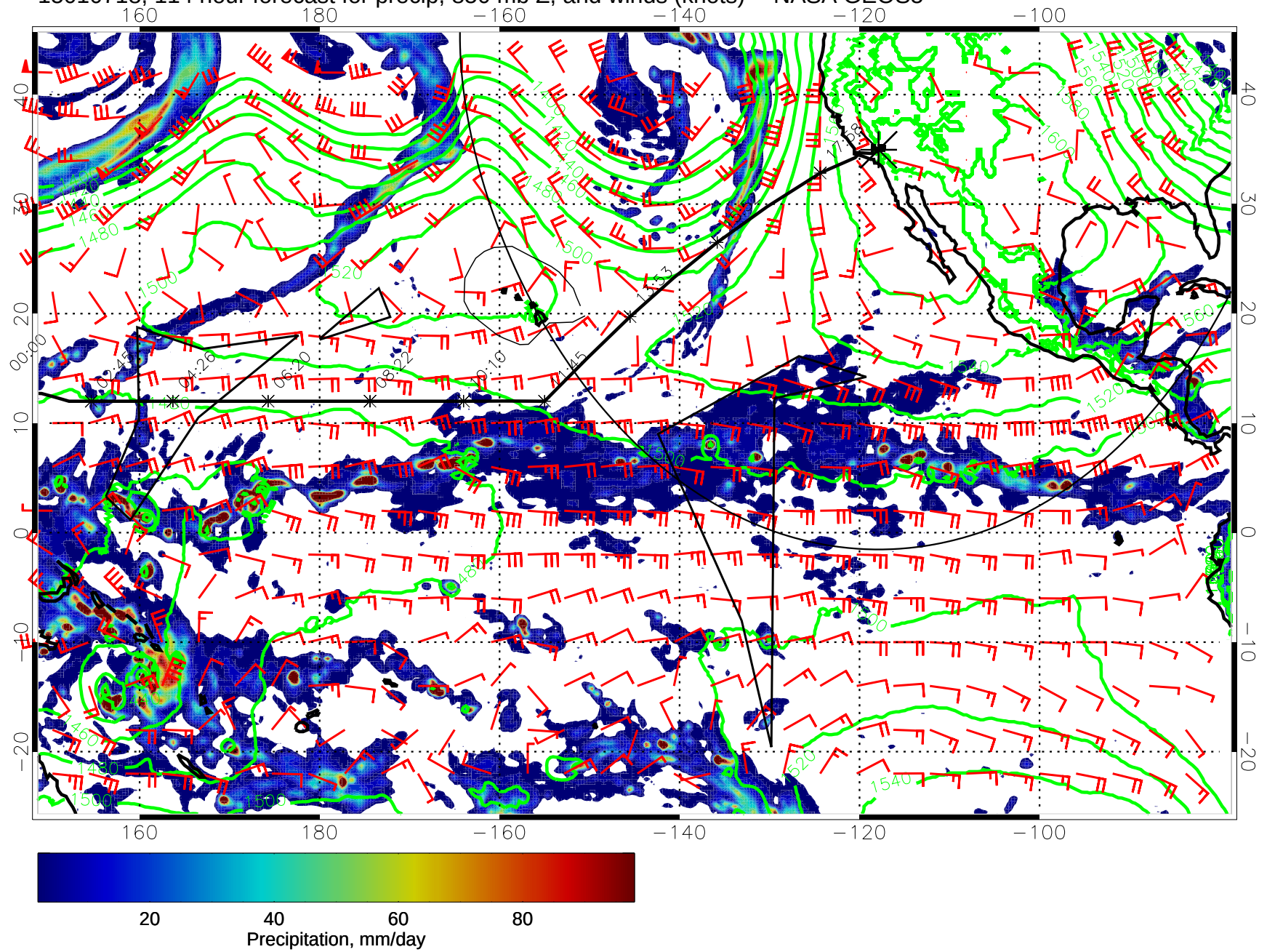
15010718, 114 hour forecast for precip, 850 mb Z, and winds (knots) -- NASA GEOS5
