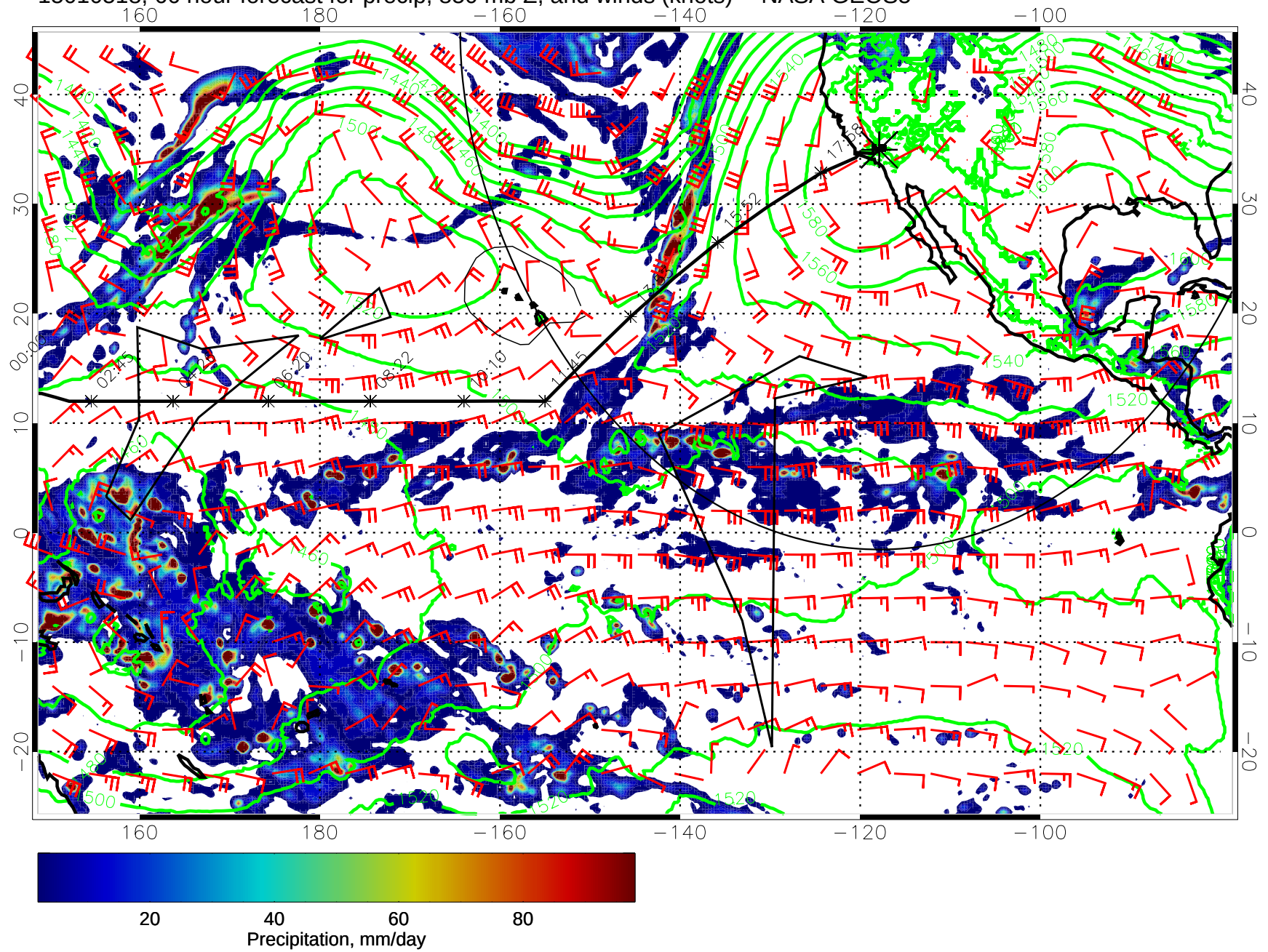
15010518, 66 hour forecast for precip, 850 mb Z, and winds (knots) -- NASA GEOS5
