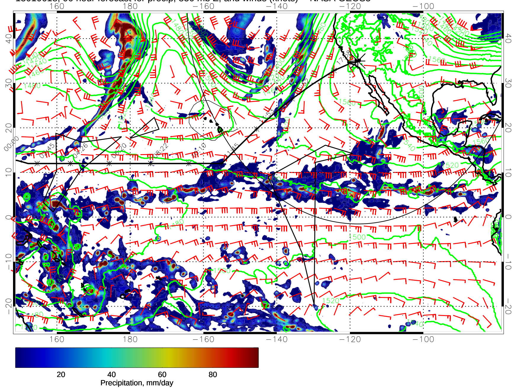
15010618, 90 hour forecast for precip, 850 mb Z, and winds (knots) -- NASA GEOS5
