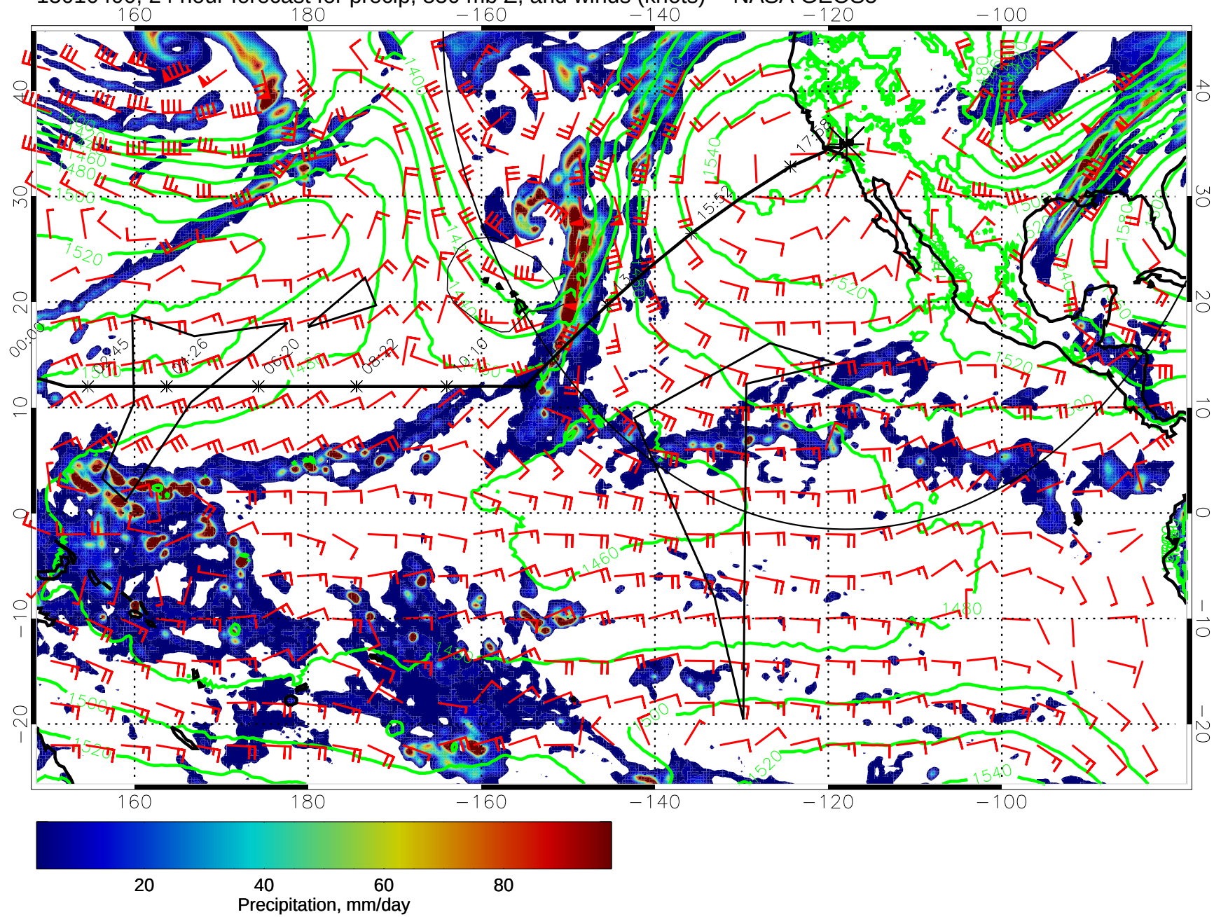
15010400, 24 hour forecast for precip, 850 mb Z, and winds (knots) -- NASA GEOS5
