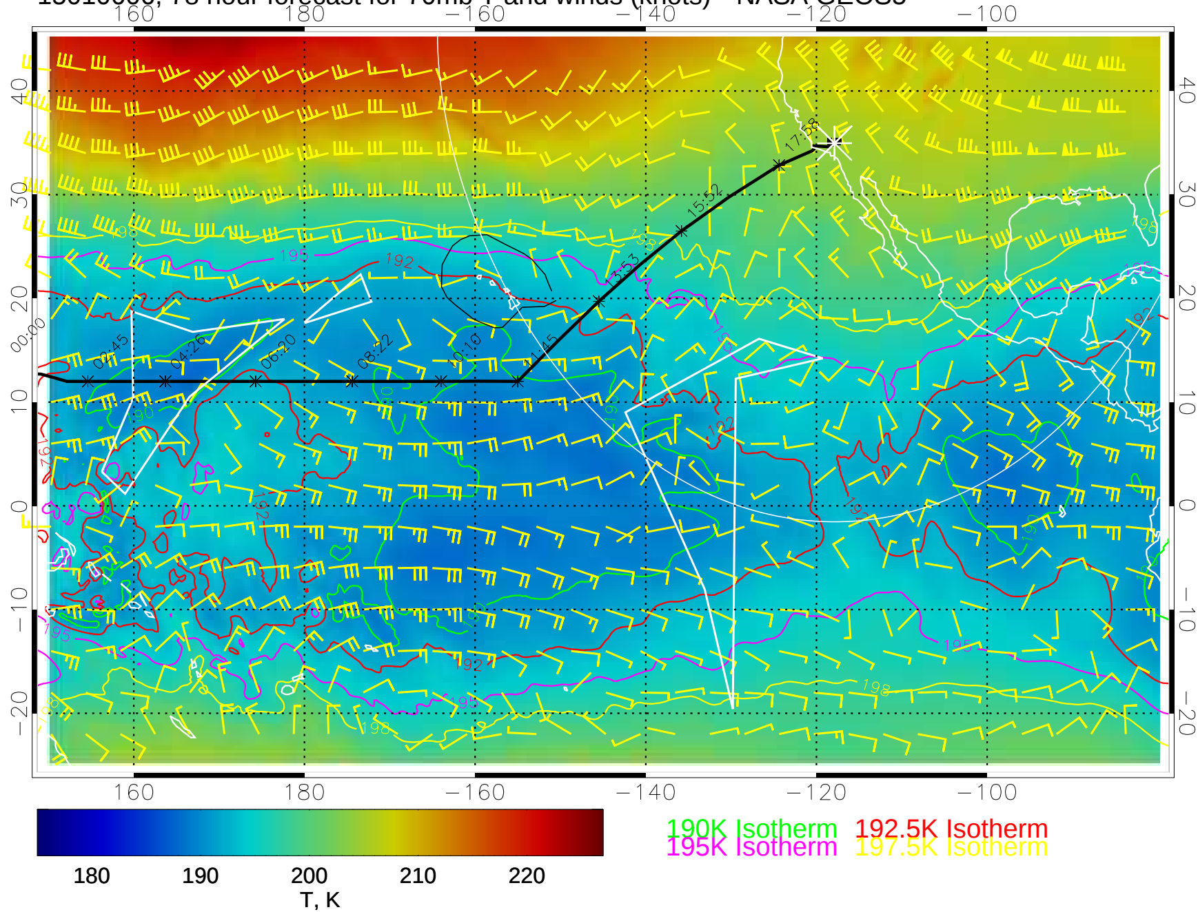
15010606, 78 hour forecast for 70mb T and winds (knots)-- NASA GEOS5
