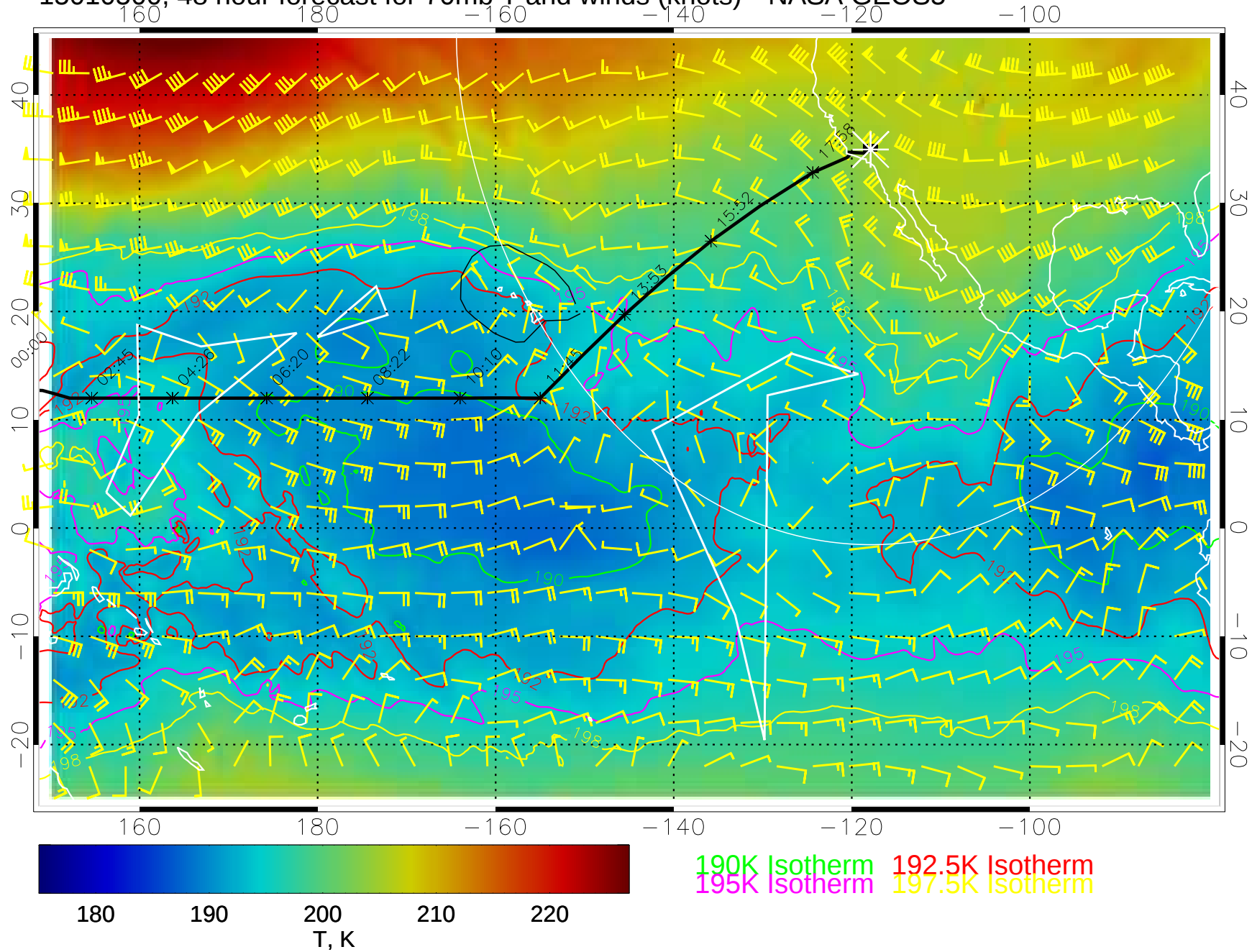
15010500, 48 hour forecast for 70mb T and winds (knots)-- NASA GEOS5
