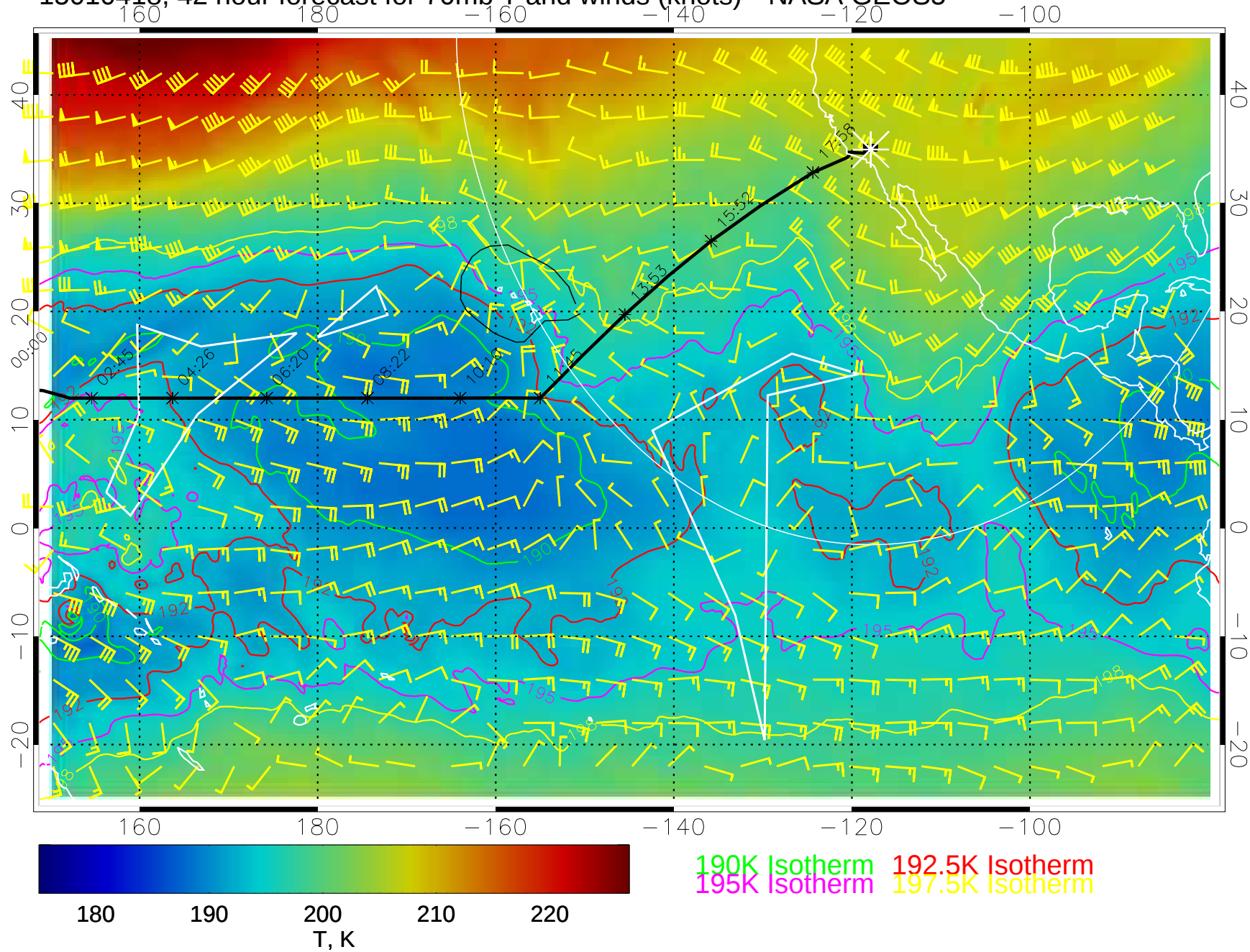
15010418, 42 hour forecast for 70mb T and winds (knots)-- NASA GEOS5
