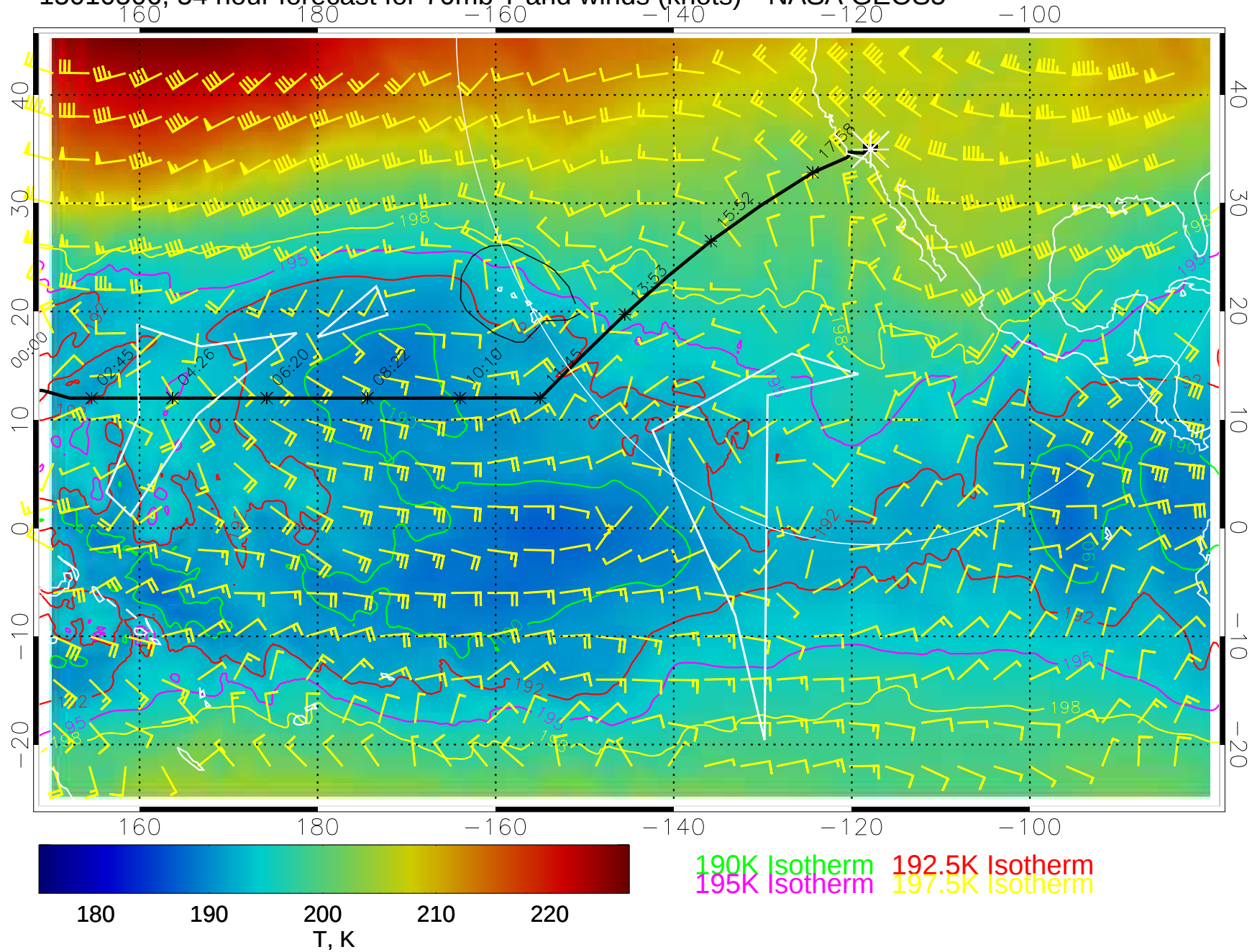
15010506, 54 hour forecast for 70mb T and winds (knots)-- NASA GEOS5
