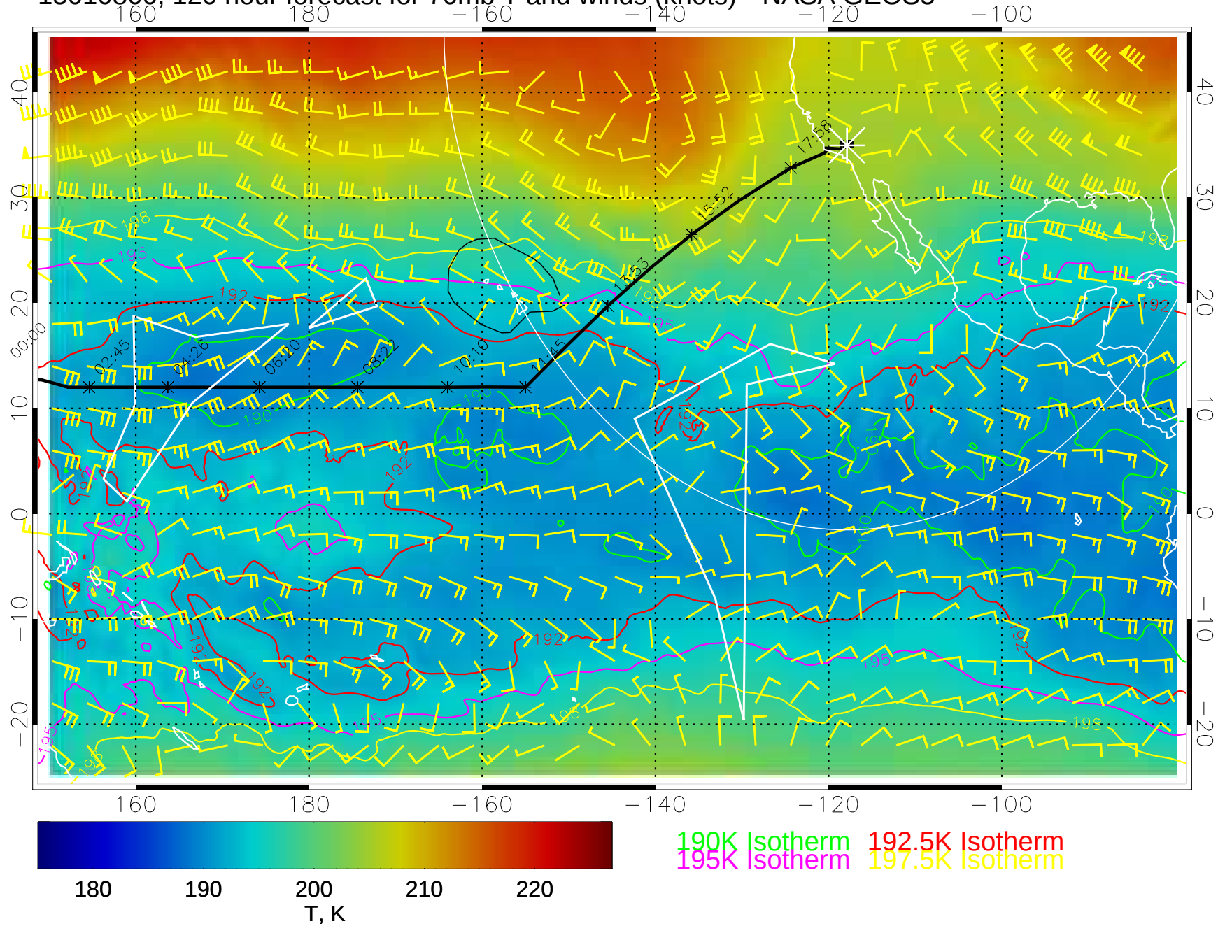
15010800, 120 hour forecast for 70mb T and winds (knots)-- NASA GEOS5
