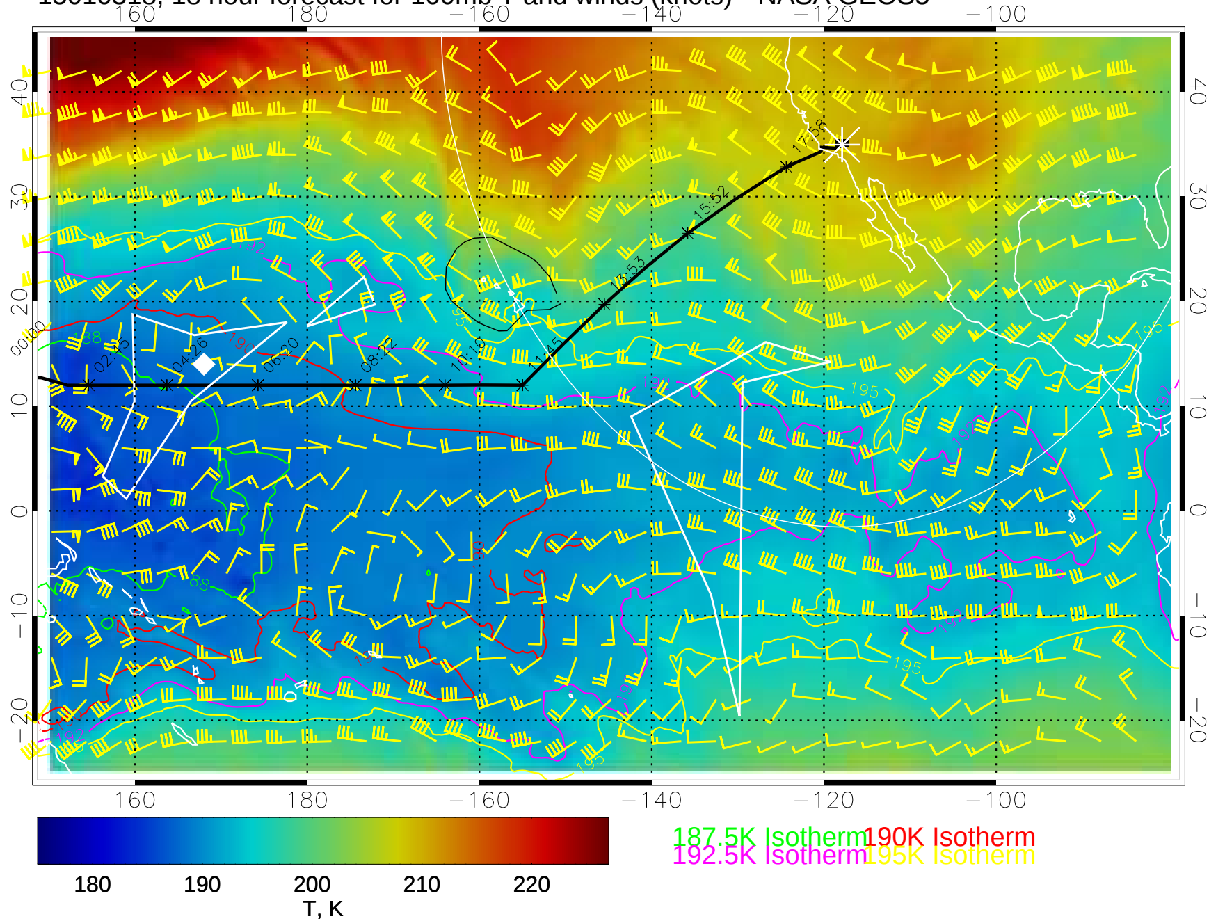
15010318, 18 hour forecast for 100mb T and winds (knots)-- NASA GEOS5
