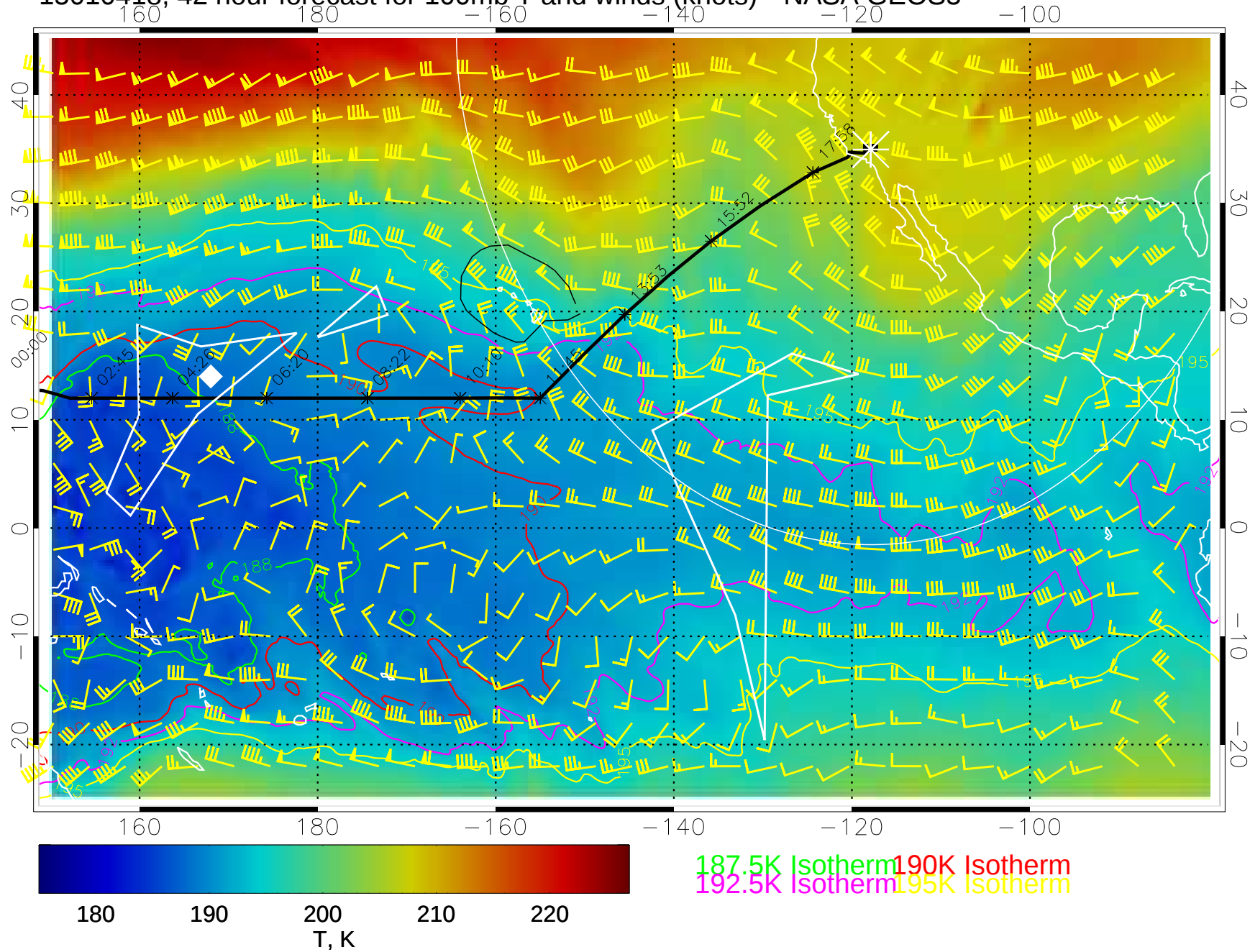
15010418, 42 hour forecast for 100mb T and winds (knots)-- NASA GEOS5
