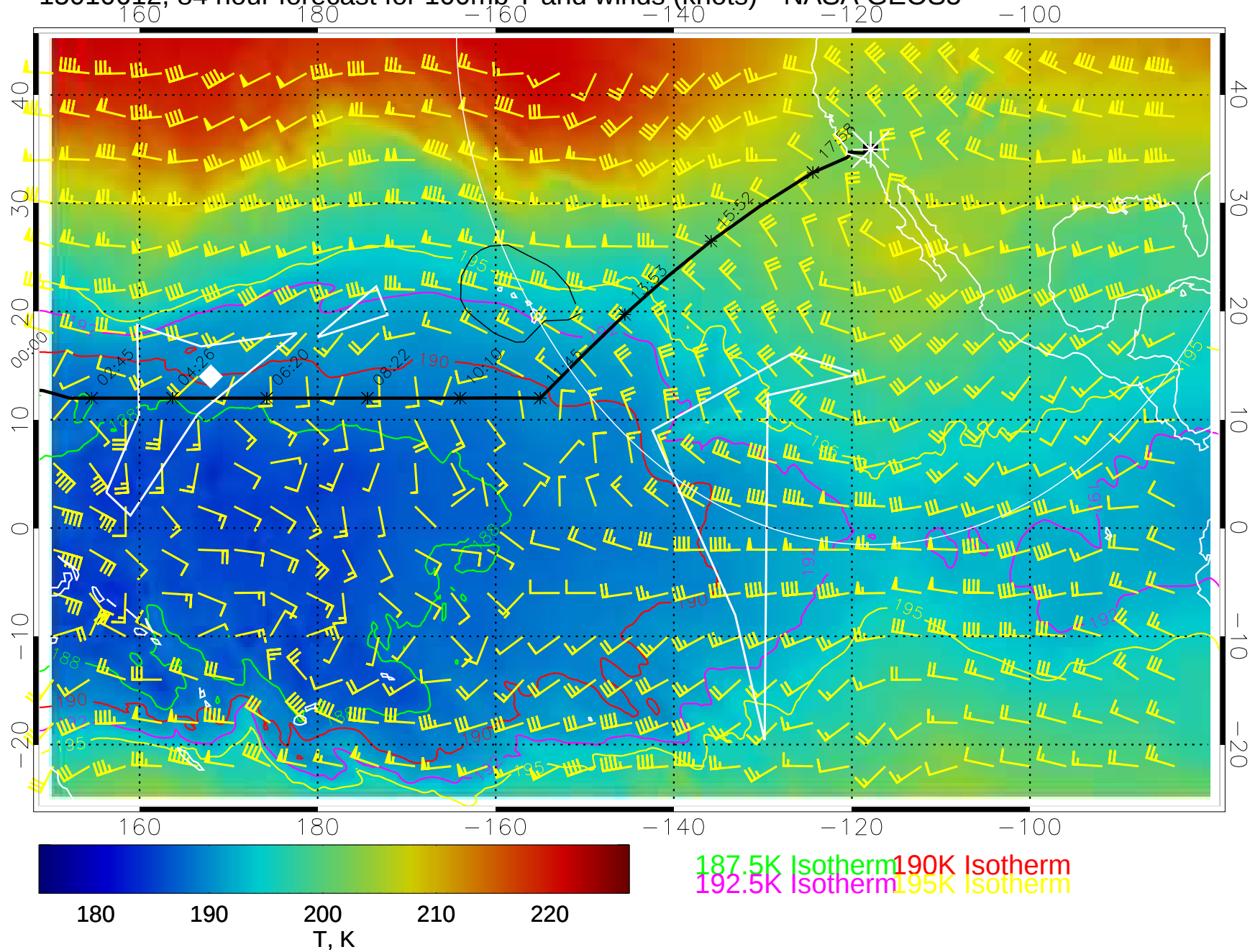
15010612, 84 hour forecast for 100mb T and winds (knots)-- NASA GEOS5
