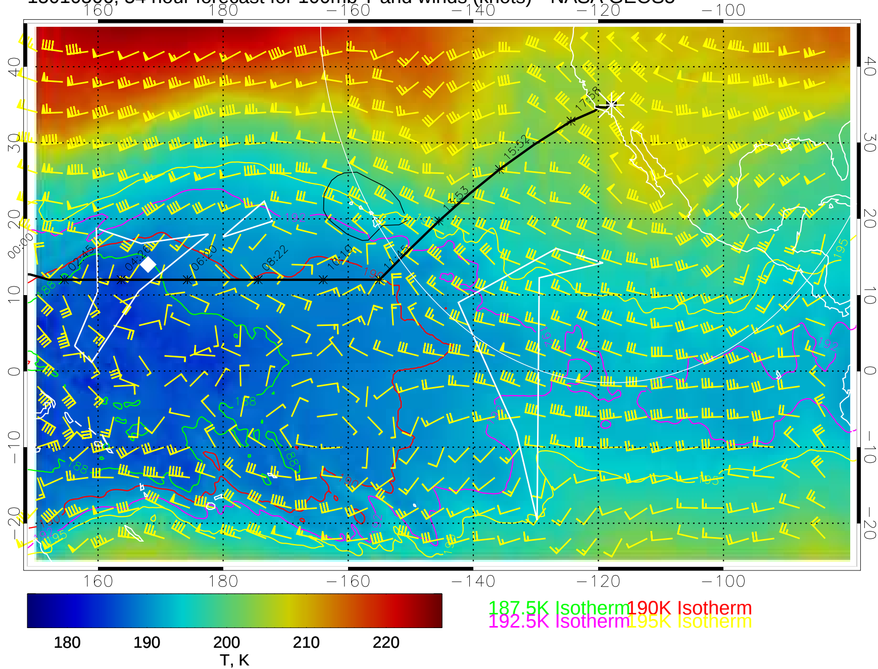
15010506, 54 hour forecast for 100mb T and winds (knots)-- NASA GEOS5
