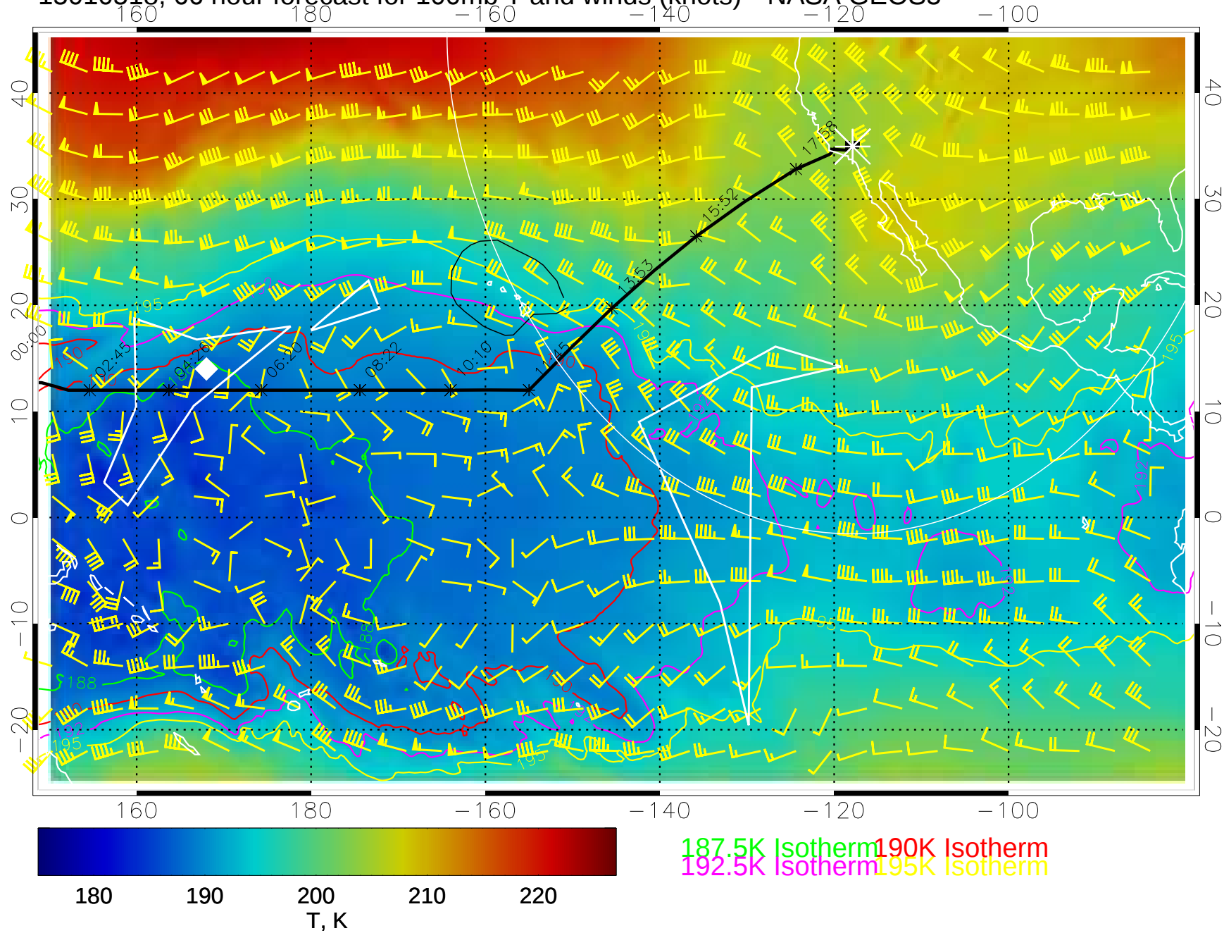
15010518, 66 hour forecast for 100mb T and winds (knots)-- NASA GEOS5
