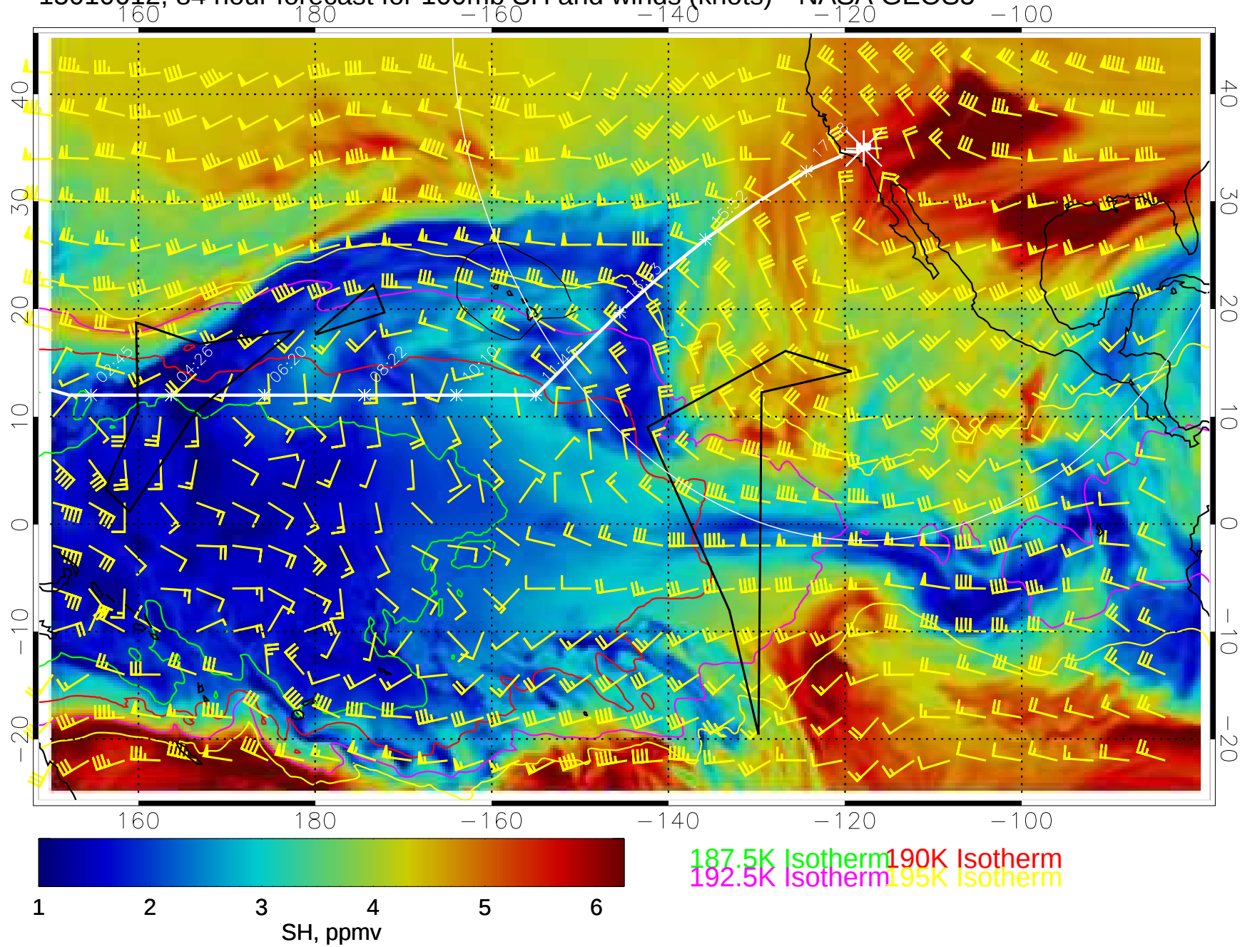
15010612, 84 hour forecast for 100mb SH and winds (knots)-- NASA GEOS5
