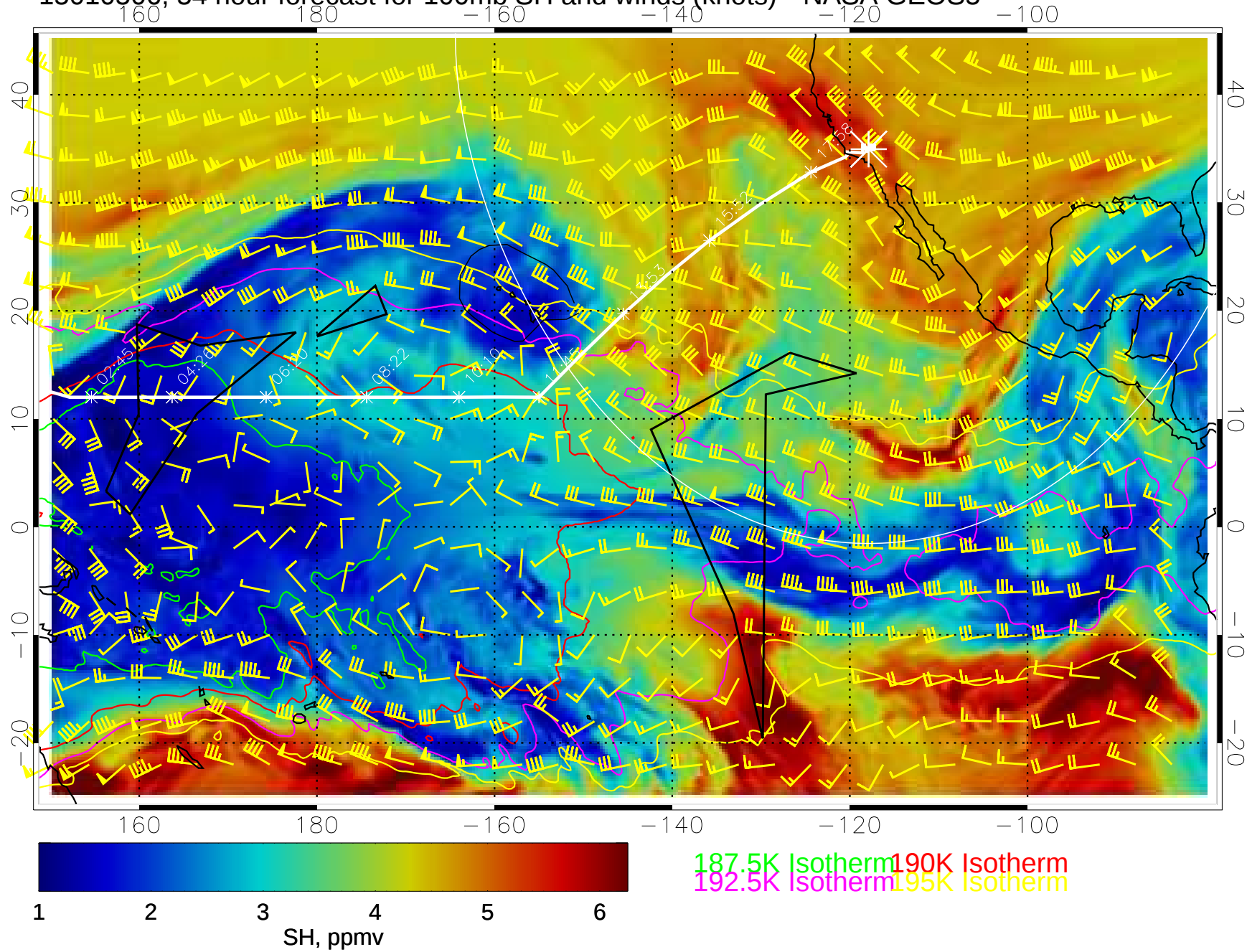
15010506, 54 hour forecast for 100mb SH and winds (knots)-- NASA GEOS5
