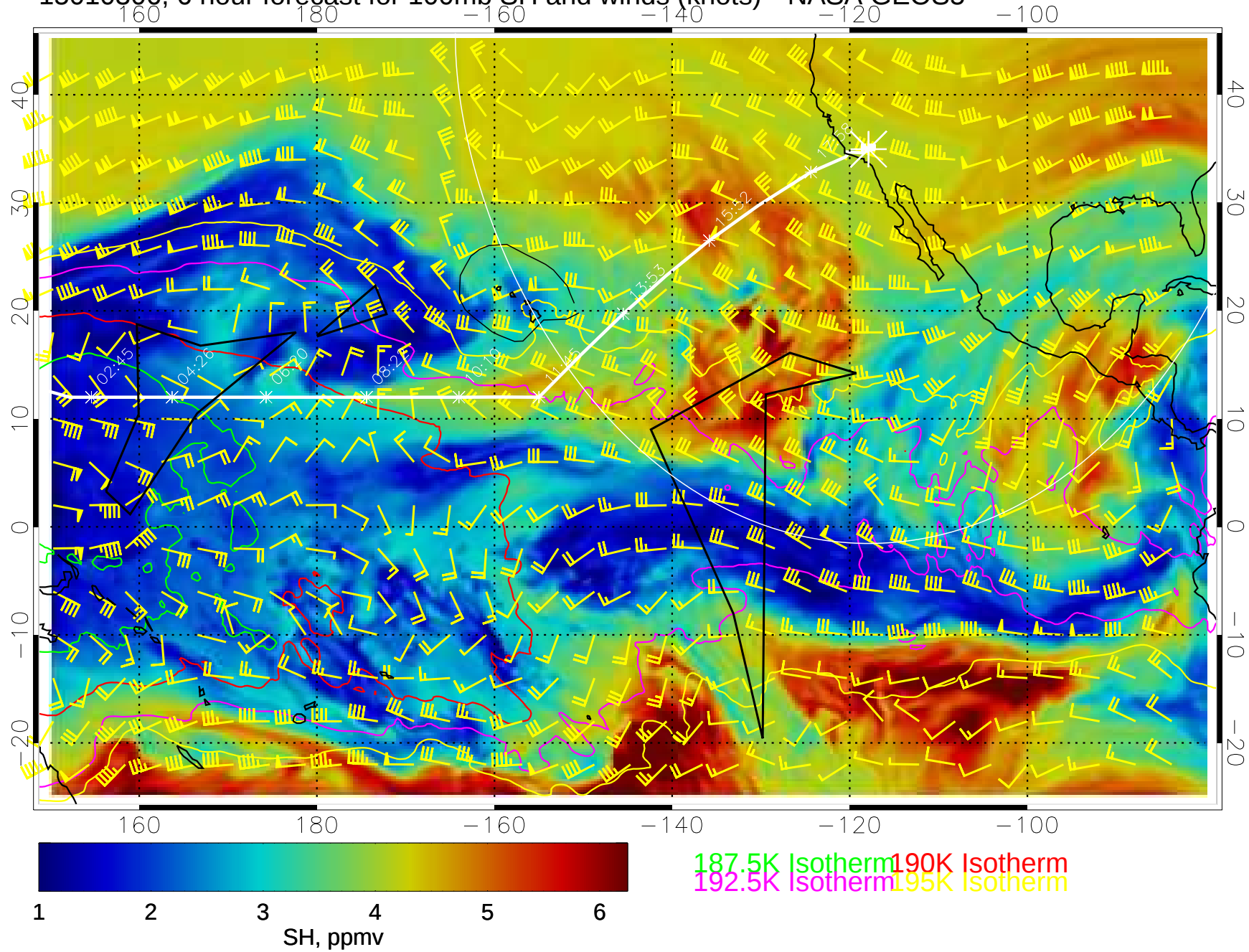
15010306, 6 hour forecast for 100mb SH and winds (knots)-- NASA GEOS5
