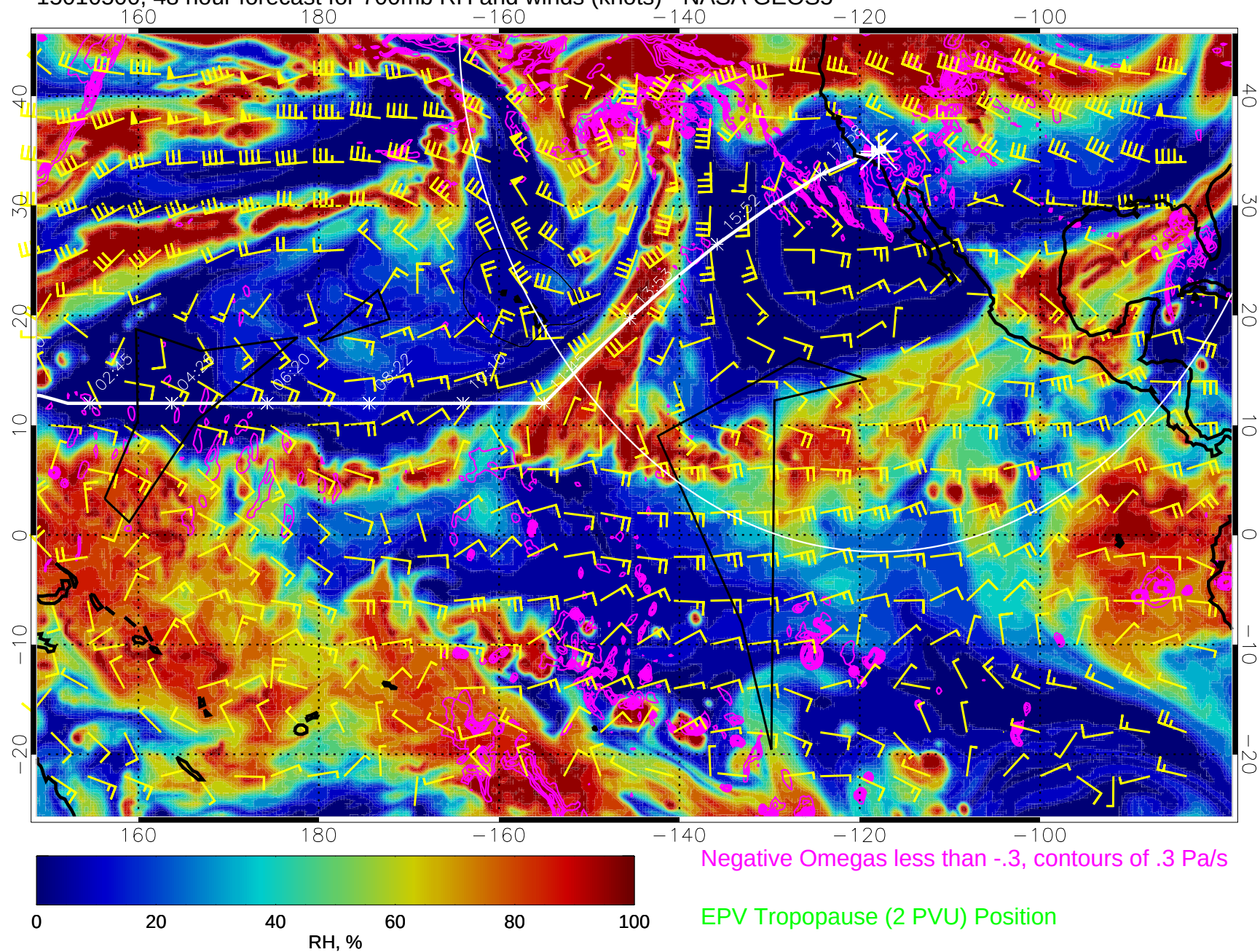
15010500, 48 hour forecast for 700mb RH and winds (knots) - NASA GEOS5
