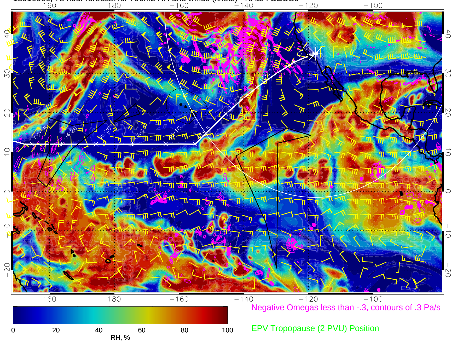
15010606, 78 hour forecast for 700mb RH and winds (knots) - NASA GEOS5
