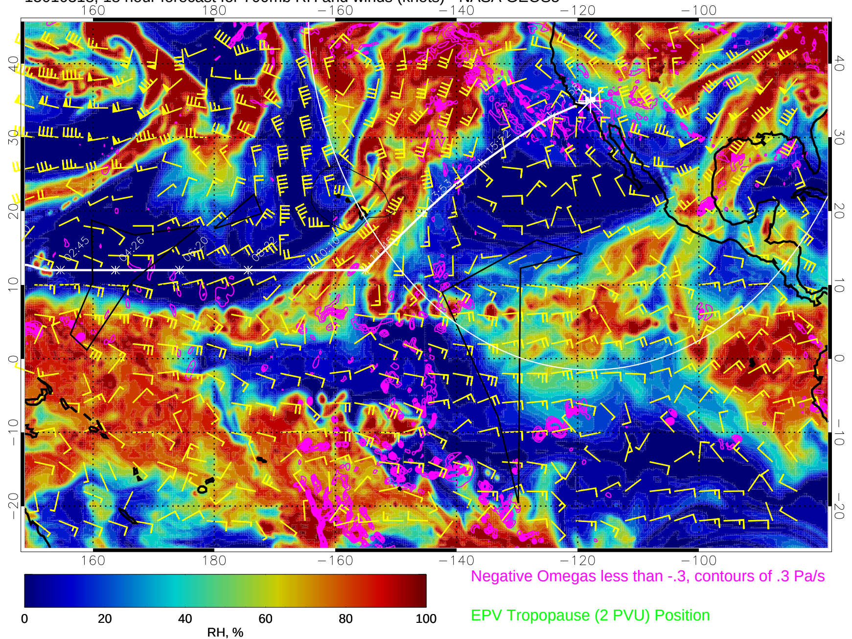
15010318, 18 hour forecast for 700mb RH and winds (knots) - NASA GEOS5
