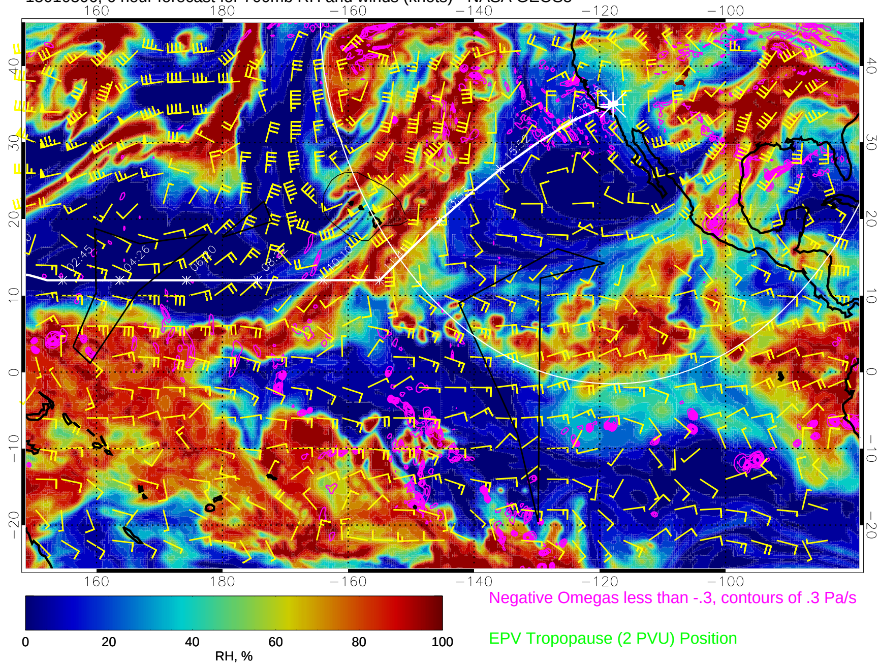
15010306, 6 hour forecast for 700mb RH and winds (knots) - NASA GEOS5
