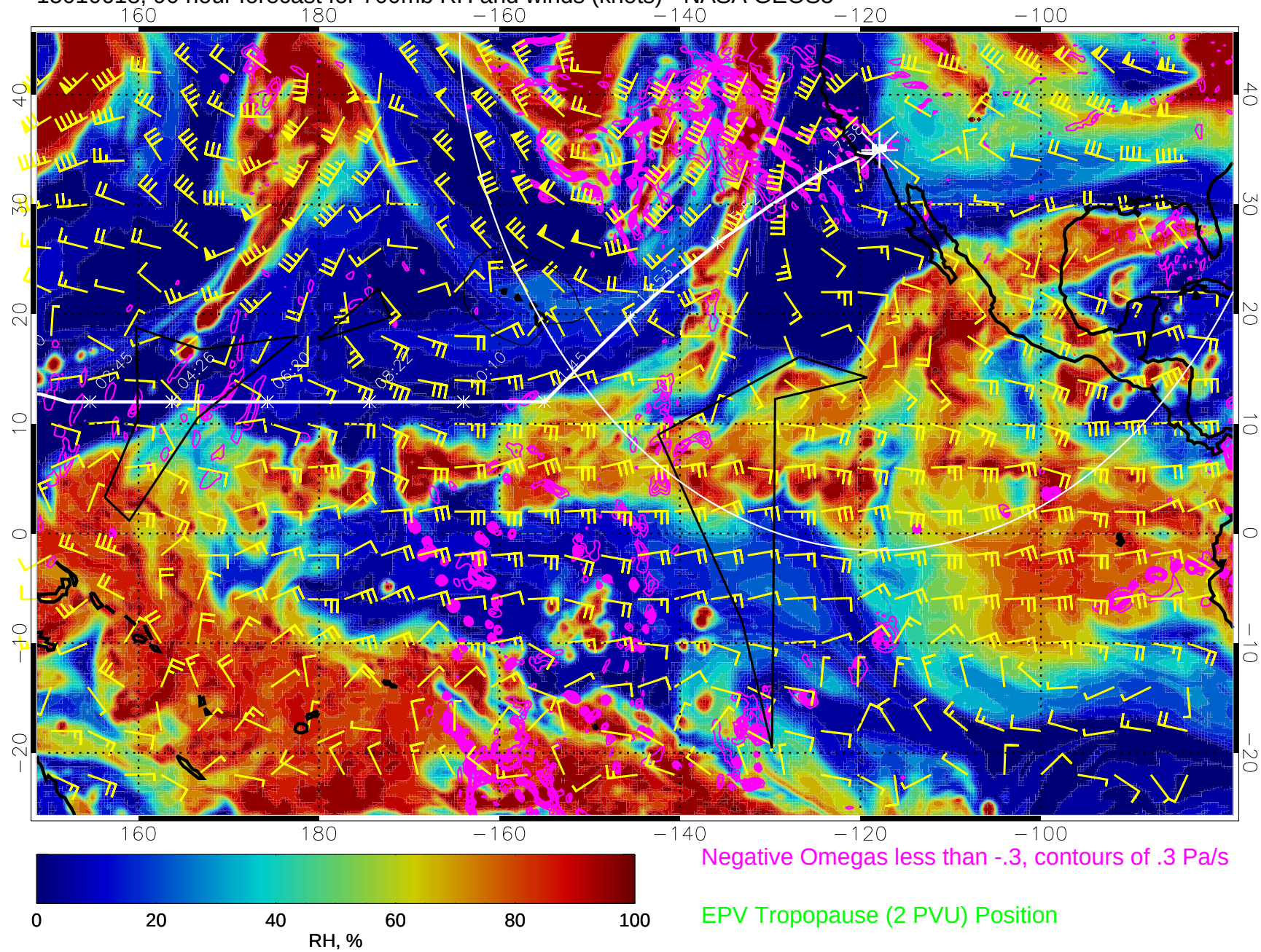
15010618, 90 hour forecast for 700mb RH and winds (knots) - NASA GEOS5
