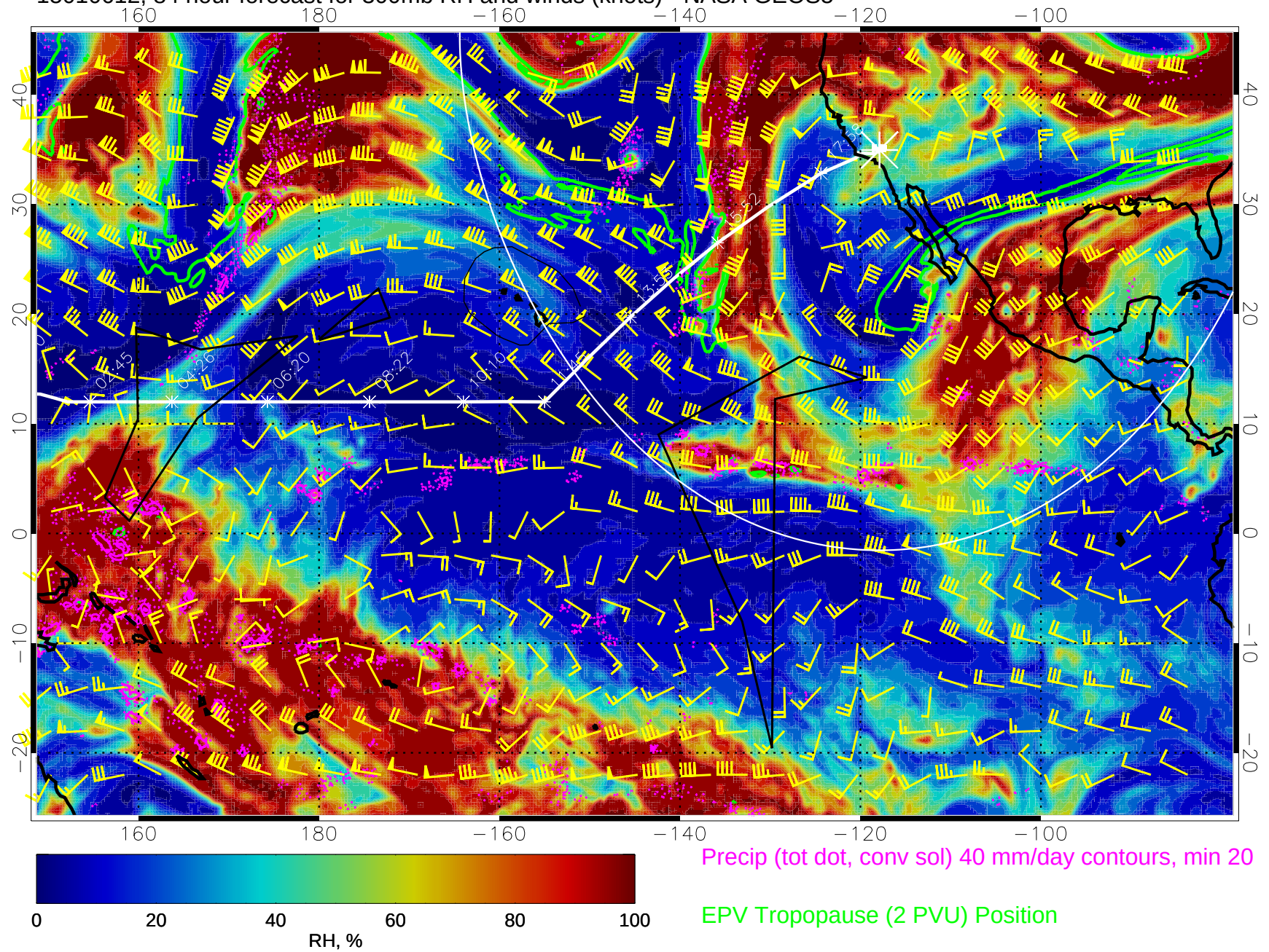
15010612, 84 hour forecast for 300mb RH and winds (knots) - NASA GEOS5
