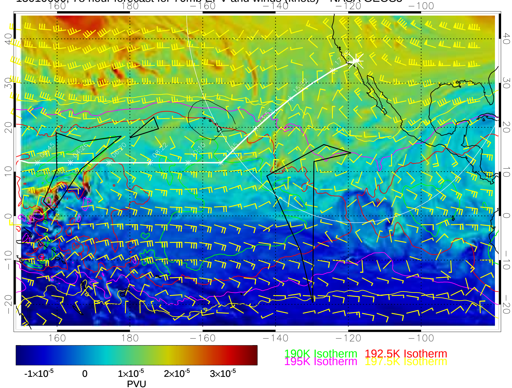
15010606, 78 hour forecast for 70mb EPV and winds (knots)-- NASA GEOS5
