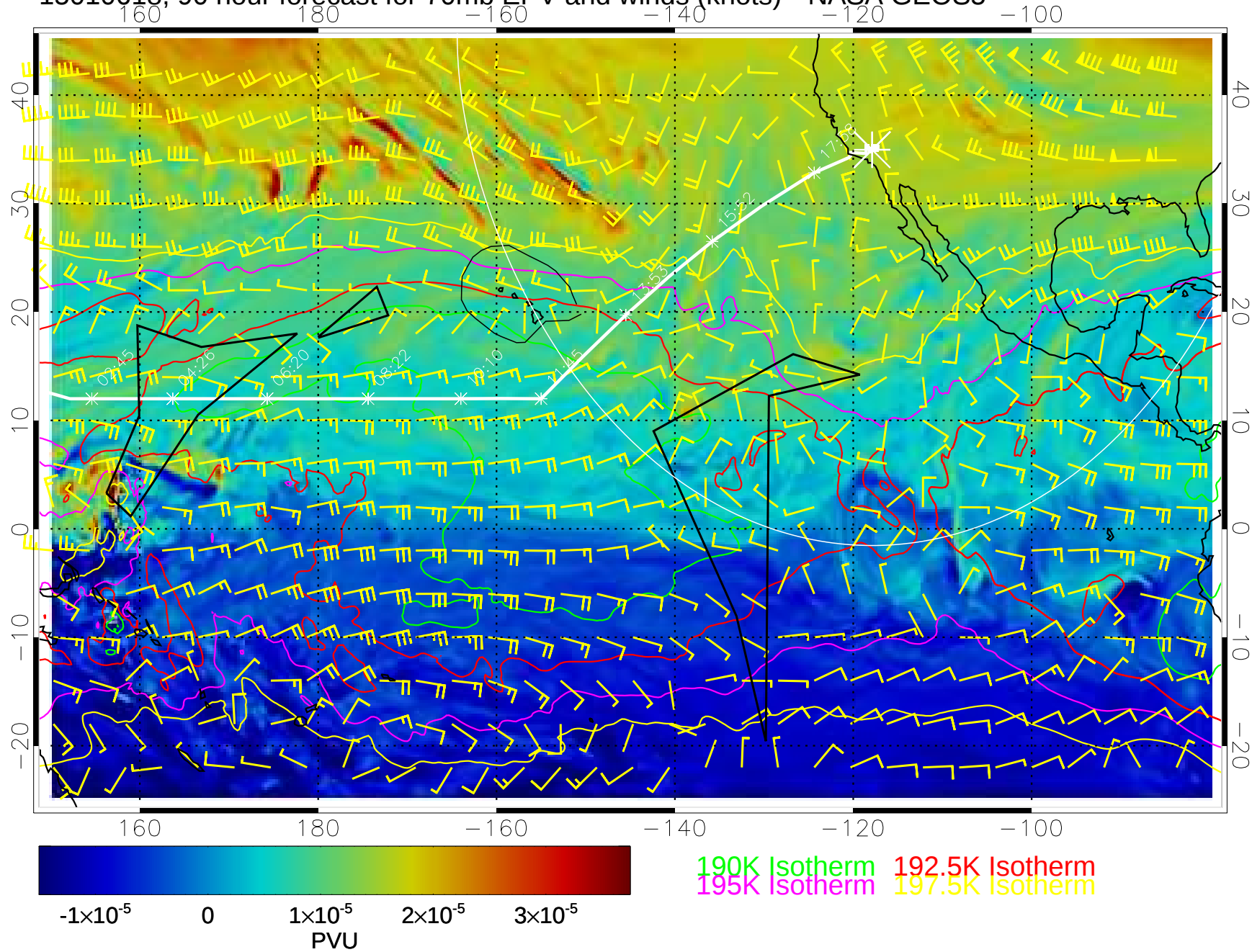
15010618, 90 hour forecast for 70mb EPV and winds (knots)-- NASA GEOS5
