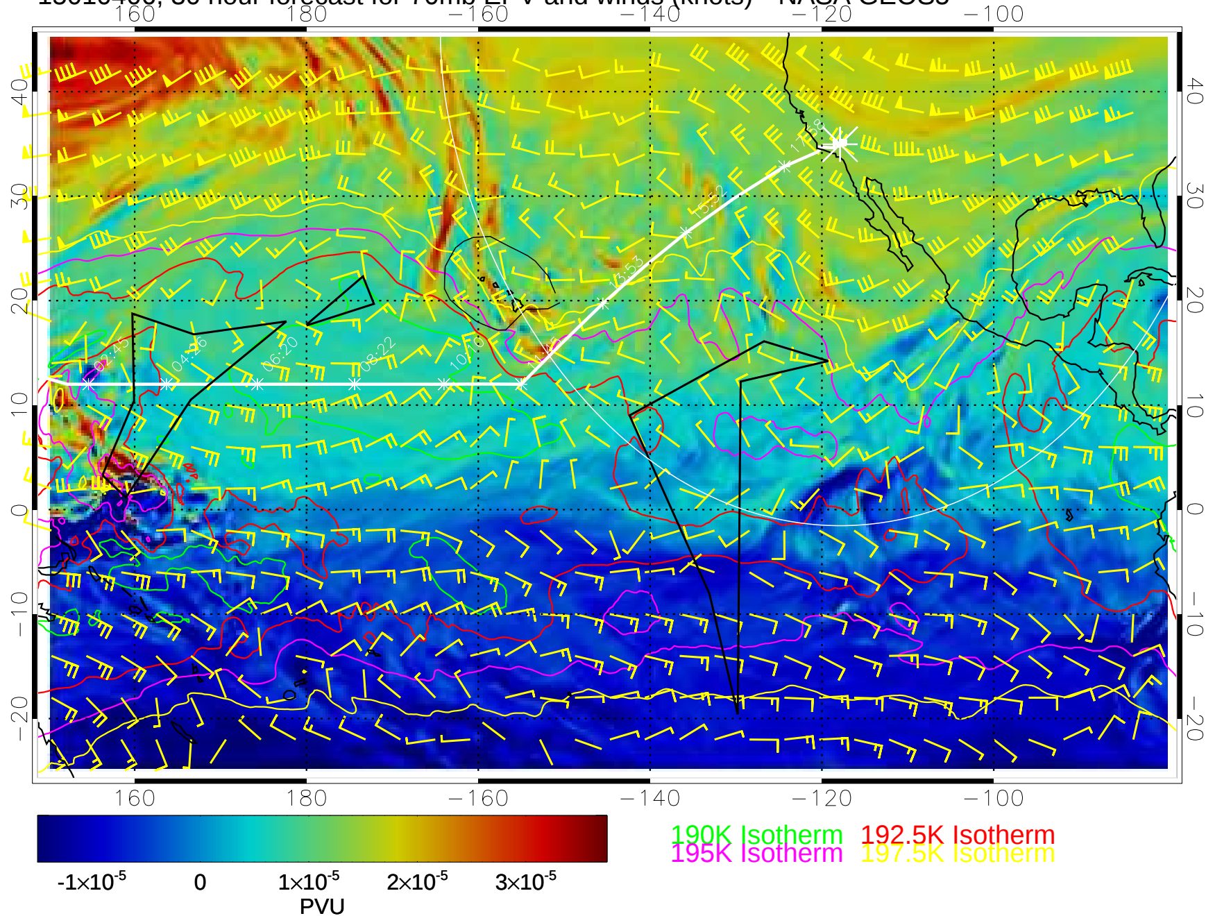
15010406, 30 hour forecast for 70mb EPV and winds (knots)-- NASA GEOS5
