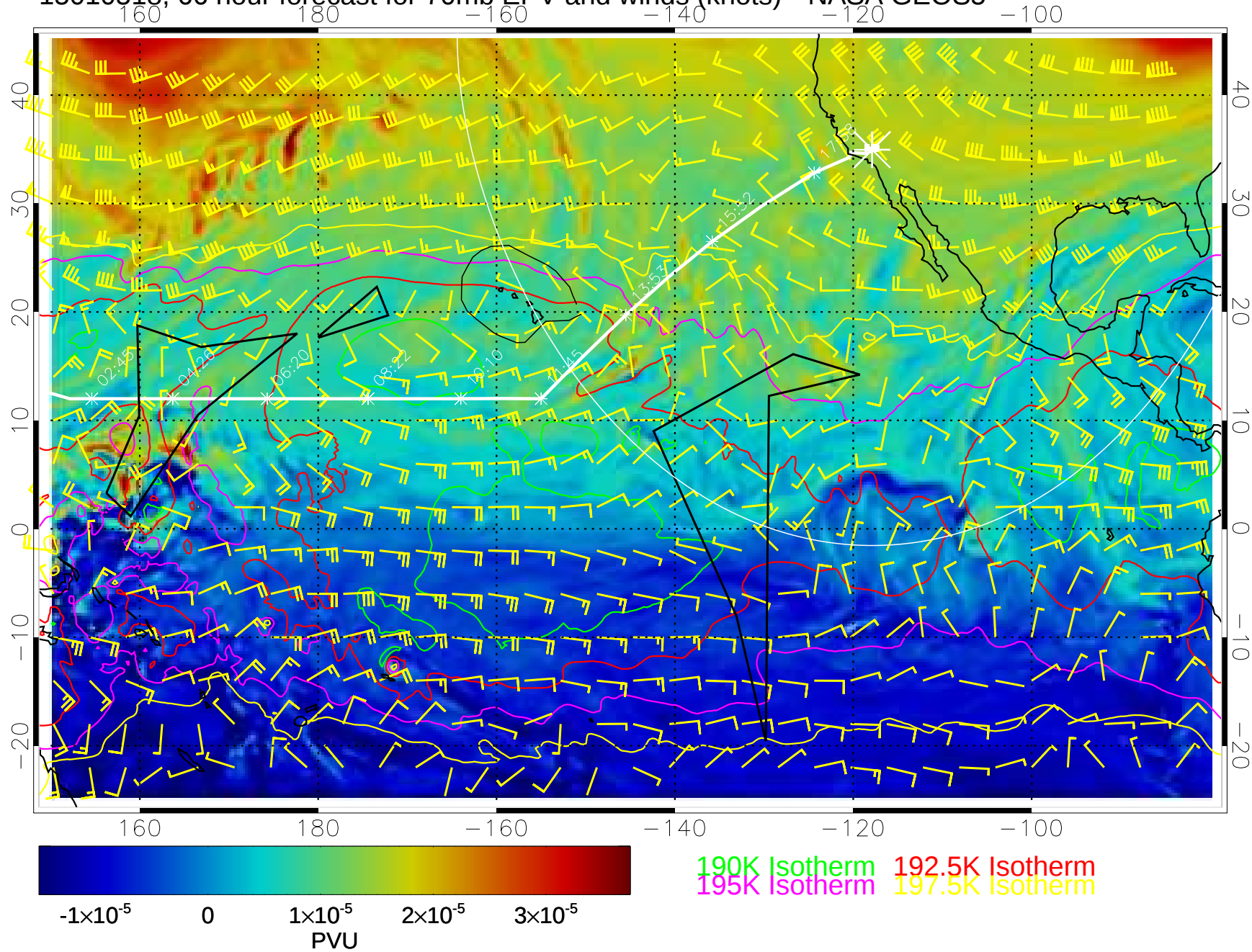
15010518, 66 hour forecast for 70mb EPV and winds (knots)-- NASA GEOS5
