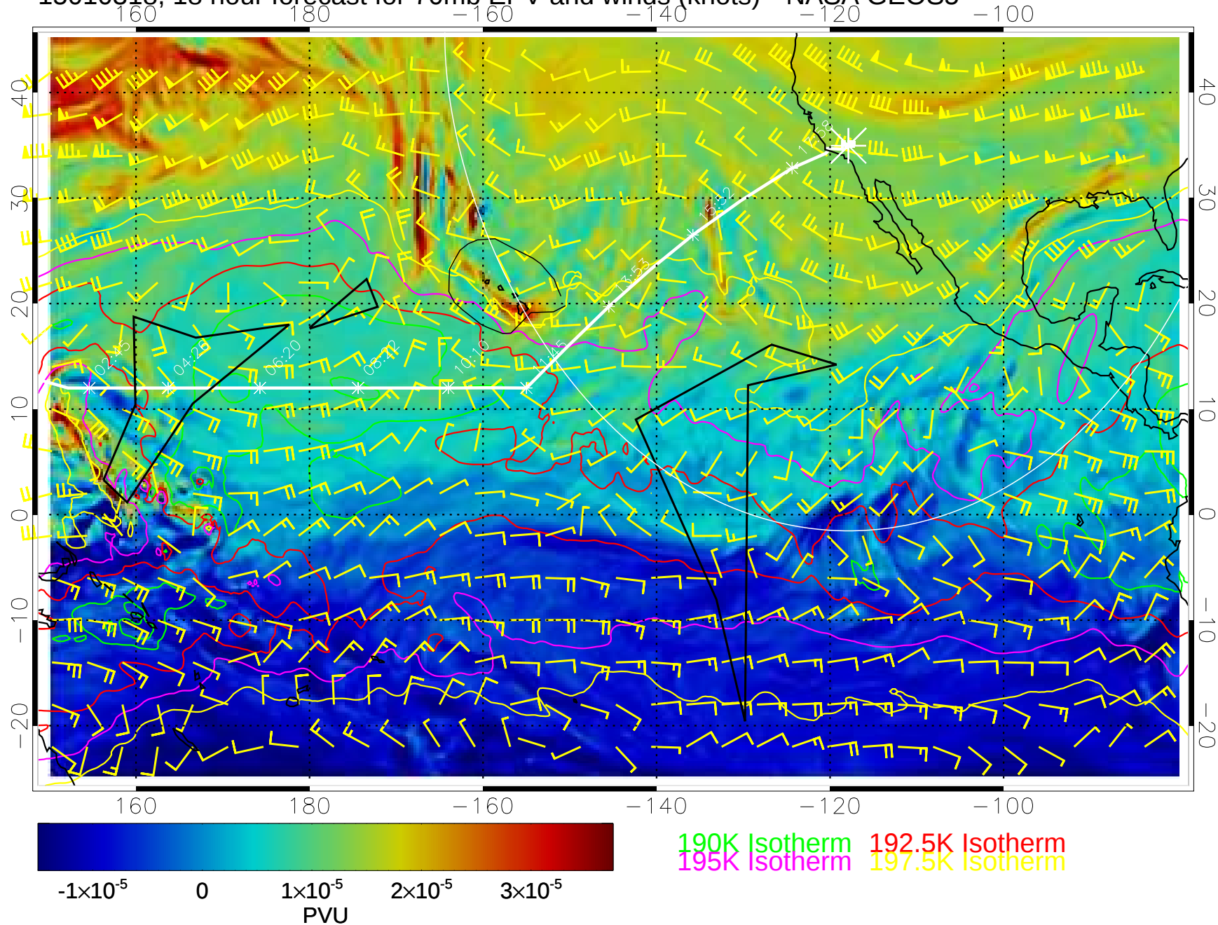
15010318, 18 hour forecast for 70mb EPV and winds (knots)-- NASA GEOS5
