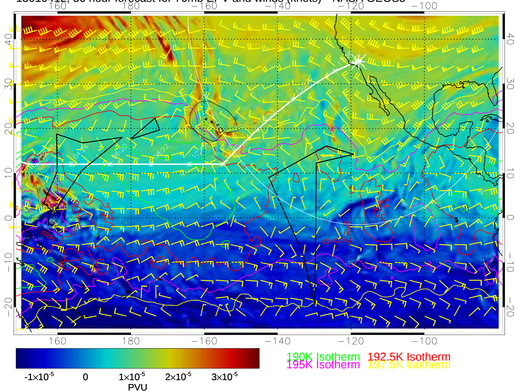
15010412, 36 hour forecast for 70mb EPV and winds (knots)-- NASA GEOS5
