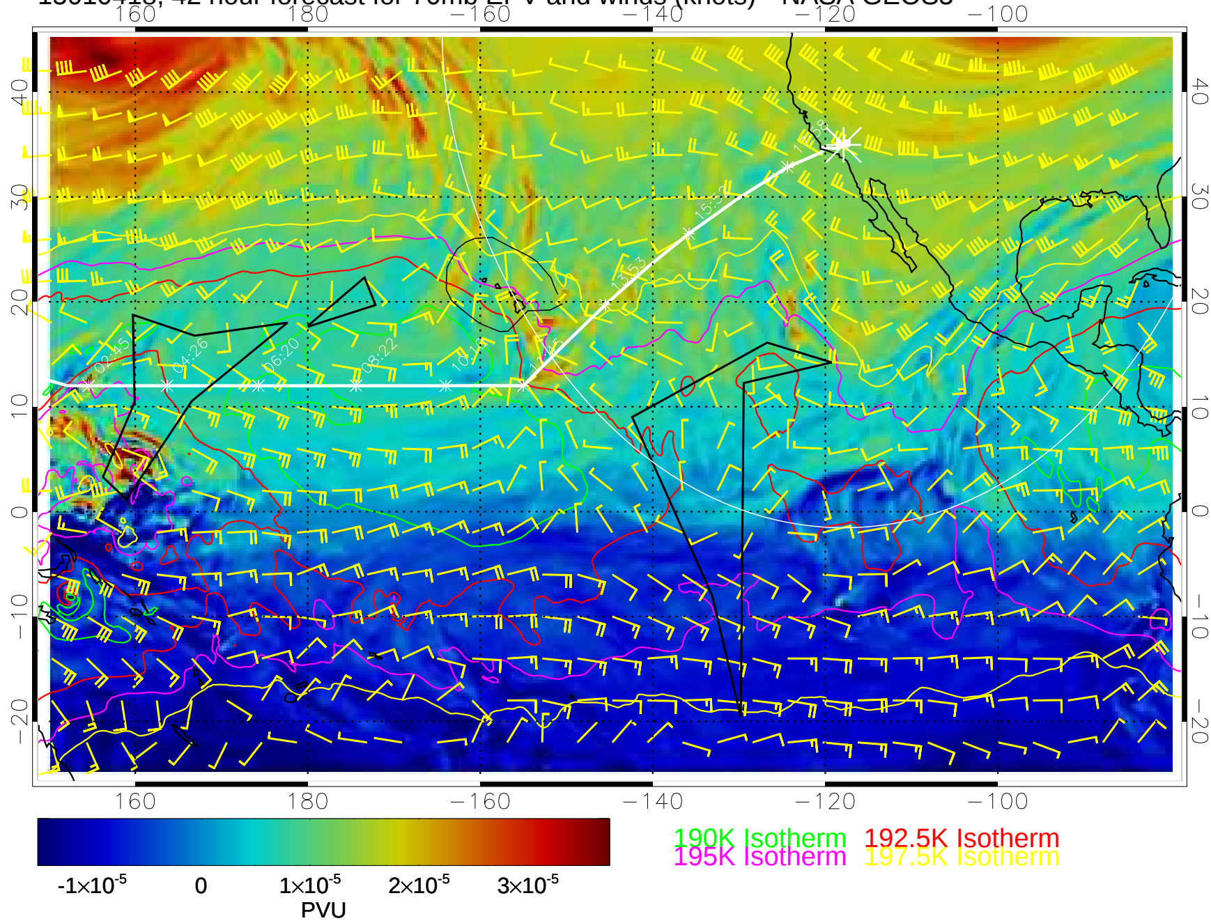
15010418, 42 hour forecast for 70mb EPV and winds (knots)-- NASA GEOS5
