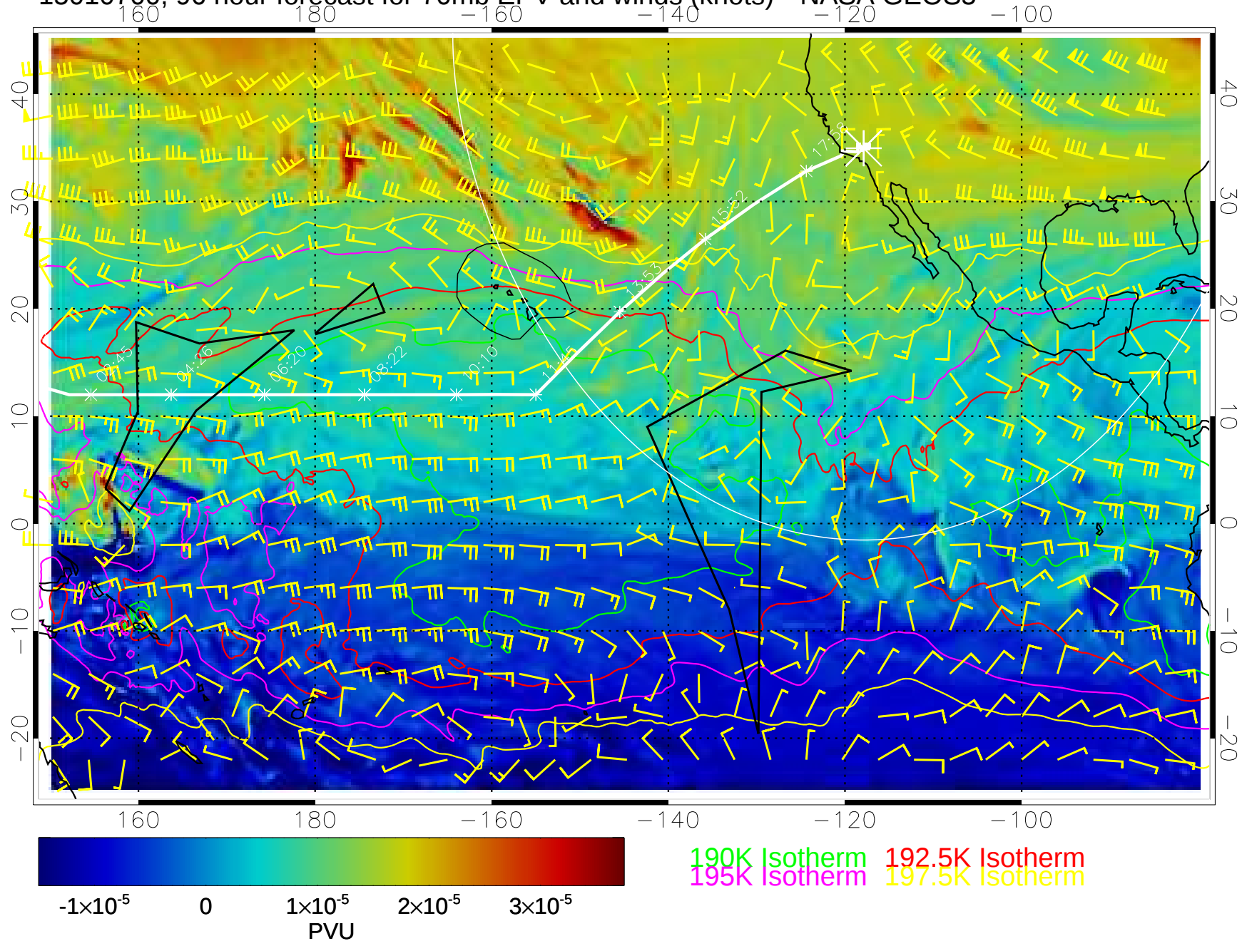
15010700, 96 hour forecast for 70mb EPV and winds (knots)-- NASA GEOS5
