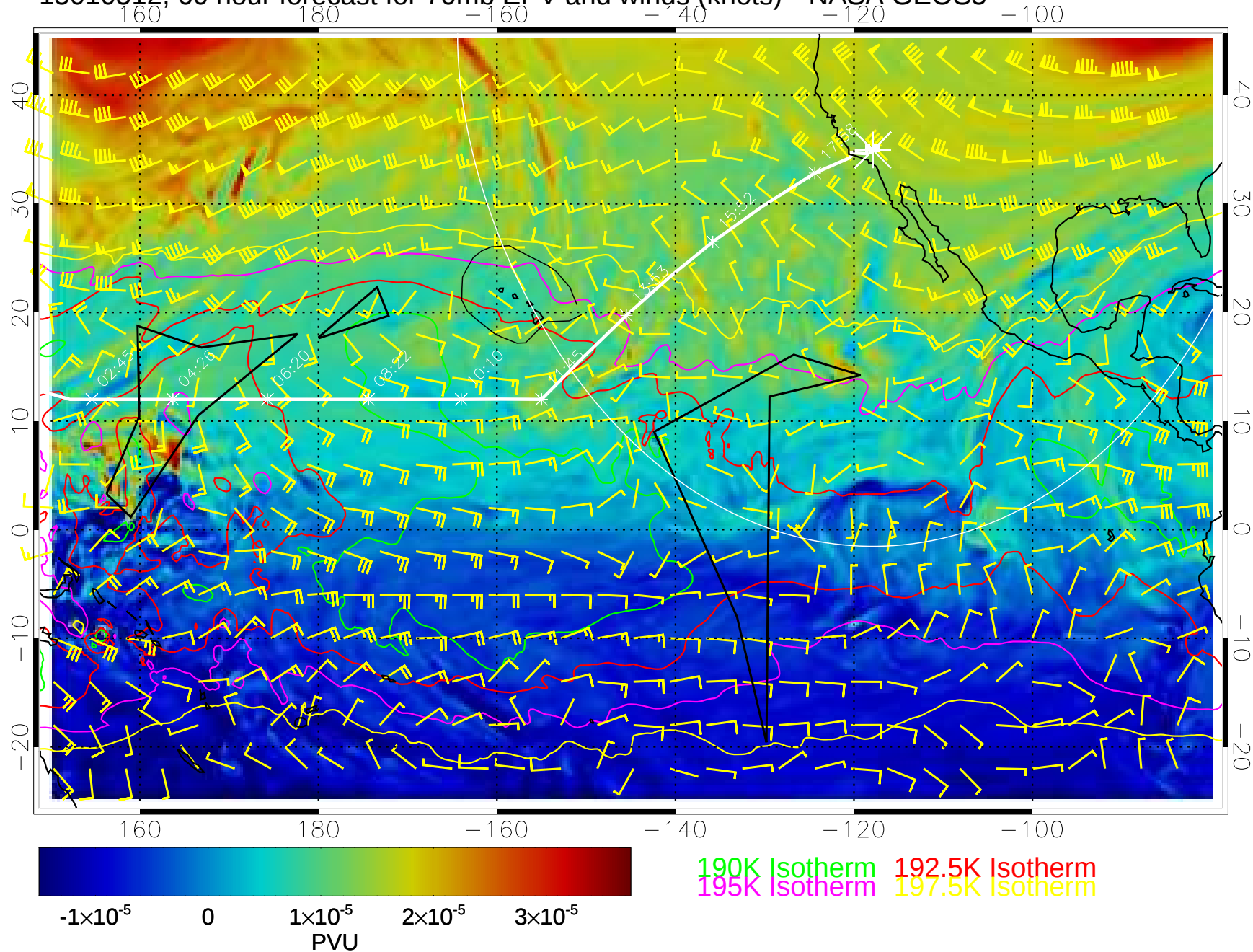
15010512, 60 hour forecast for 70mb EPV and winds (knots)-- NASA GEOS5
