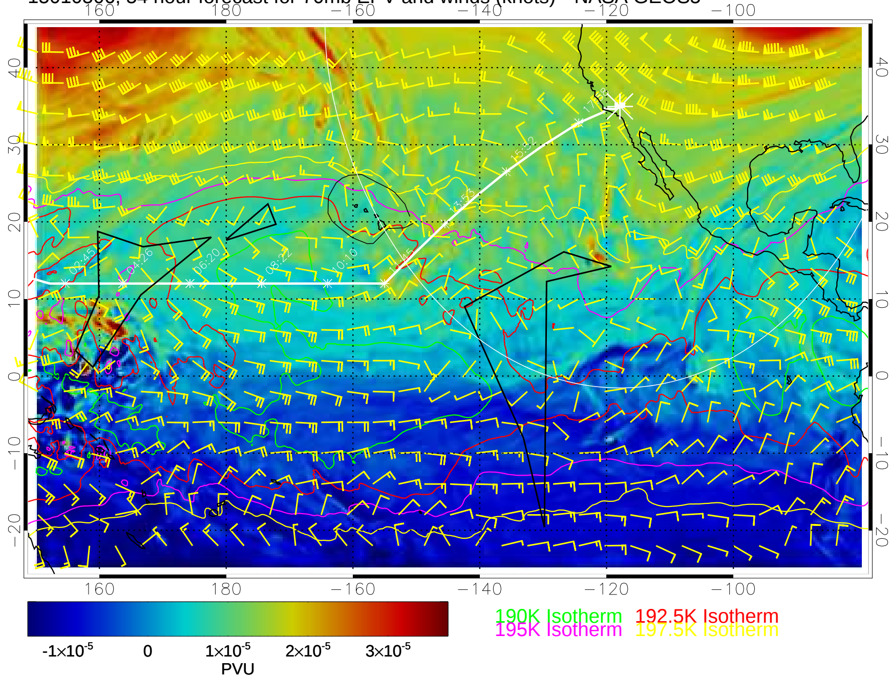
15010506, 54 hour forecast for 70mb EPV and winds (knots)-- NASA GEOS5
