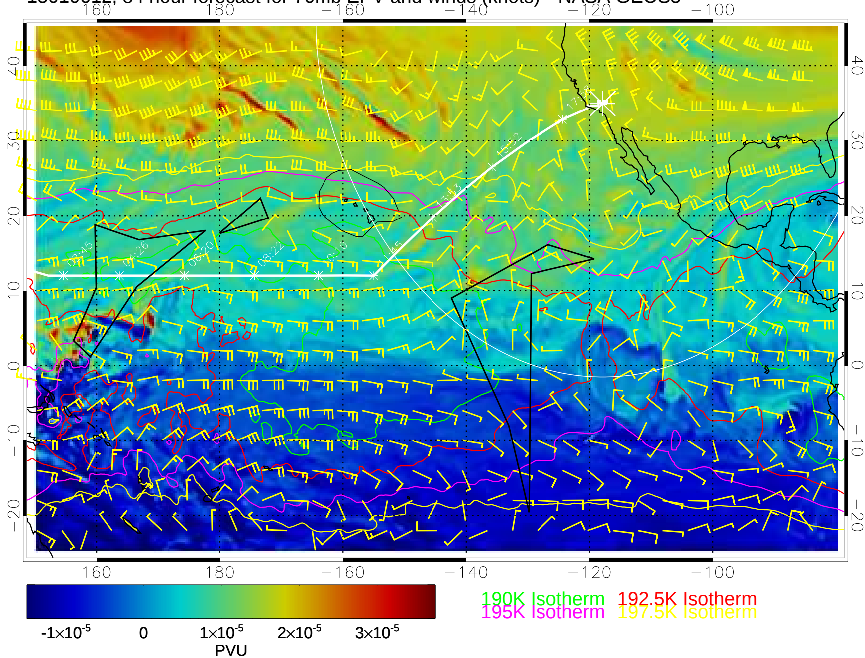
15010612, 84 hour forecast for 70mb EPV and winds (knots)-- NASA GEOS5
