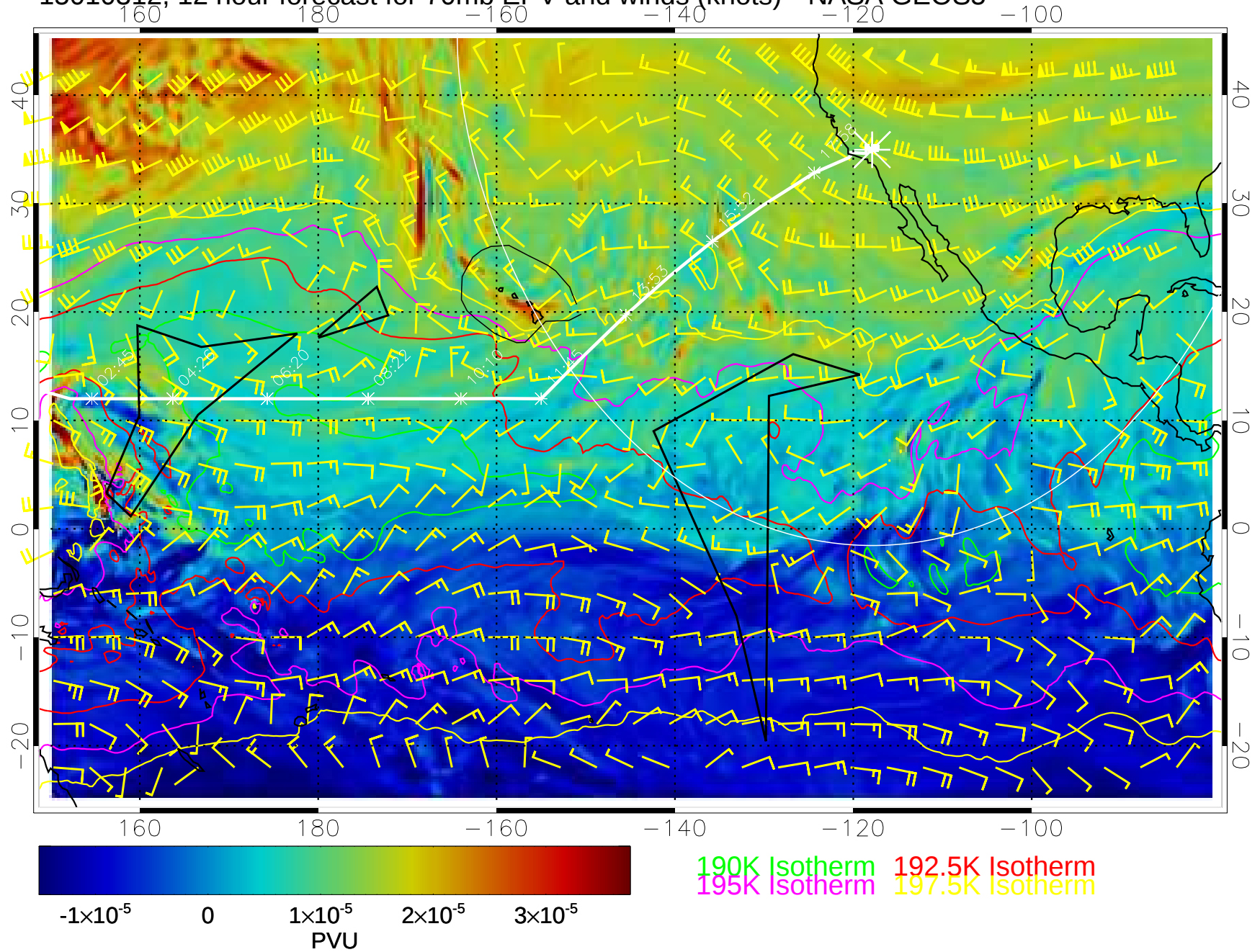
15010312, 12 hour forecast for 70mb EPV and winds (knots)-- NASA GEOS5
