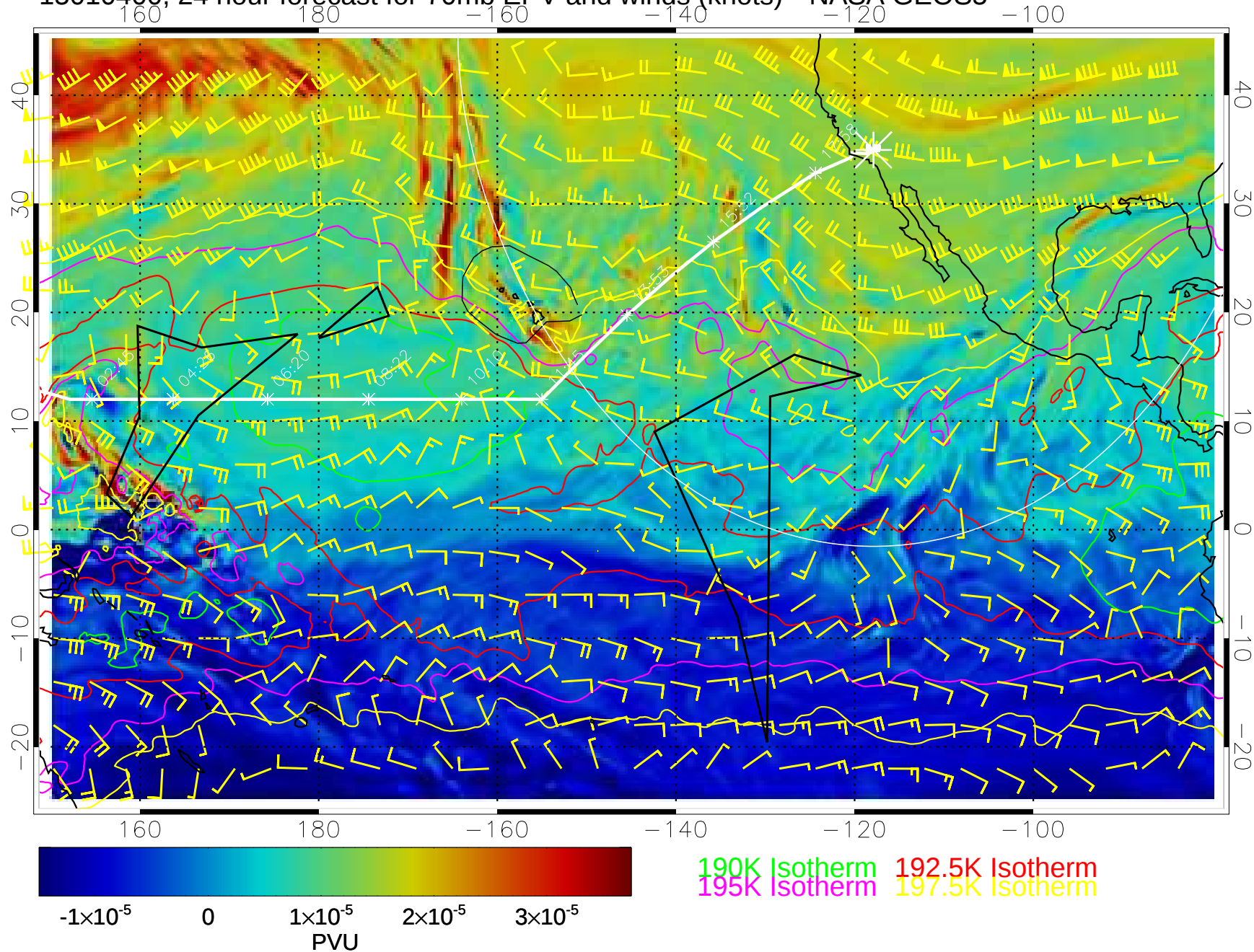
15010400, 24 hour forecast for 70mb EPV and winds (knots)-- NASA GEOS5
