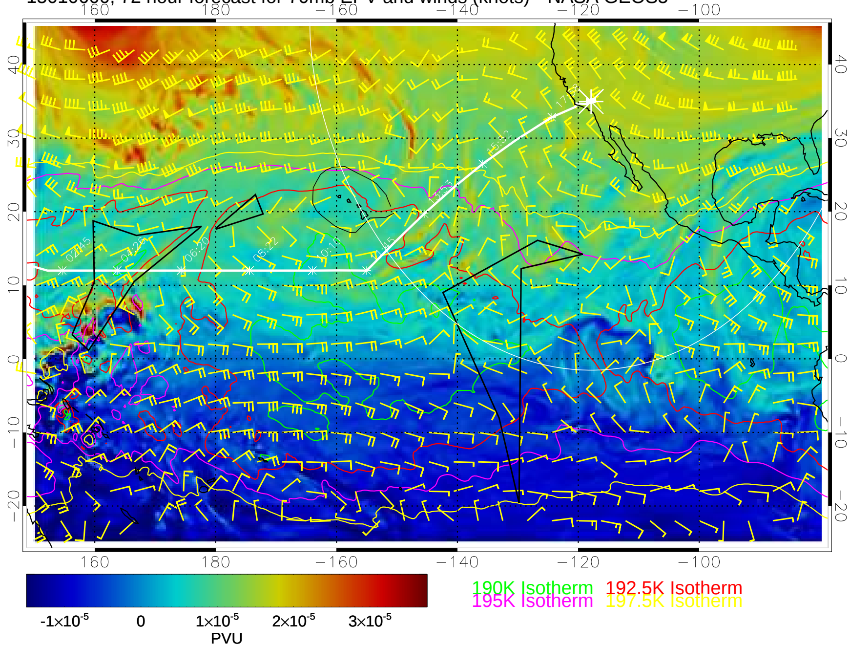
15010600, 72 hour forecast for 70mb EPV and winds (knots)-- NASA GEOS5
