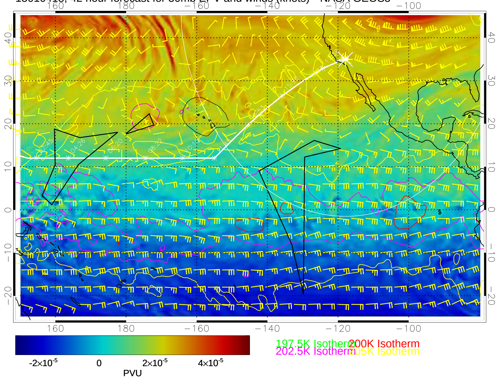
15010418, 42 hour forecast for 50mb EPV and winds (knots)-- NASA GEOS5
