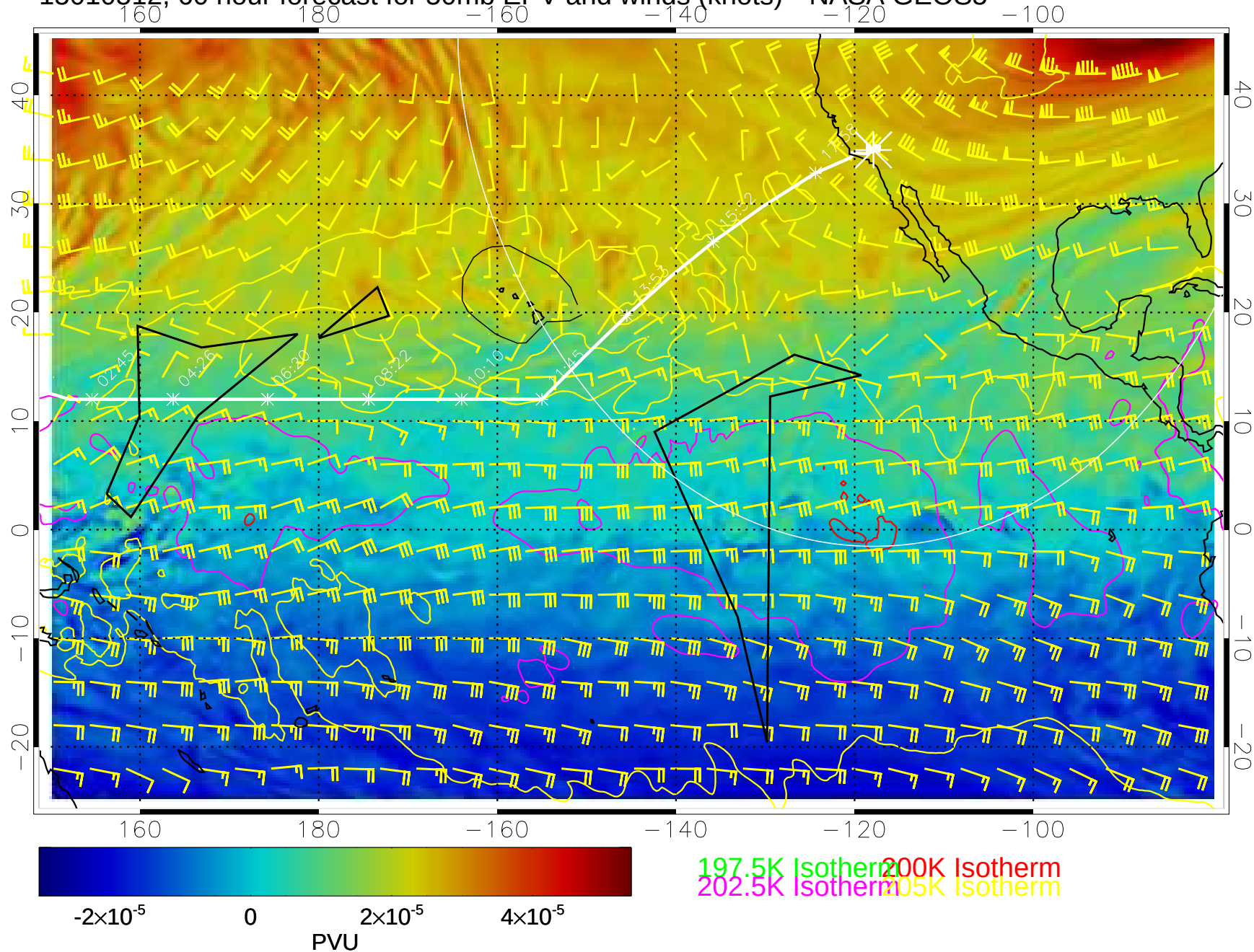
15010512, 60 hour forecast for 50mb EPV and winds (knots)-- NASA GEOS5
