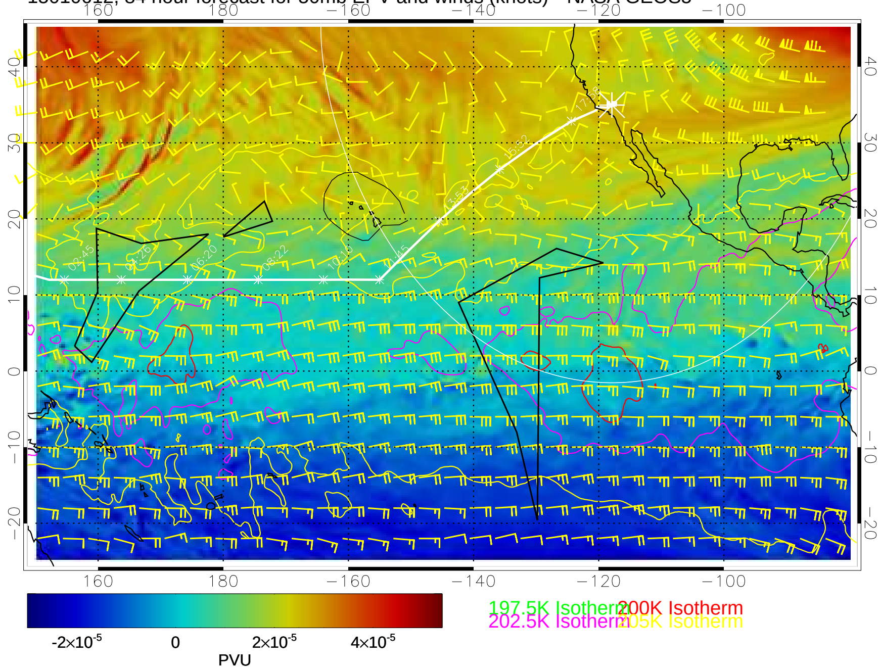
15010612, 84 hour forecast for 50mb EPV and winds (knots)-- NASA GEOS5
