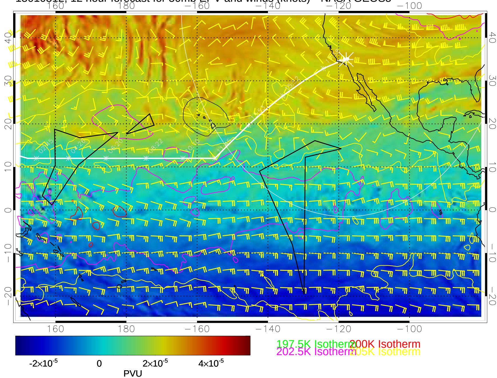
15010312, 12 hour forecast for 50mb EPV and winds (knots)-- NASA GEOS5
