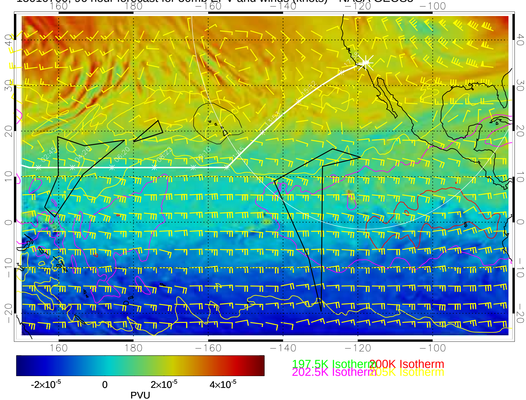
15010700, 96 hour forecast for 50mb EPV and winds (knots)-- NASA GEOS5
