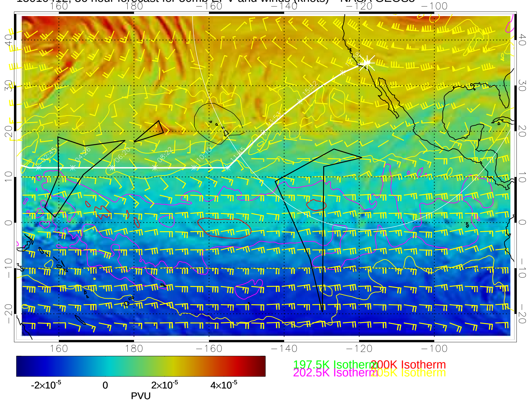
15010412, 36 hour forecast for 50mb EPV and winds (knots)-- NASA GEOS5
