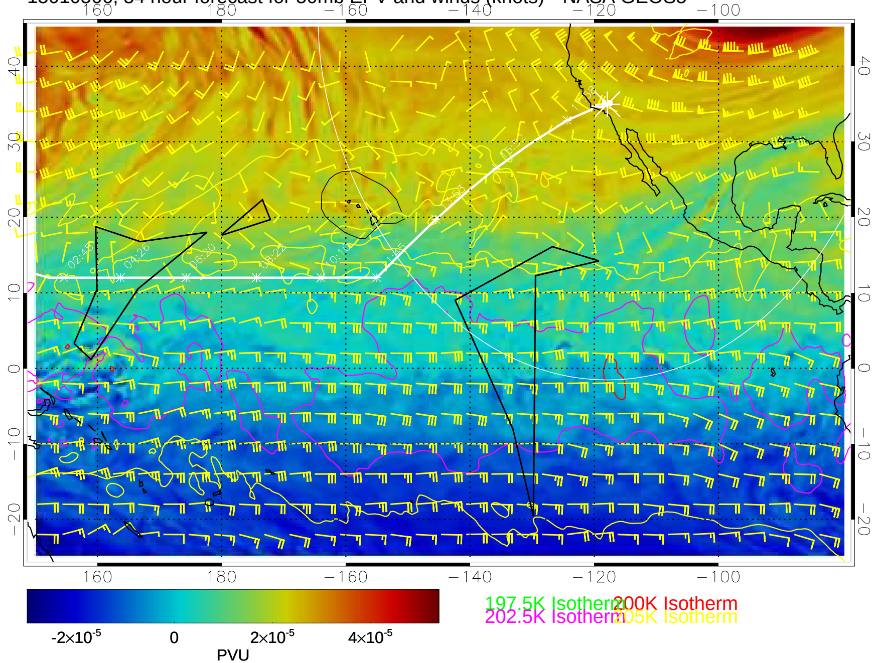
15010506, 54 hour forecast for 50mb EPV and winds (knots)-- NASA GEOS5
