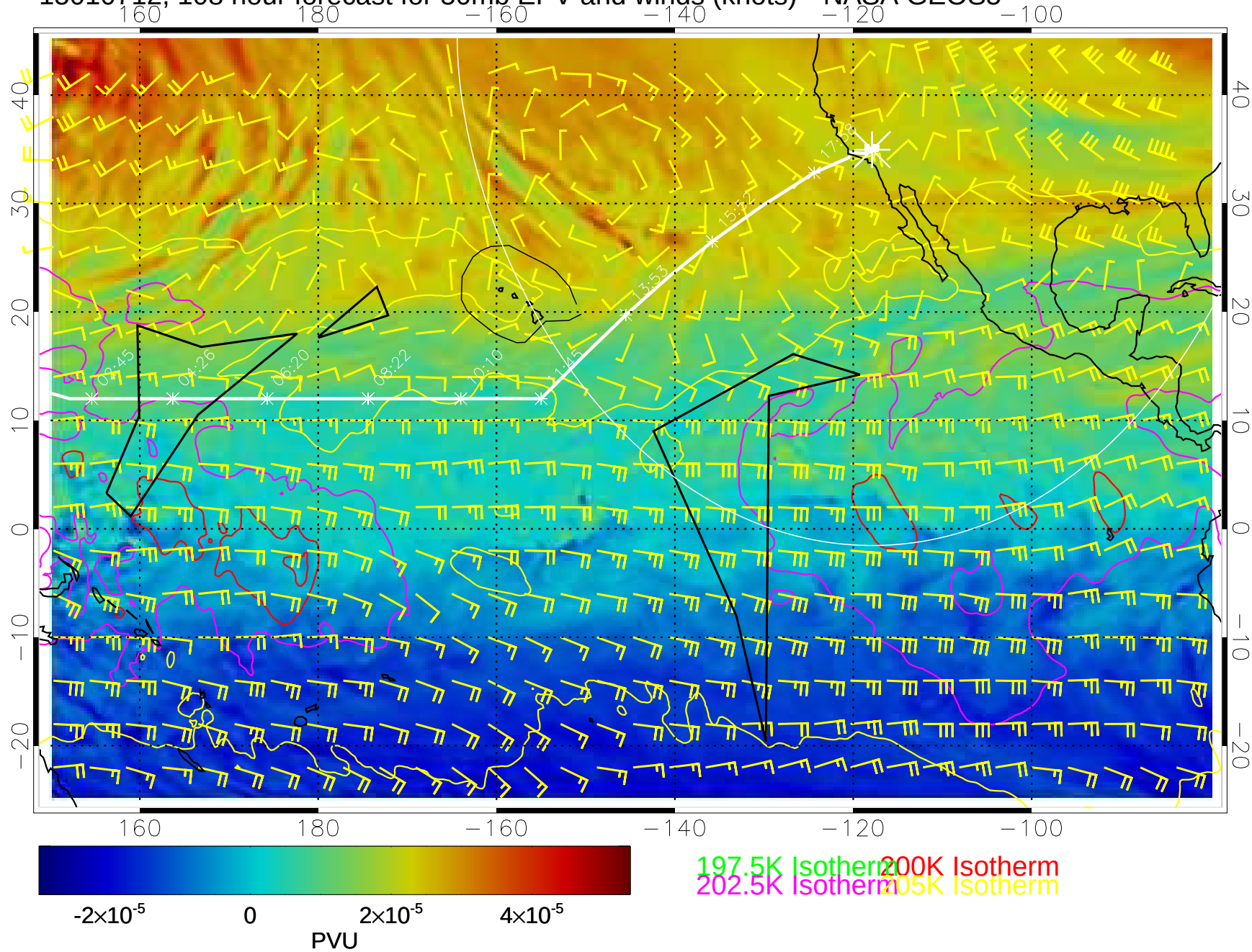
15010712, 108 hour forecast for 50mb EPV and winds (knots)-- NASA GEOS5
