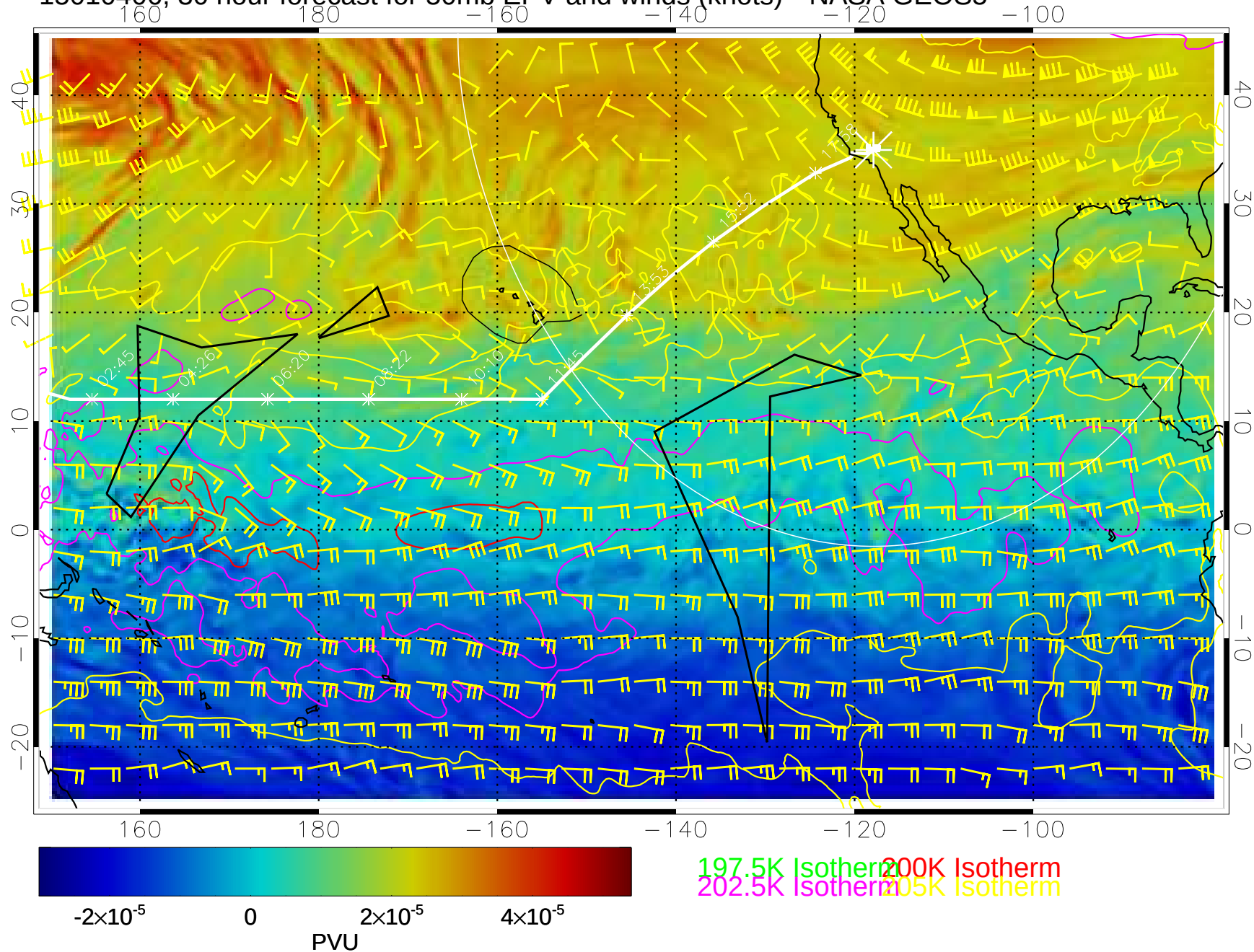
15010406, 30 hour forecast for 50mb EPV and winds (knots)-- NASA GEOS5
