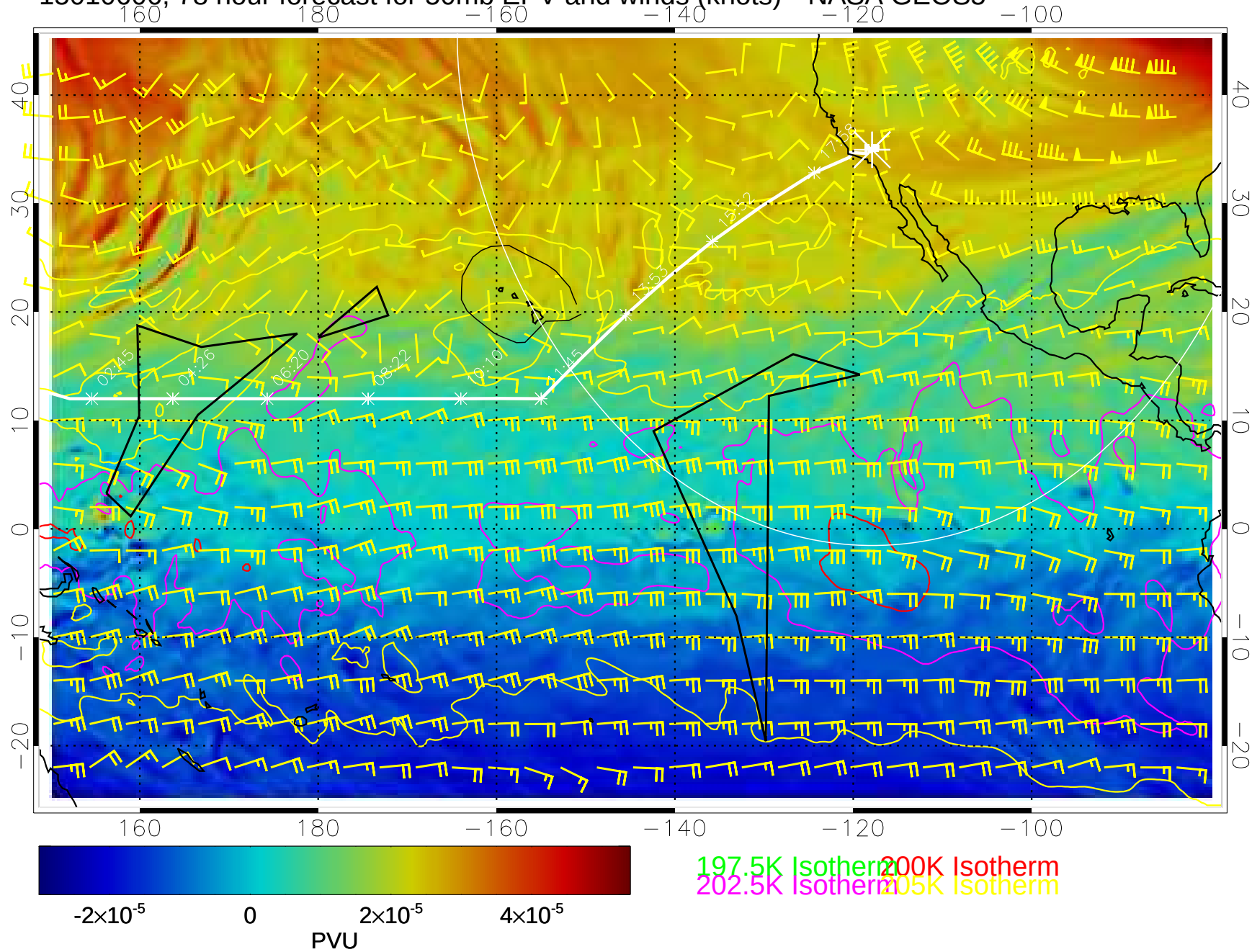
15010606, 78 hour forecast for 50mb EPV and winds (knots)-- NASA GEOS5
