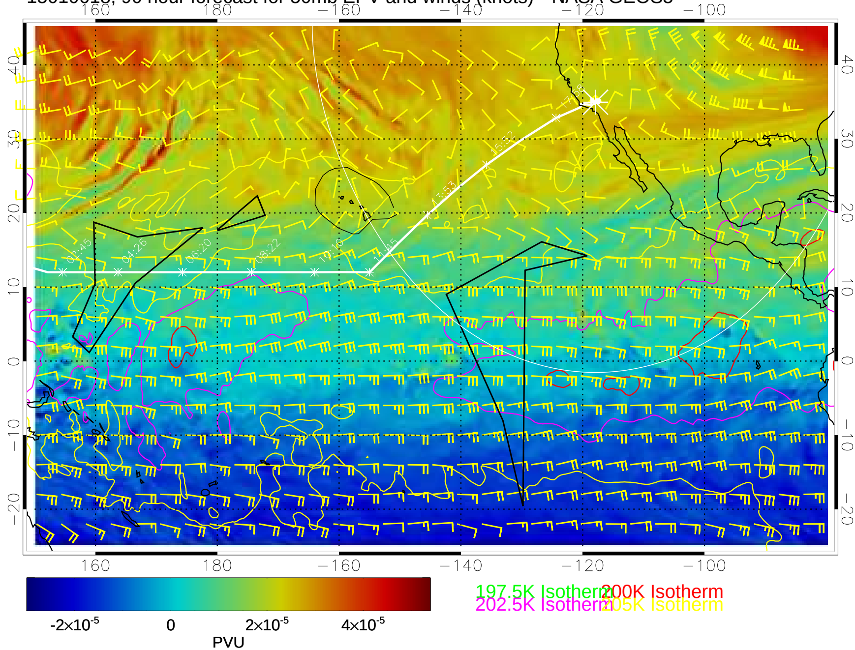
15010618, 90 hour forecast for 50mb EPV and winds (knots)-- NASA GEOS5
