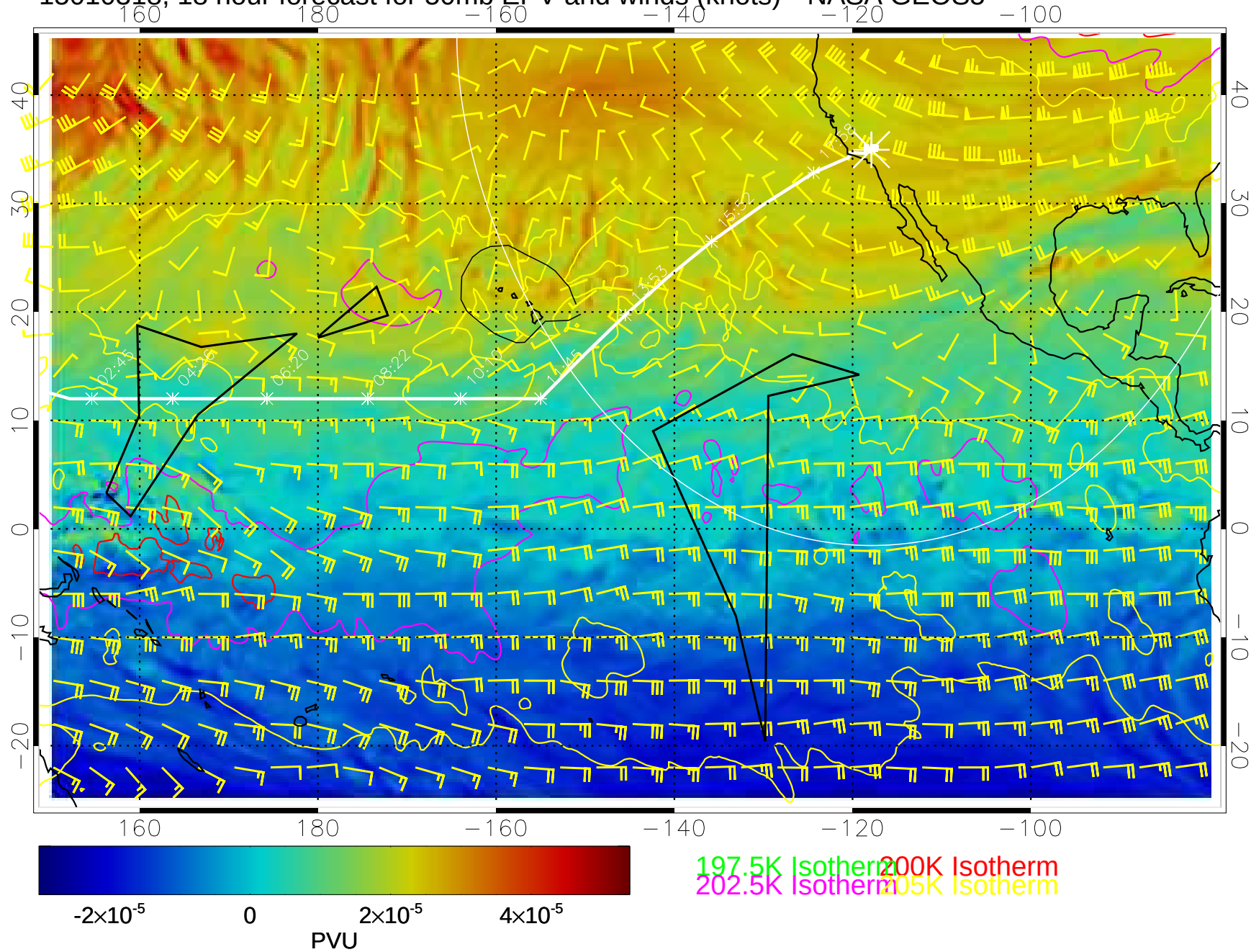
15010318, 18 hour forecast for 50mb EPV and winds (knots)-- NASA GEOS5
