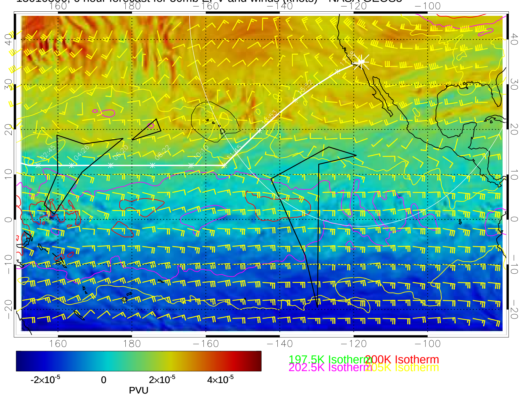
15010306, 6 hour forecast for 50mb EPV and winds (knots)-- NASA GEOS5
