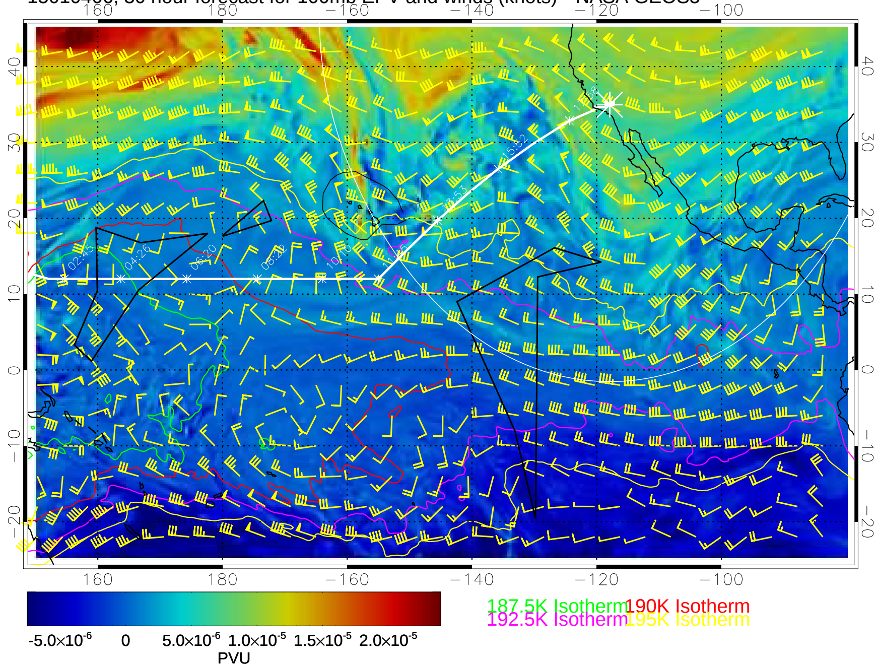
15010406, 30 hour forecast for 100mb EPV and winds (knots)-- NASA GEOS5
