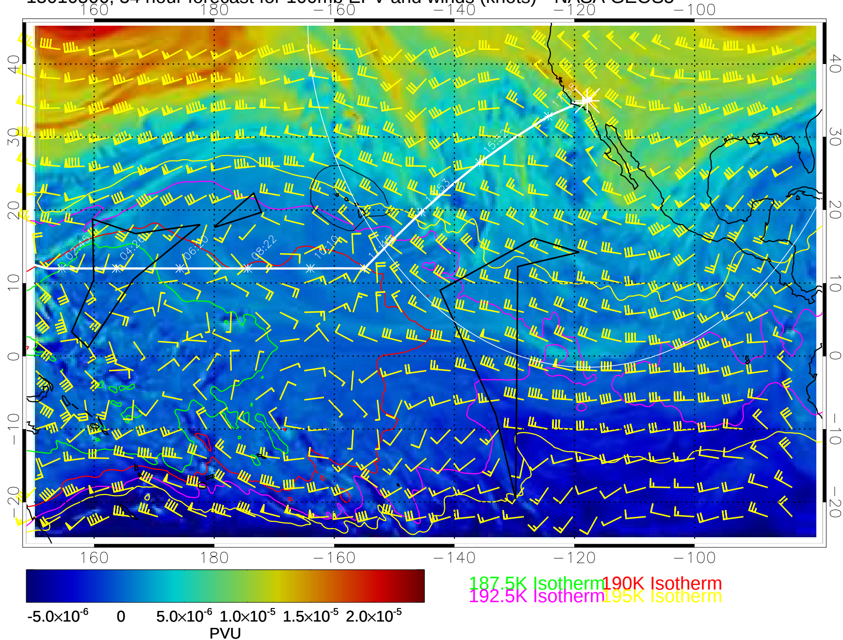
15010506, 54 hour forecast for 100mb EPV and winds (knots)-- NASA GEOS5
