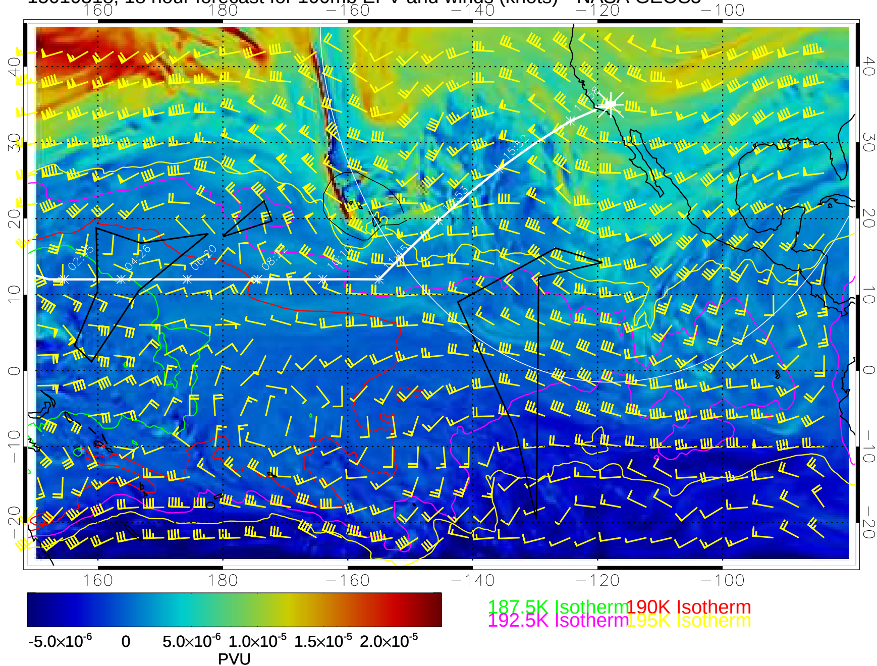
15010318, 18 hour forecast for 100mb EPV and winds (knots)-- NASA GEOS5
