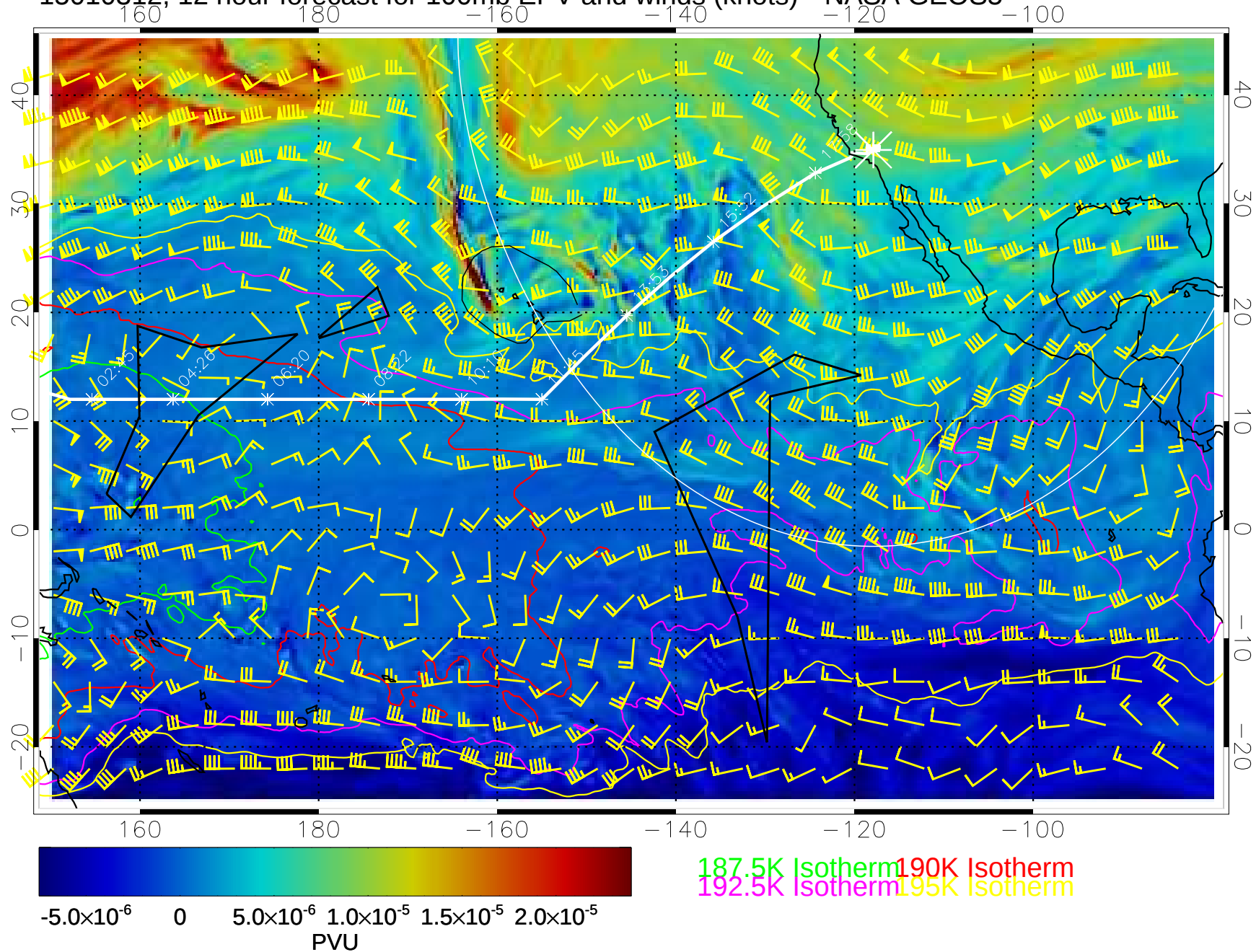
15010312, 12 hour forecast for 100mb EPV and winds (knots)-- NASA GEOS5
