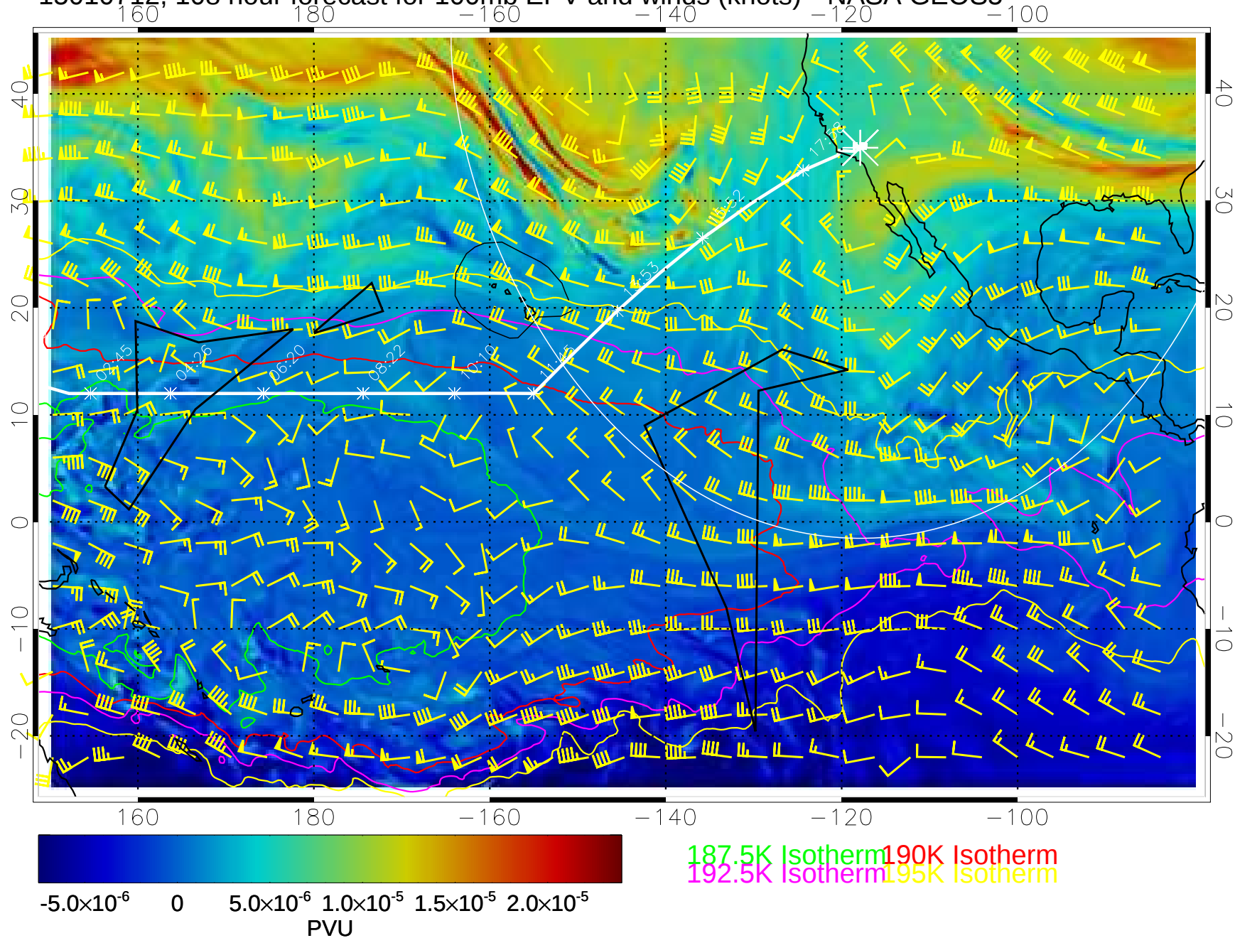
15010712, 108 hour forecast for 100mb EPV and winds (knots)-- NASA GEOS5
