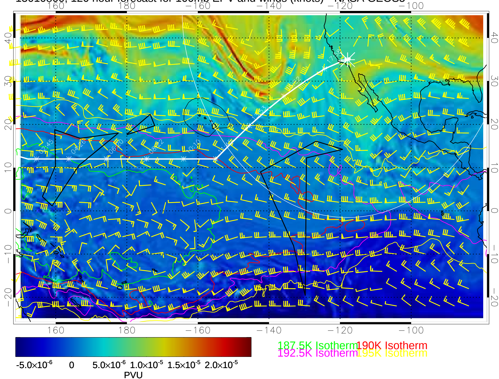
15010800, 120 hour forecast for 100mb EPV and winds (knots)-- NASA GEOS5
