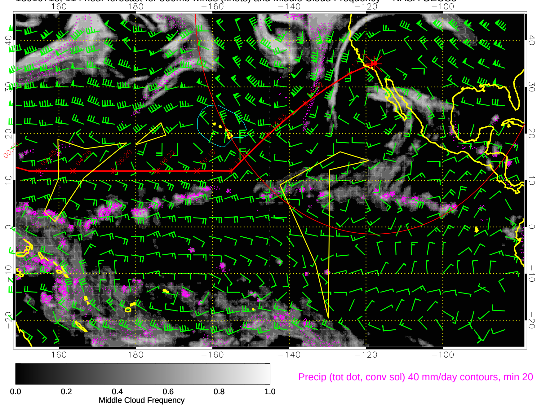
15010718, 114 hour forecast for 500mb winds (knots) and Middle Cloud Frequency -- NASA GEOS5
