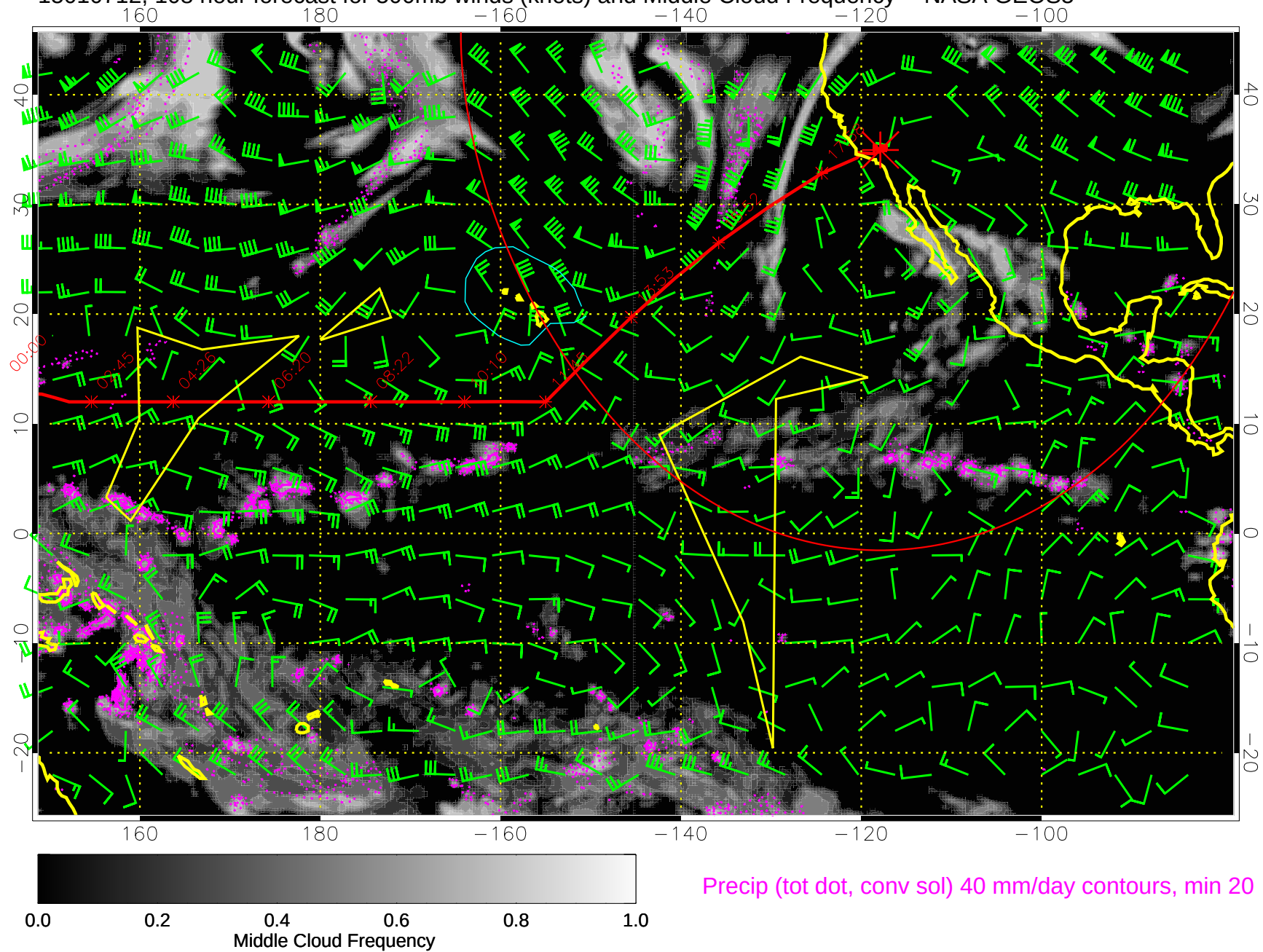
15010712, 108 hour forecast for 500mb winds (knots) and Middle Cloud Frequency -- NASA GEOS5
