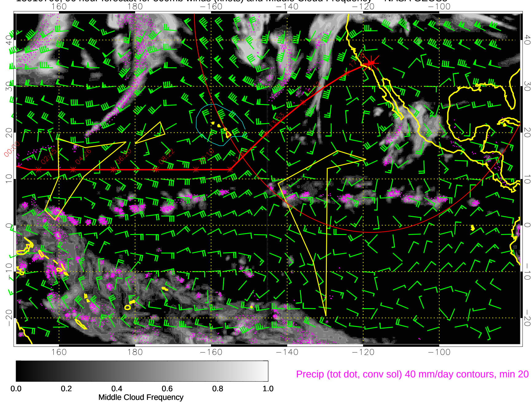
15010700, 96 hour forecast for 500mb winds (knots) and Middle Cloud Frequency -- NASA GEOS5
