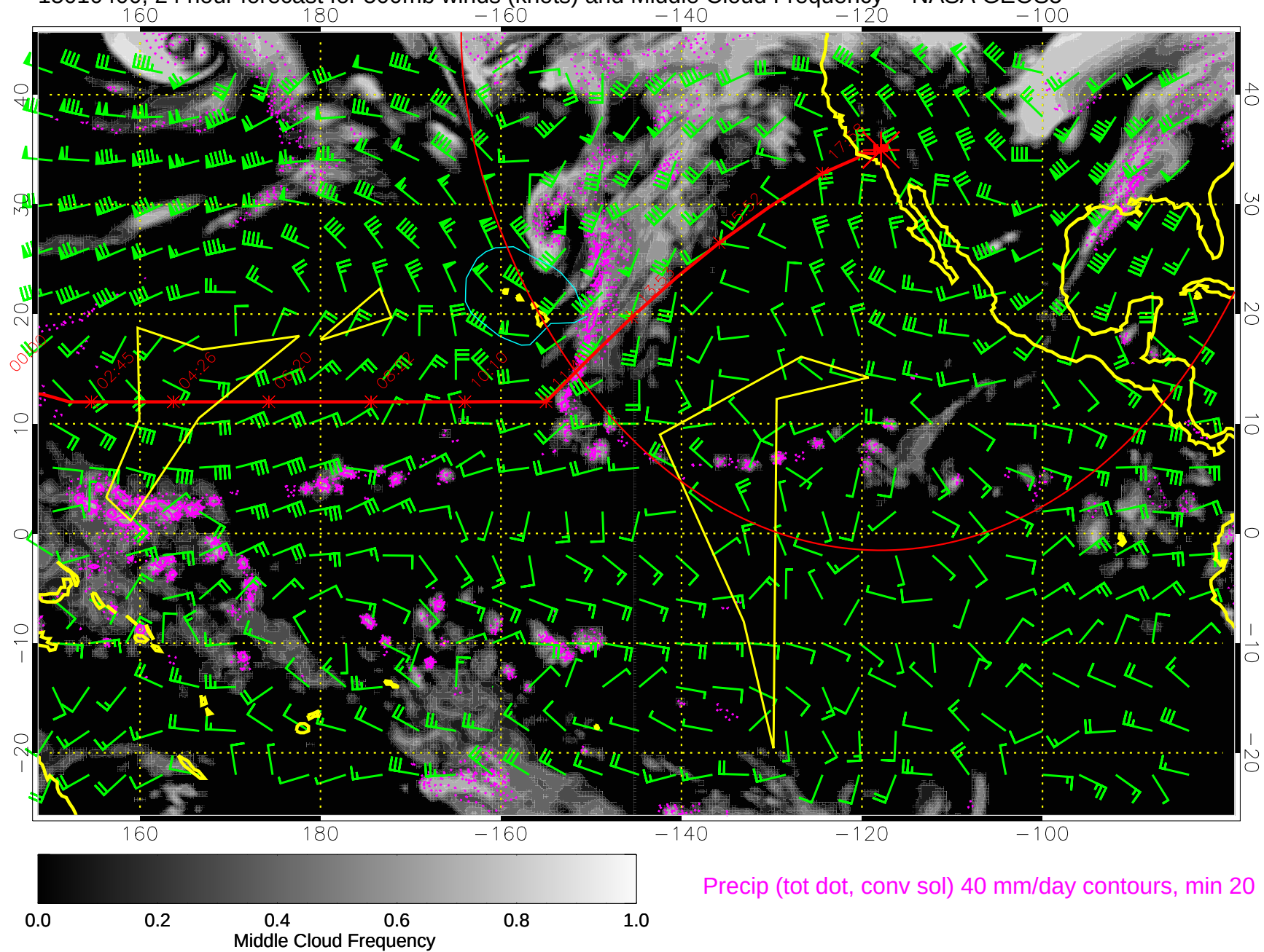
15010400, 24 hour forecast for 500mb winds (knots) and Middle Cloud Frequency -- NASA GEOS5
