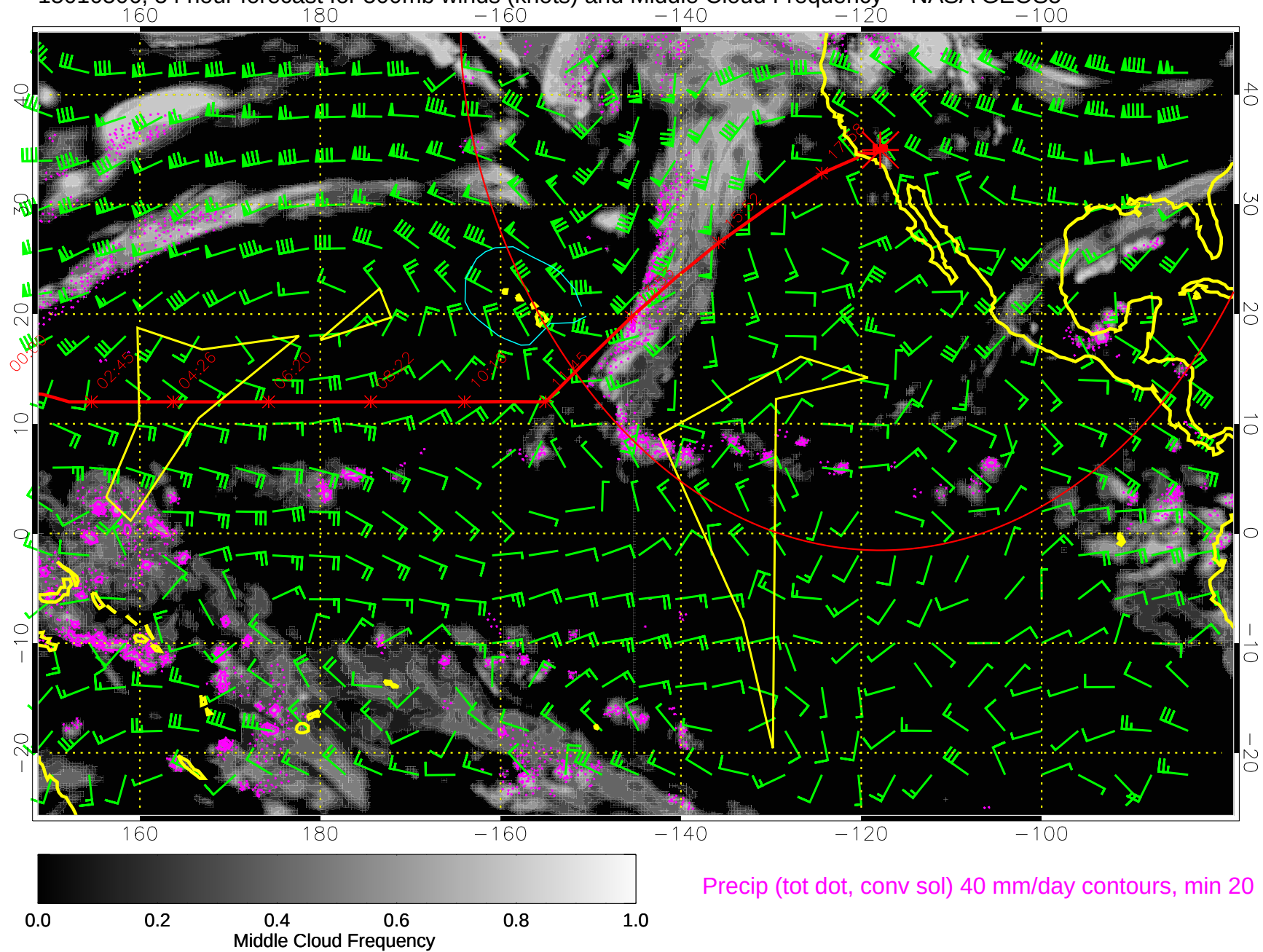
15010506, 54 hour forecast for 500mb winds (knots) and Middle Cloud Frequency -- NASA GEOS5
