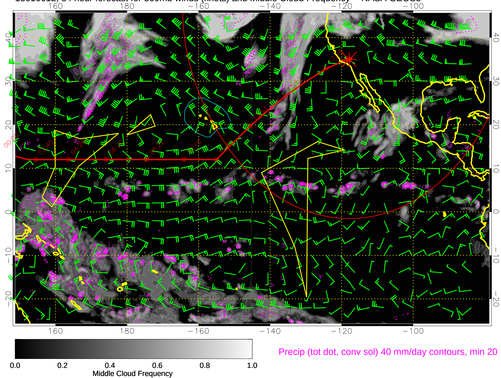
15010612, 84 hour forecast for 500mb winds (knots) and Middle Cloud Frequency -- NASA GEOS5
