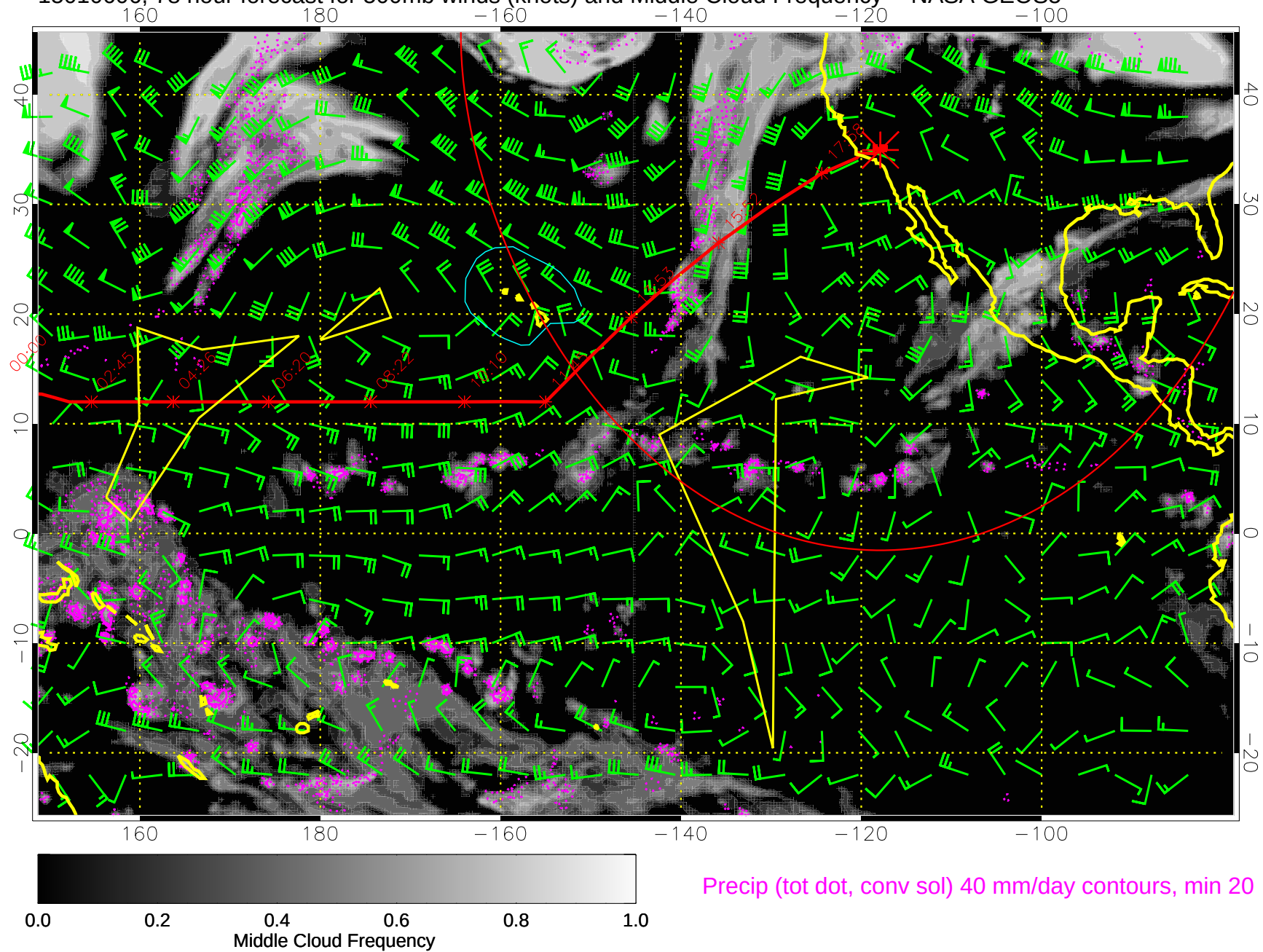
15010606, 78 hour forecast for 500mb winds (knots) and Middle Cloud Frequency -- NASA GEOS5
