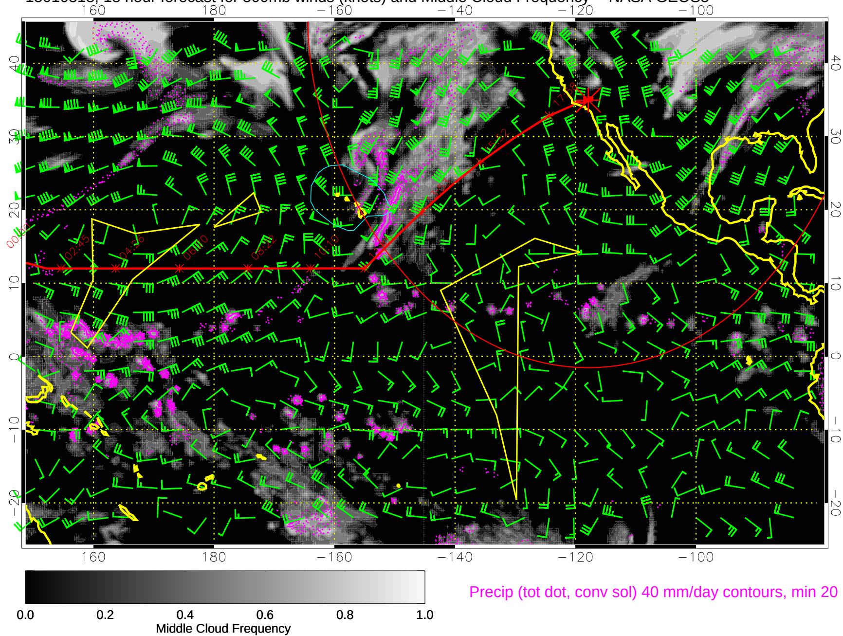
15010318, 18 hour forecast for 500mb winds (knots) and Middle Cloud Frequency -- NASA GEOS5
