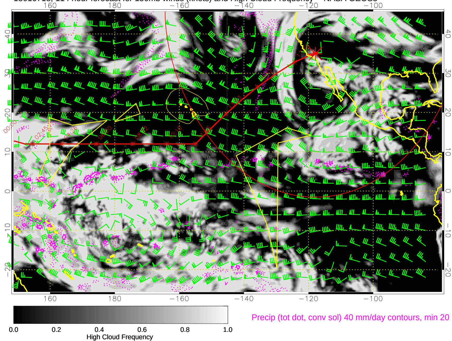
15010718, 114 hour forecast for 150mb winds (knots) and High Cloud Frequency -- NASA GEOS5
