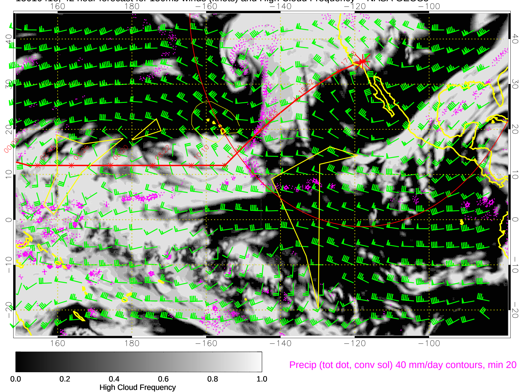
15010418, 42 hour forecast for 150mb winds (knots) and High Cloud Frequency -- NASA GEOS5
