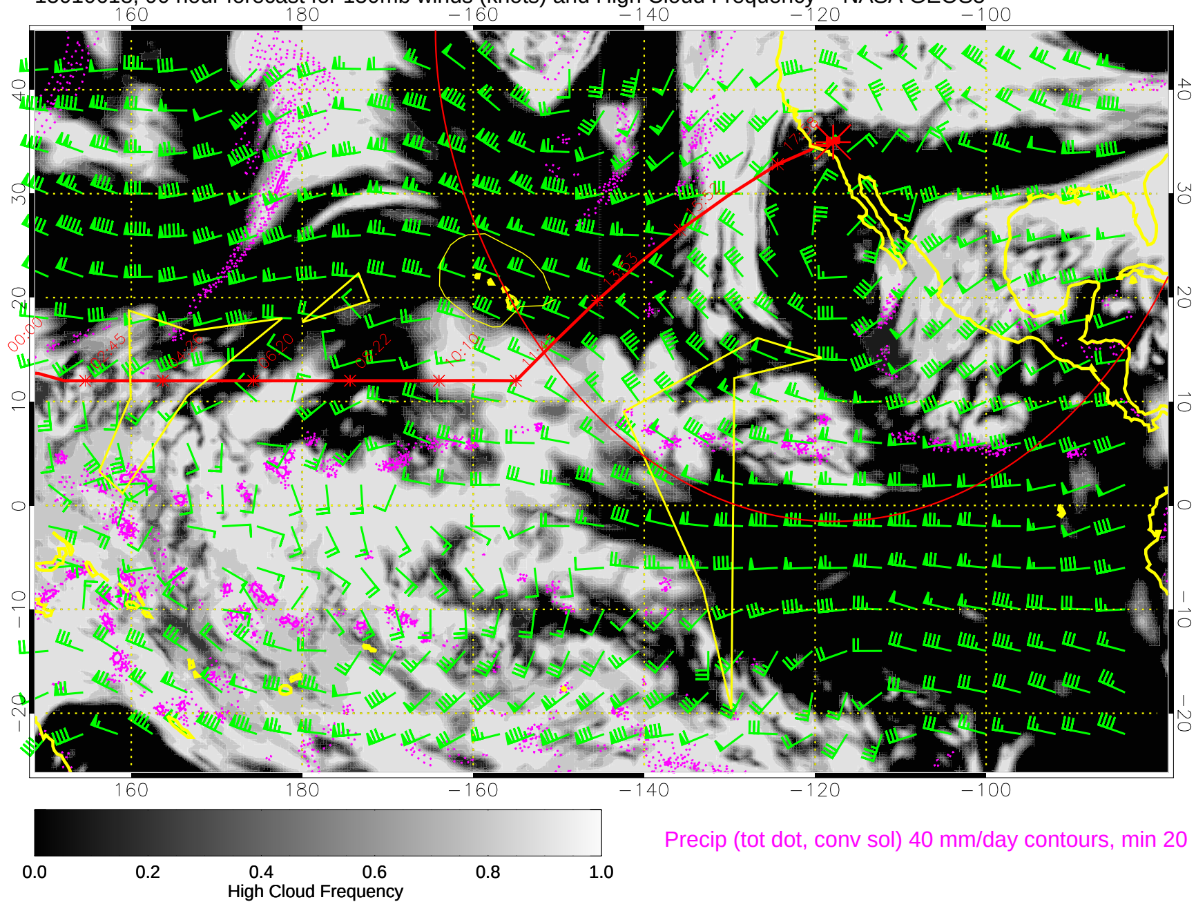
15010618, 90 hour forecast for 150mb winds (knots) and High Cloud Frequency -- NASA GEOS5
