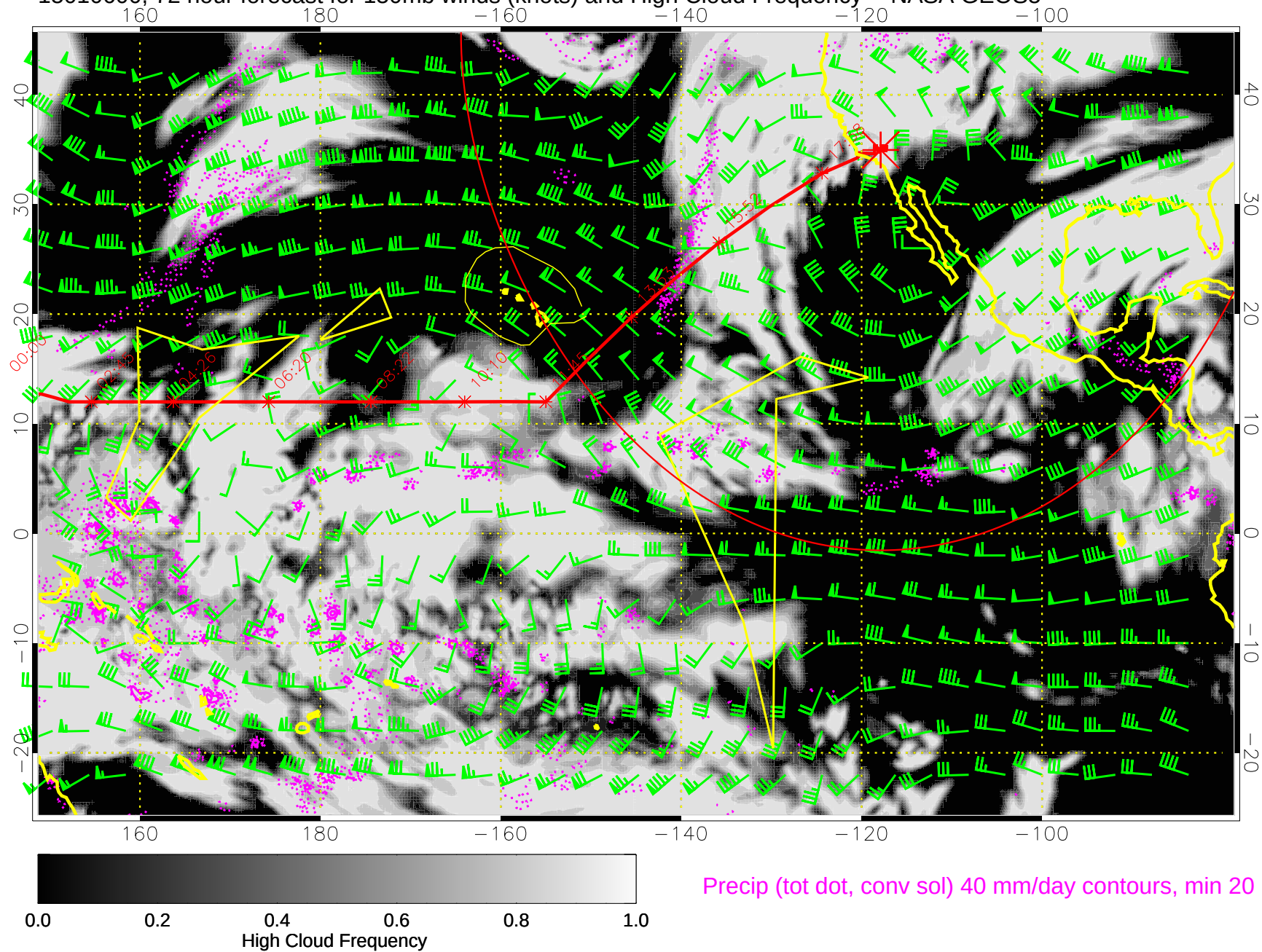
15010600, 72 hour forecast for 150mb winds (knots) and High Cloud Frequency -- NASA GEOS5
