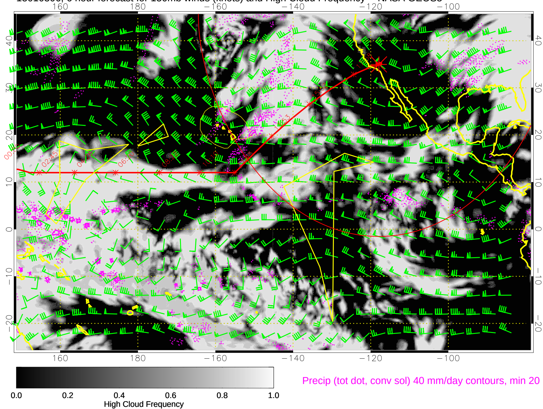
15010306, 6 hour forecast for 150mb winds (knots) and High Cloud Frequency -- NASA GEOS5
