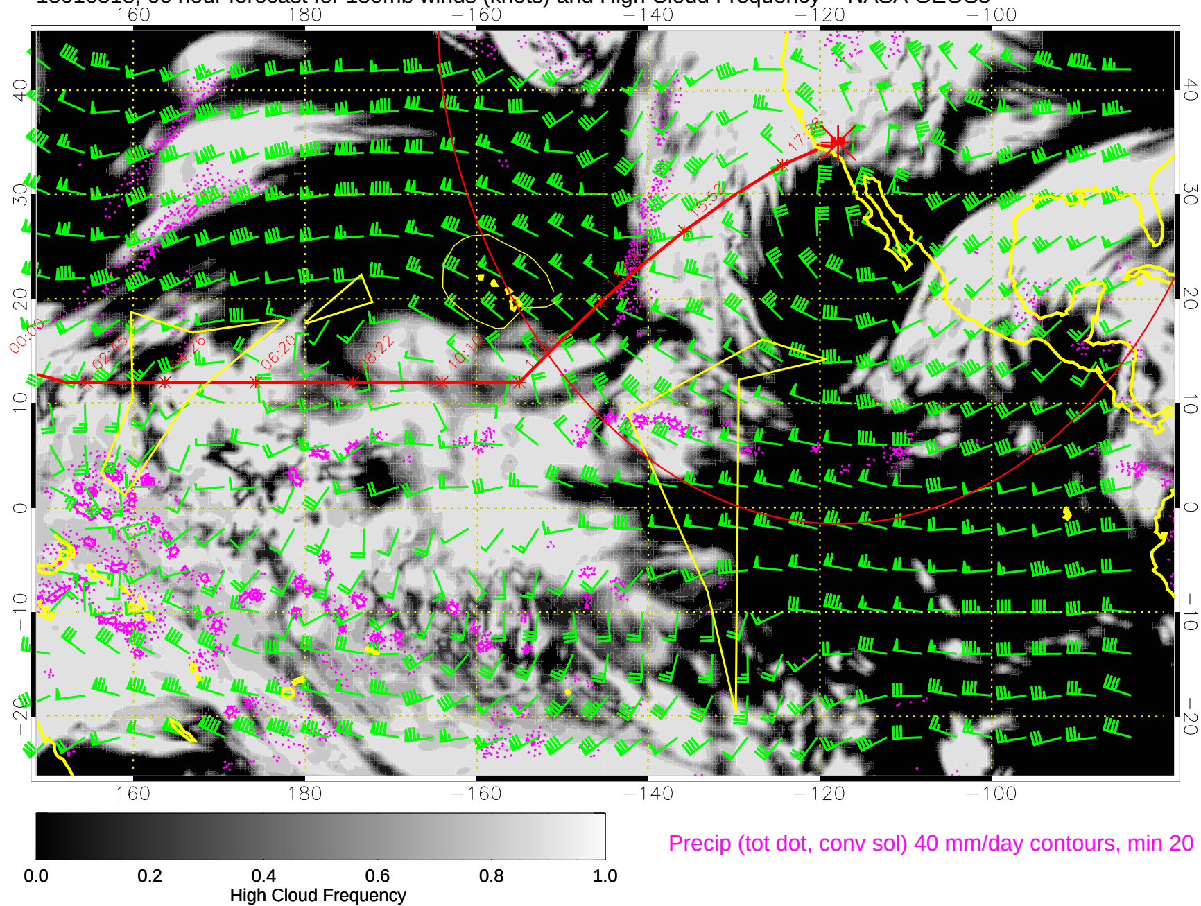
15010518, 66 hour forecast for 150mb winds (knots) and High Cloud Frequency -- NASA GEOS5
