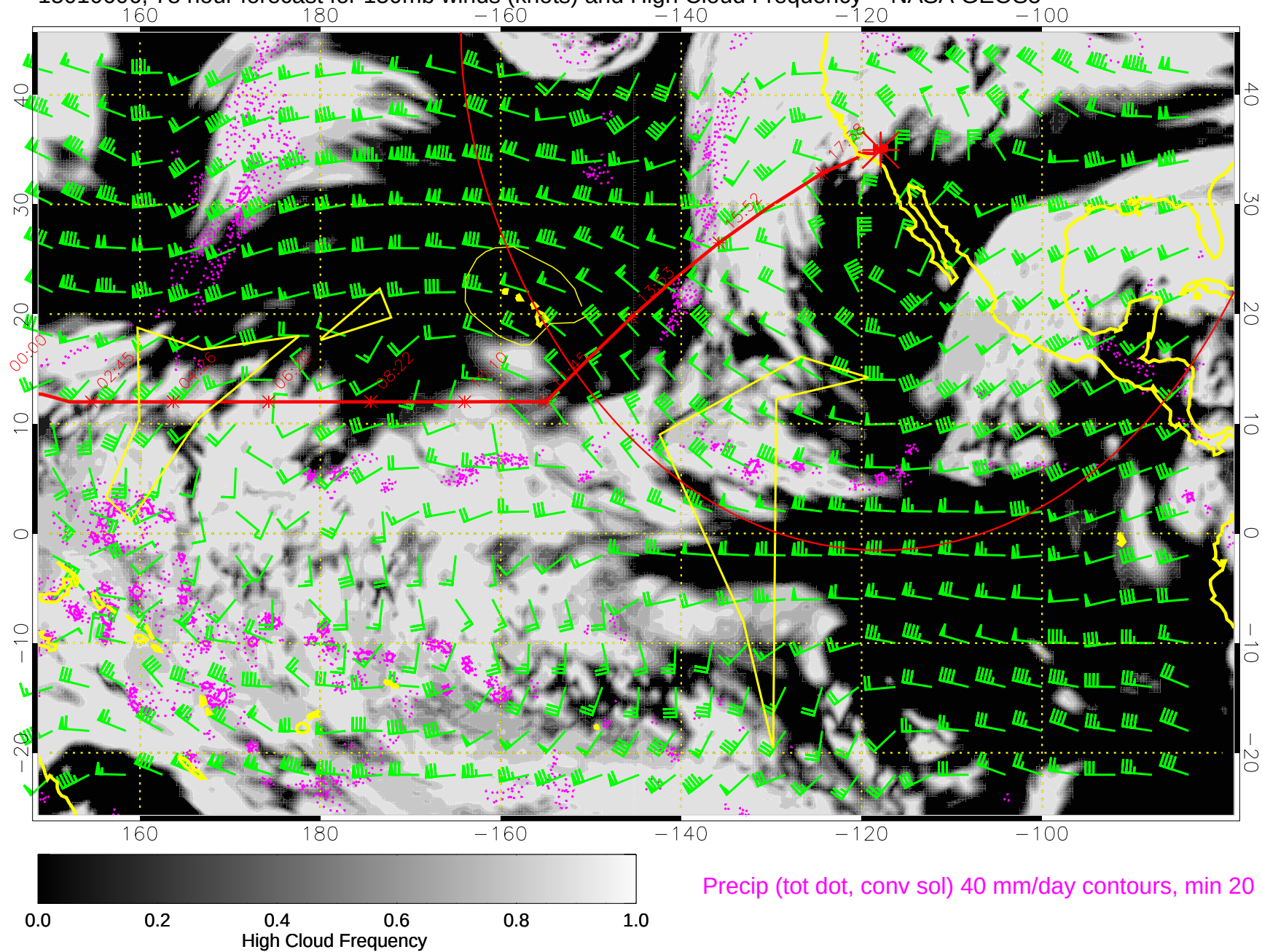
15010606, 78 hour forecast for 150mb winds (knots) and High Cloud Frequency -- NASA GEOS5
