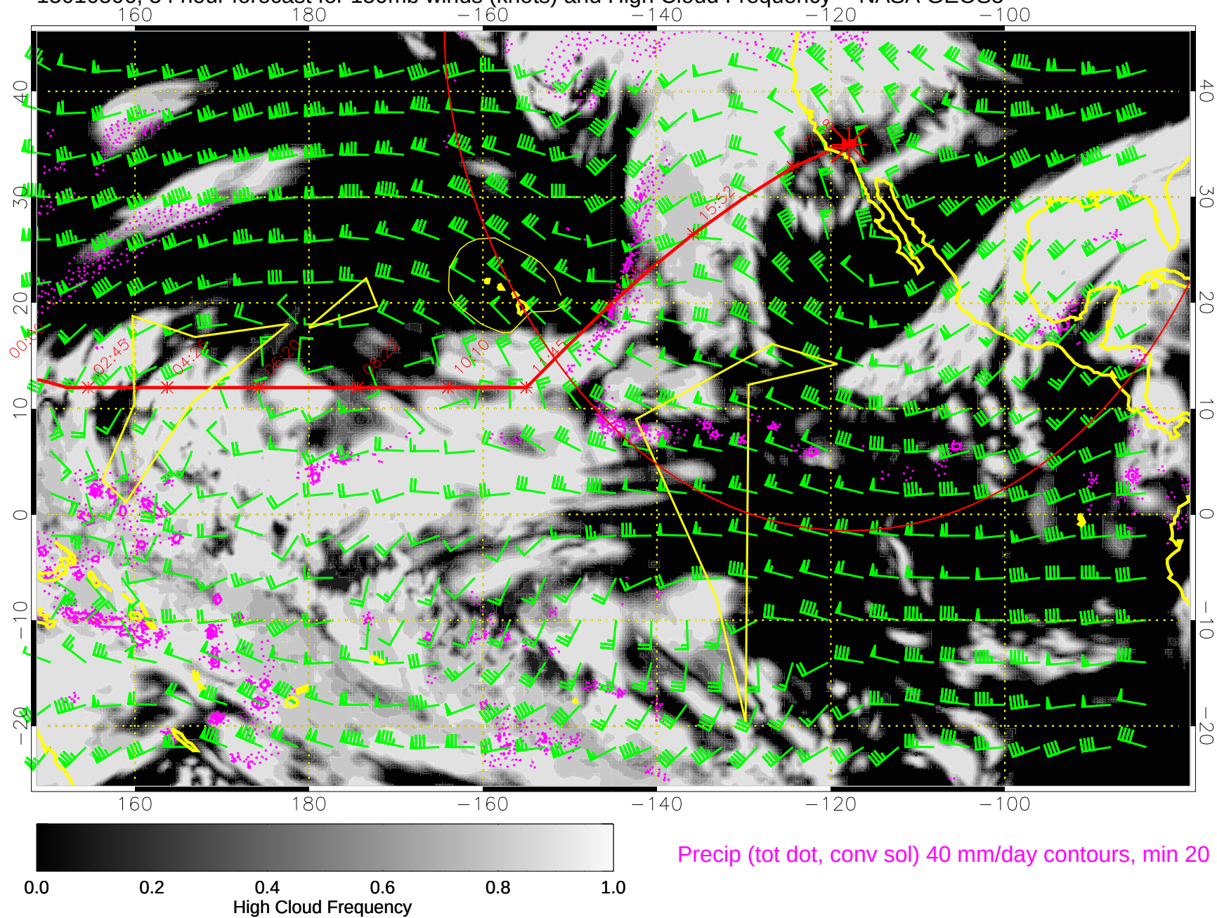
15010506, 54 hour forecast for 150mb winds (knots) and High Cloud Frequency -- NASA GEOS5
