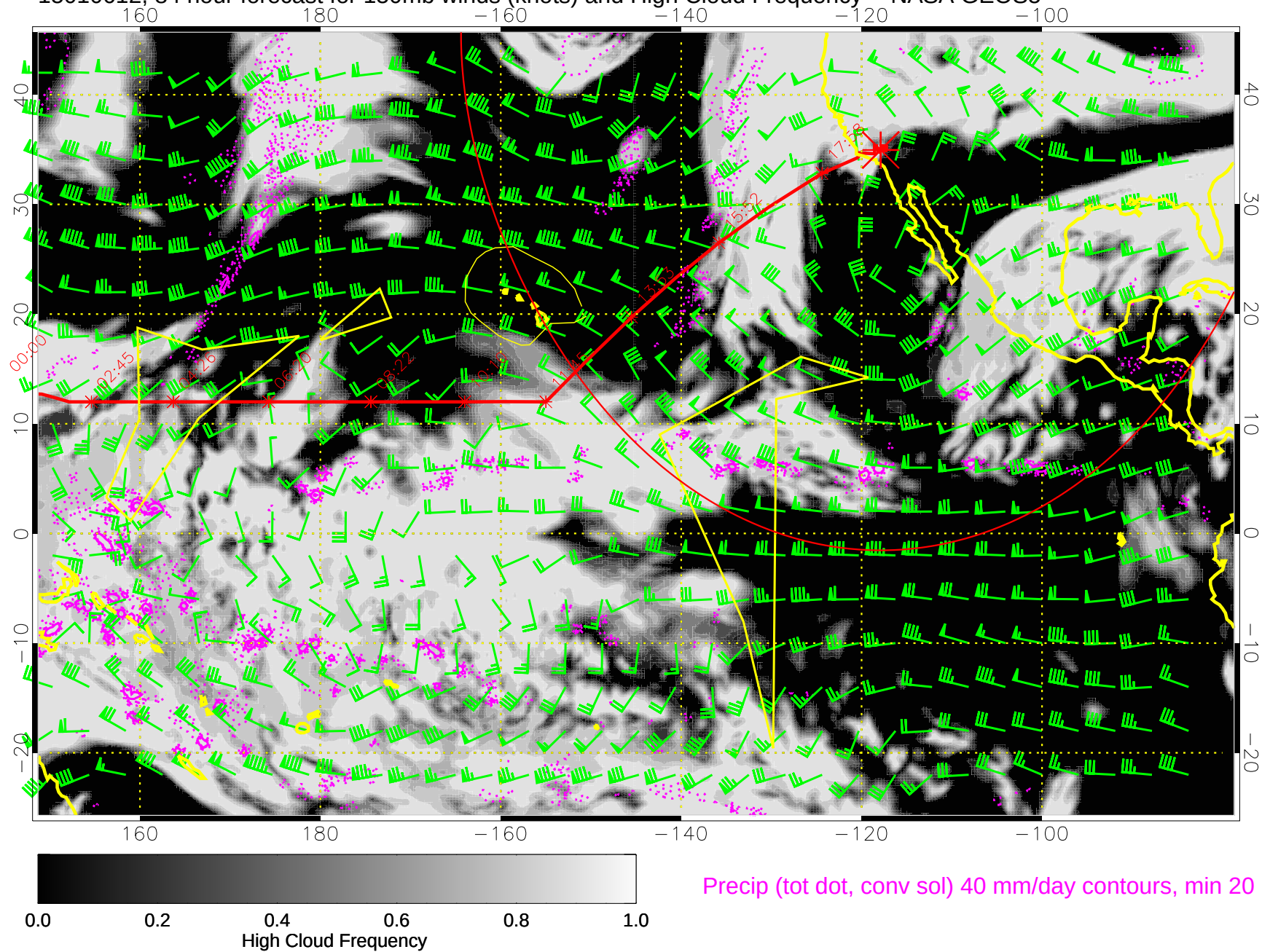
15010612, 84 hour forecast for 150mb winds (knots) and High Cloud Frequency -- NASA GEOS5
