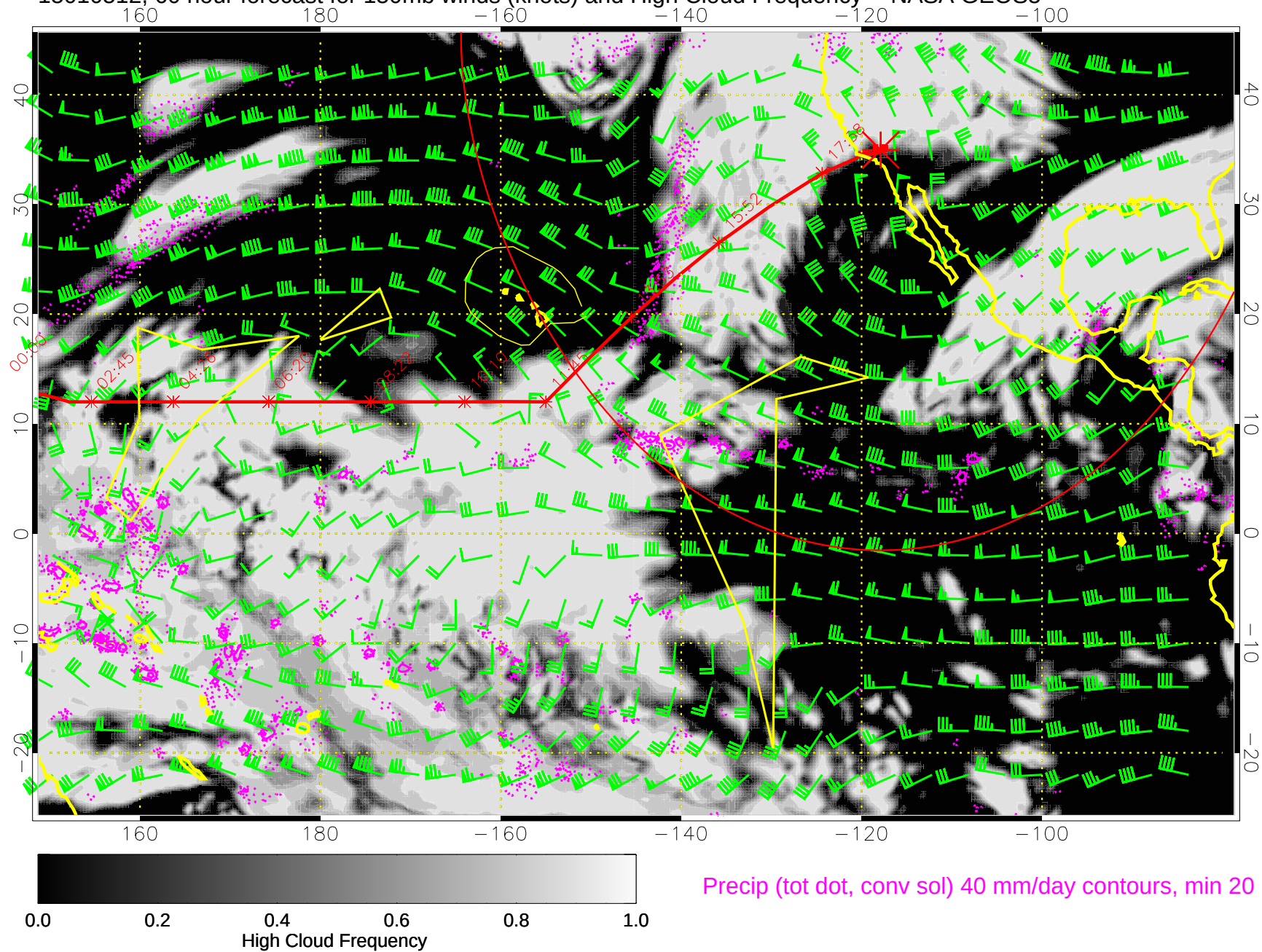
15010512, 60 hour forecast for 150mb winds (knots) and High Cloud Frequency -- NASA GEOS5
