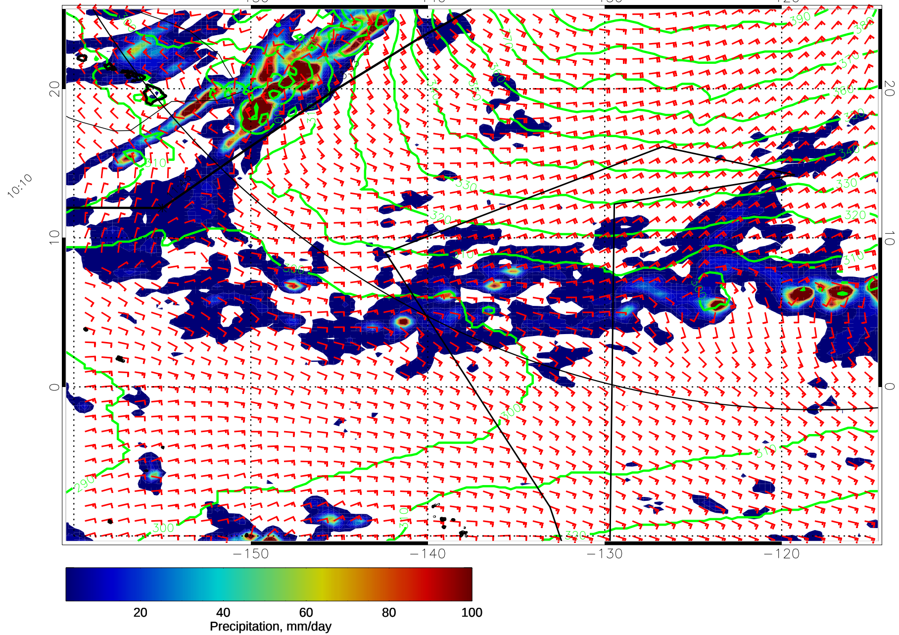
15010306, 54 hour forecast for 975mb Z, Precip., and Surface Winds (knots) -- NASA GEOS5
