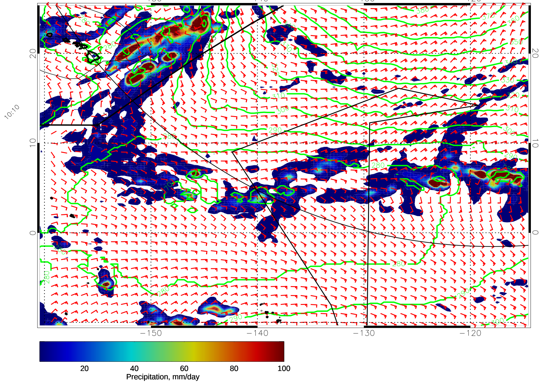
15010300, 48 hour forecast for 975mb Z, Precip., and Surface Winds (knots) -- NASA GEOS5
