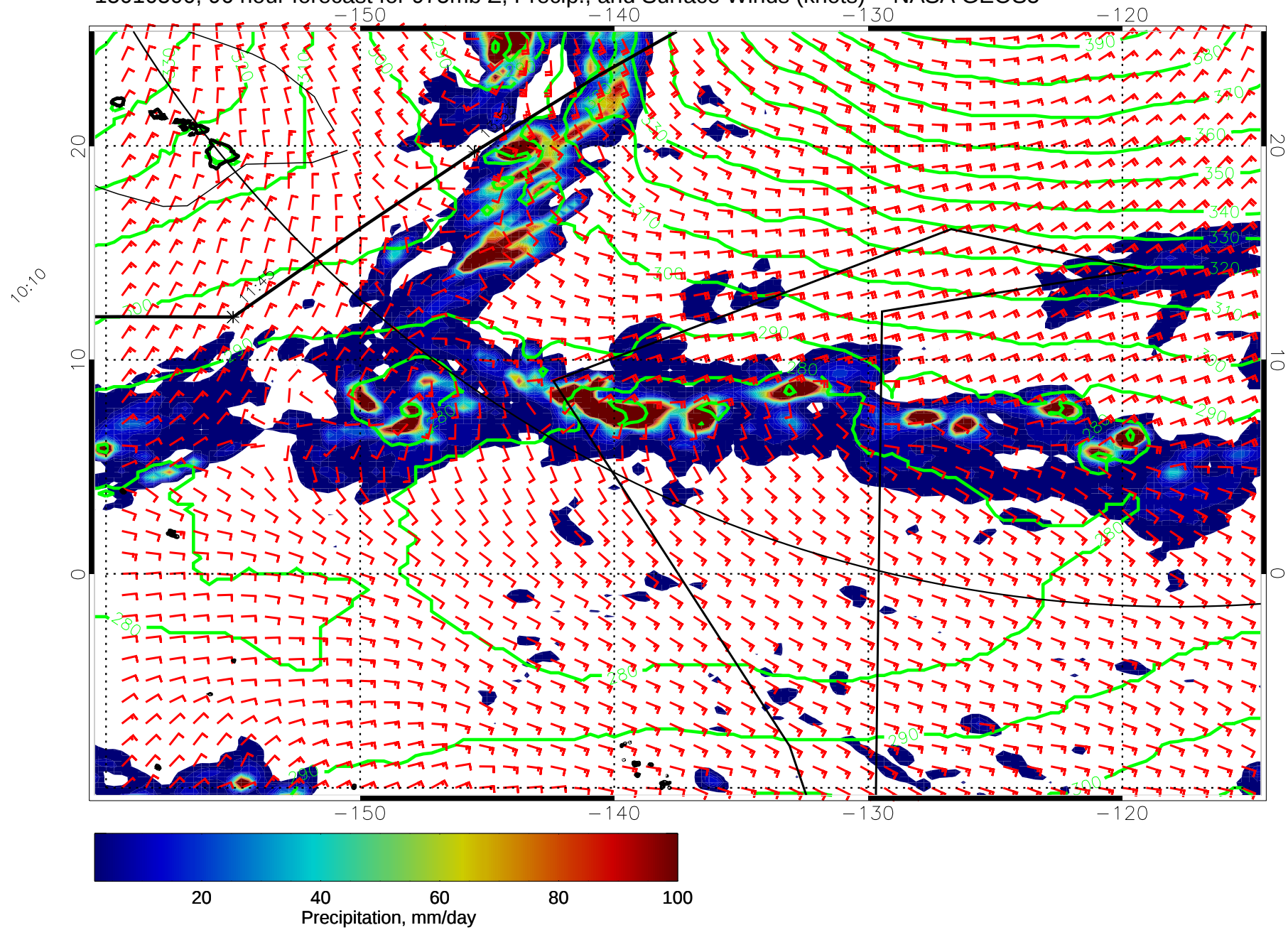
15010500, 96 hour forecast for 975mb Z, Precip., and Surface Winds (knots) -- NASA GEOS5
