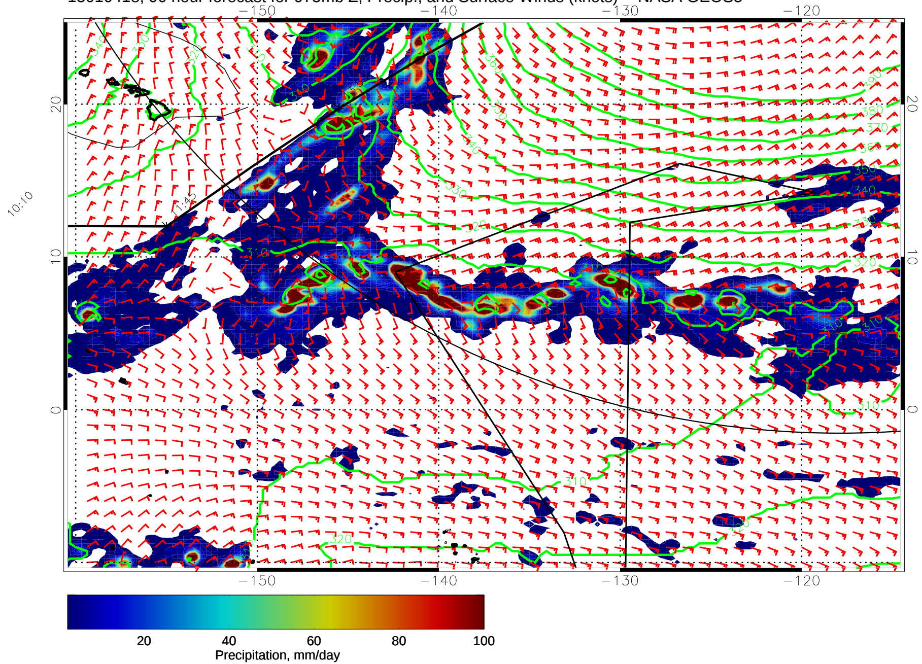
15010418, 90 hour forecast for 975mb Z, Precip., and Surface Winds (knots) -- NASA GEOS5
