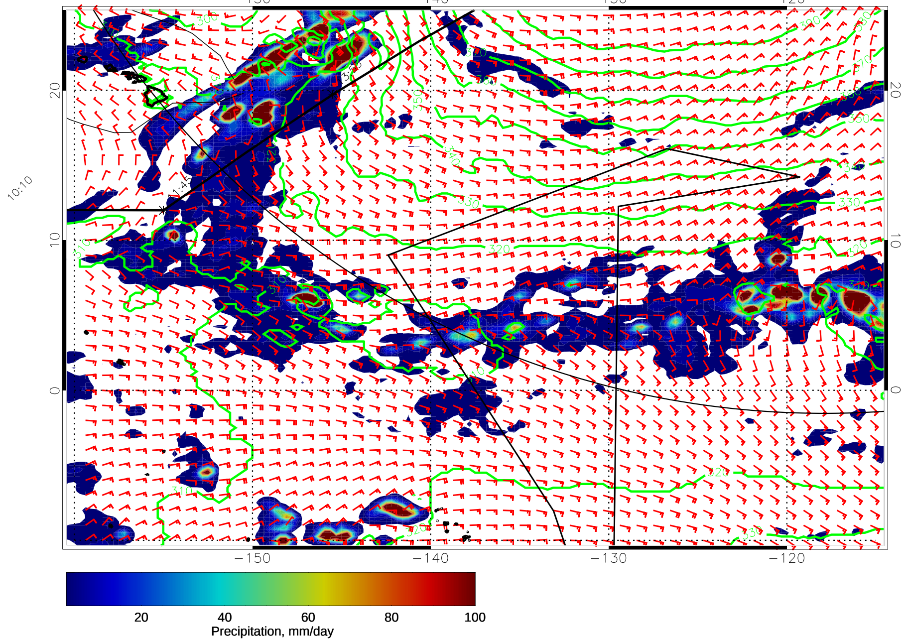
15010218, 42 hour forecast for 975mb Z, Precip., and Surface Winds (knots) -- NASA GEOS5
