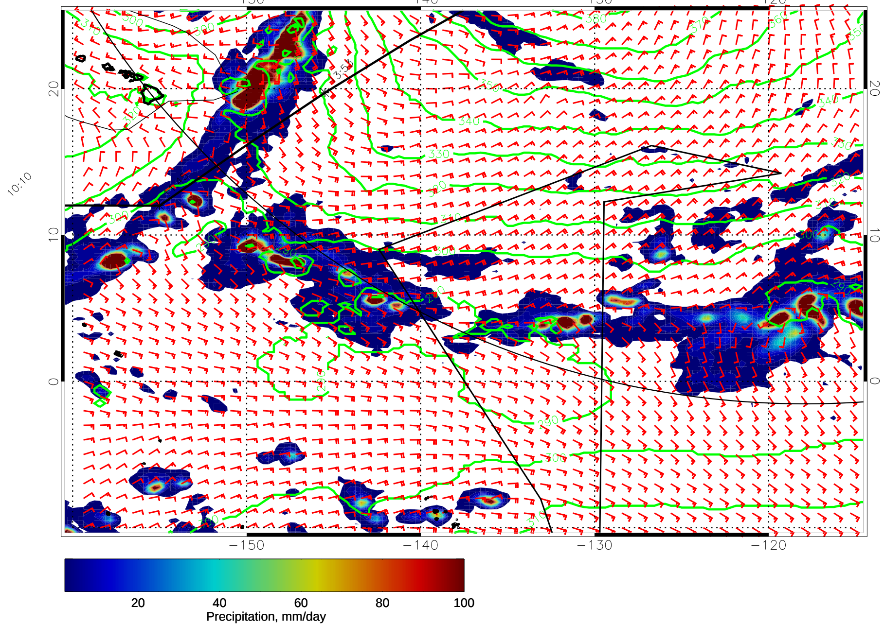
15010200, 24 hour forecast for 975mb Z, Precip., and Surface Winds (knots) -- NASA GEOS5
