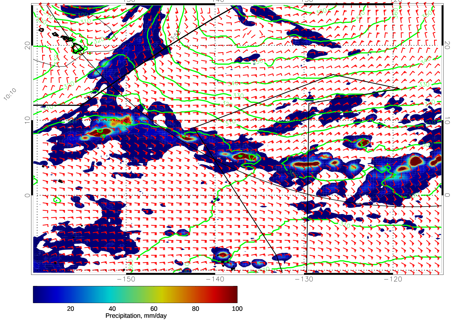
15010112, 12 hour forecast for 975mb Z, Precip., and Surface Winds (knots) -- NASA GEOS5
