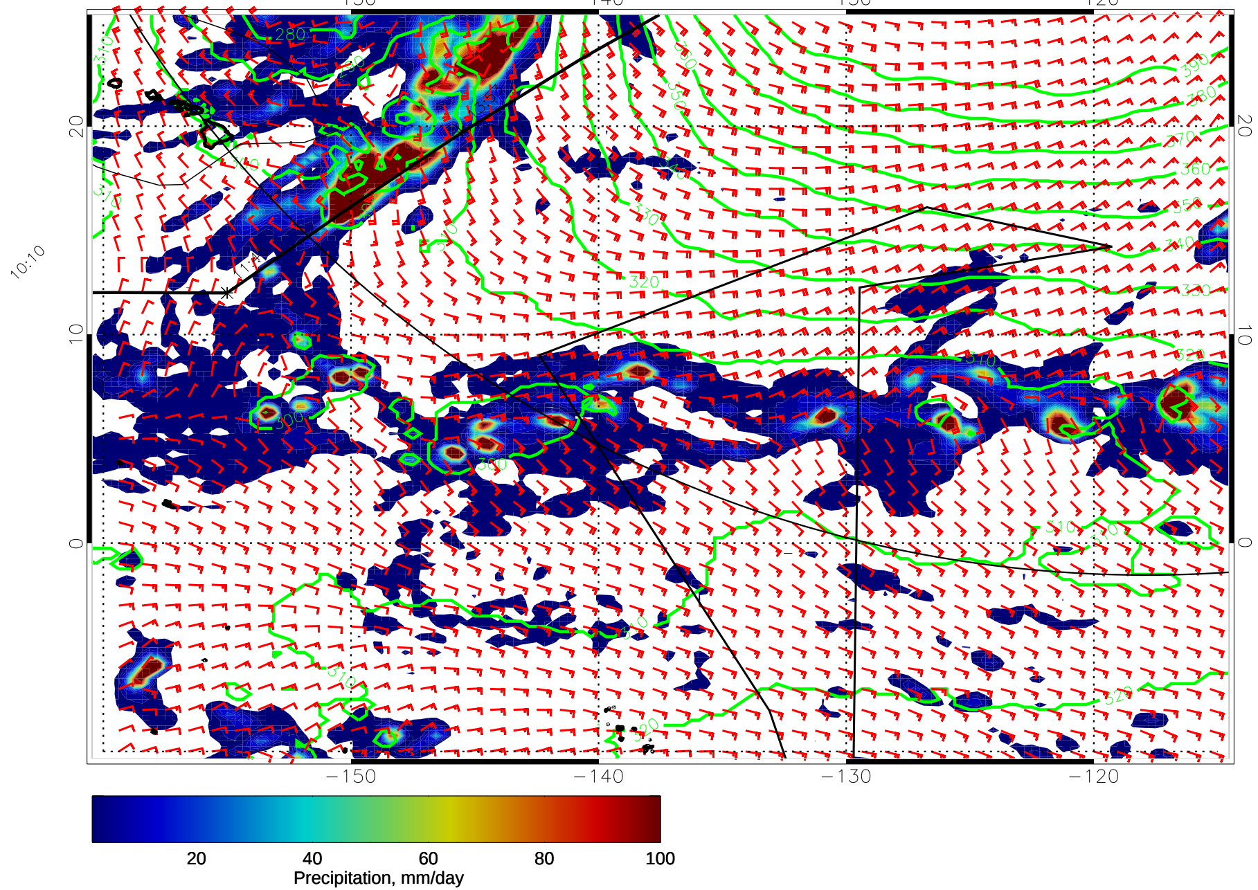
15010318, 66 hour forecast for 975mb Z, Precip., and Surface Winds (knots) -- NASA GEOS5
