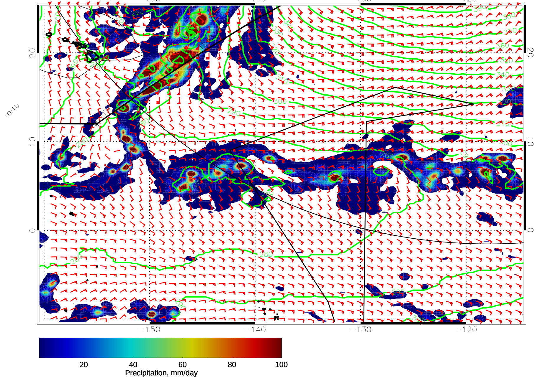
15010400, 72 hour forecast for 975mb Z, Precip., and Surface Winds (knots) -- NASA GEOS5
