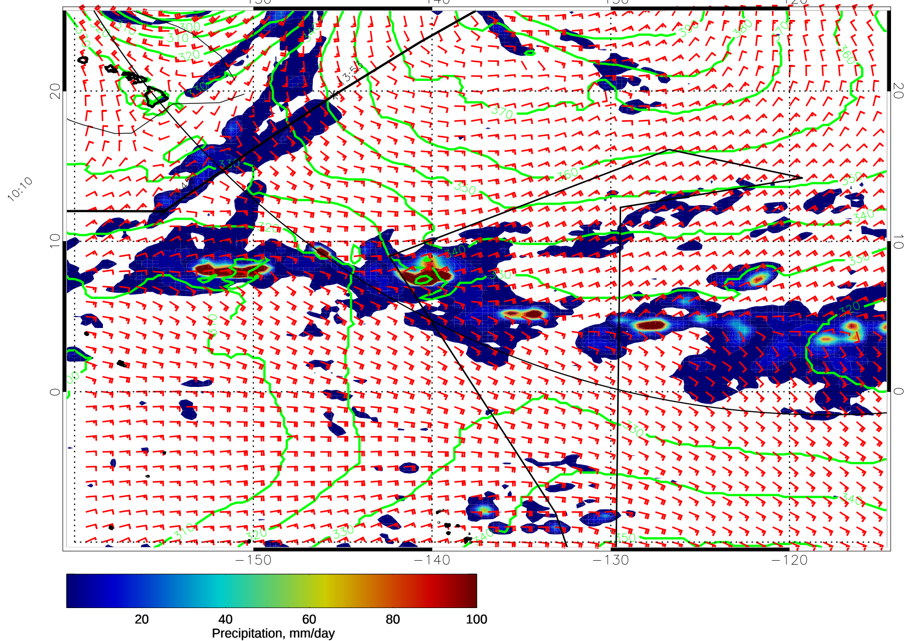
15010106, 6 hour forecast for 975mb Z, Precip., and Surface Winds (knots) -- NASA GEOS5
