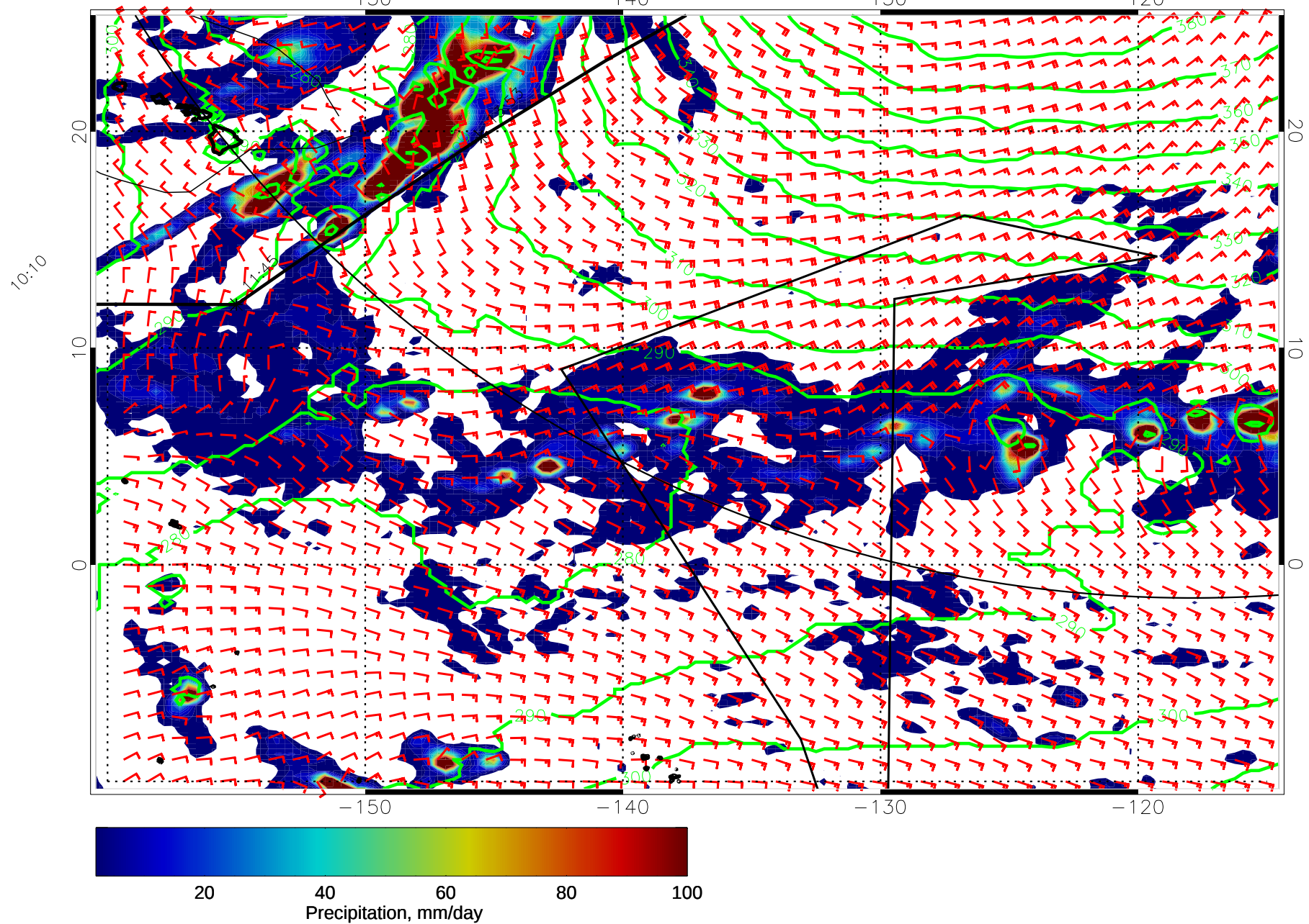
15010312, 60 hour forecast for 975mb Z, Precip., and Surface Winds (knots) -- NASA GEOS5
