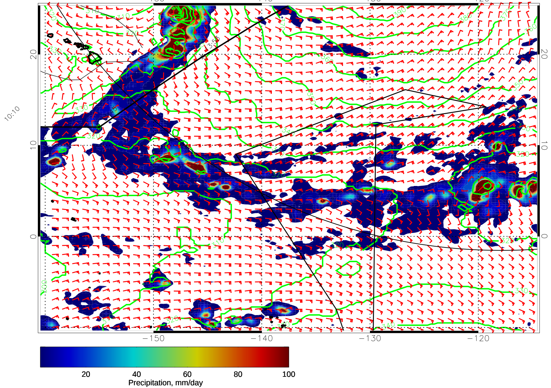
15010206, 30 hour forecast for 975mb Z, Precip., and Surface Winds (knots) -- NASA GEOS5
