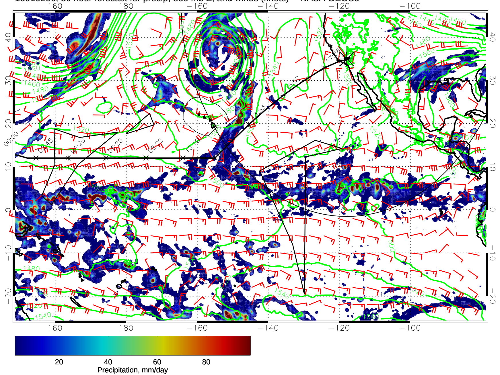
15010206, 30 hour forecast for precip, 850 mb Z, and winds (knots) -- NASA GEOS5
