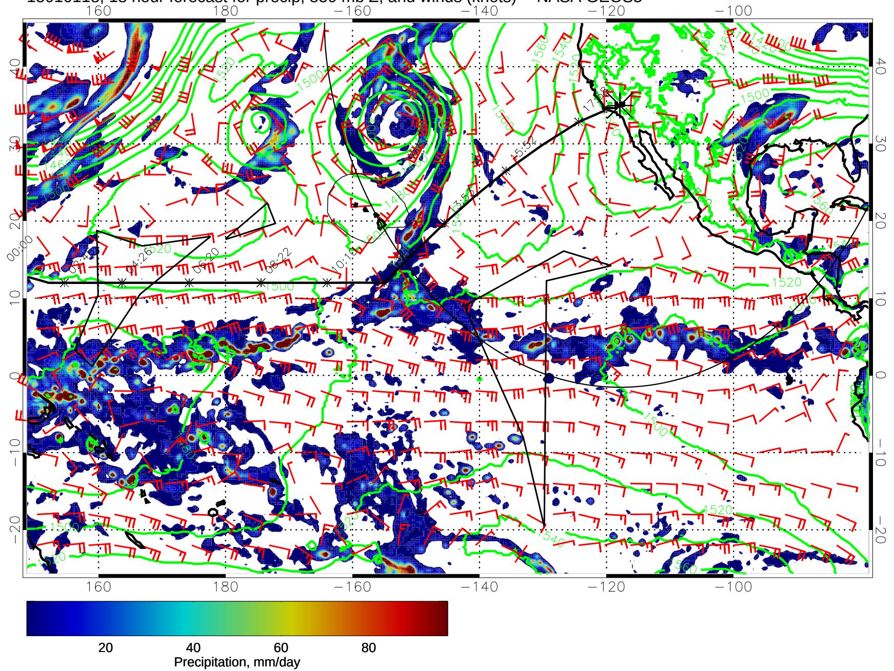
15010118, 18 hour forecast for precip, 850 mb Z, and winds (knots) -- NASA GEOS5
