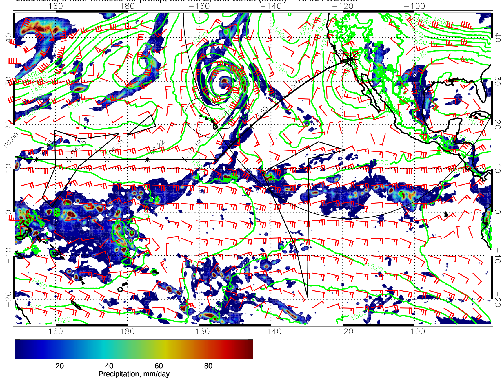
15010106, 6 hour forecast for precip, 850 mb Z, and winds (knots) -- NASA GEOS5
