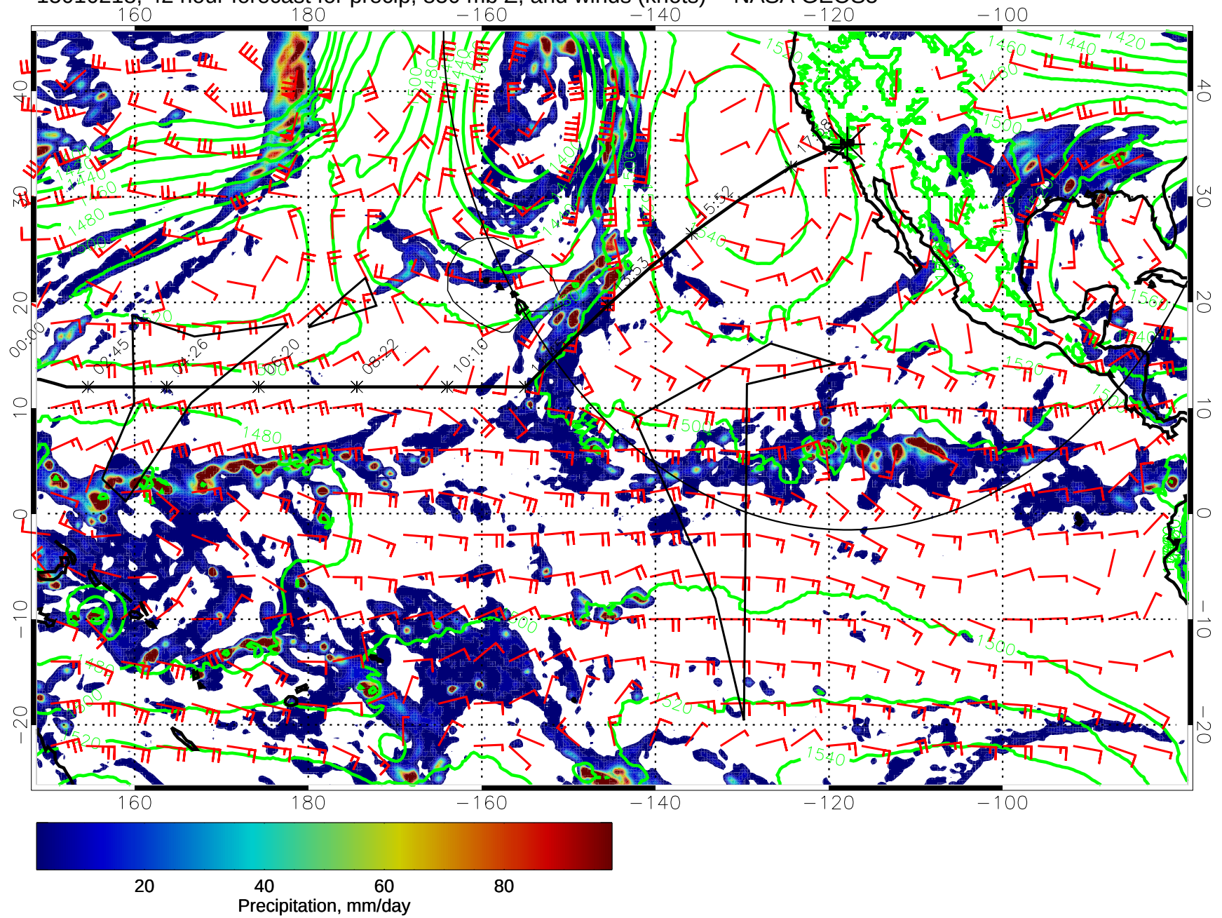
15010218, 42 hour forecast for precip, 850 mb Z, and winds (knots) -- NASA GEOS5
