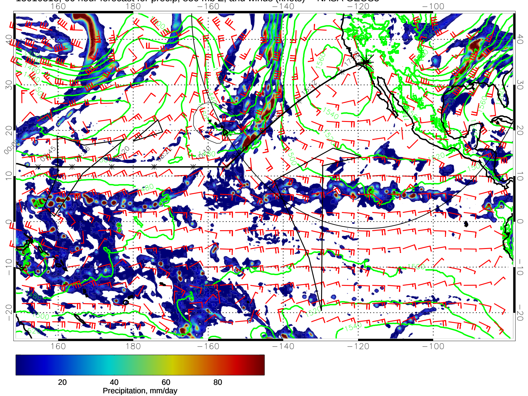
15010318, 66 hour forecast for precip, 850 mb Z, and winds (knots) -- NASA GEOS5
