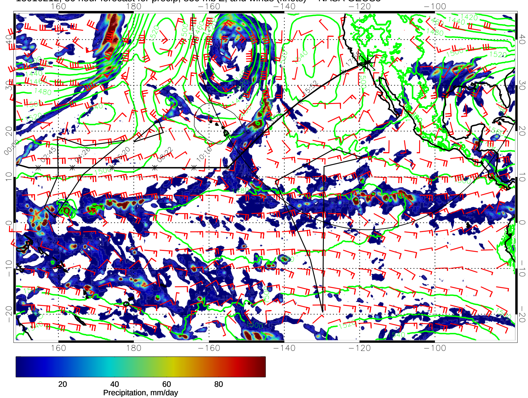
15010212, 36 hour forecast for precip, 850 mb Z, and winds (knots) -- NASA GEOS5
