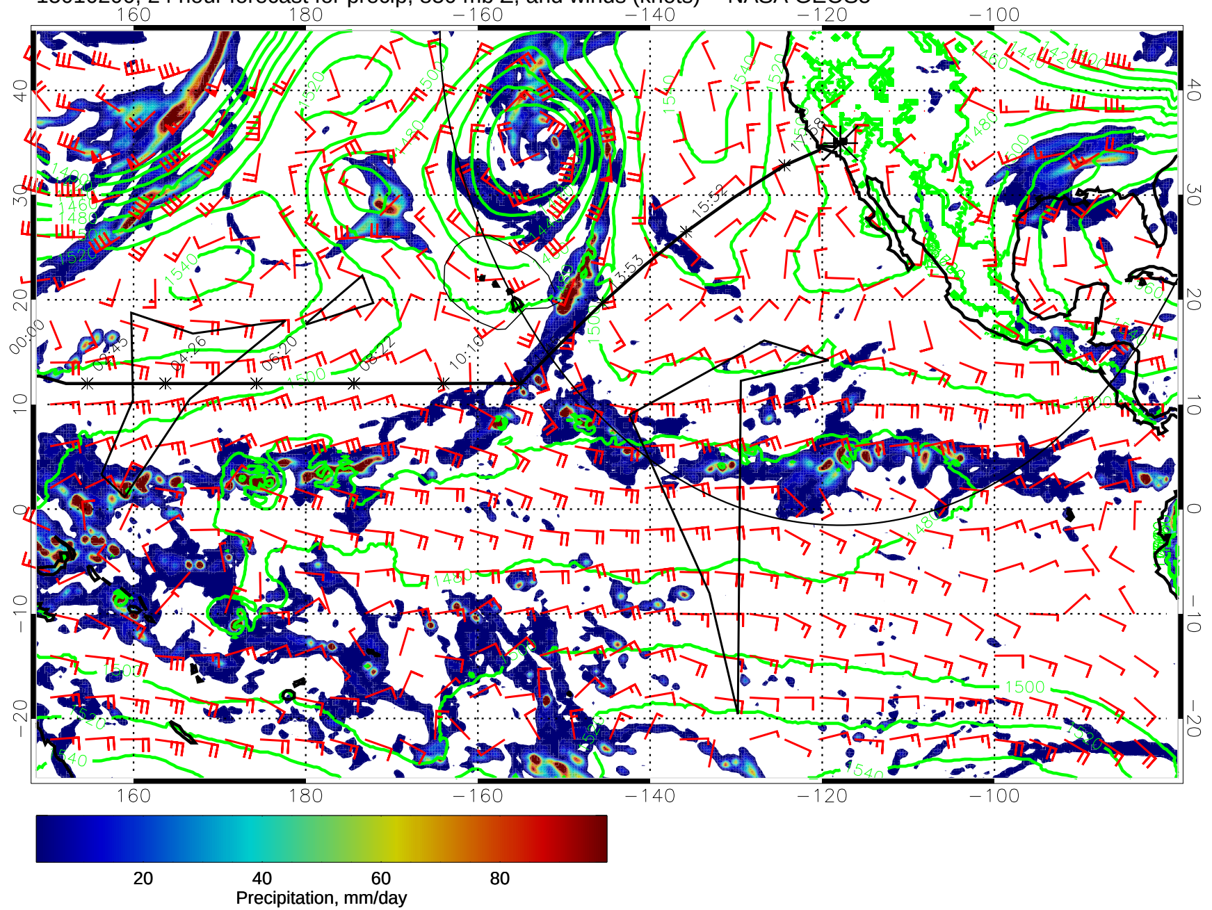
15010200, 24 hour forecast for precip, 850 mb Z, and winds (knots) -- NASA GEOS5
