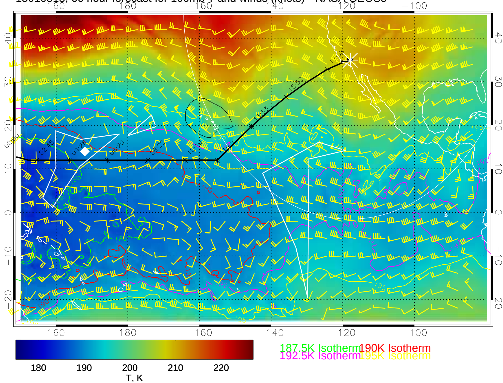
15010318, 66 hour forecast for 100mb T and winds (knots)-- NASA GEOS5
