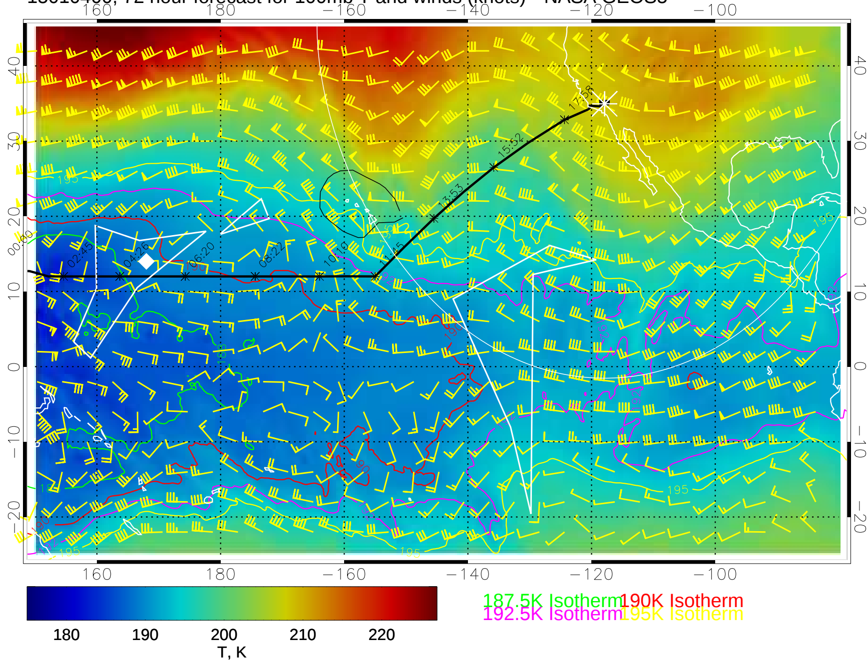
15010400, 72 hour forecast for 100mb T and winds (knots)-- NASA GEOS5
