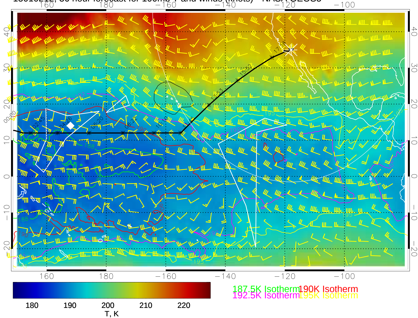
15010212, 36 hour forecast for 100mb T and winds (knots)-- NASA GEOS5
