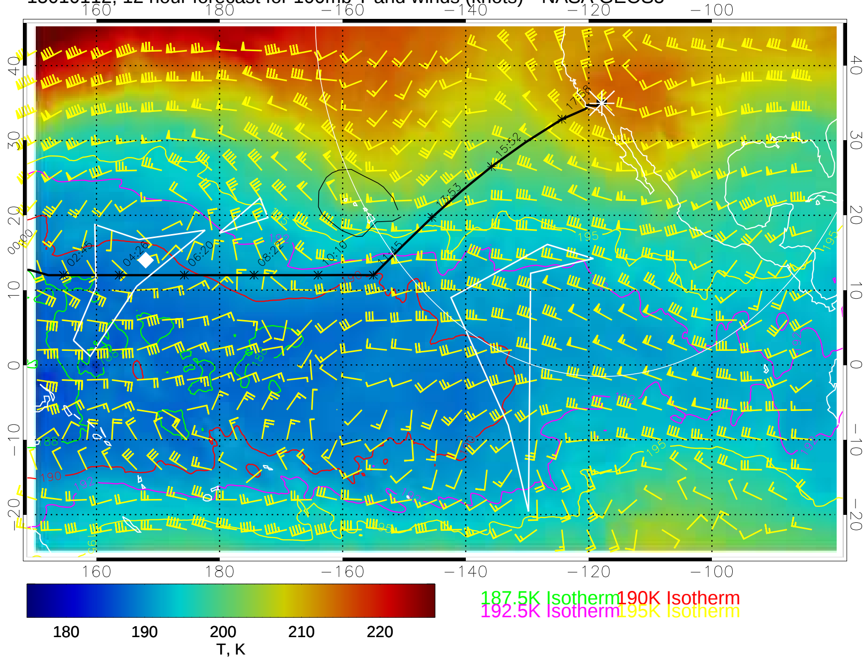
15010112, 12 hour forecast for 100mb T and winds (knots)-- NASA GEOS5
