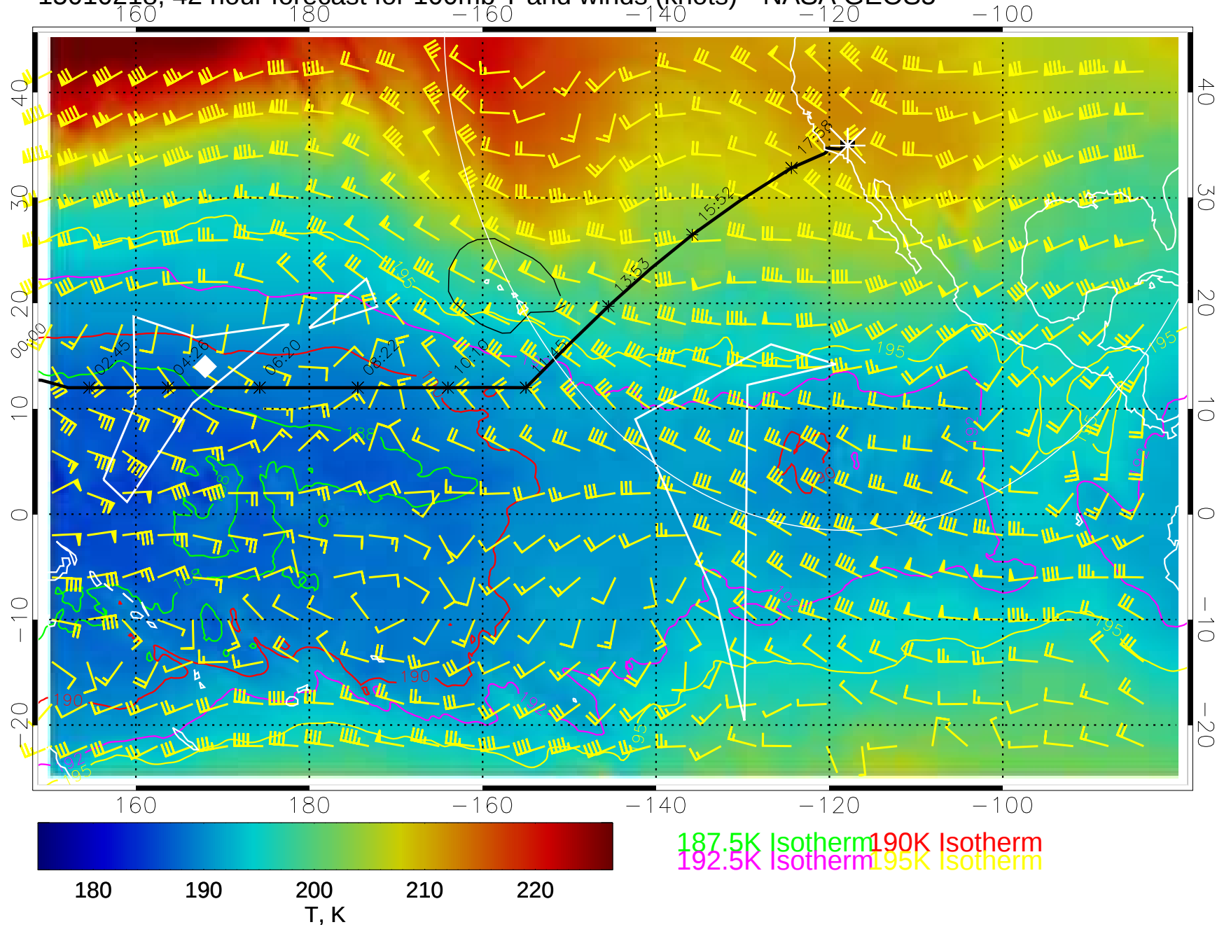
15010218, 42 hour forecast for 100mb T and winds (knots)-- NASA GEOS5
