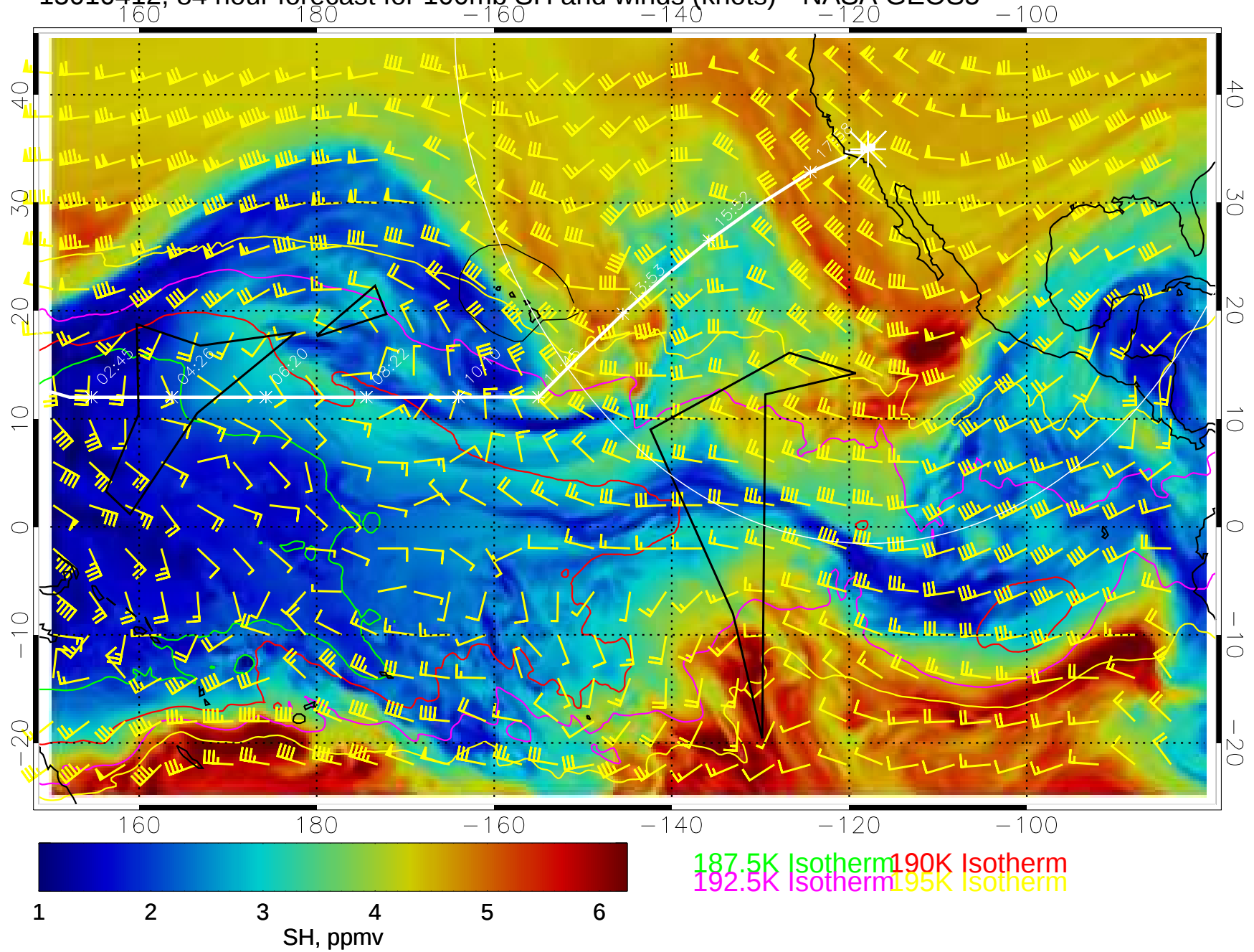
15010412, 84 hour forecast for 100mb SH and winds (knots)-- NASA GEOS5
