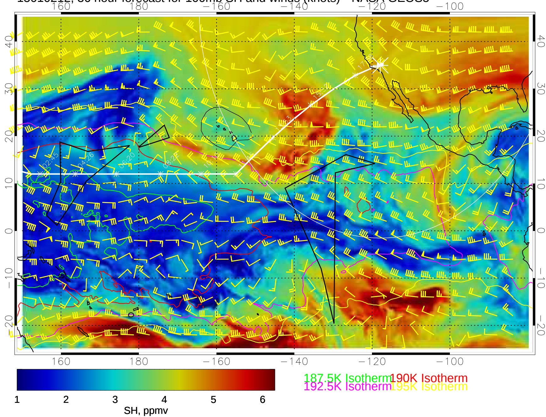
15010212, 36 hour forecast for 100mb SH and winds (knots)-- NASA GEOS5
