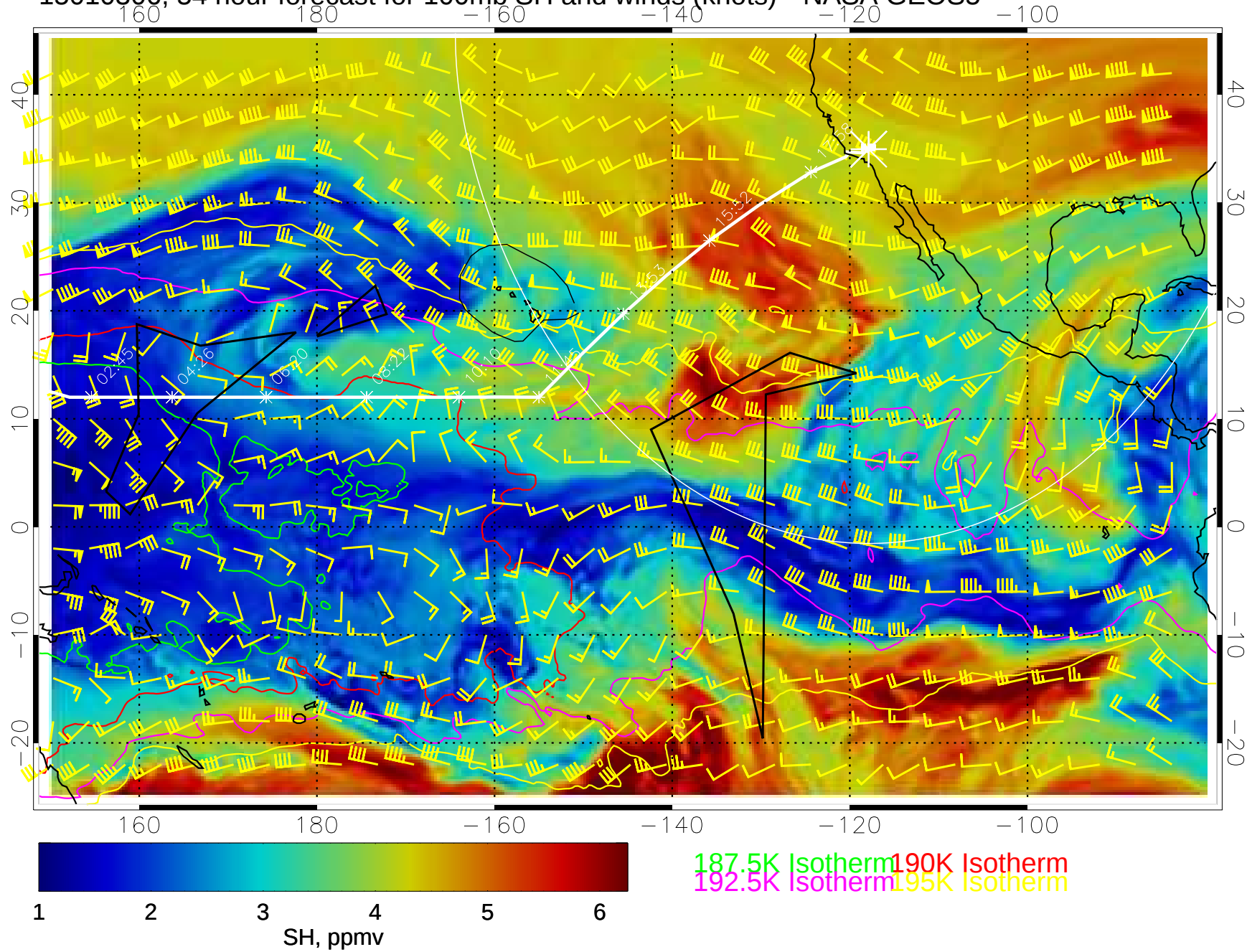
15010306, 54 hour forecast for 100mb SH and winds (knots)-- NASA GEOS5
