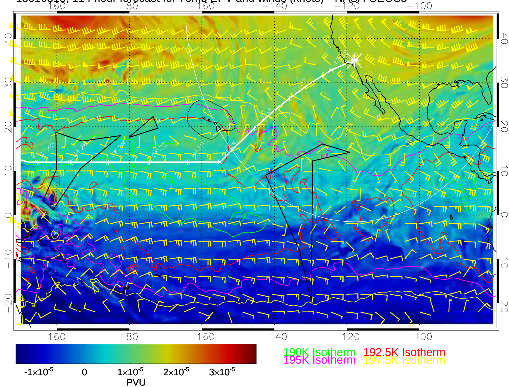
15010518, 114 hour forecast for 70mb EPV and winds (knots)-- NASA GEOS5
