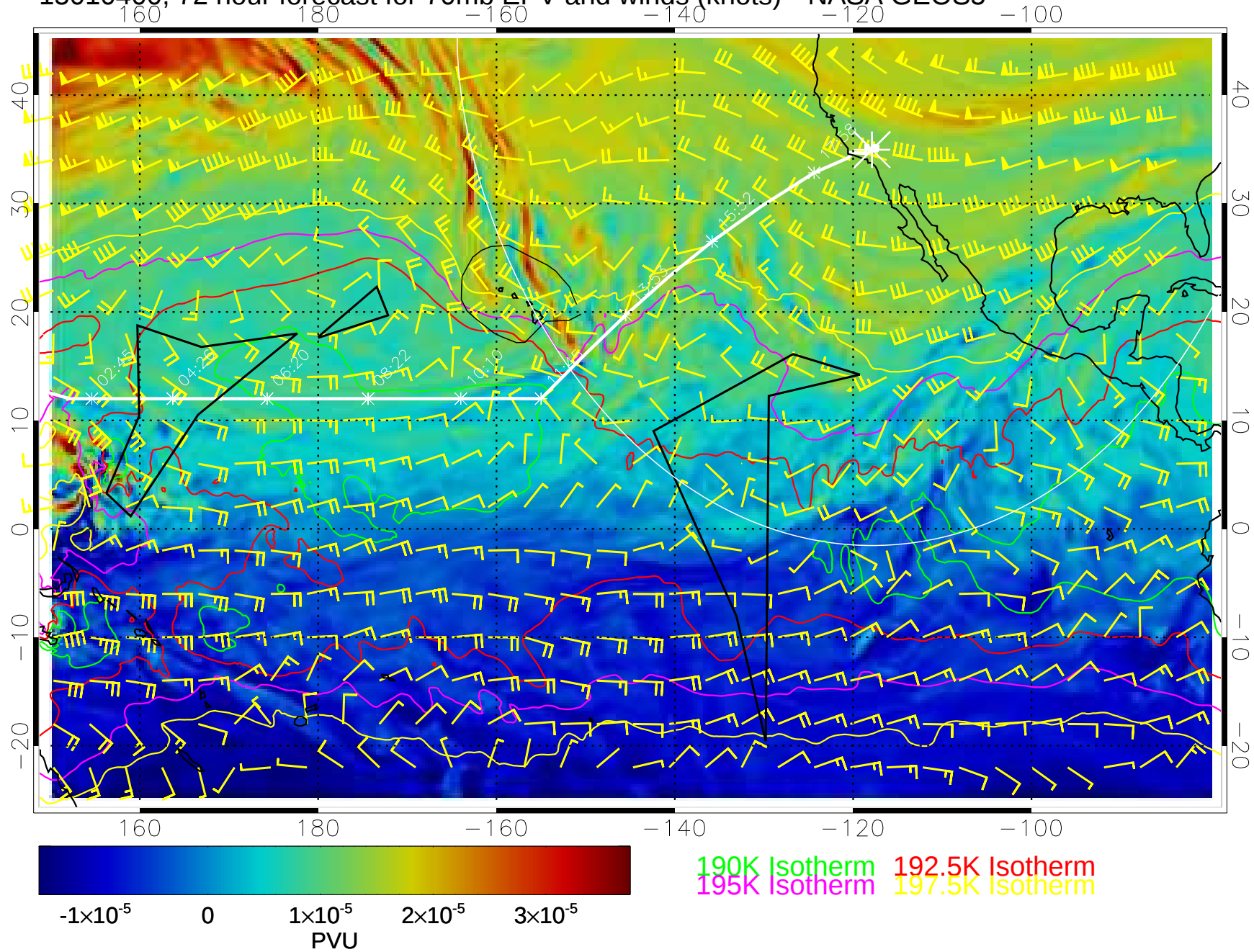
15010400, 72 hour forecast for 70mb EPV and winds (knots)-- NASA GEOS5
