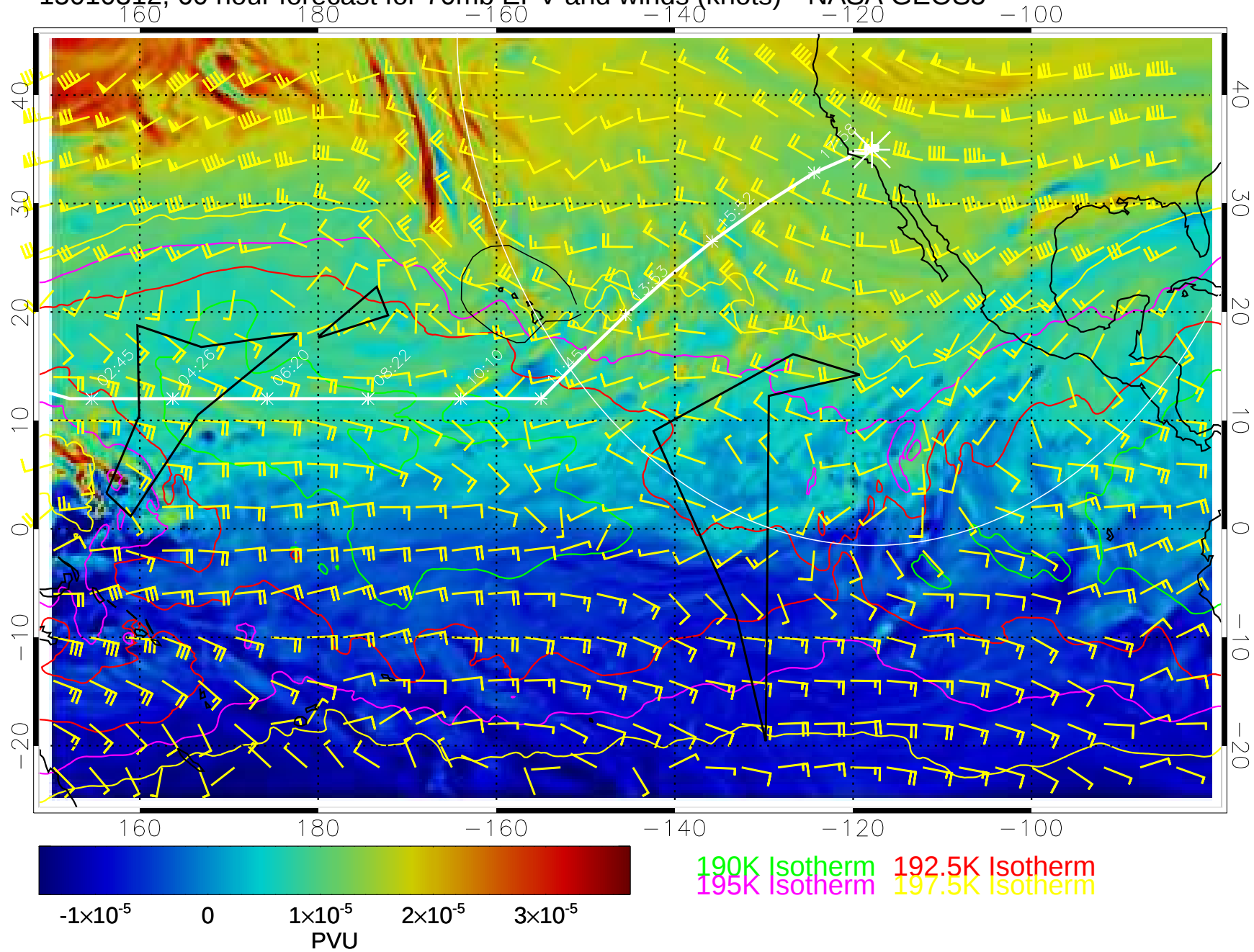
15010312, 60 hour forecast for 70mb EPV and winds (knots)-- NASA GEOS5
