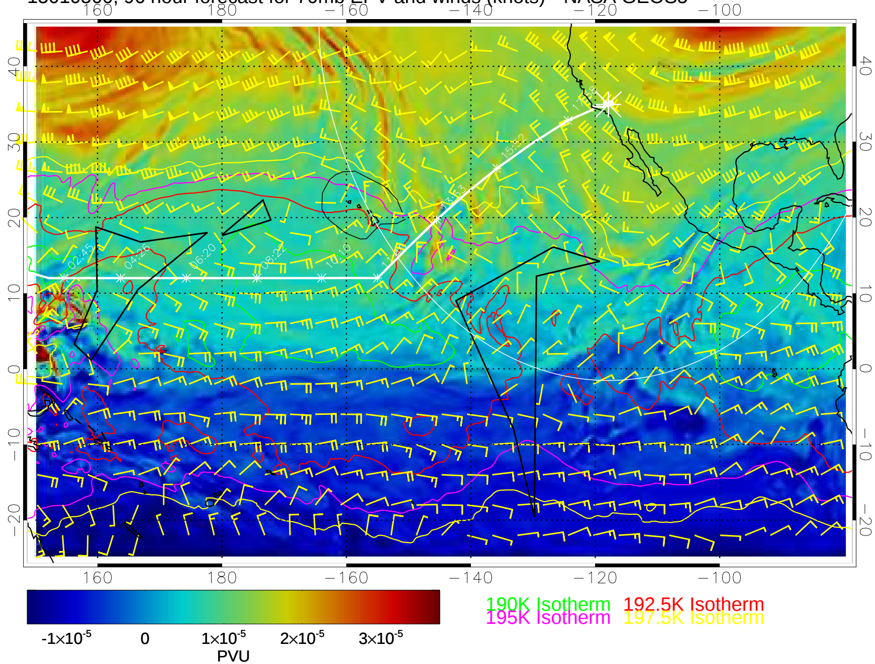
15010500, 96 hour forecast for 70mb EPV and winds (knots)-- NASA GEOS5
