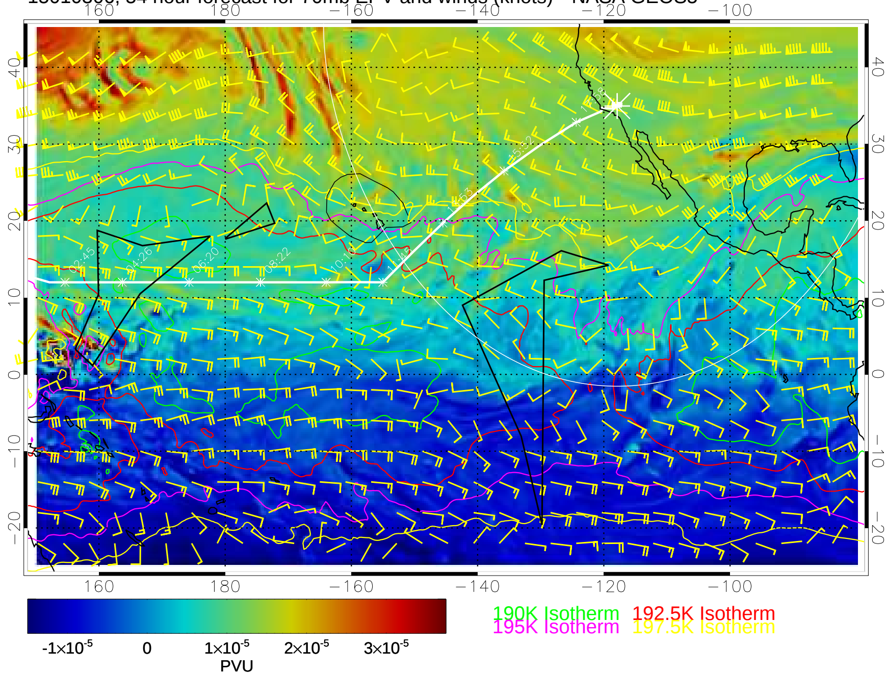
15010306, 54 hour forecast for 70mb EPV and winds (knots)-- NASA GEOS5
