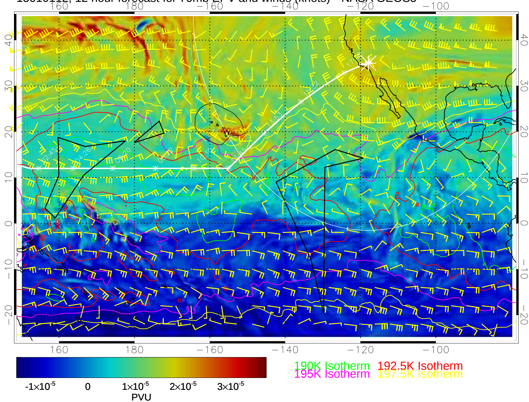
15010112, 12 hour forecast for 70mb EPV and winds (knots)-- NASA GEOS5
