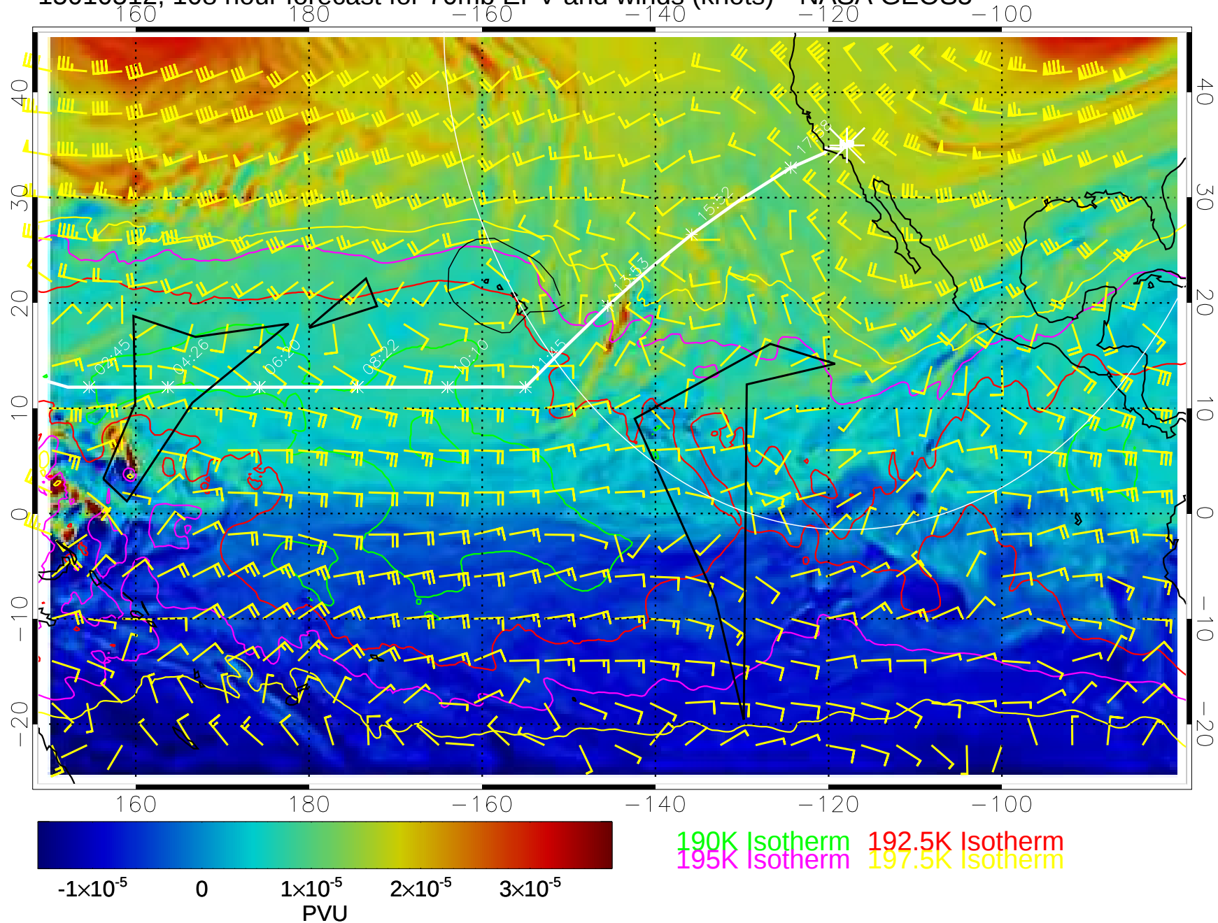
15010512, 108 hour forecast for 70mb EPV and winds (knots)-- NASA GEOS5
