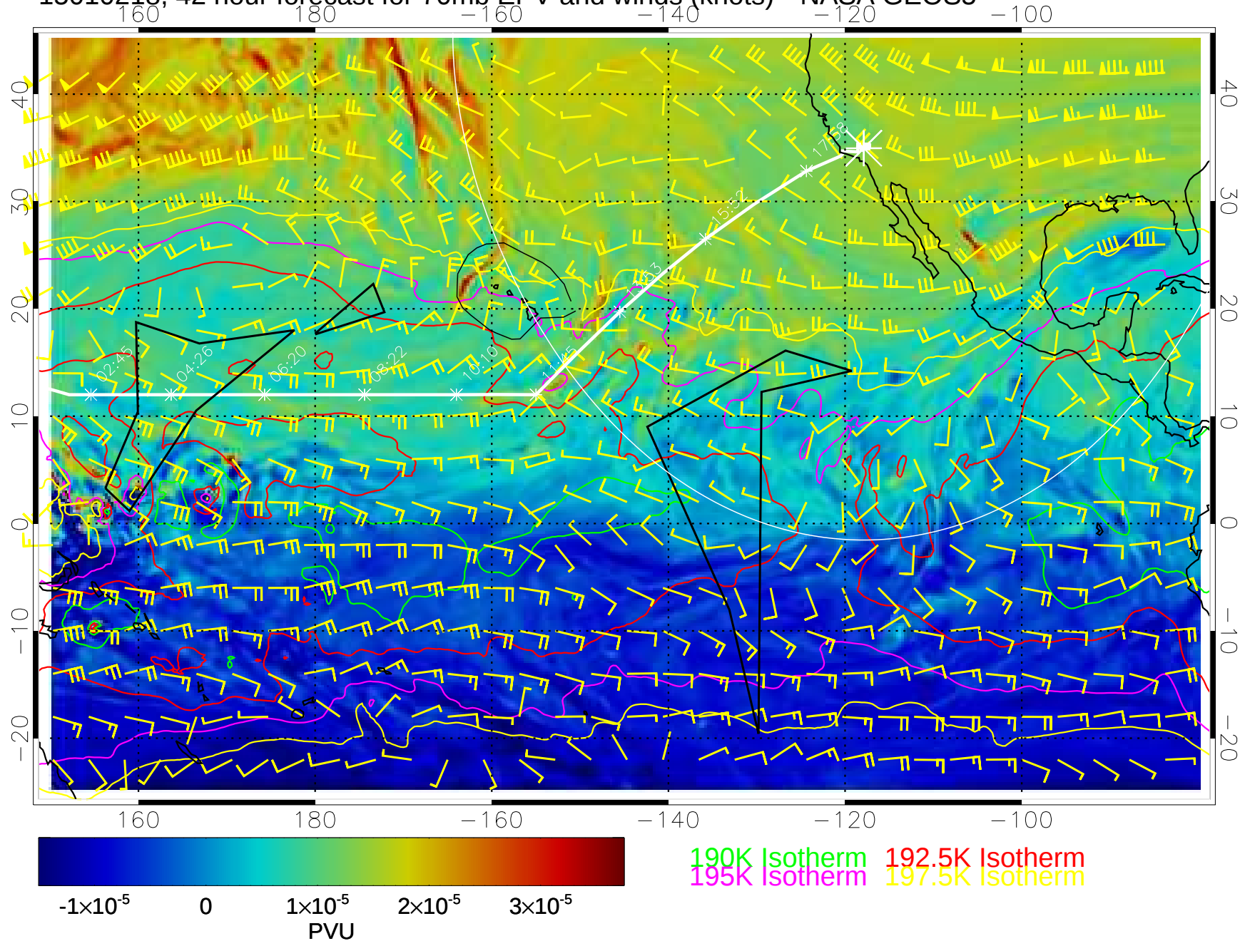
15010218, 42 hour forecast for 70mb EPV and winds (knots)-- NASA GEOS5
