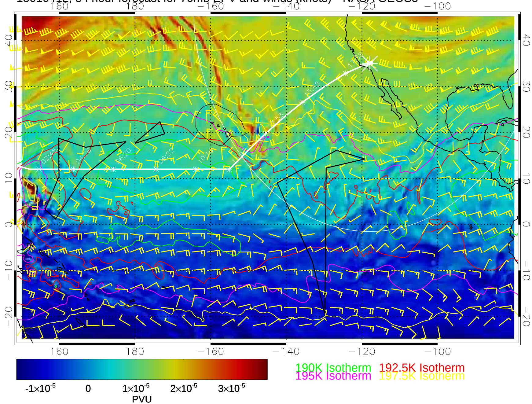
15010412, 84 hour forecast for 70mb EPV and winds (knots)-- NASA GEOS5
