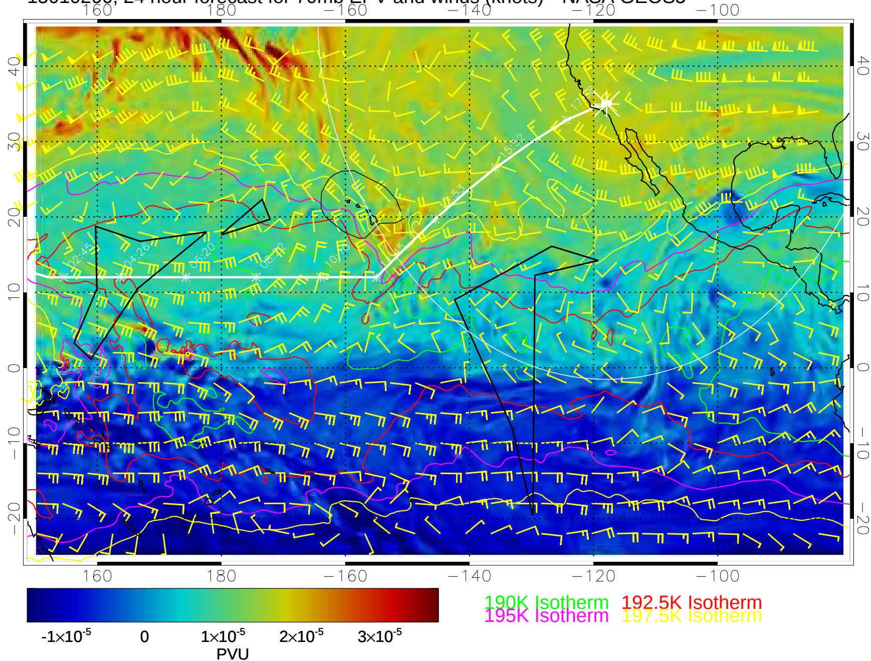
15010200, 24 hour forecast for 70mb EPV and winds (knots)-- NASA GEOS5
