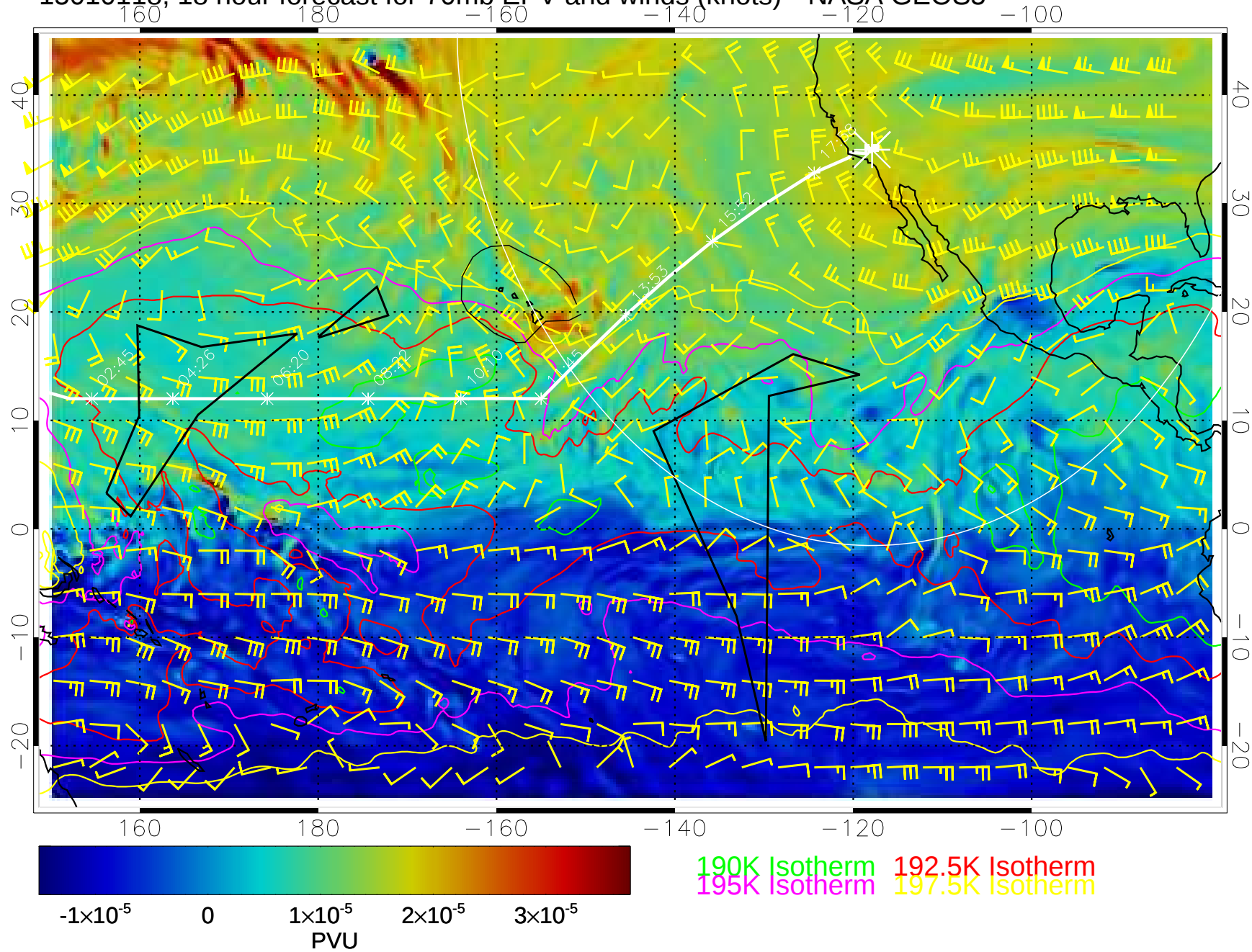
15010118, 18 hour forecast for 70mb EPV and winds (knots)-- NASA GEOS5
