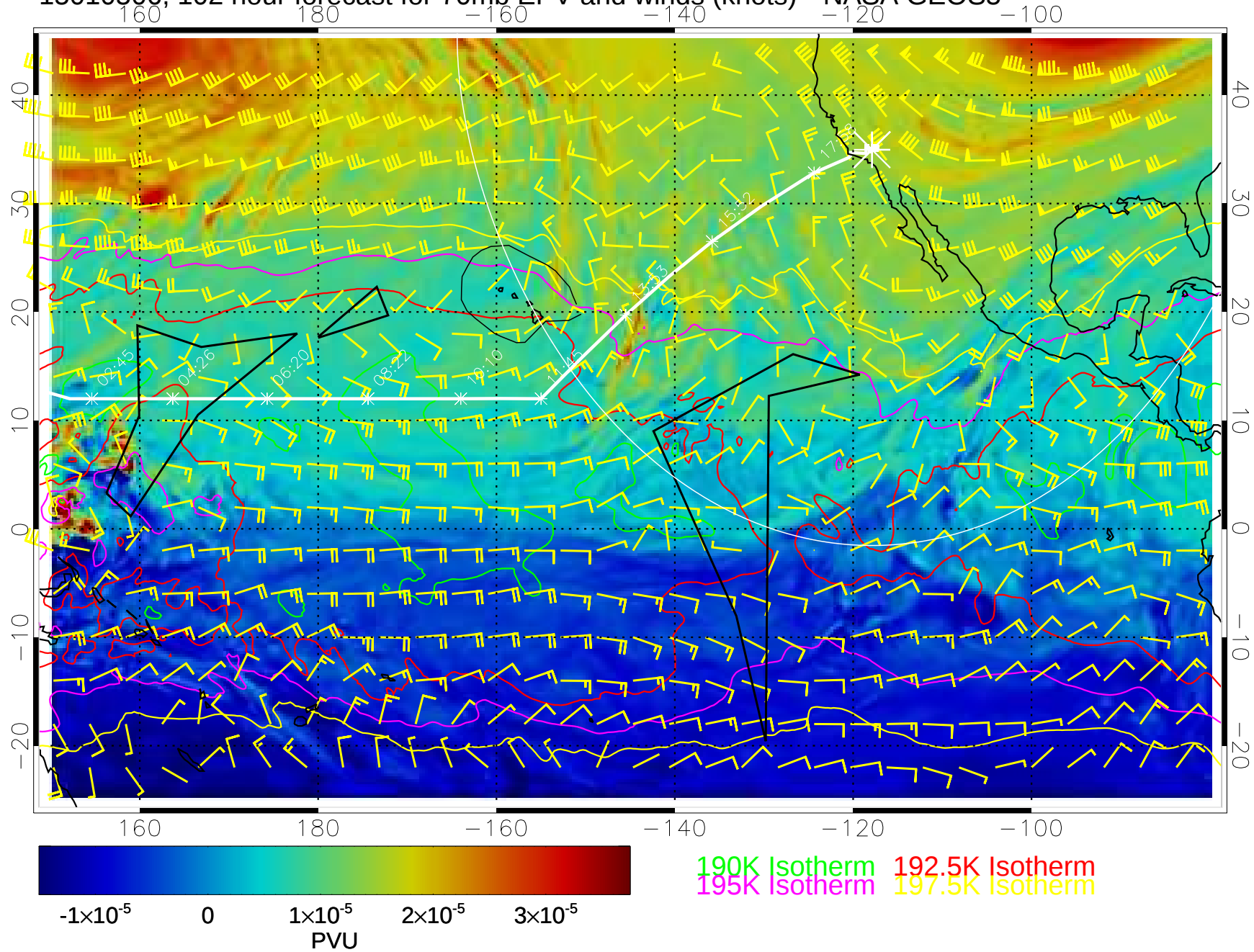
15010506, 102 hour forecast for 70mb EPV and winds (knots)-- NASA GEOS5
