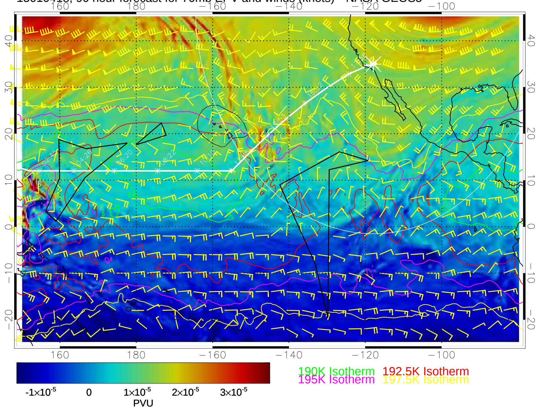
15010418, 90 hour forecast for 70mb EPV and winds (knots)-- NASA GEOS5
