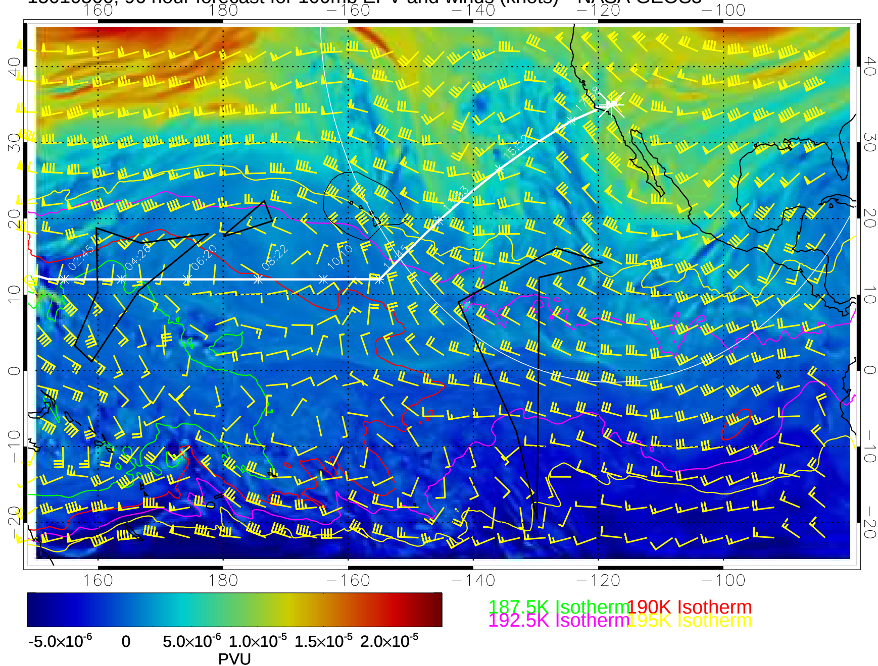
15010500, 96 hour forecast for 100mb EPV and winds (knots)-- NASA GEOS5
