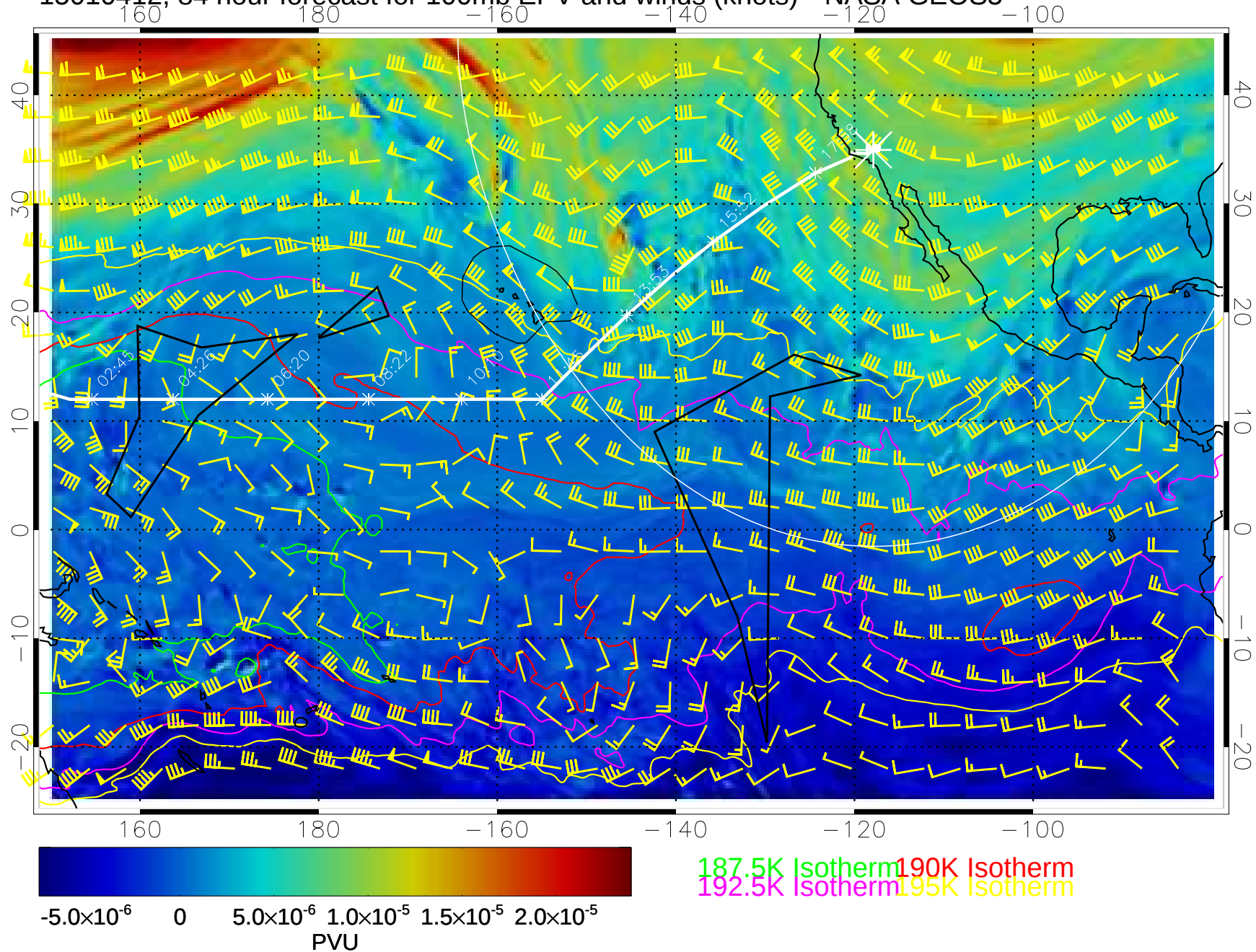
15010412, 84 hour forecast for 100mb EPV and winds (knots)-- NASA GEOS5
