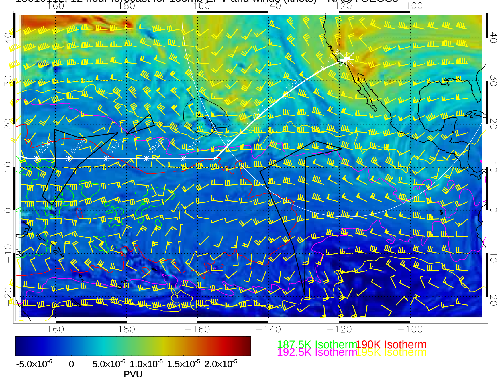
15010112, 12 hour forecast for 100mb EPV and winds (knots)-- NASA GEOS5
