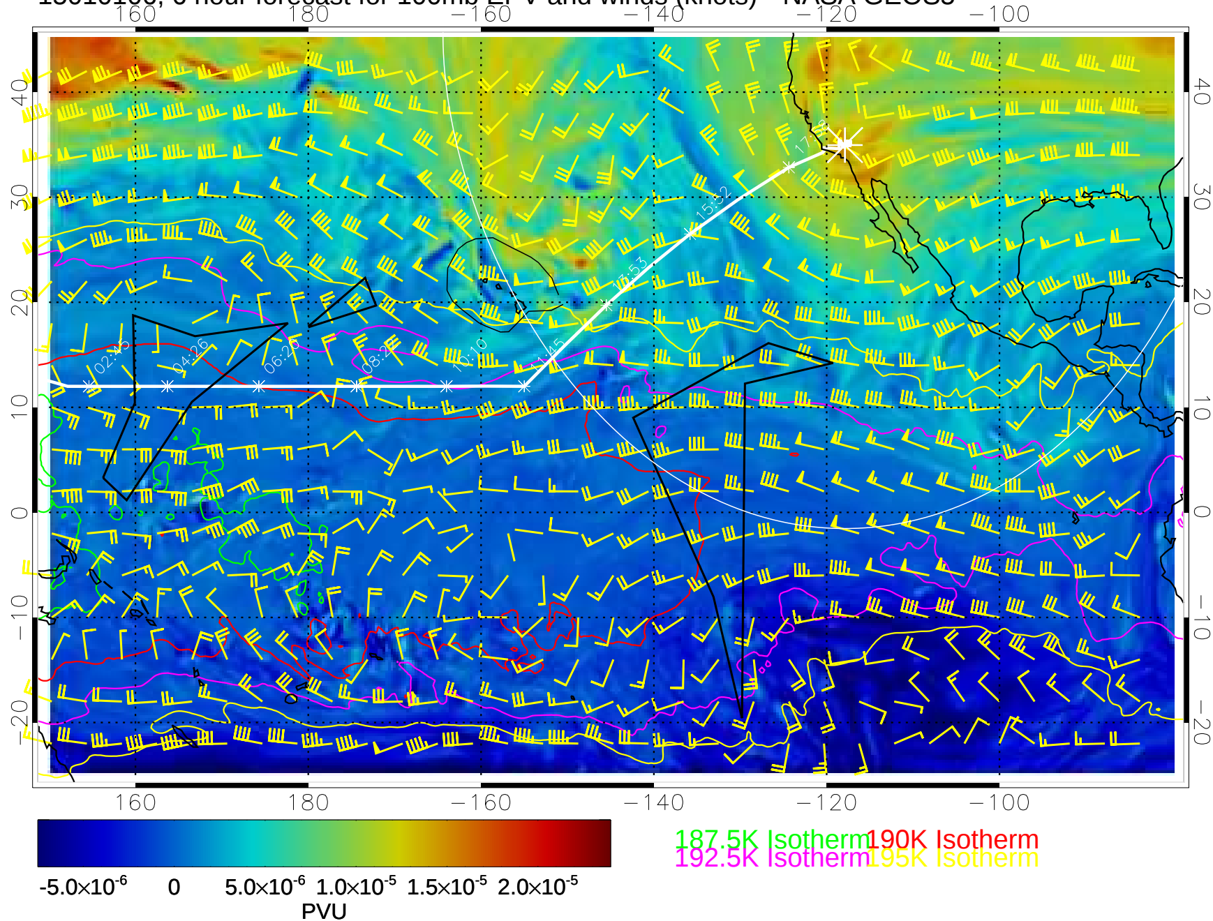
15010106, 6 hour forecast for 100mb EPV and winds (knots)-- NASA GEOS5
