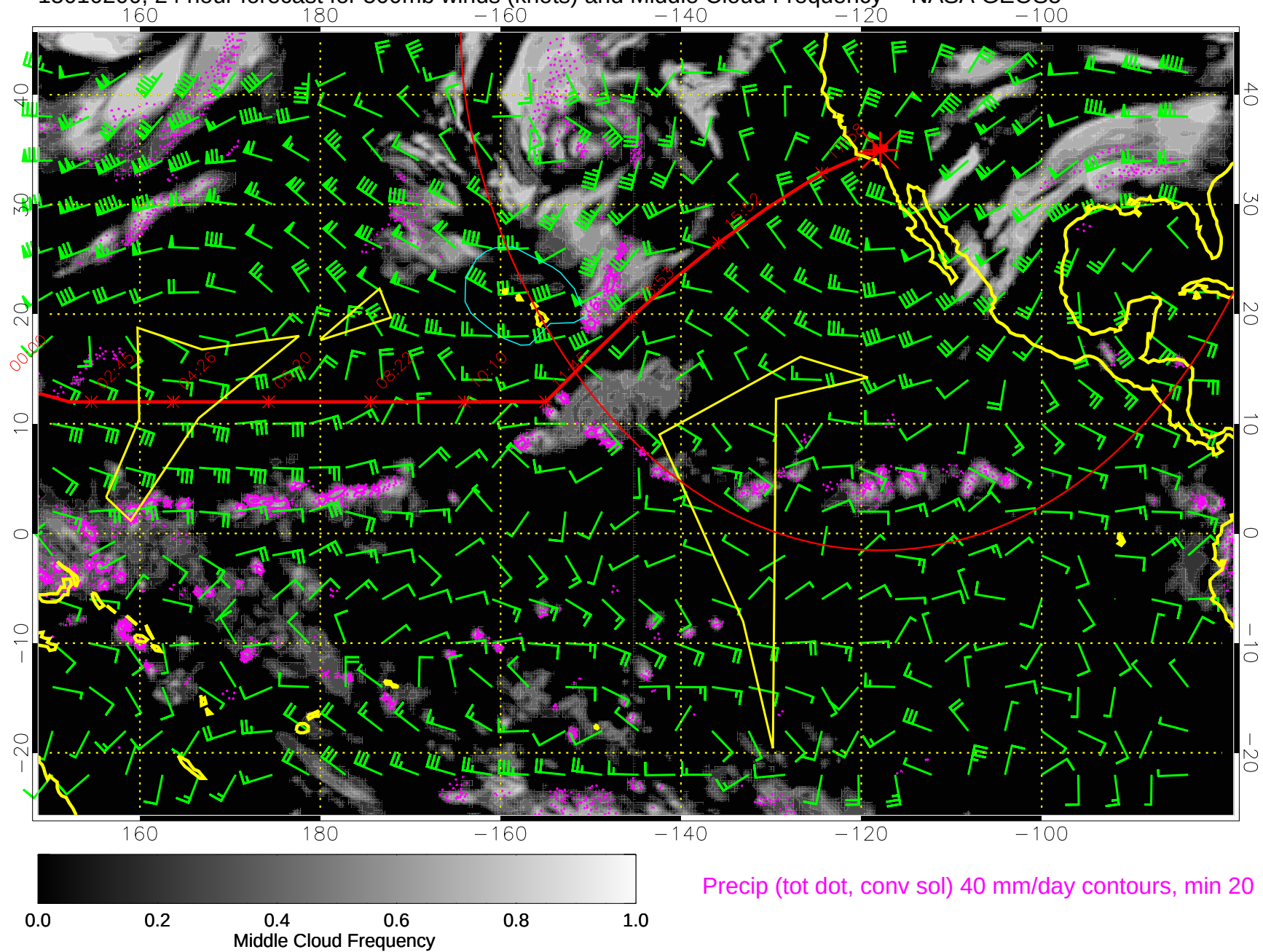
15010200, 24 hour forecast for 500mb winds (knots) and Middle Cloud Frequency -- NASA GEOS5
