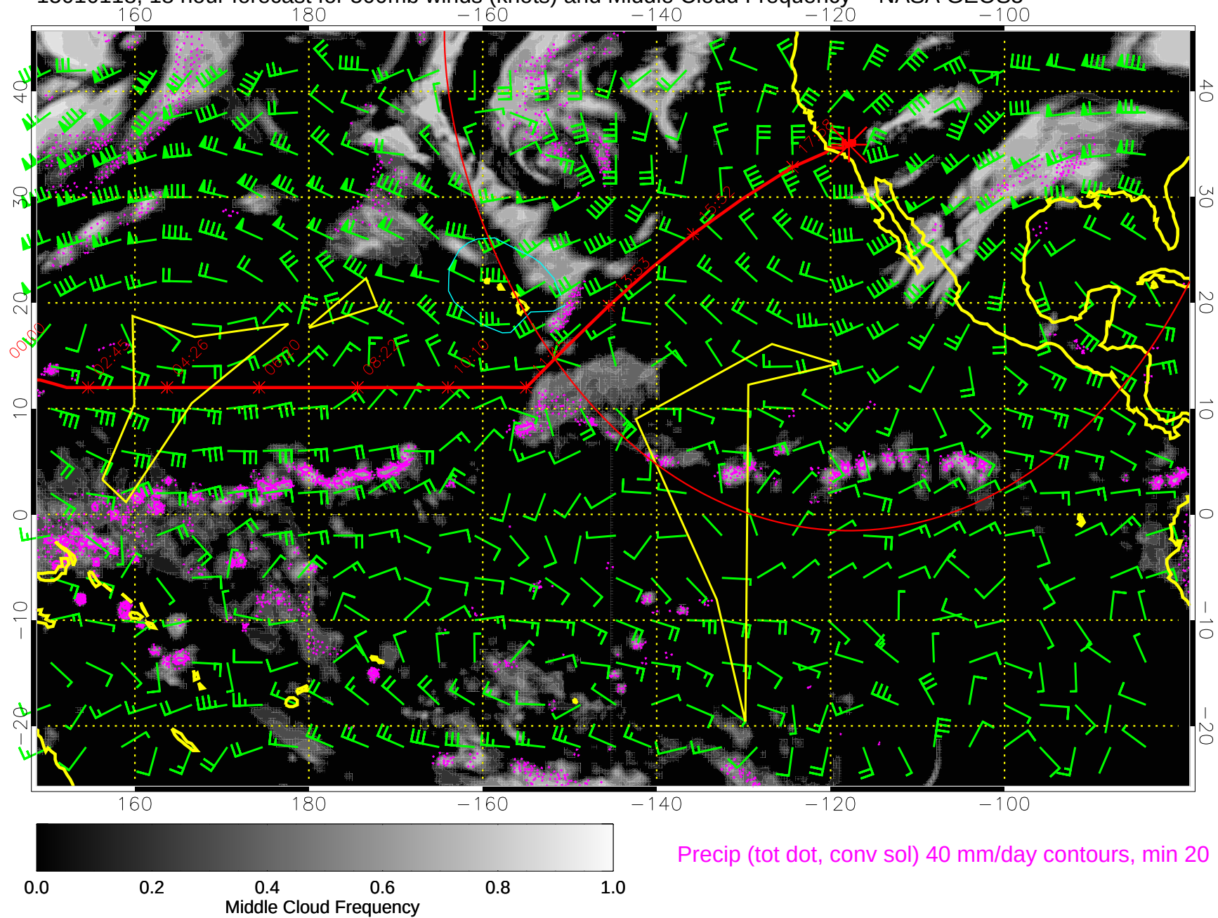
15010118, 18 hour forecast for 500mb winds (knots) and Middle Cloud Frequency -- NASA GEOS5
