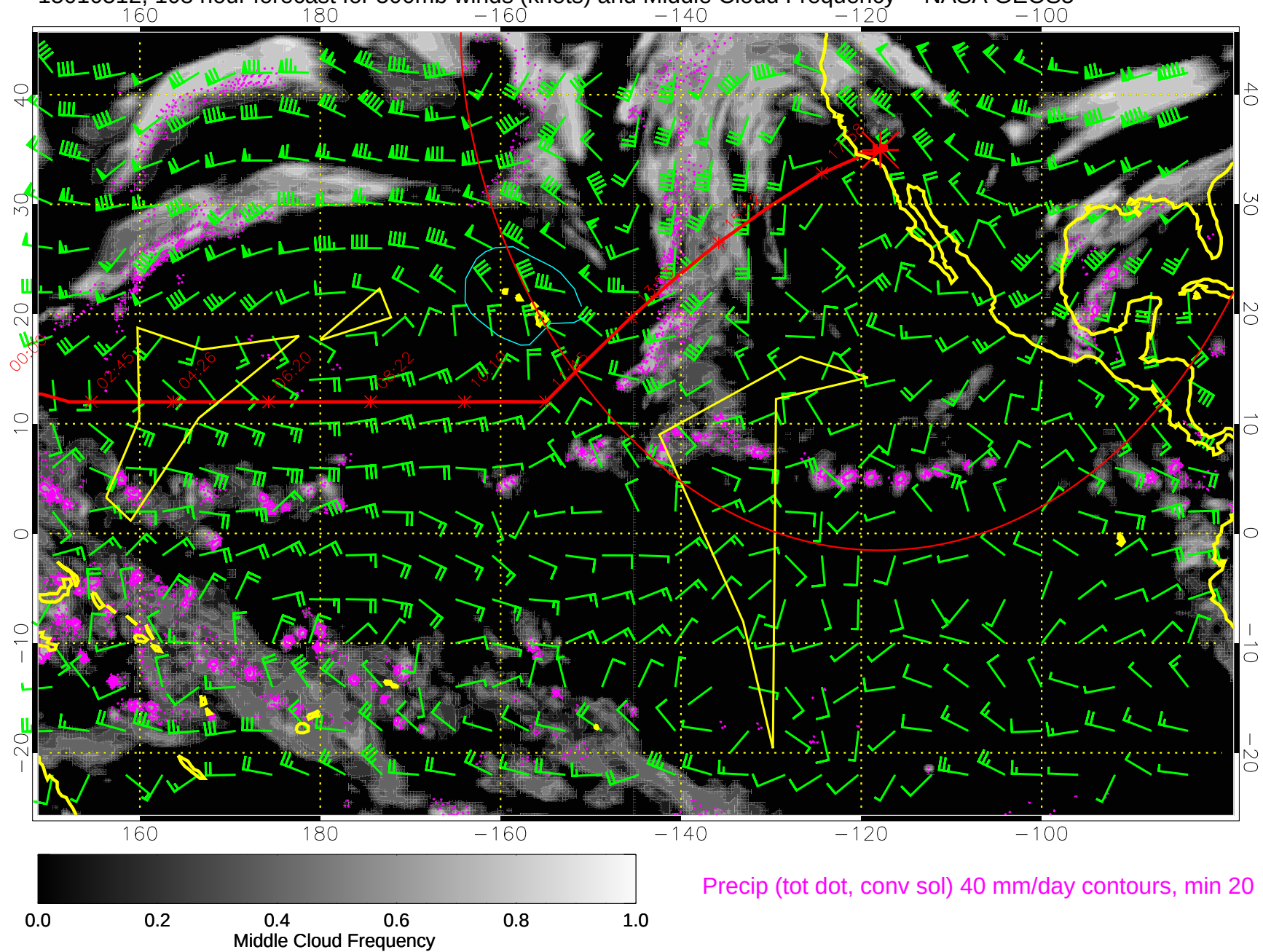
15010512, 108 hour forecast for 500mb winds (knots) and Middle Cloud Frequency -- NASA GEOS5
