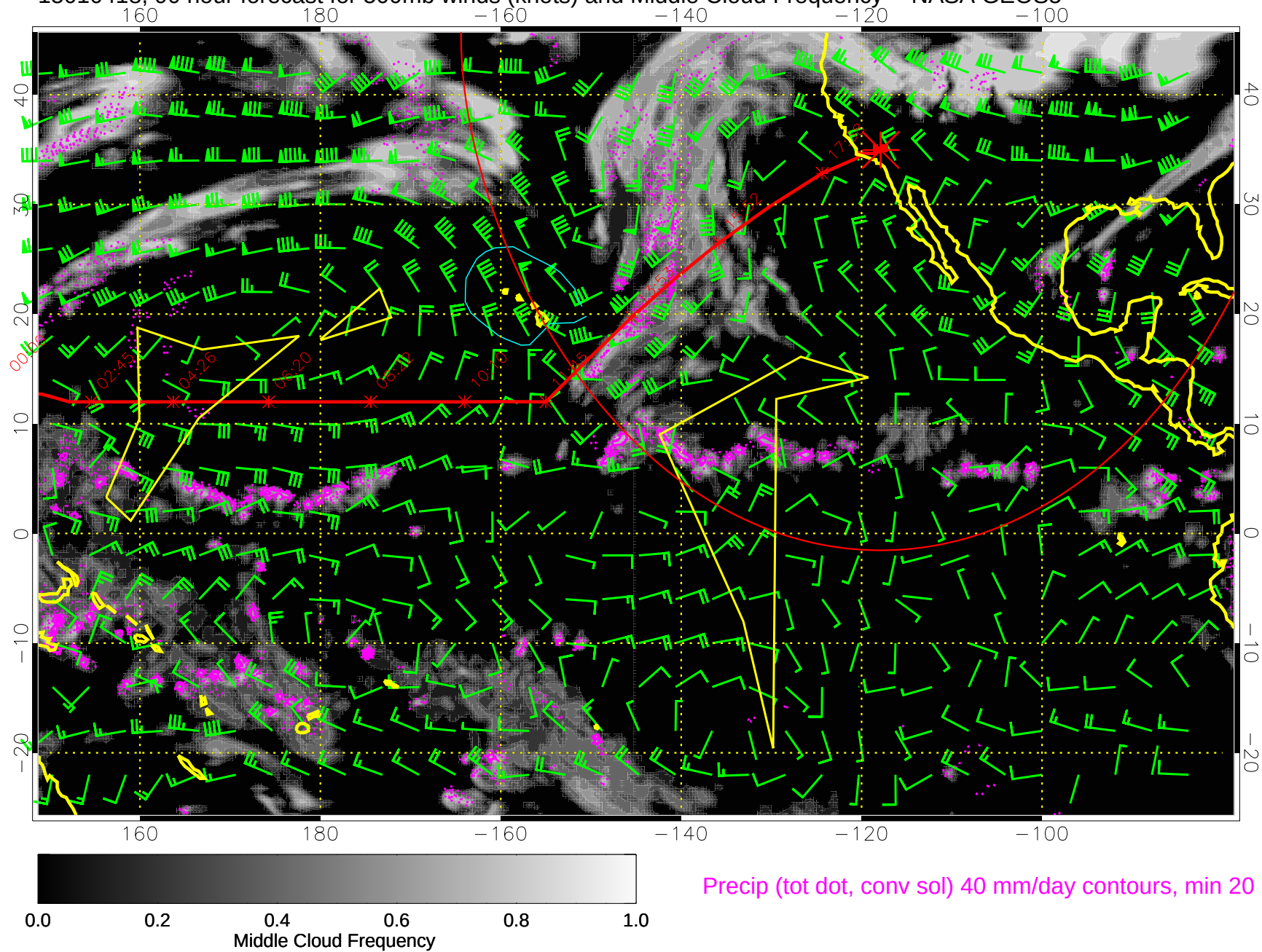
15010418, 90 hour forecast for 500mb winds (knots) and Middle Cloud Frequency -- NASA GEOS5
