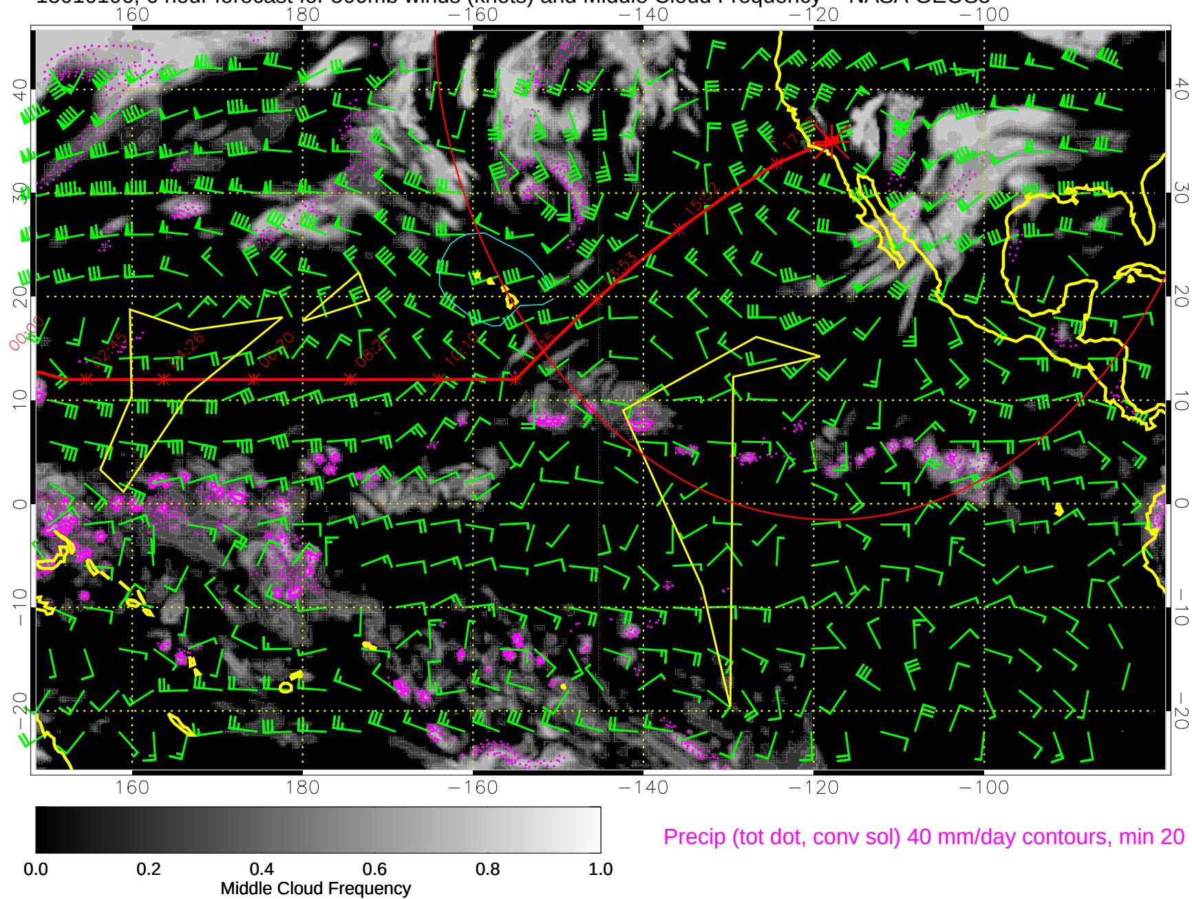
15010106, 6 hour forecast for 500mb winds (knots) and Middle Cloud Frequency -- NASA GEOS5
