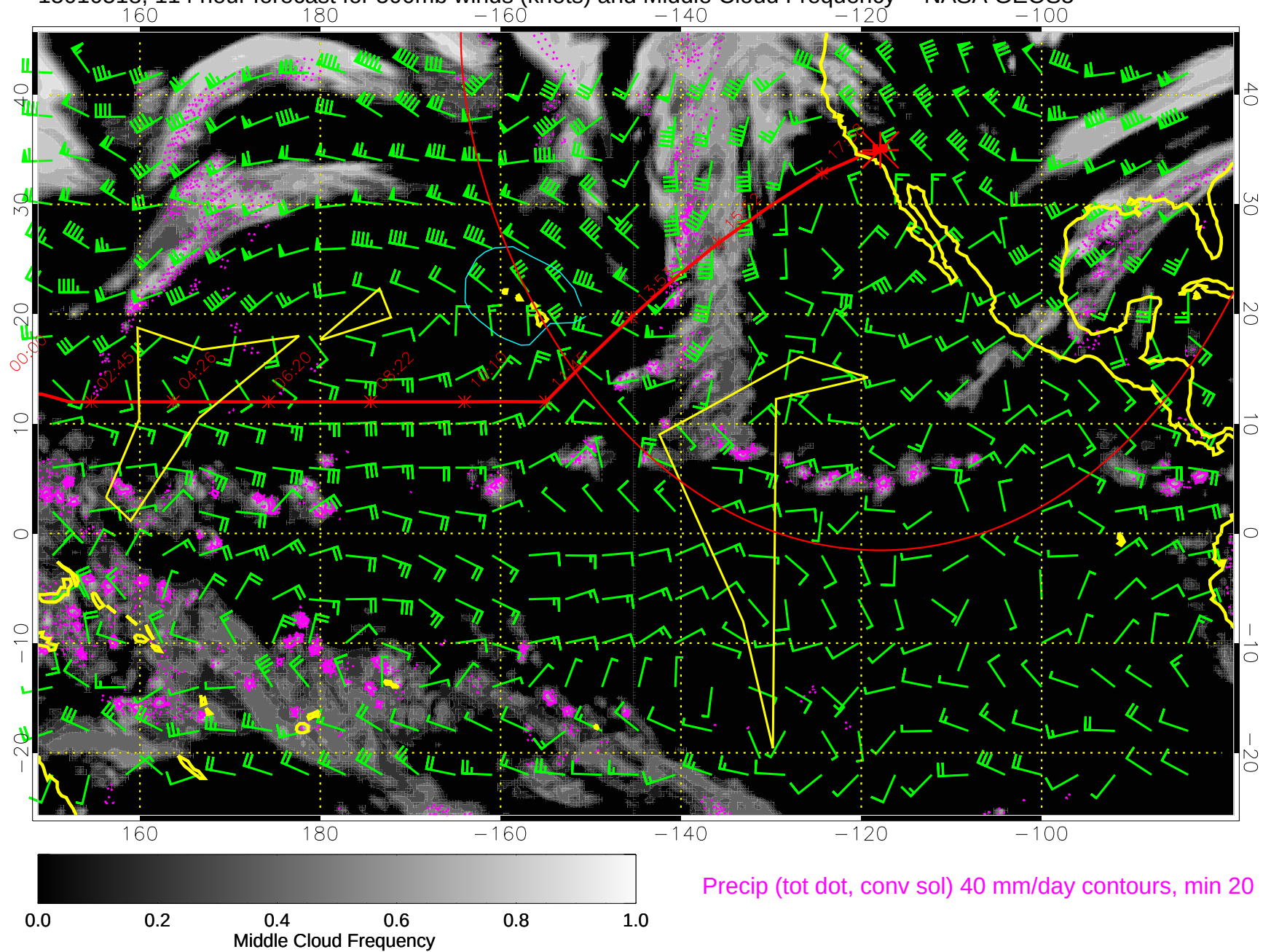
15010518, 114 hour forecast for 500mb winds (knots) and Middle Cloud Frequency -- NASA GEOS5
