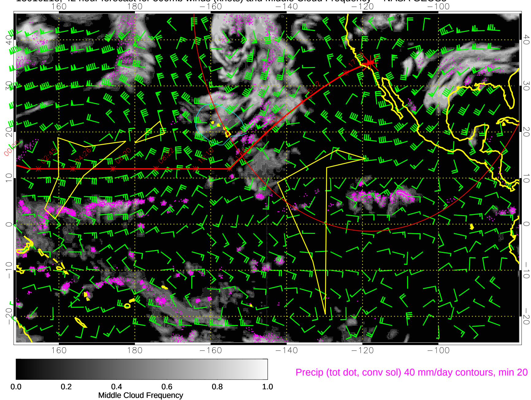
15010218, 42 hour forecast for 500mb winds (knots) and Middle Cloud Frequency -- NASA GEOS5
