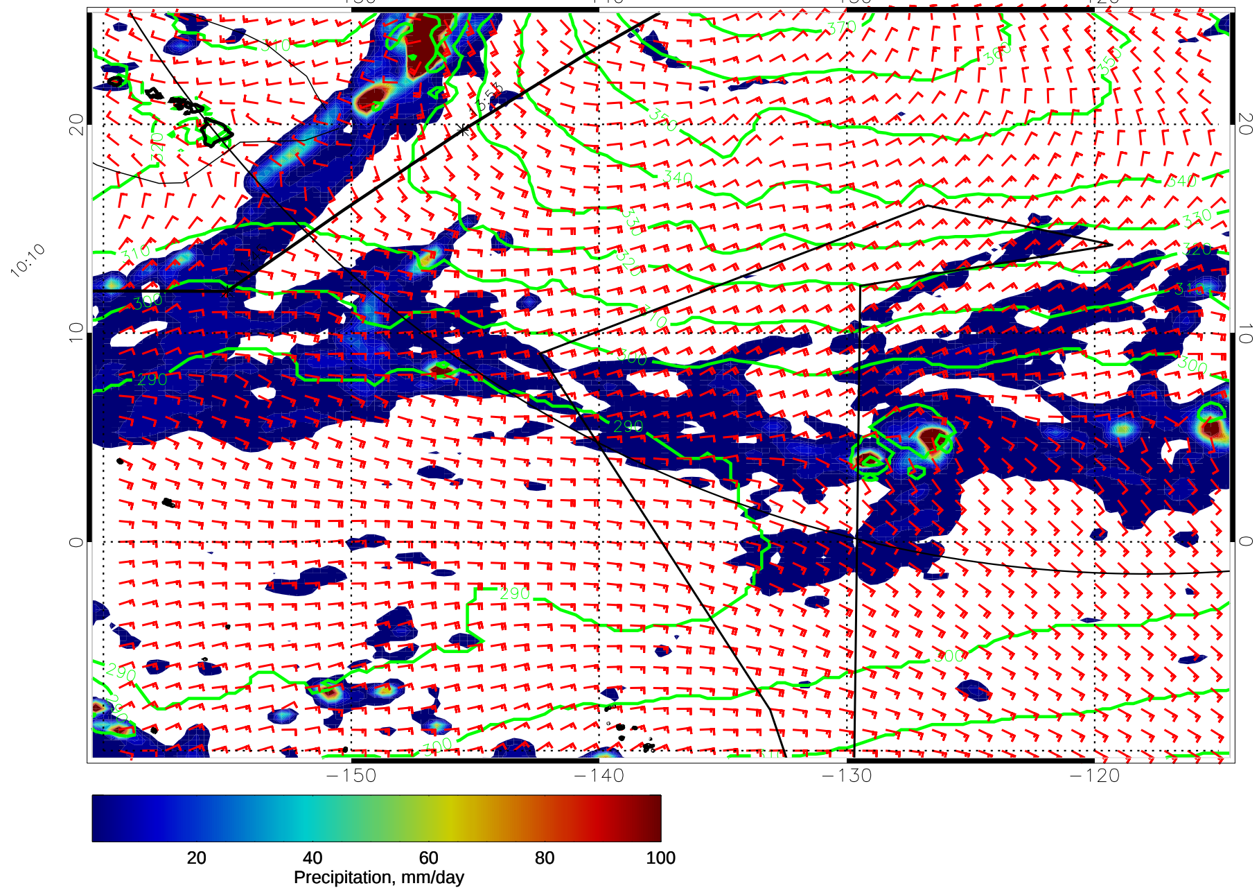
15010200, 96 hour forecast for 975mb Z, Precip., and Surface Winds (knots) -- NASA GEOS5
