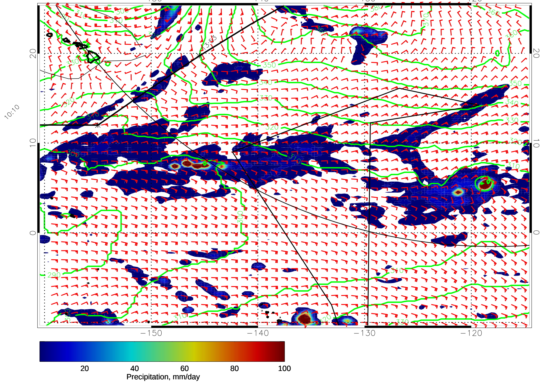
15010100, 72 hour forecast for 975mb Z, Precip., and Surface Winds (knots) -- NASA GEOS5
