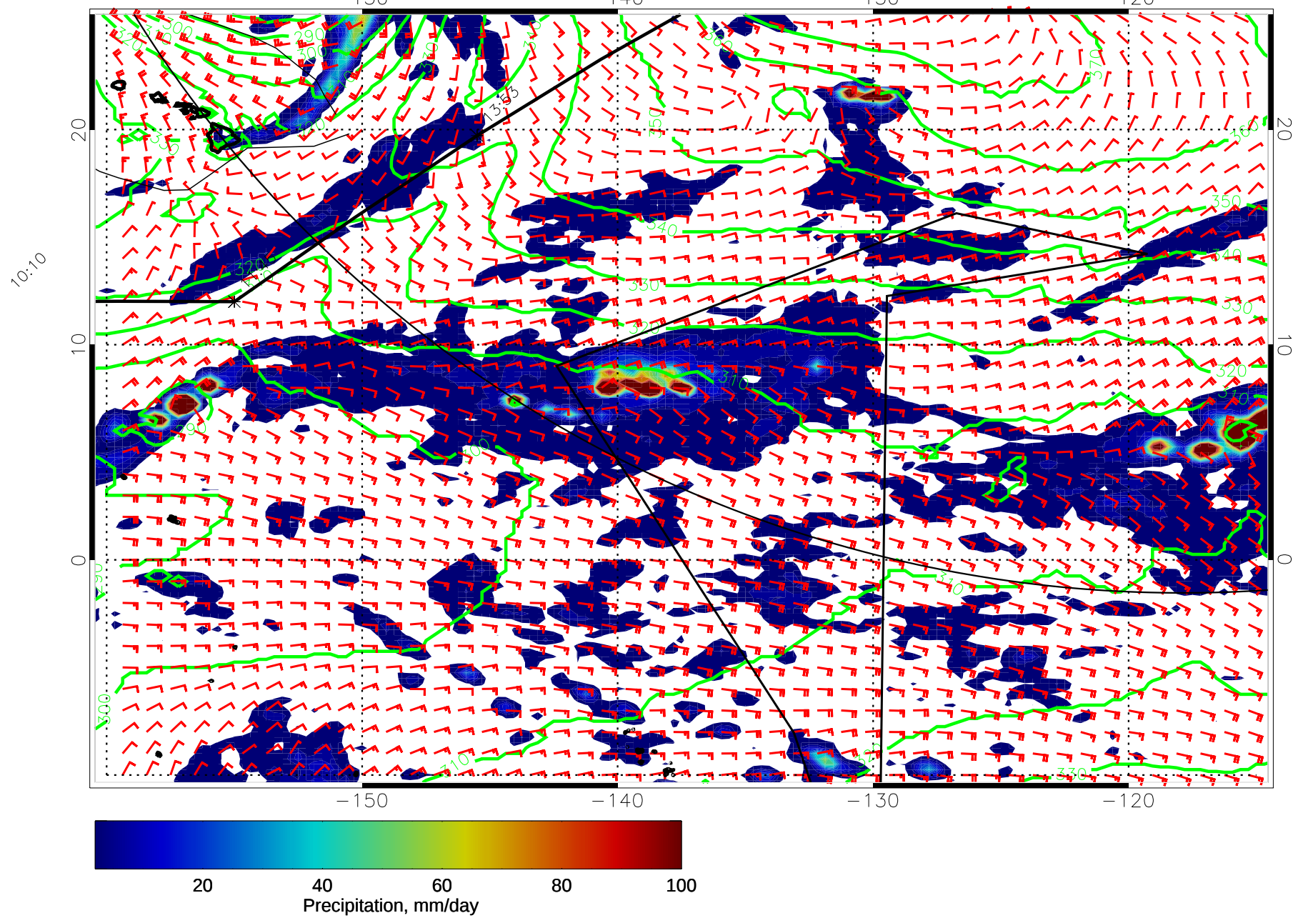
14123112, 60 hour forecast for 975mb Z, Precip., and Surface Winds (knots) -- NASA GEOS5
