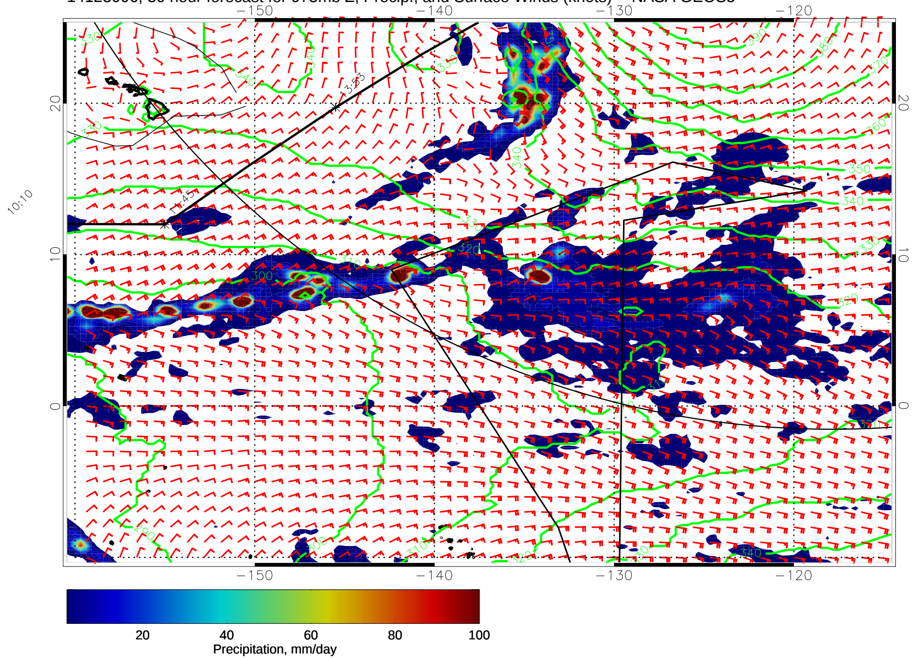
14123006, 30 hour forecast for 975mb Z, Precip., and Surface Winds (knots) -- NASA GEOS5
