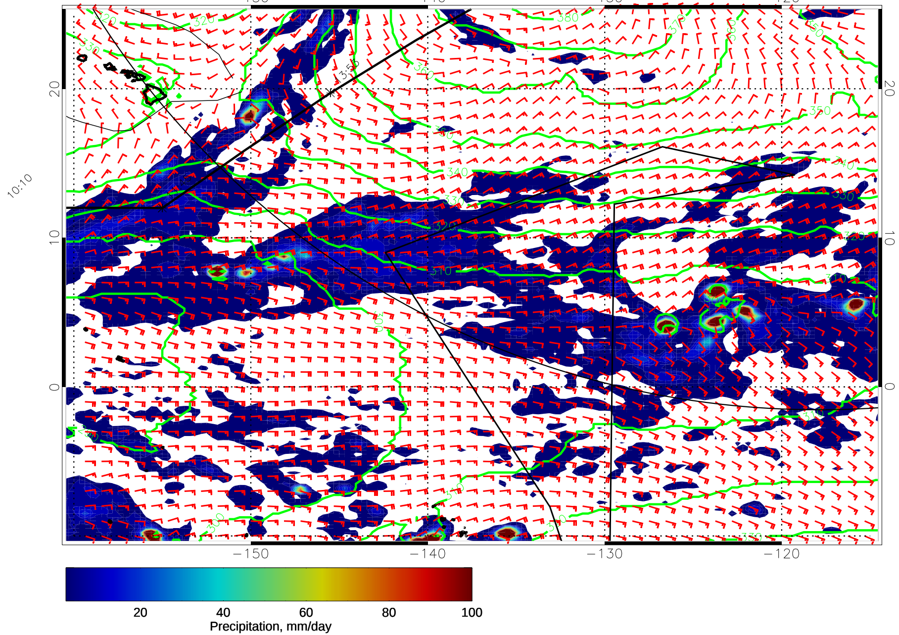
15010112, 84 hour forecast for 975mb Z, Precip., and Surface Winds (knots) -- NASA GEOS5
