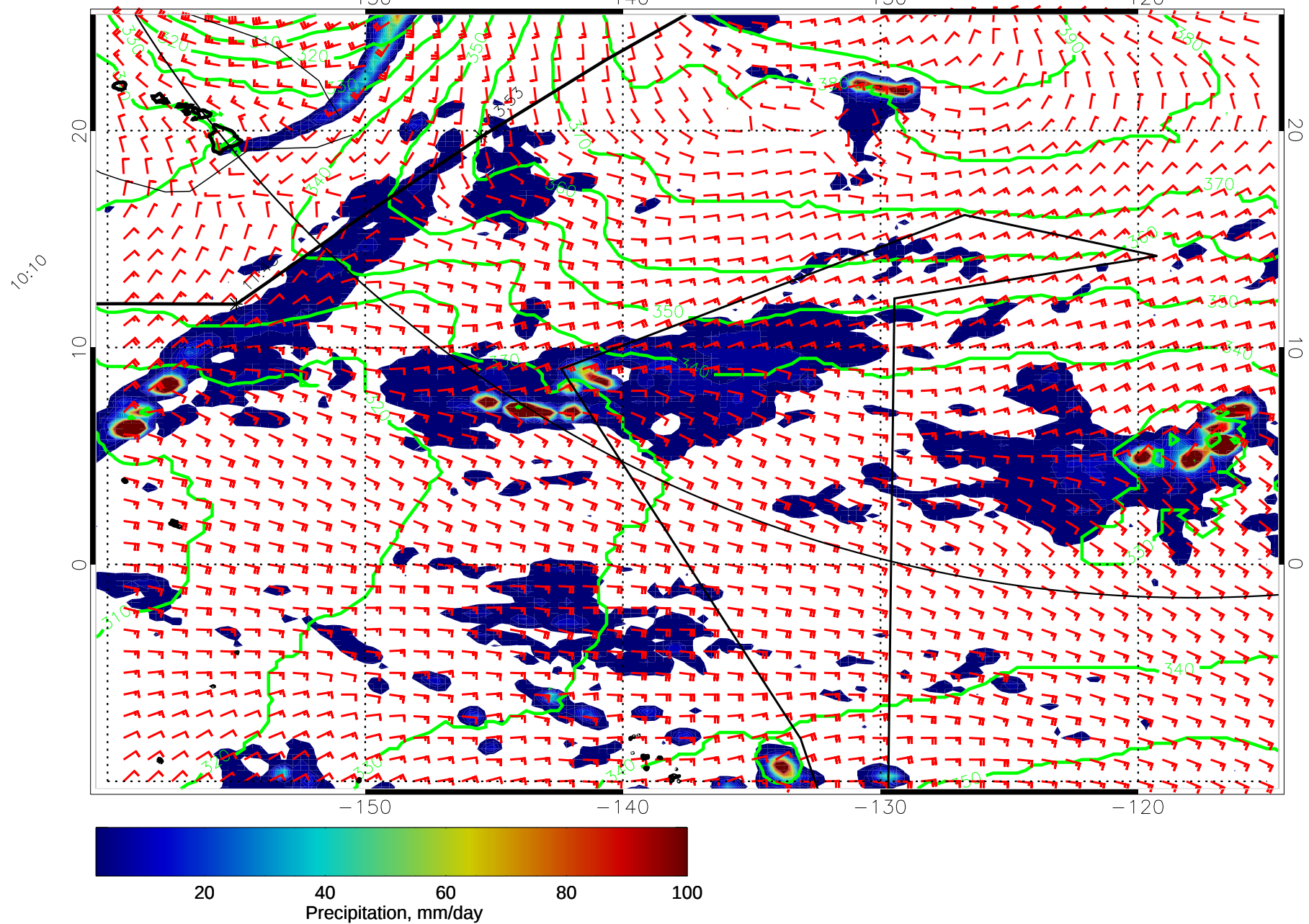
14123118, 66 hour forecast for 975mb Z, Precip., and Surface Winds (knots) -- NASA GEOS5
