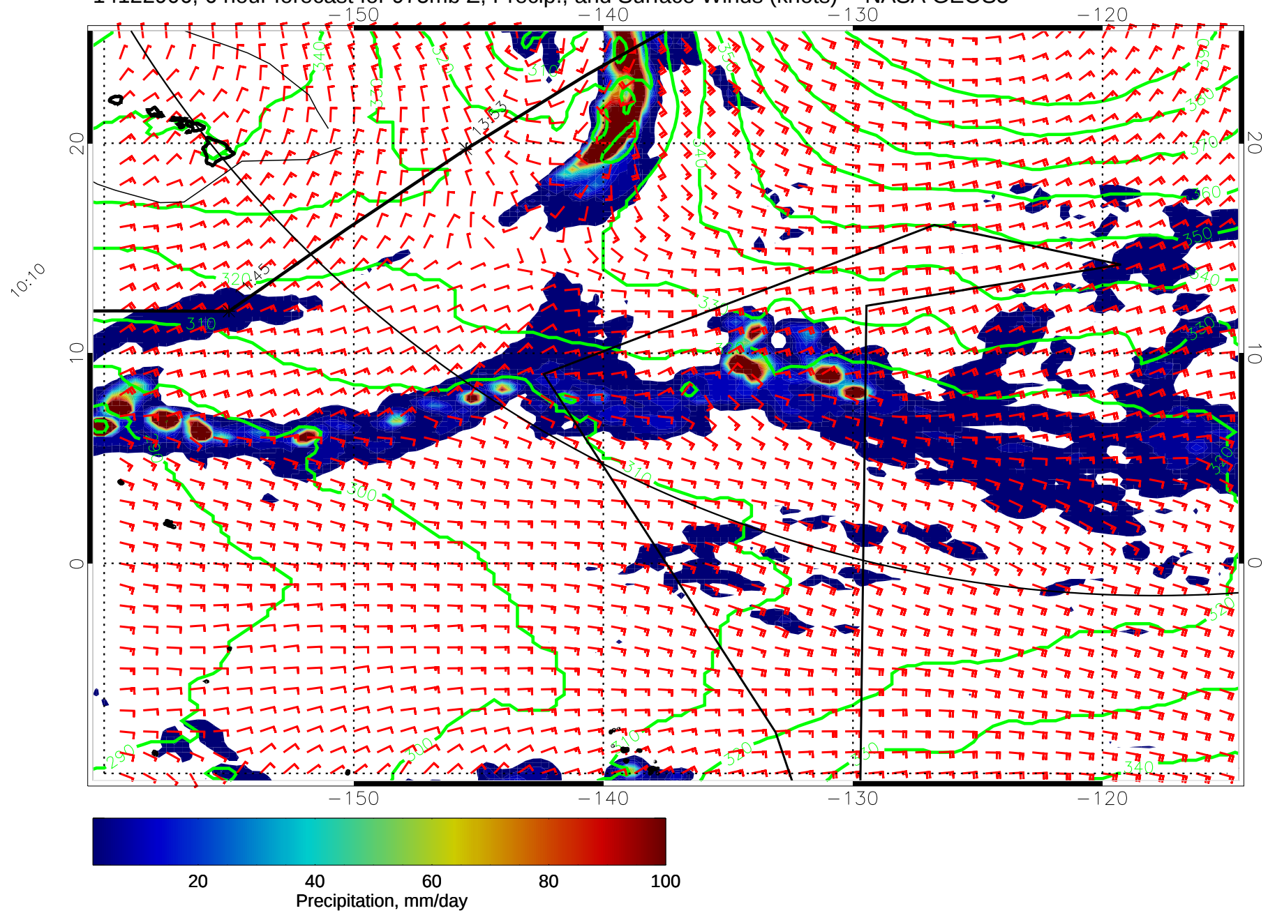
14122906, 6 hour forecast for 975mb Z, Precip., and Surface Winds (knots) -- NASA GEOS5
