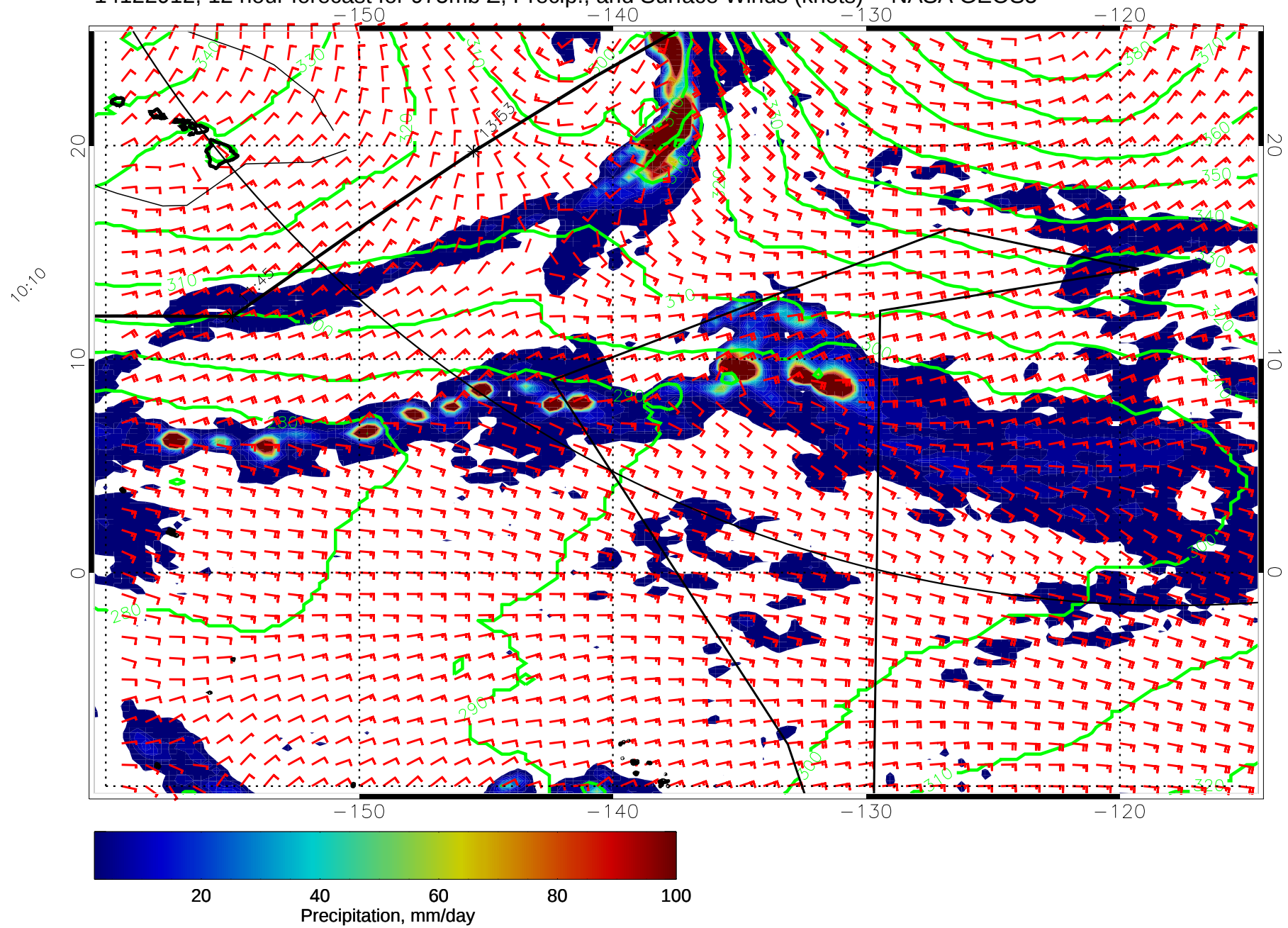
14122912, 12 hour forecast for 975mb Z, Precip., and Surface Winds (knots) -- NASA GEOS5
