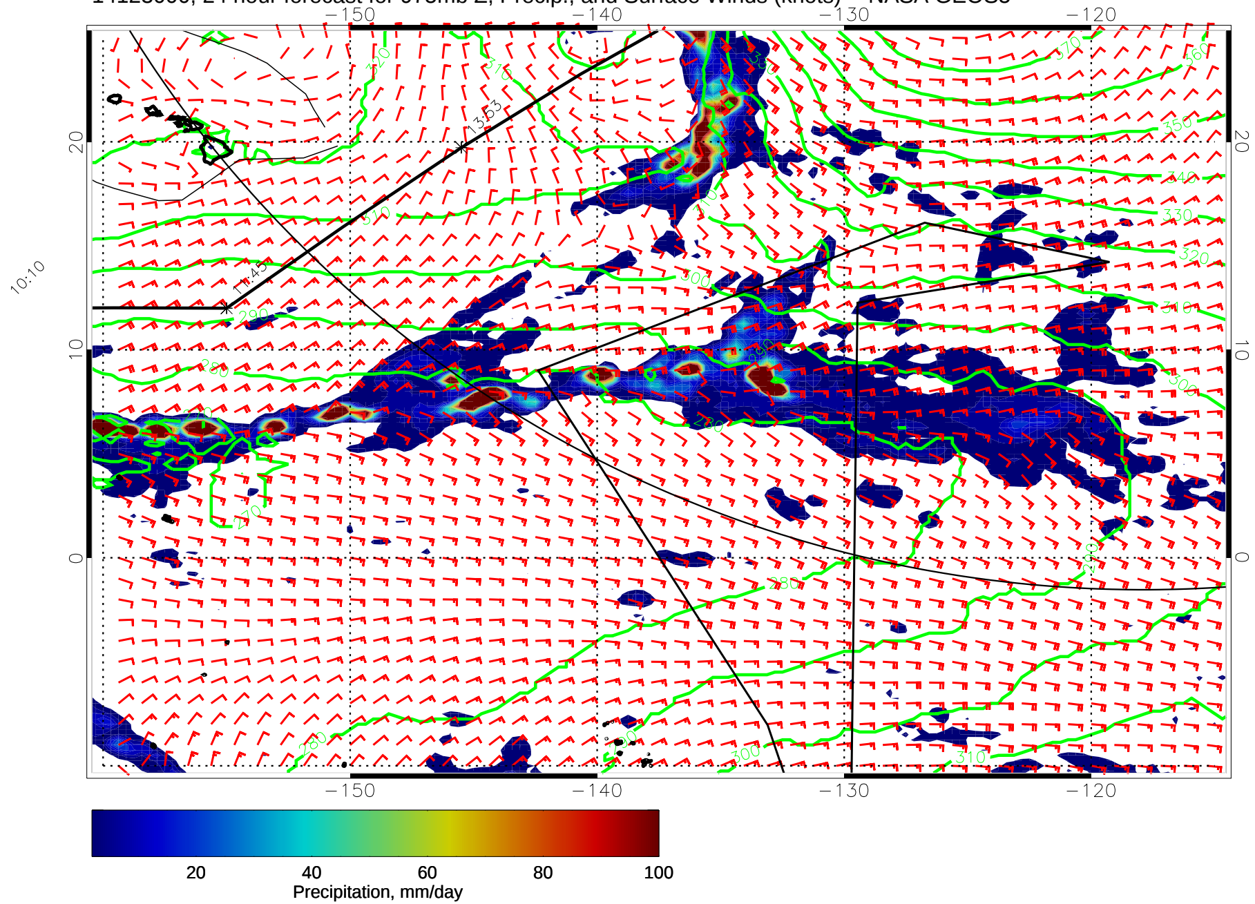
14123000, 24 hour forecast for 975mb Z, Precip., and Surface Winds (knots) -- NASA GEOS5
