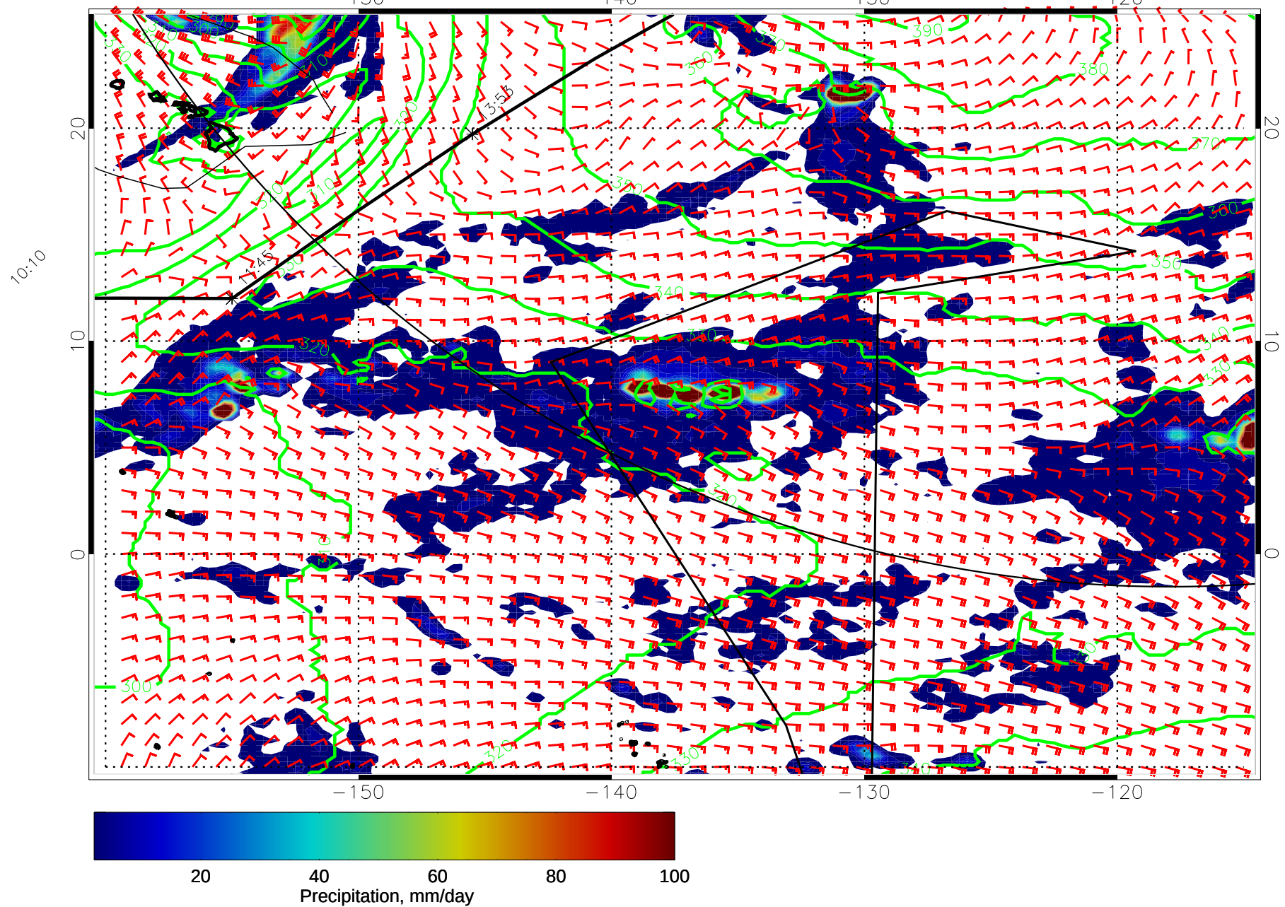
14123106, 54 hour forecast for 975mb Z, Precip., and Surface Winds (knots) -- NASA GEOS5
