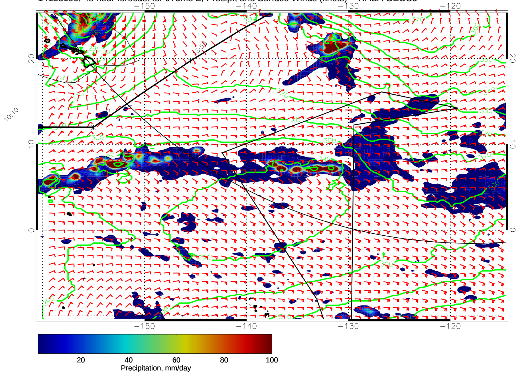
14123100, 48 hour forecast for 975mb Z, Precip., and Surface Winds (knots) -- NASA GEOS5
