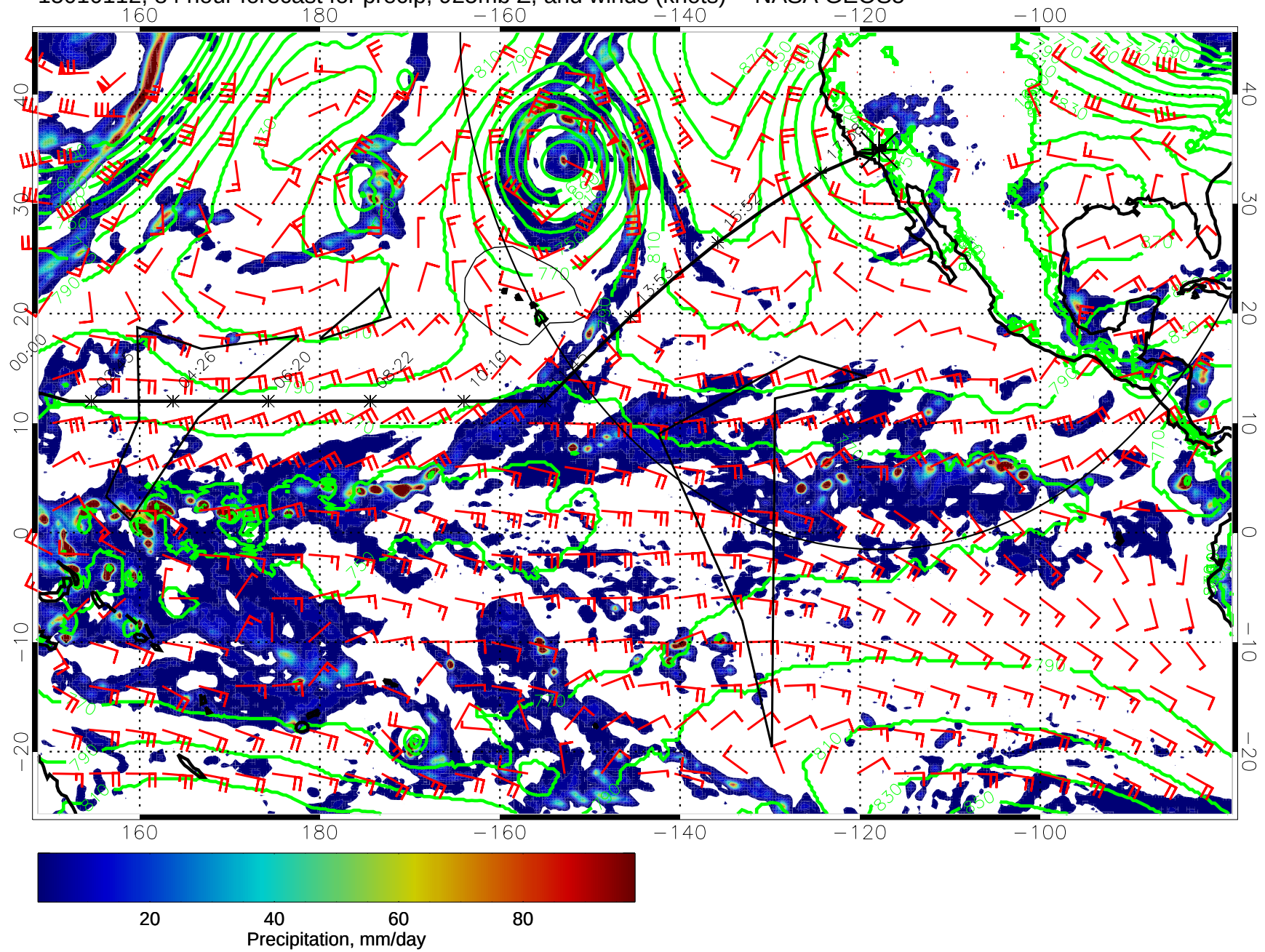
15010112, 84 hour forecast for precip, 925mb Z, and winds (knots) -- NASA GEOS5
