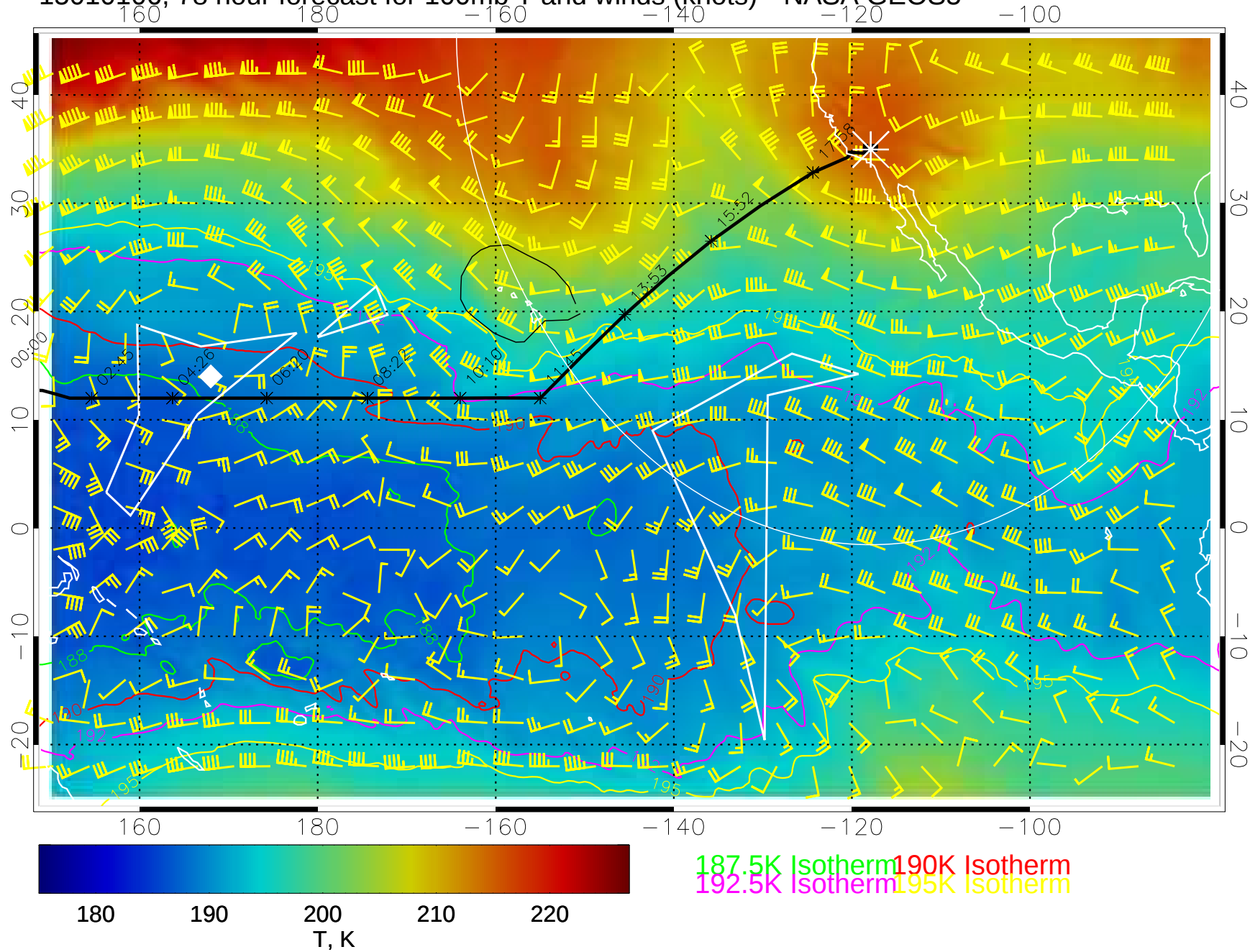
15010106, 78 hour forecast for 100mb T and winds (knots)-- NASA GEOS5
