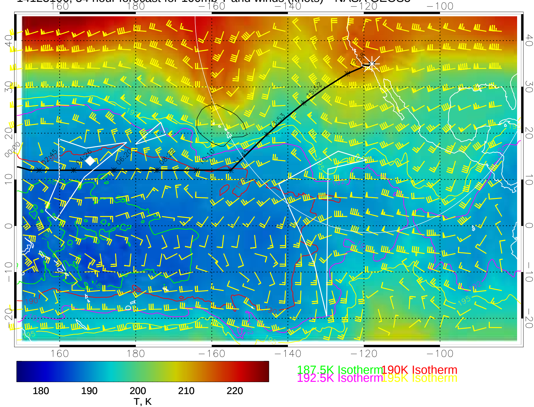
14123106, 54 hour forecast for 100mb T and winds (knots)-- NASA GEOS5
