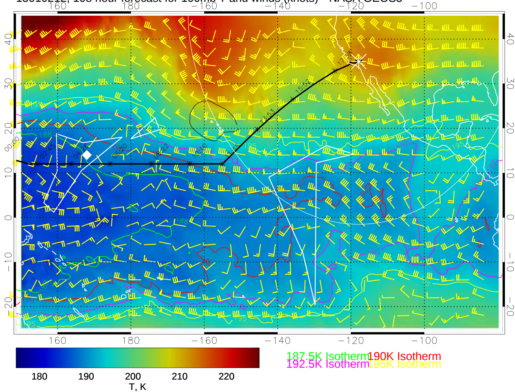
15010212, 108 hour forecast for 100mb T and winds (knots)-- NASA GEOS5
