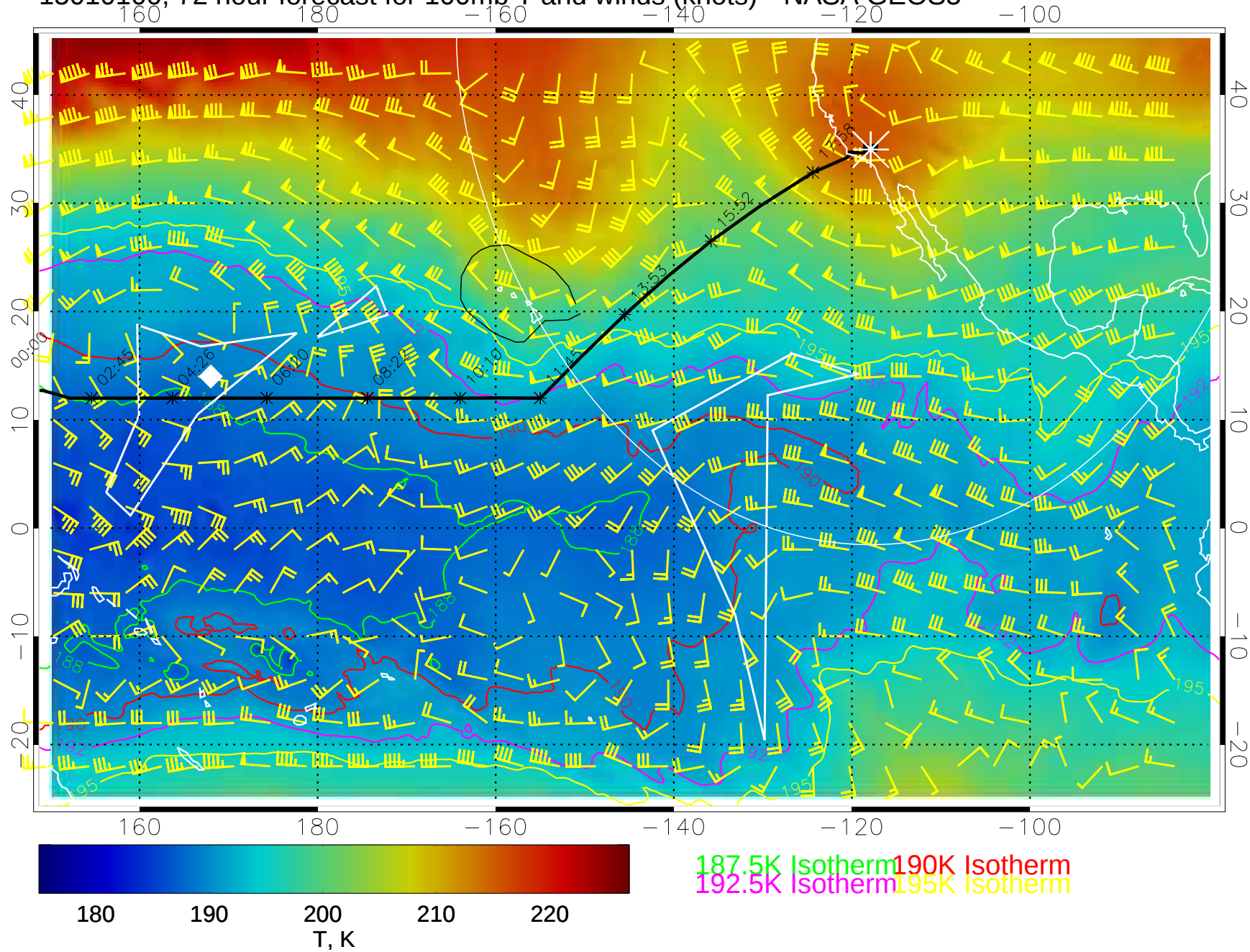
15010100, 72 hour forecast for 100mb T and winds (knots)-- NASA GEOS5
