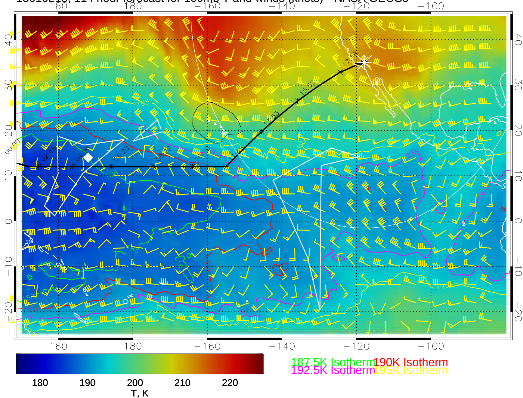
15010218, 114 hour forecast for 100mb T and winds (knots)-- NASA GEOS5
