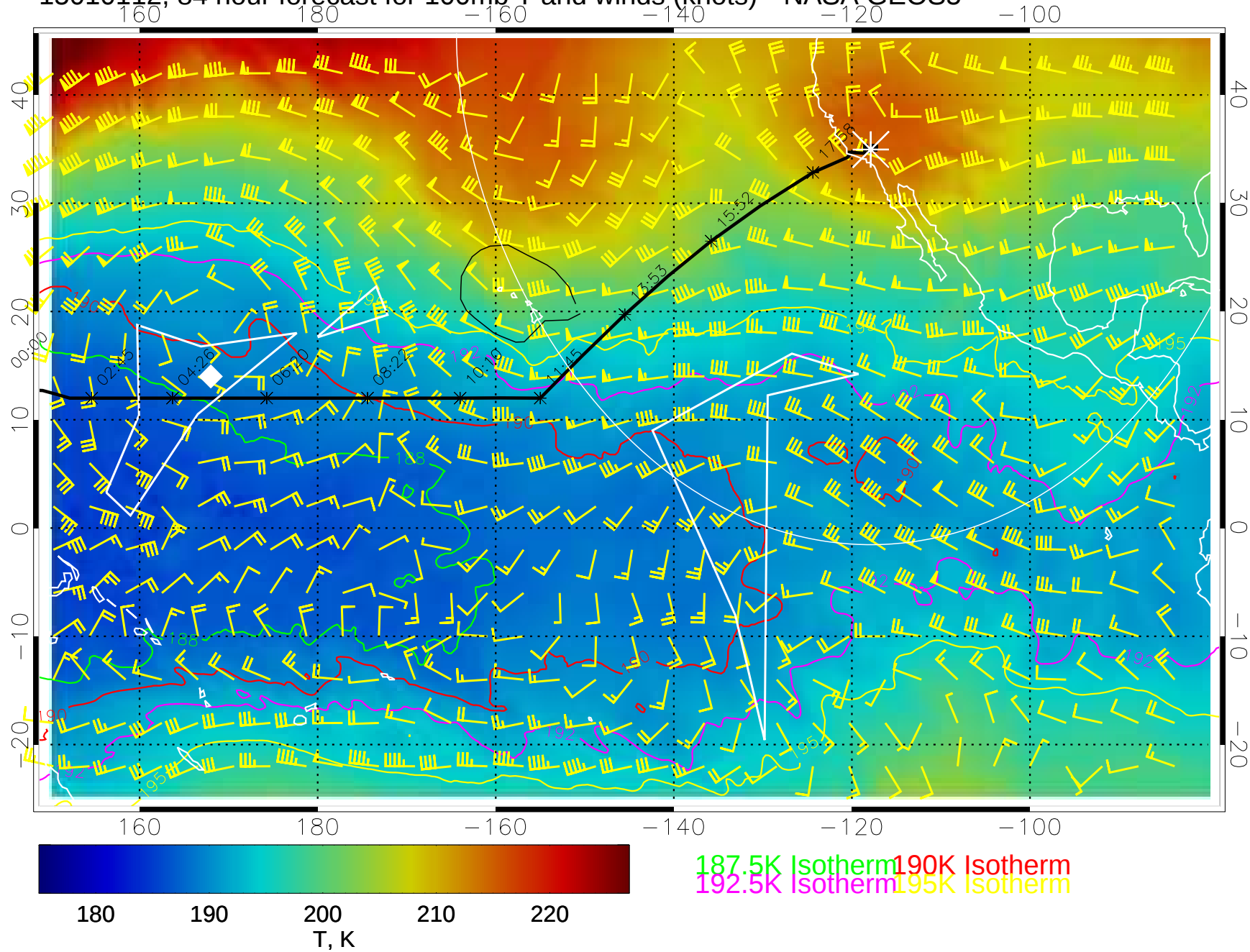
15010112, 84 hour forecast for 100mb T and winds (knots)-- NASA GEOS5
