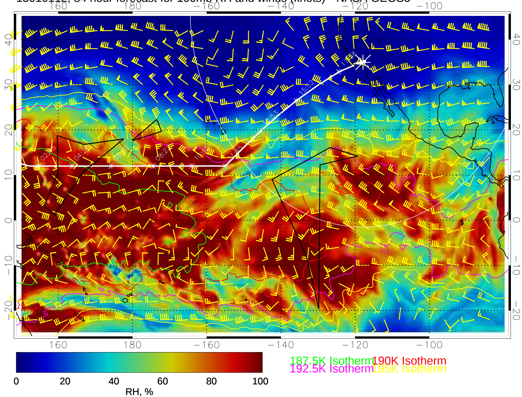
15010112, 84 hour forecast for 100mb RH and winds (knots)-- NASA GEOS5
