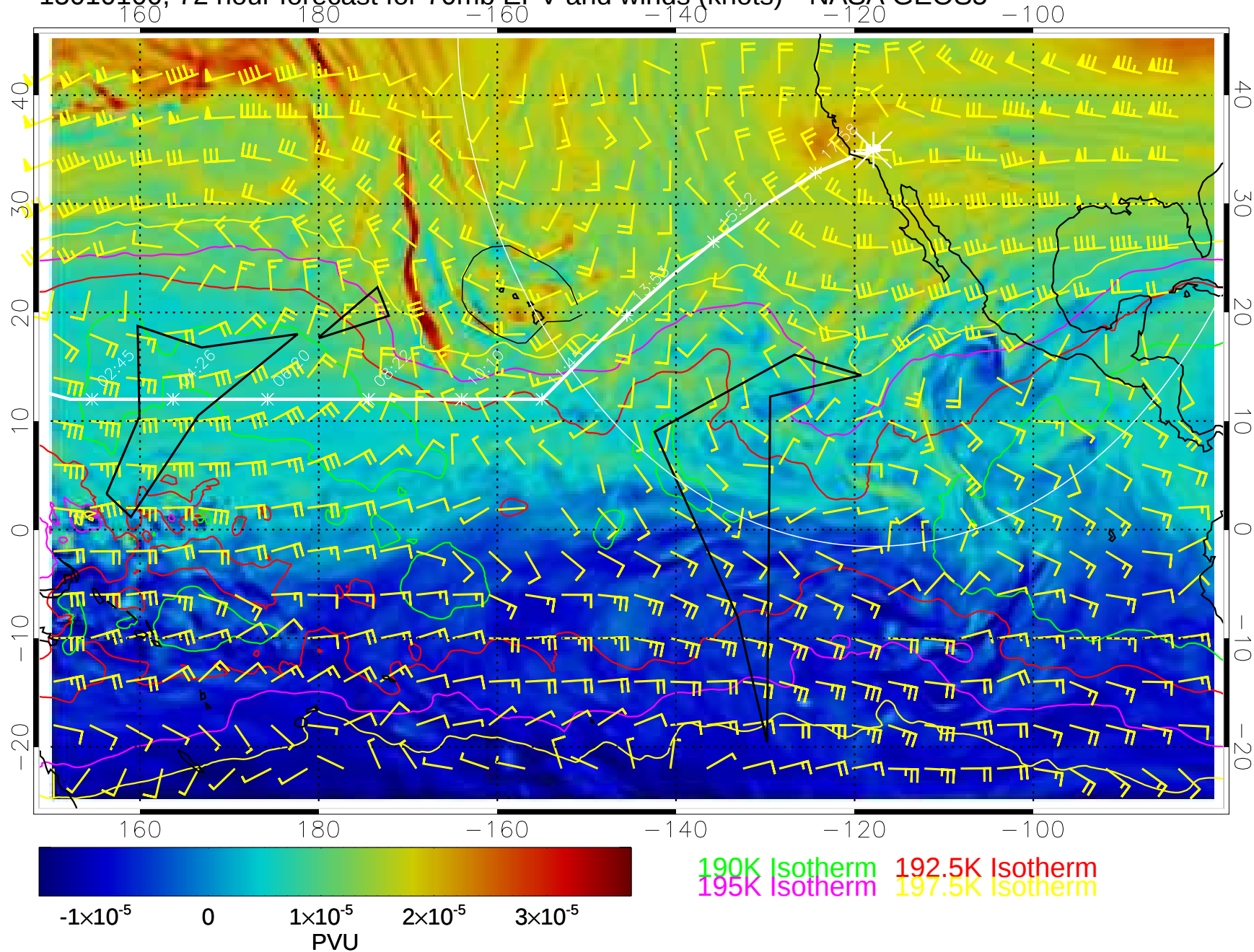
15010100, 72 hour forecast for 70mb EPV and winds (knots)-- NASA GEOS5
