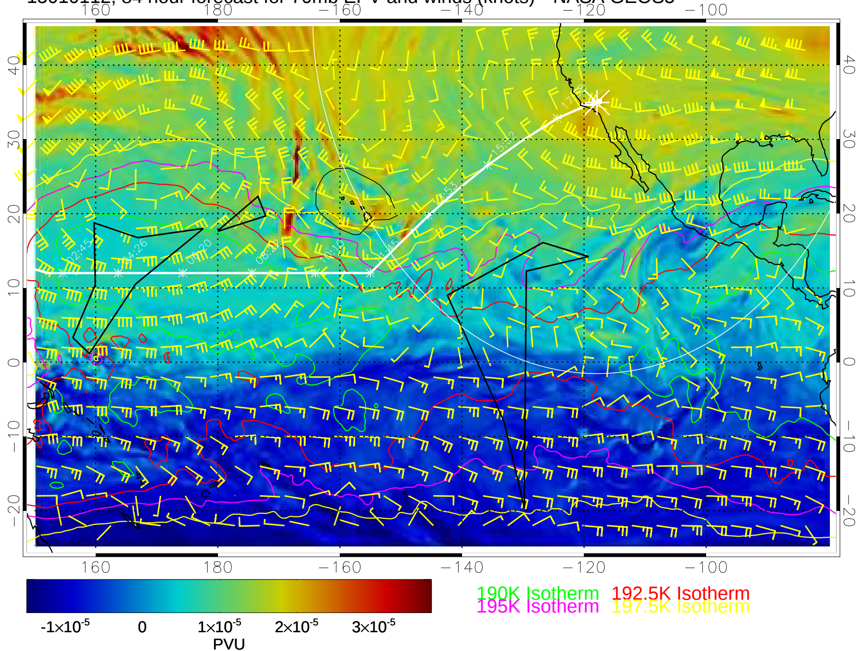
15010112, 84 hour forecast for 70mb EPV and winds (knots)-- NASA GEOS5
