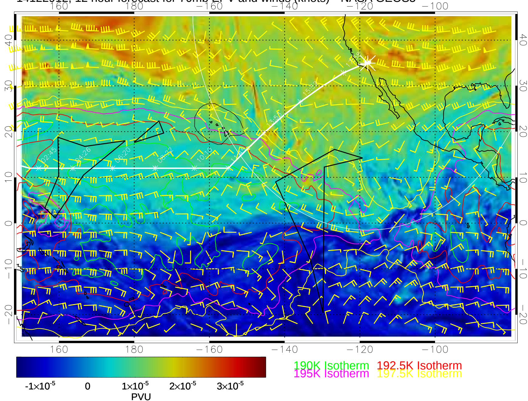
14122912, 12 hour forecast for 70mb EPV and winds (knots)-- NASA GEOS5
