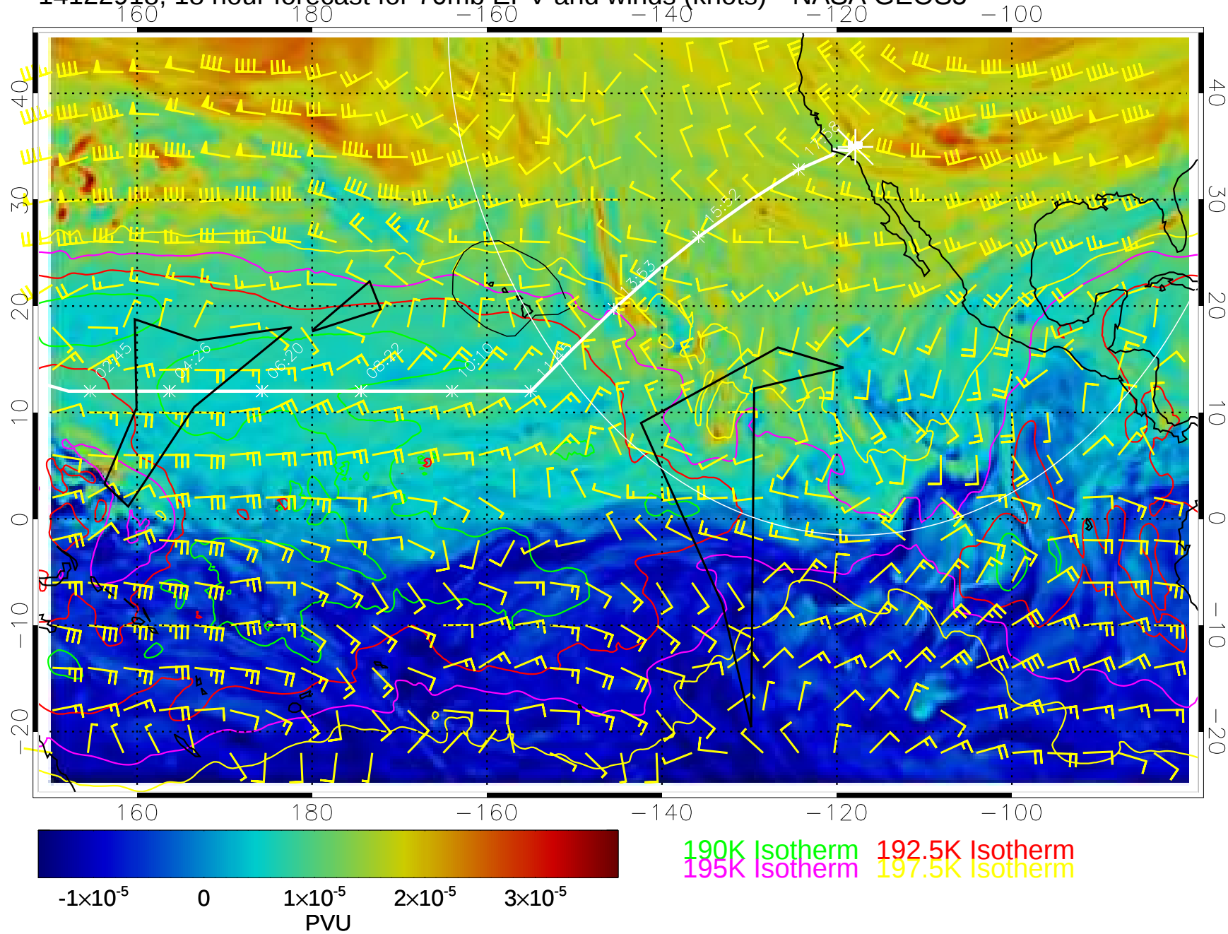
14122918, 18 hour forecast for 70mb EPV and winds (knots)-- NASA GEOS5
