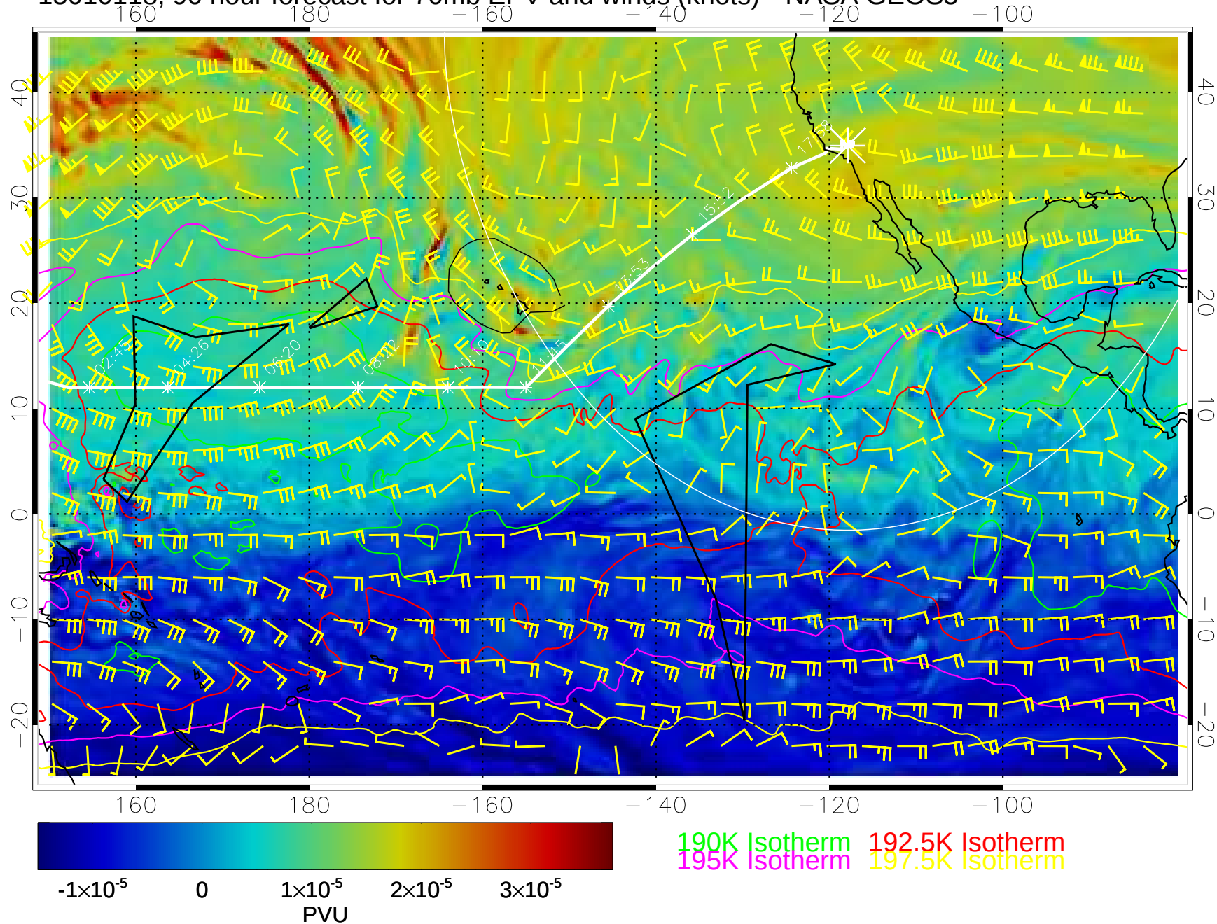
15010118, 90 hour forecast for 70mb EPV and winds (knots)-- NASA GEOS5
