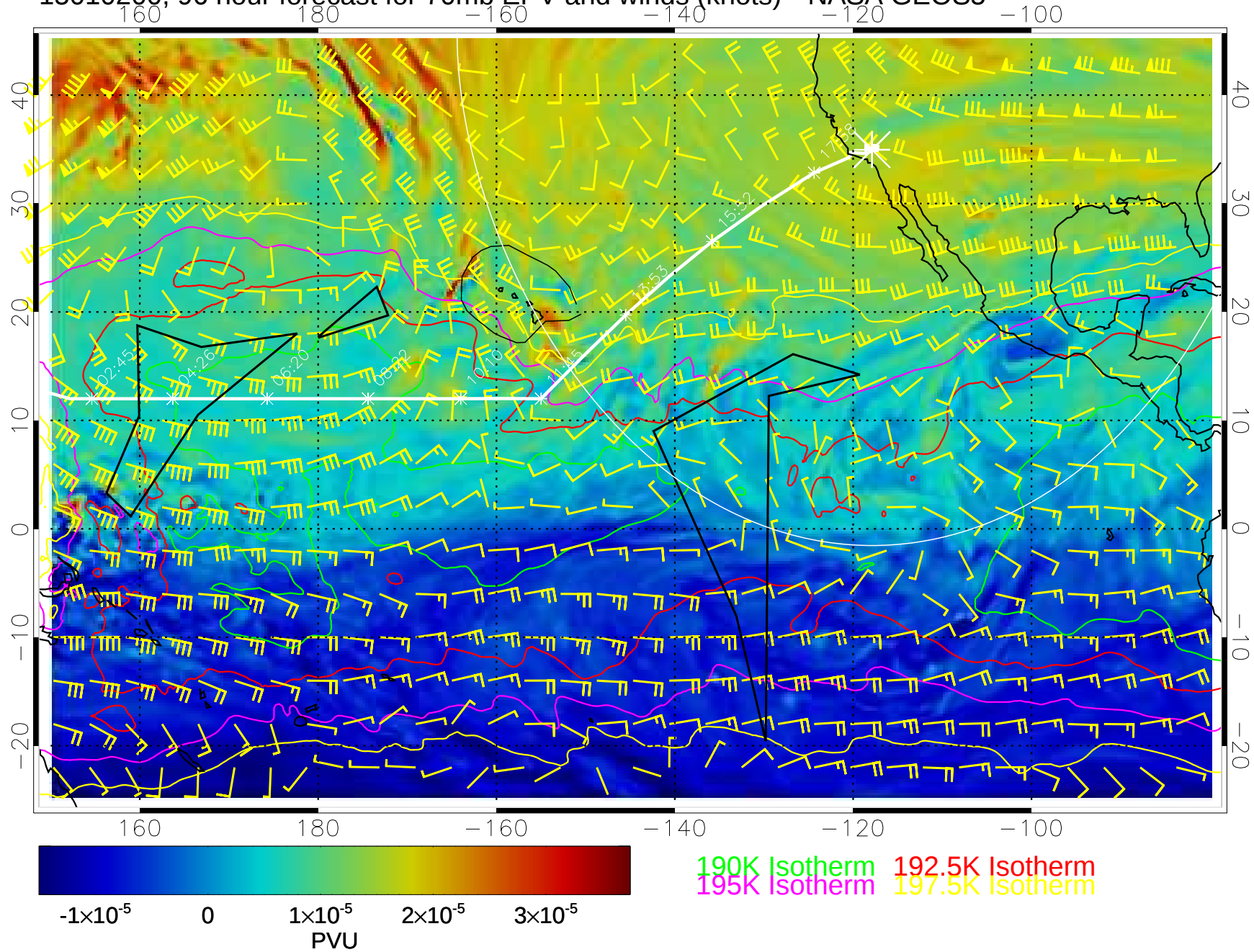
15010200, 96 hour forecast for 70mb EPV and winds (knots)-- NASA GEOS5
