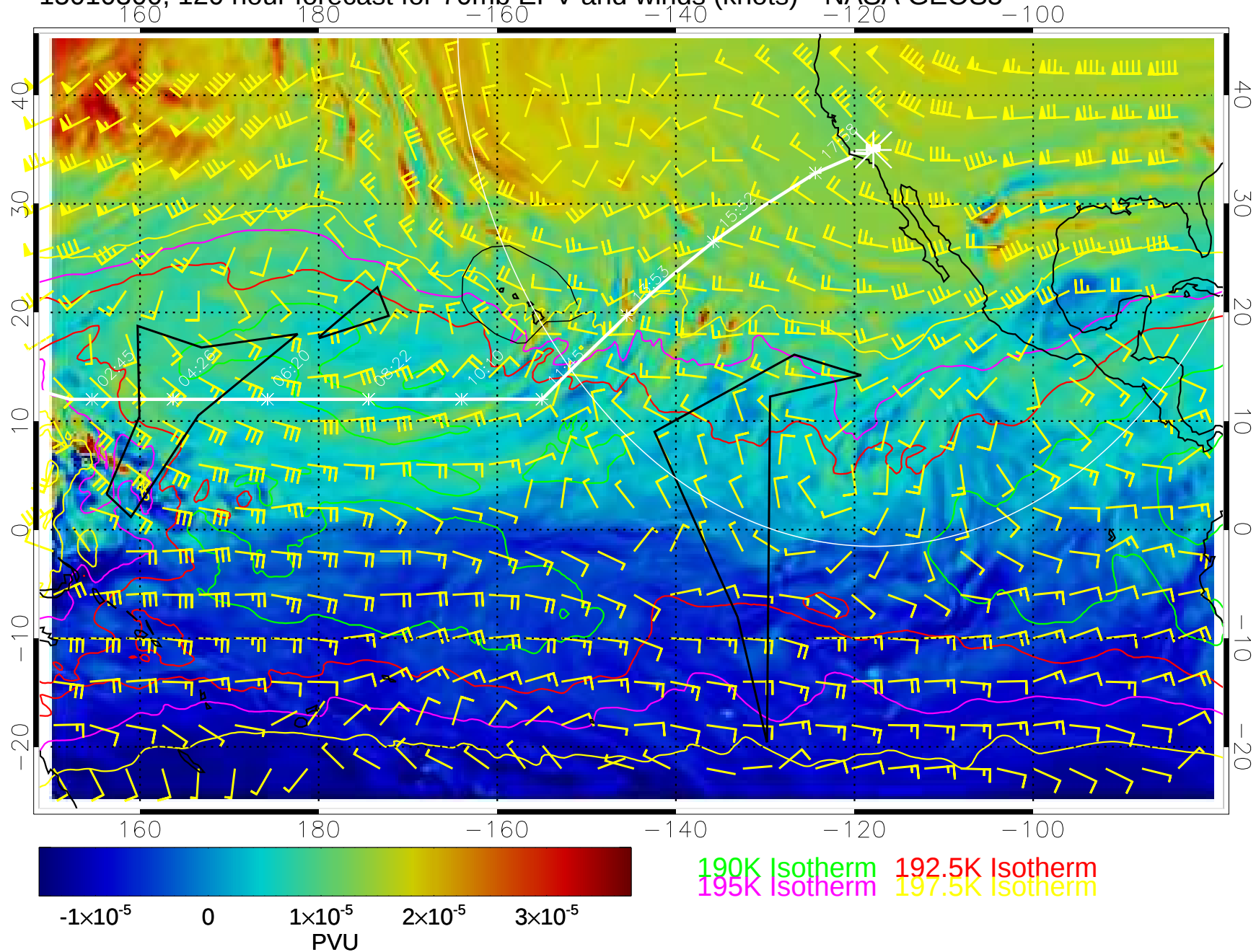
15010300, 120 hour forecast for 70mb EPV and winds (knots)-- NASA GEOS5
