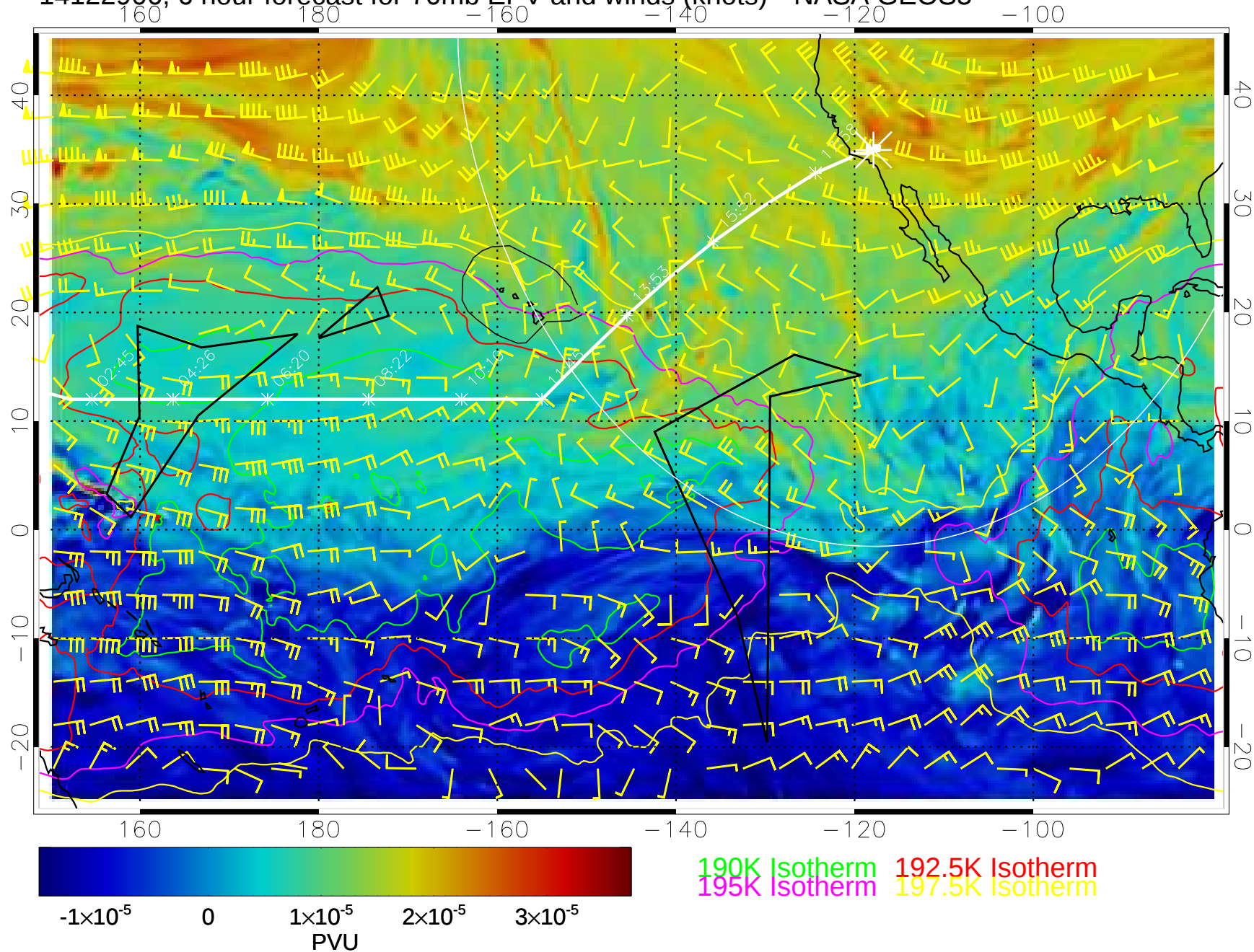
14122906, 6 hour forecast for 70mb EPV and winds (knots)-- NASA GEOS5
