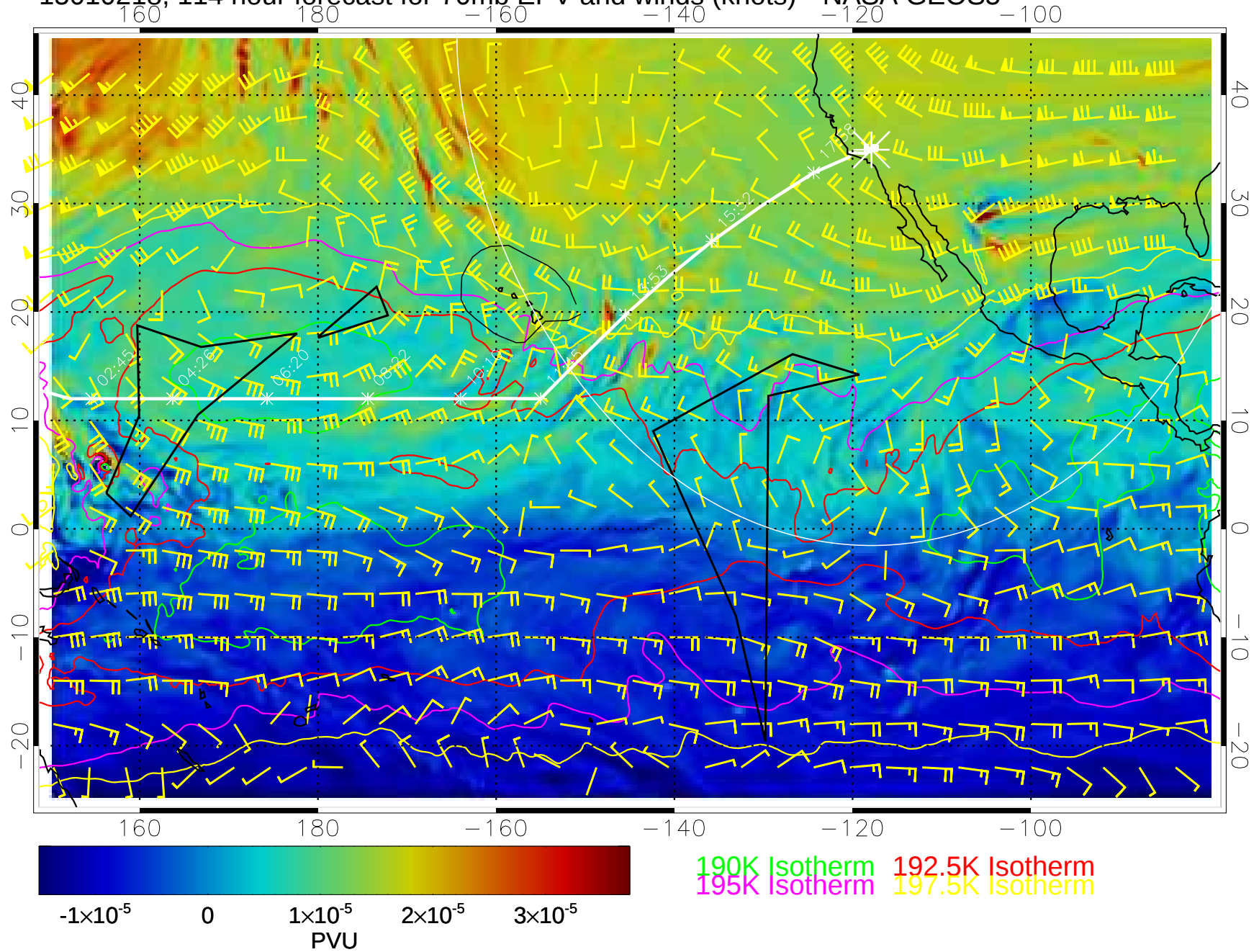
15010218, 114 hour forecast for 70mb EPV and winds (knots)-- NASA GEOS5
