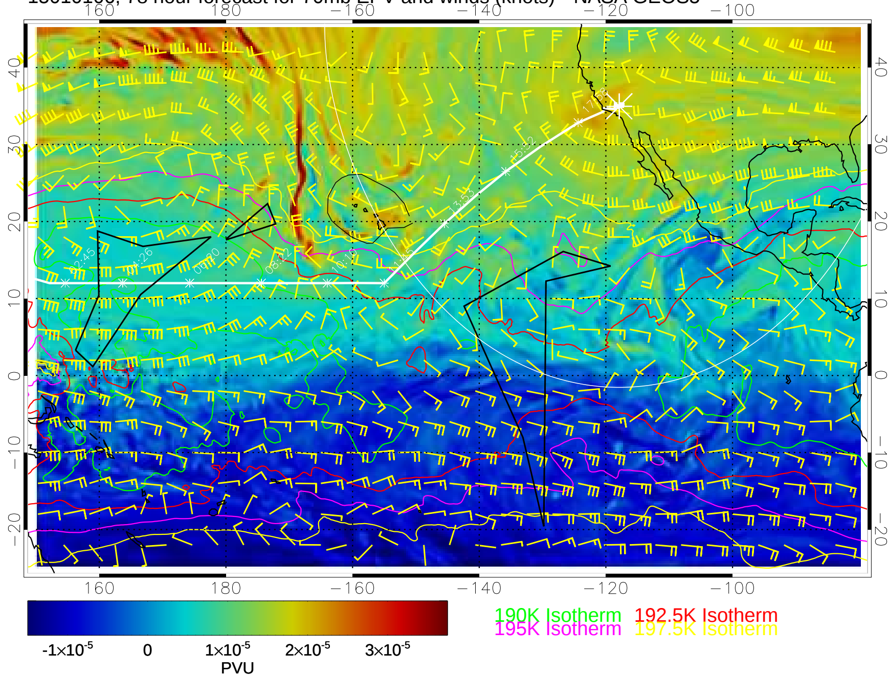
15010106, 78 hour forecast for 70mb EPV and winds (knots)-- NASA GEOS5
