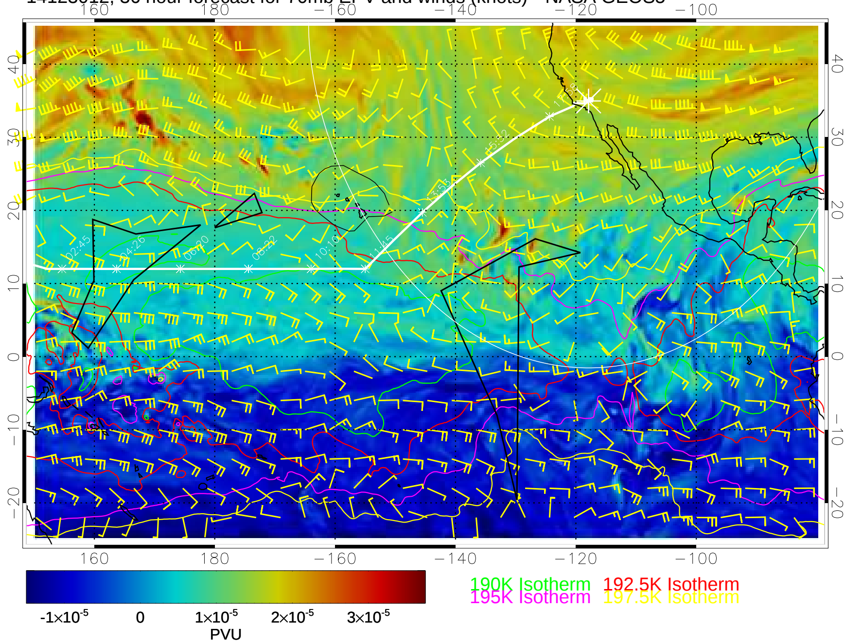
14123012, 36 hour forecast for 70mb EPV and winds (knots)-- NASA GEOS5
