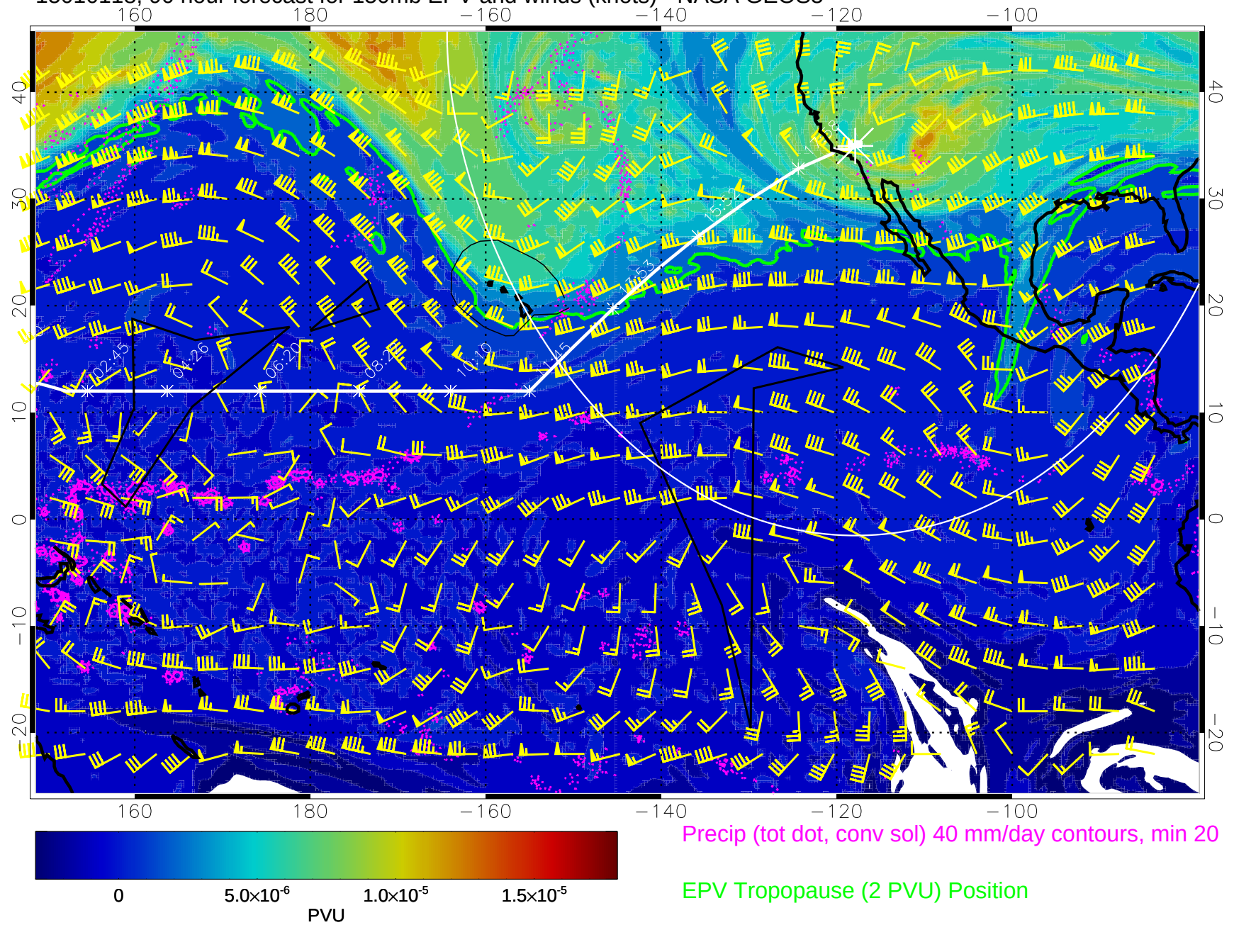
15010118, 90 hour forecast for 150mb EPV and winds (knots) - NASA GEOS5
