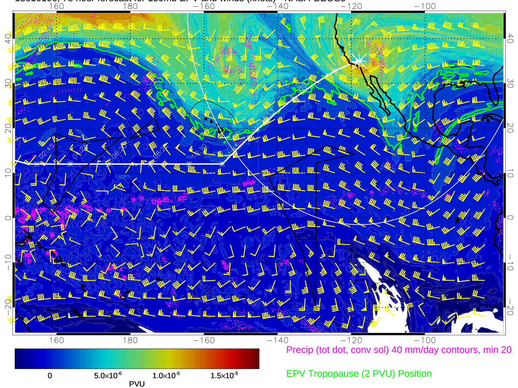
15010106, 78 hour forecast for 150mb EPV and winds (knots) - NASA GEOS5
