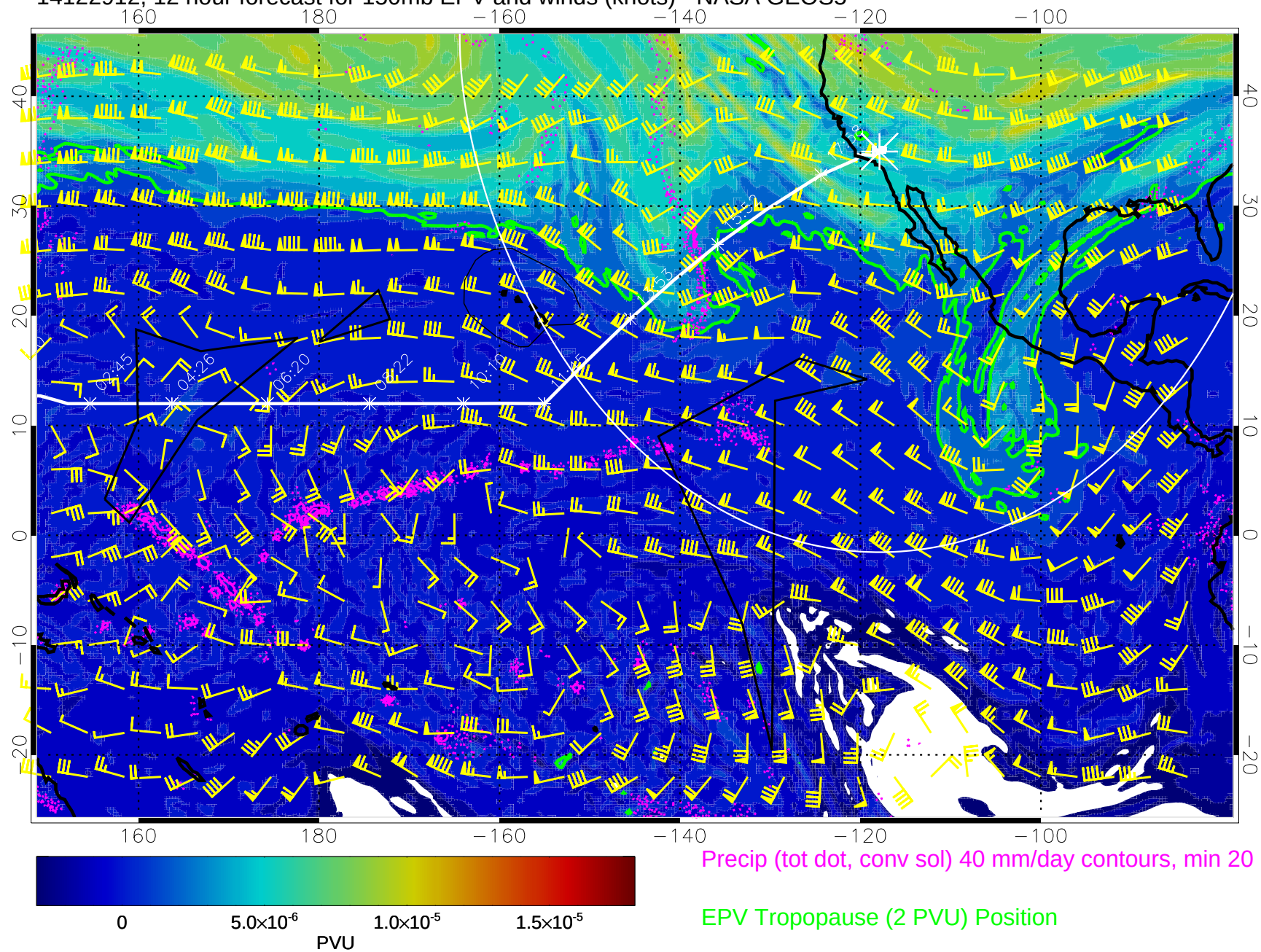
14122912, 12 hour forecast for 150mb EPV and winds (knots) - NASA GEOS5
