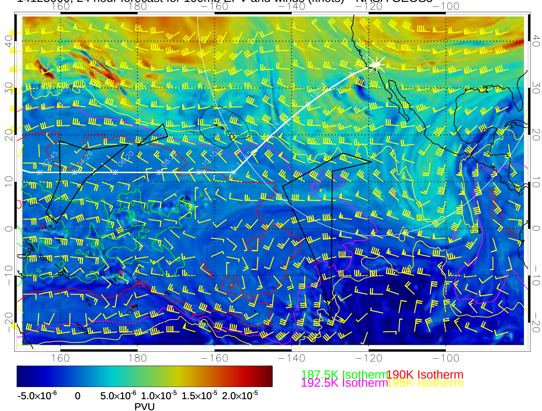
14123000, 24 hour forecast for 100mb EPV and winds (knots)-- NASA GEOS5
