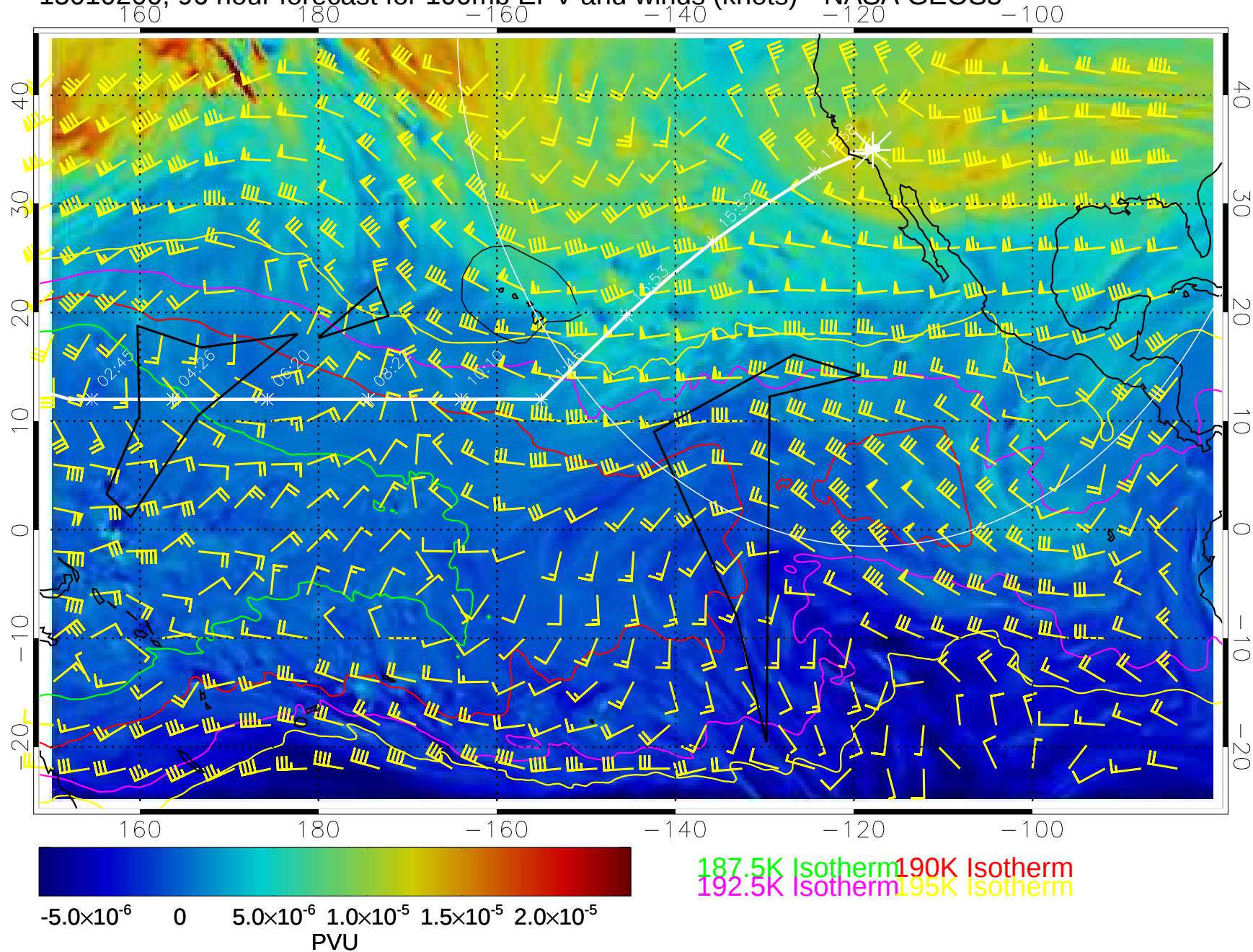
15010200, 96 hour forecast for 100mb EPV and winds (knots)-- NASA GEOS5
