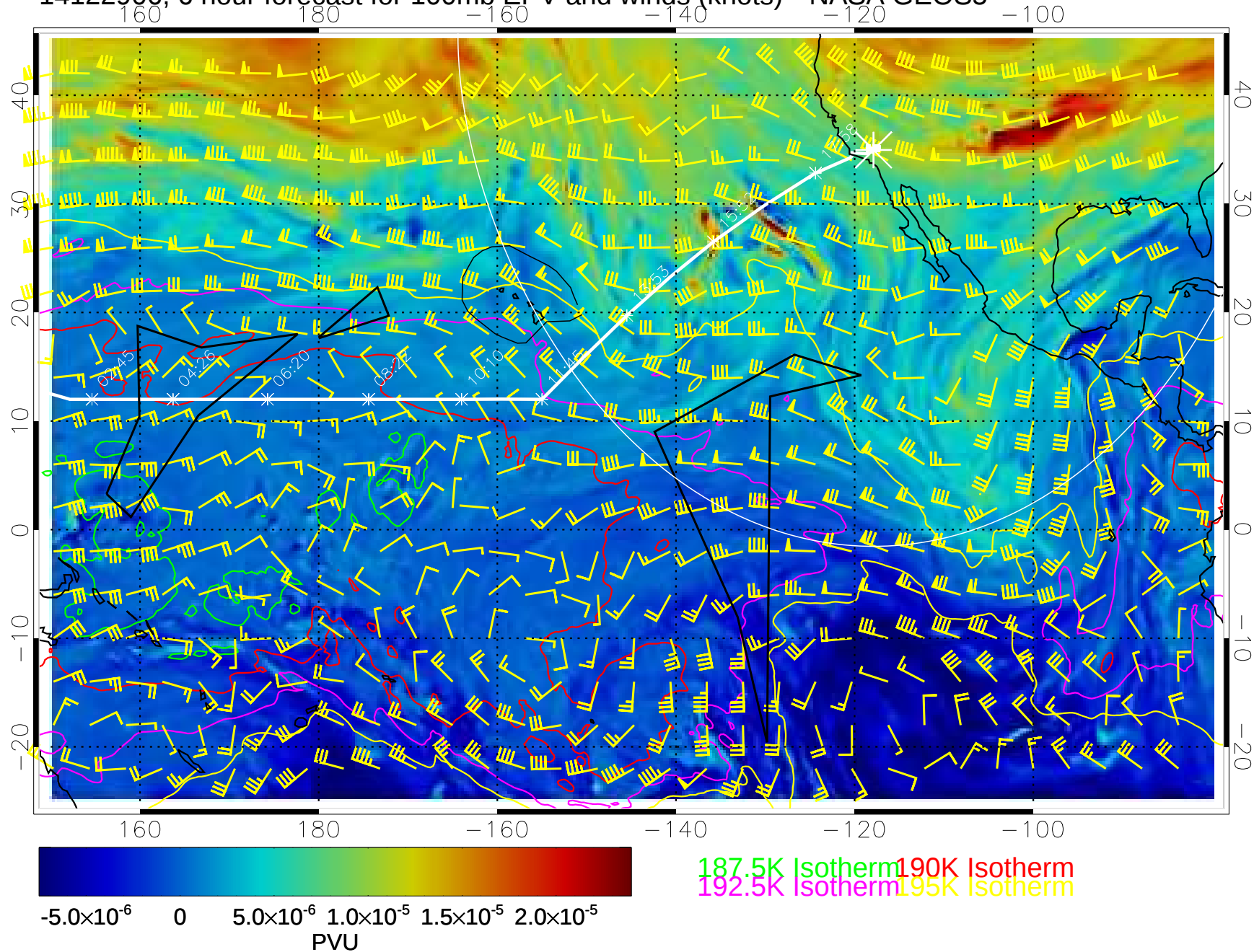
14122906, 6 hour forecast for 100mb EPV and winds (knots)-- NASA GEOS5
