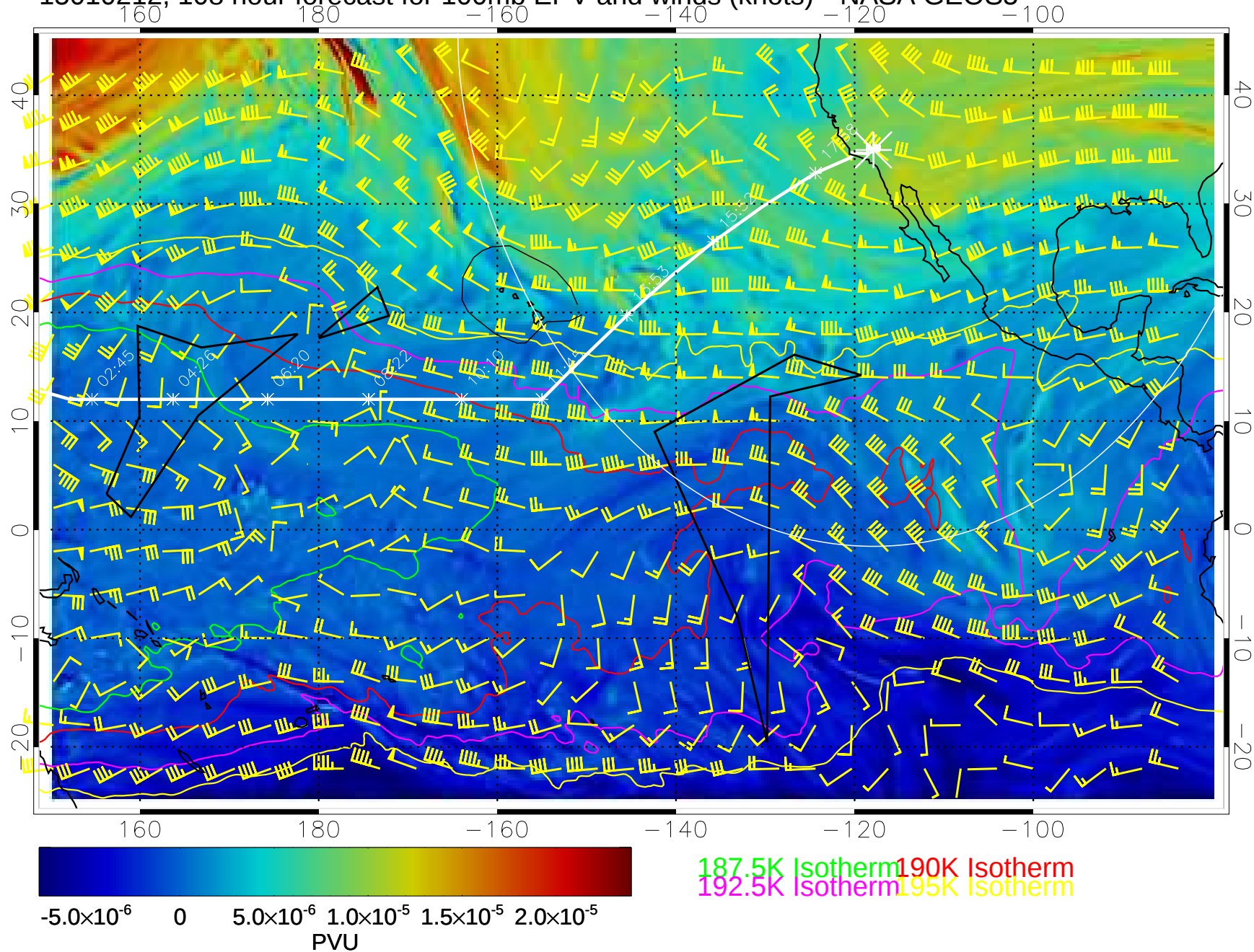
15010212, 108 hour forecast for 100mb EPV and winds (knots)-- NASA GEOS5
