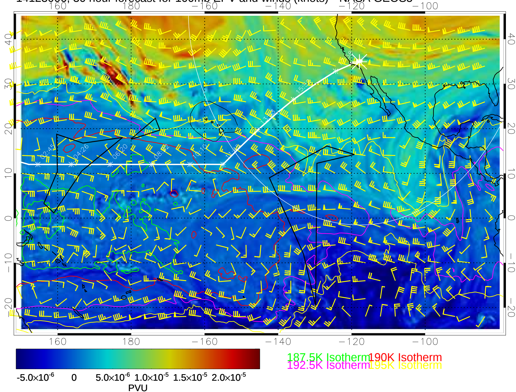
14123006, 30 hour forecast for 100mb EPV and winds (knots)-- NASA GEOS5
