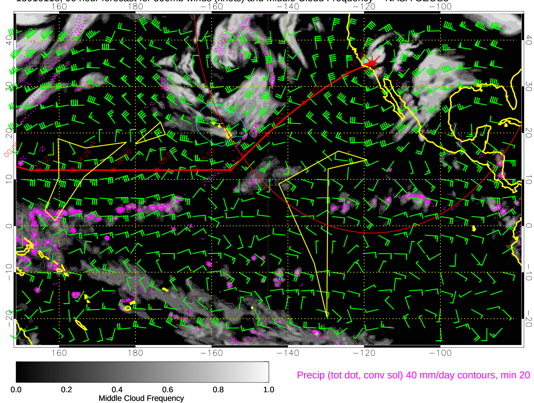
15010118, 90 hour forecast for 500mb winds (knots) and Middle Cloud Frequency -- NASA GEOS5
