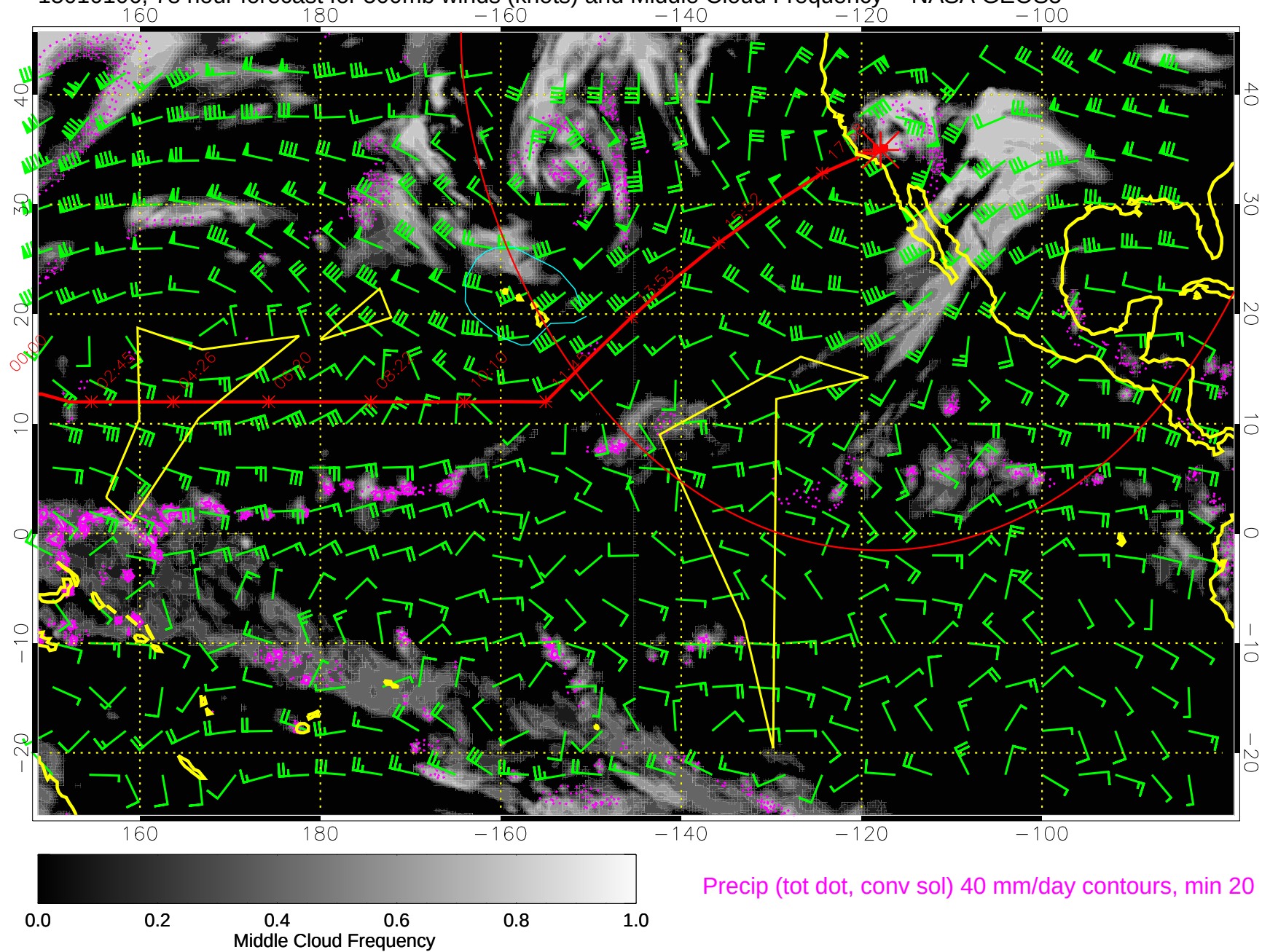
15010106, 78 hour forecast for 500mb winds (knots) and Middle Cloud Frequency -- NASA GEOS5
