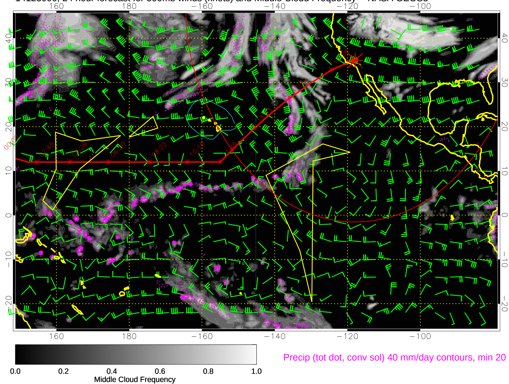
14123000, 24 hour forecast for 500mb winds (knots) and Middle Cloud Frequency -- NASA GEOS5
