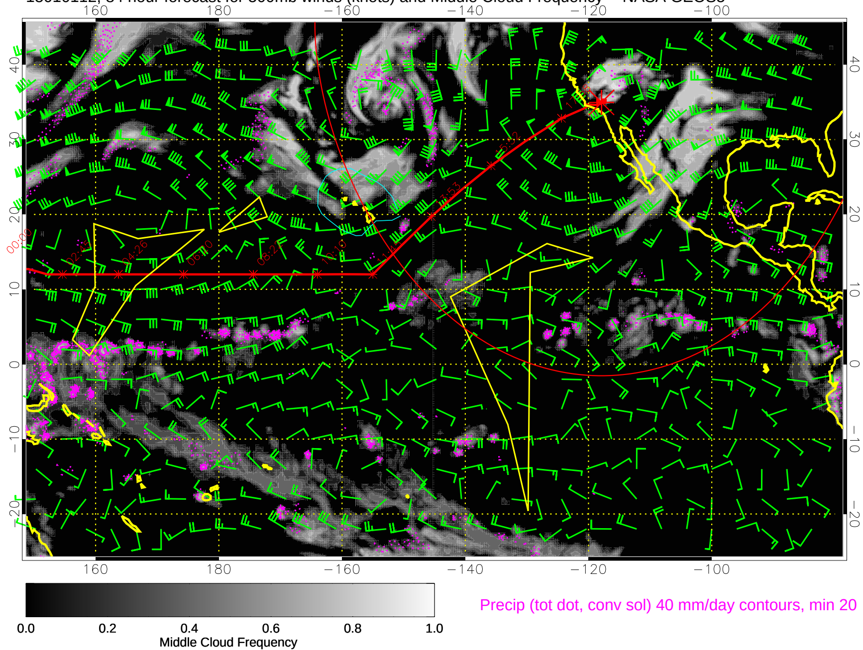
15010112, 84 hour forecast for 500mb winds (knots) and Middle Cloud Frequency -- NASA GEOS5
