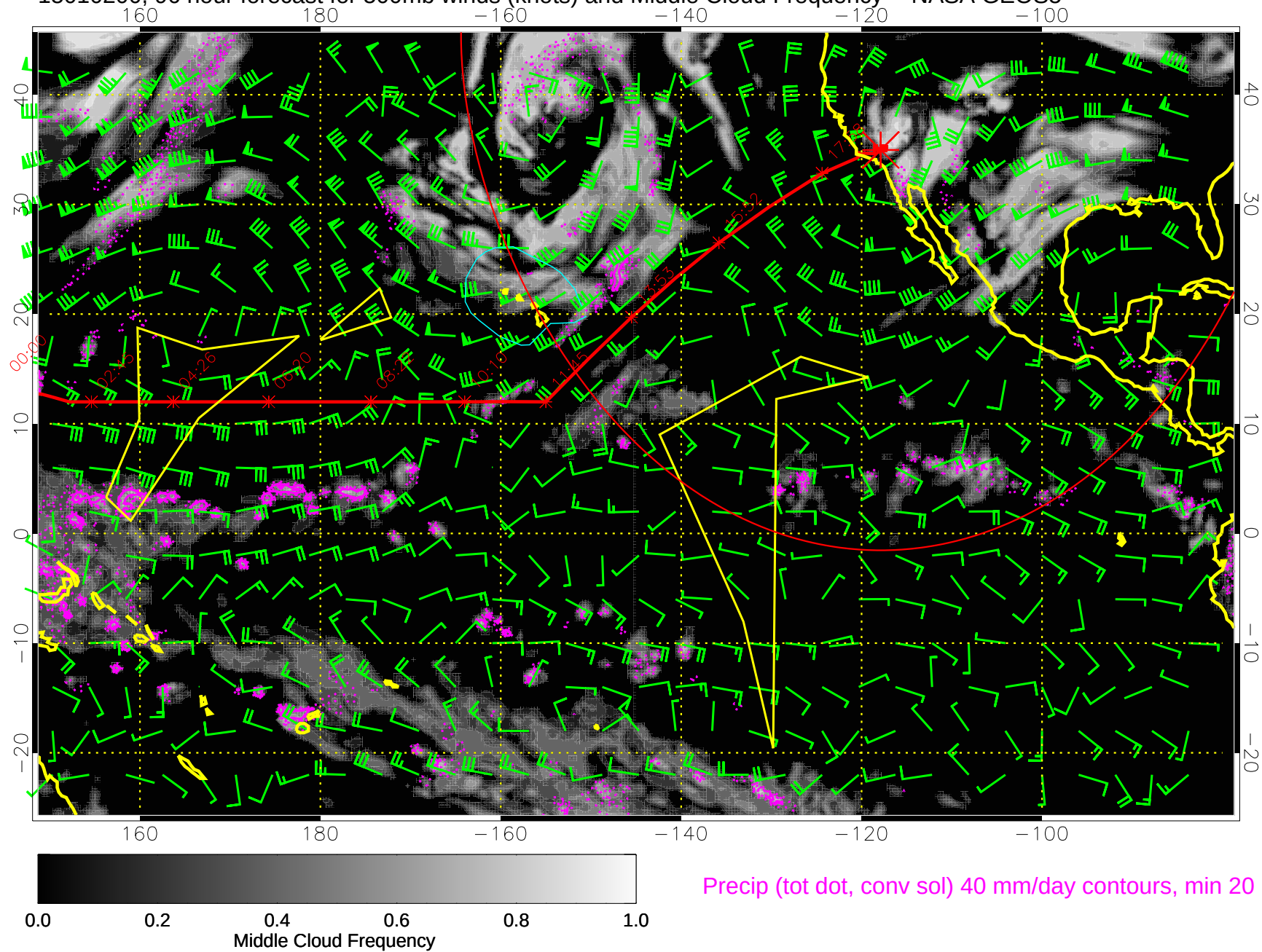
15010200, 96 hour forecast for 500mb winds (knots) and Middle Cloud Frequency -- NASA GEOS5
