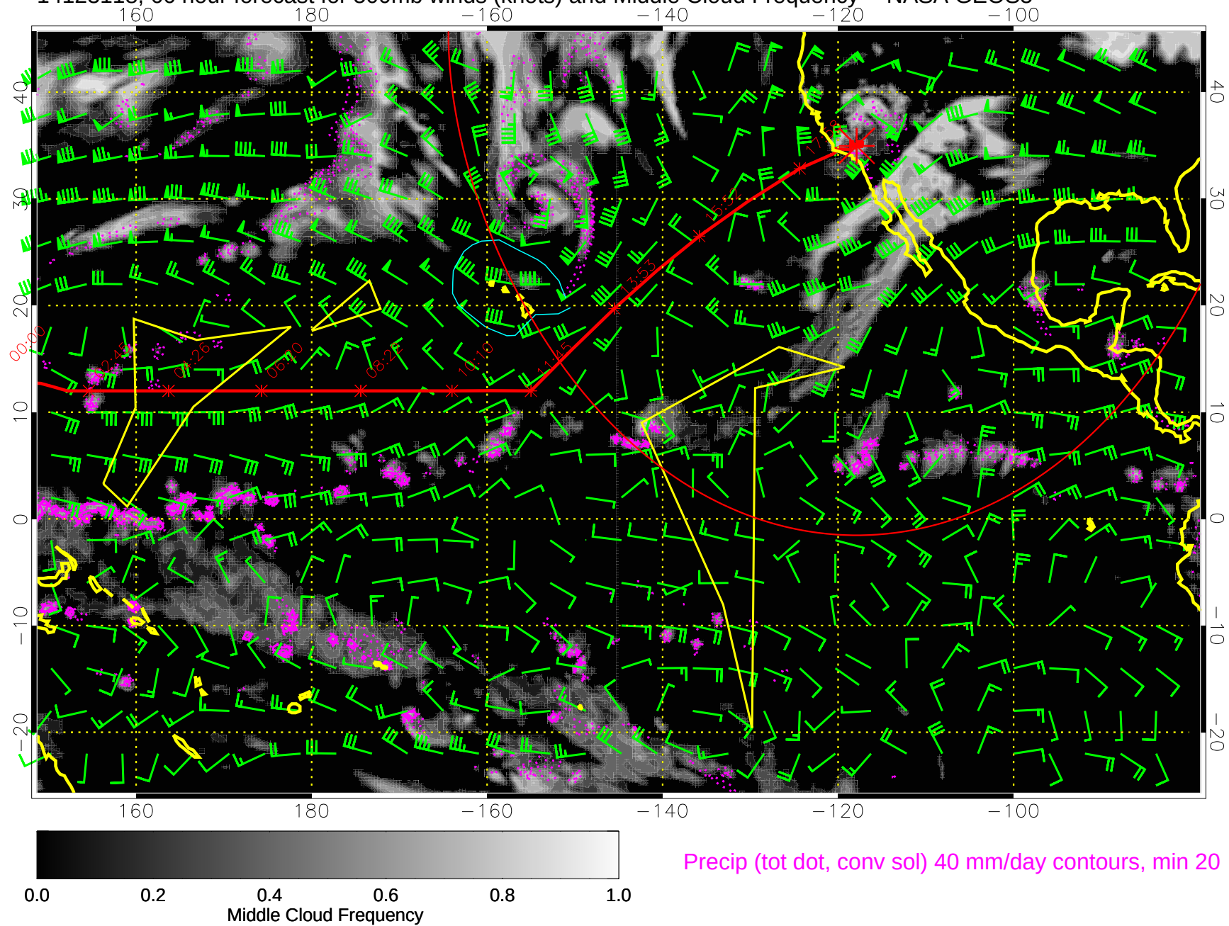
14123118, 66 hour forecast for 500mb winds (knots) and Middle Cloud Frequency -- NASA GEOS5
