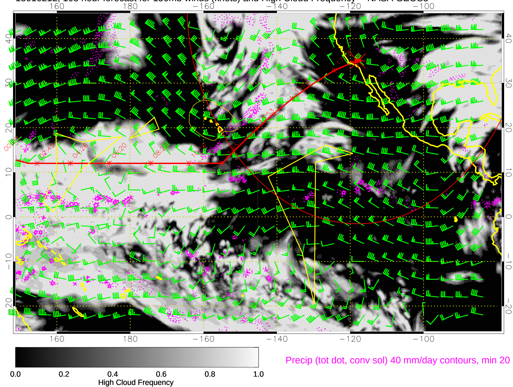
15010212, 108 hour forecast for 150mb winds (knots) and High Cloud Frequency -- NASA GEOS5
