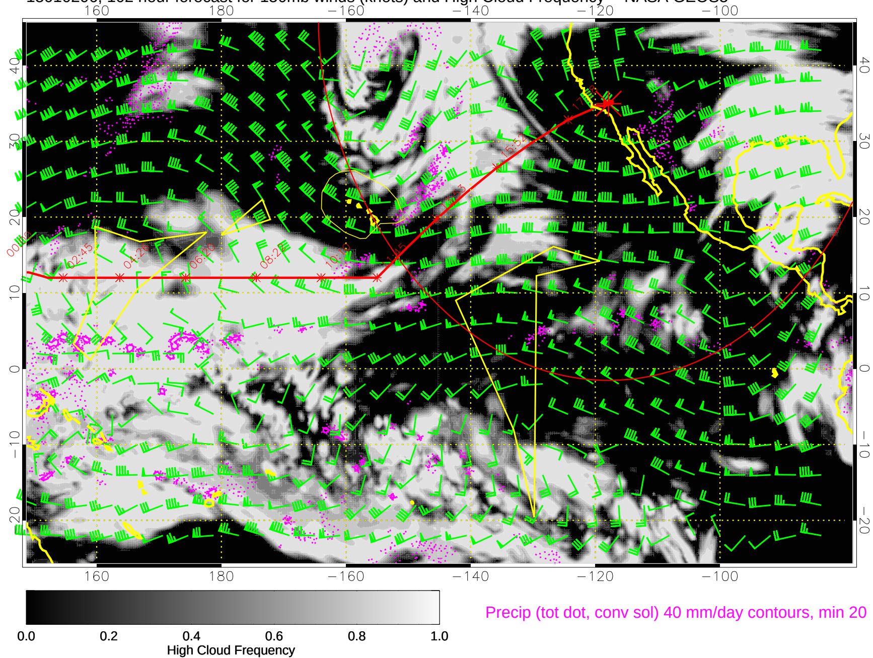
15010206, 102 hour forecast for 150mb winds (knots) and High Cloud Frequency -- NASA GEOS5
