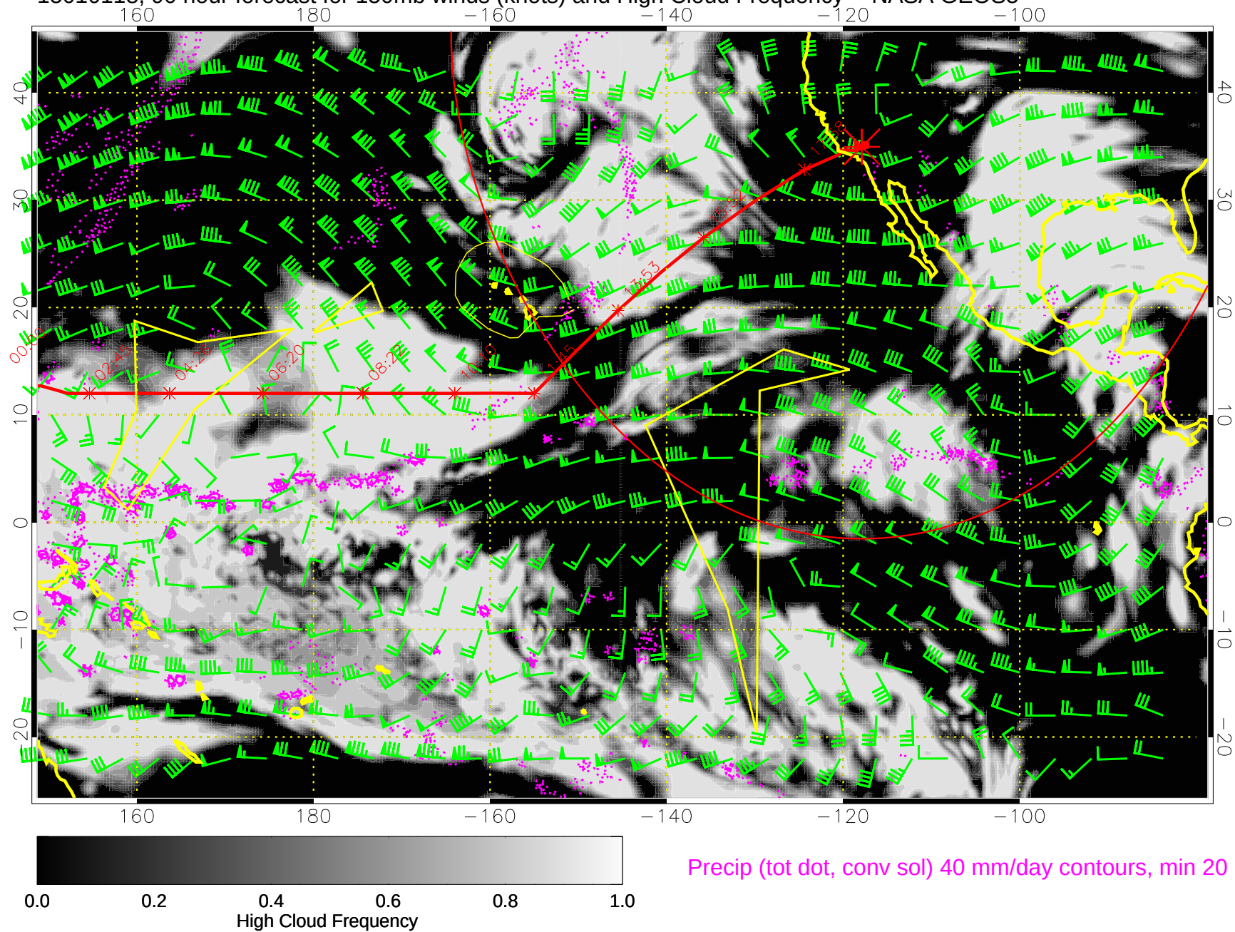
15010118, 90 hour forecast for 150mb winds (knots) and High Cloud Frequency -- NASA GEOS5
