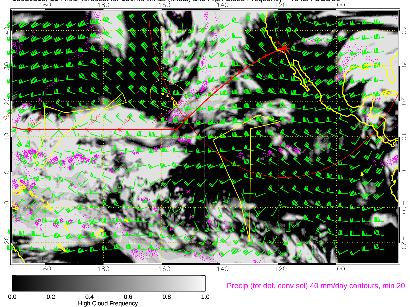
15010218, 114 hour forecast for 150mb winds (knots) and High Cloud Frequency -- NASA GEOS5
