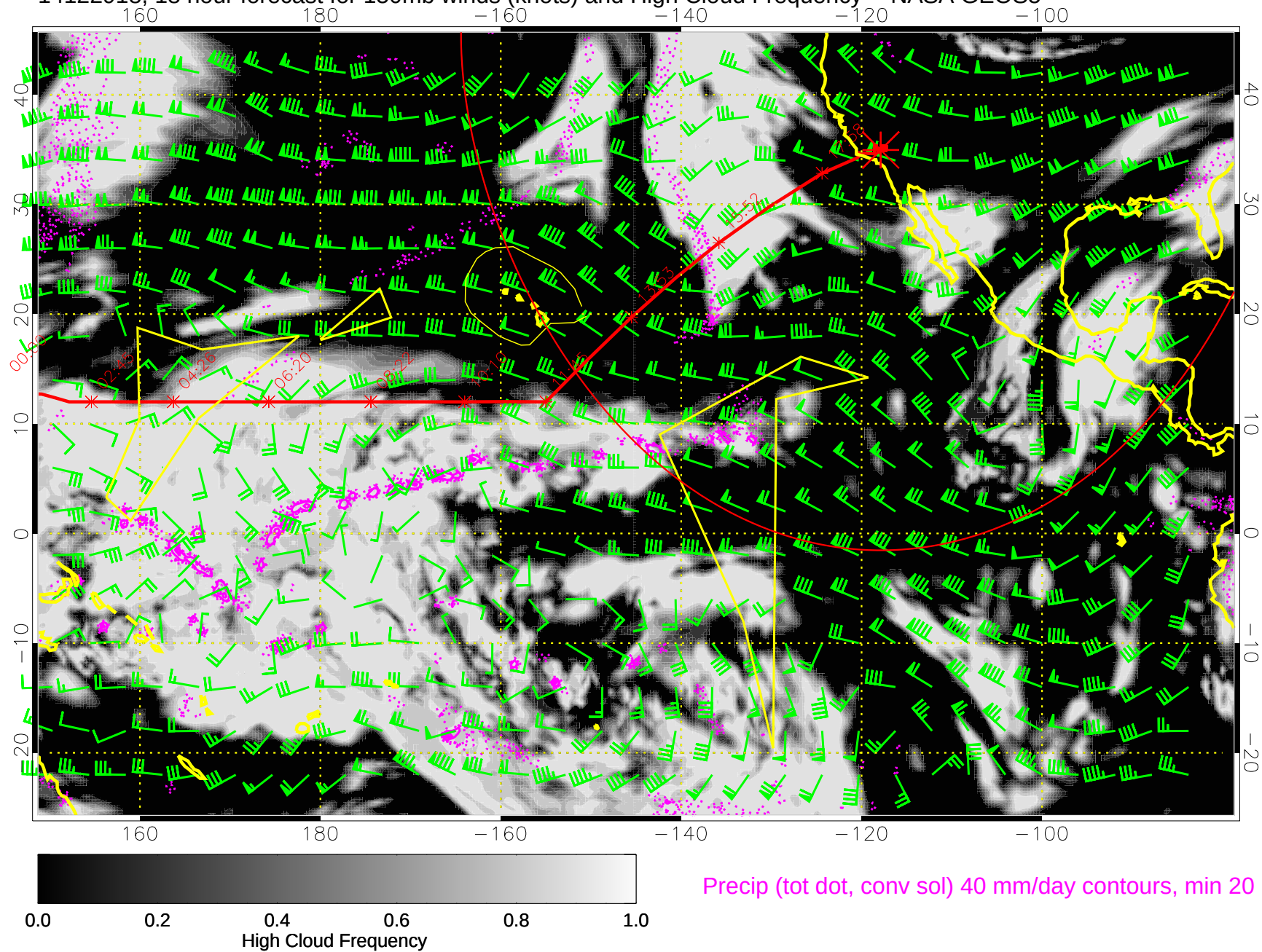
14122918, 18 hour forecast for 150mb winds (knots) and High Cloud Frequency -- NASA GEOS5
