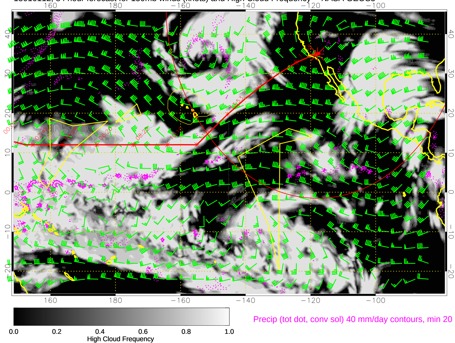
15010112, 84 hour forecast for 150mb winds (knots) and High Cloud Frequency -- NASA GEOS5
