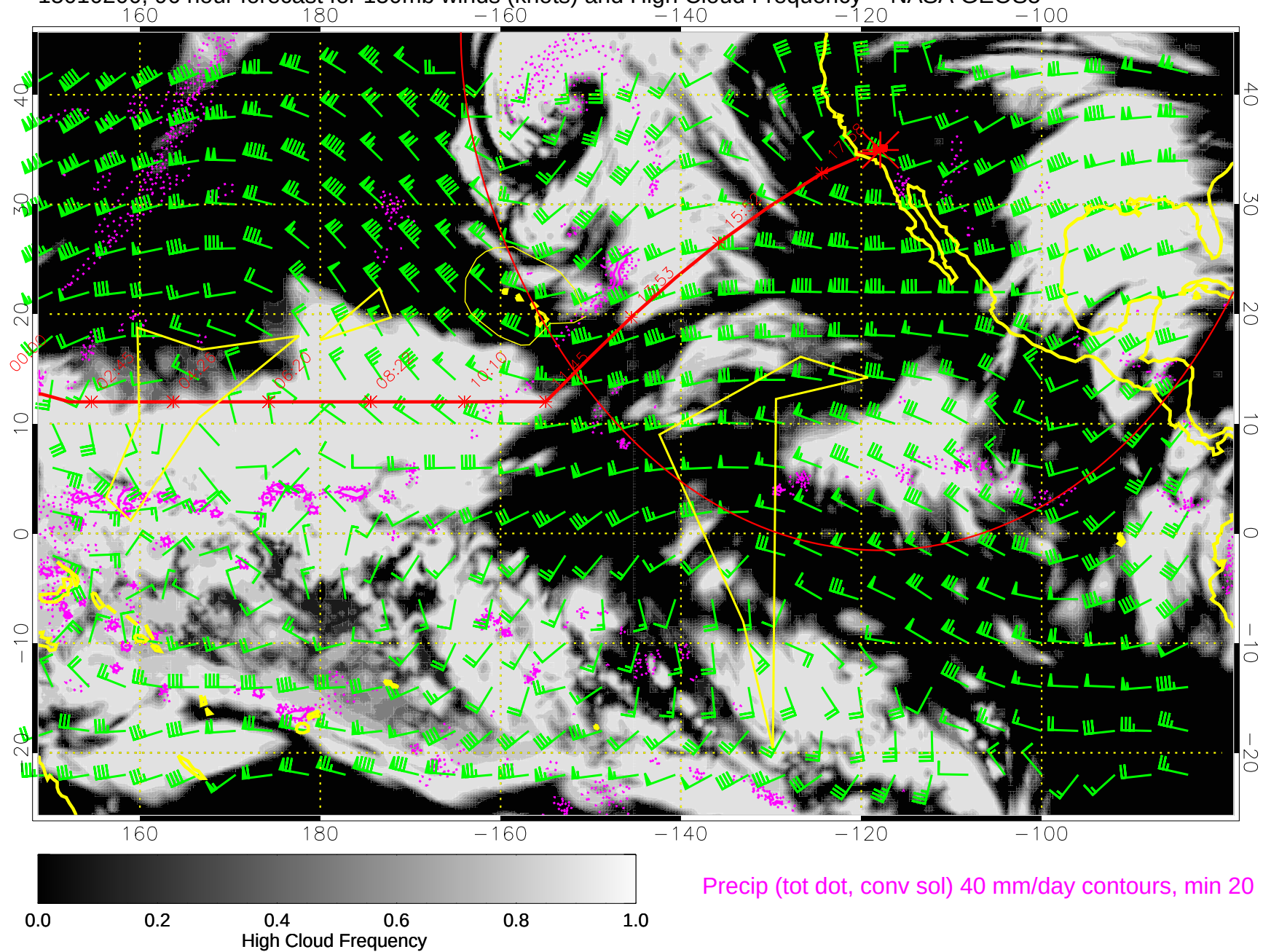
15010200, 96 hour forecast for 150mb winds (knots) and High Cloud Frequency -- NASA GEOS5
