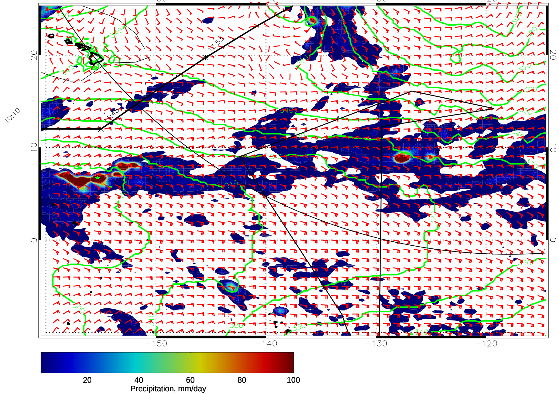
14123018, 90 hour forecast for 975mb Z, Precip., and Surface Winds (knots) -- NASA GEOS5
