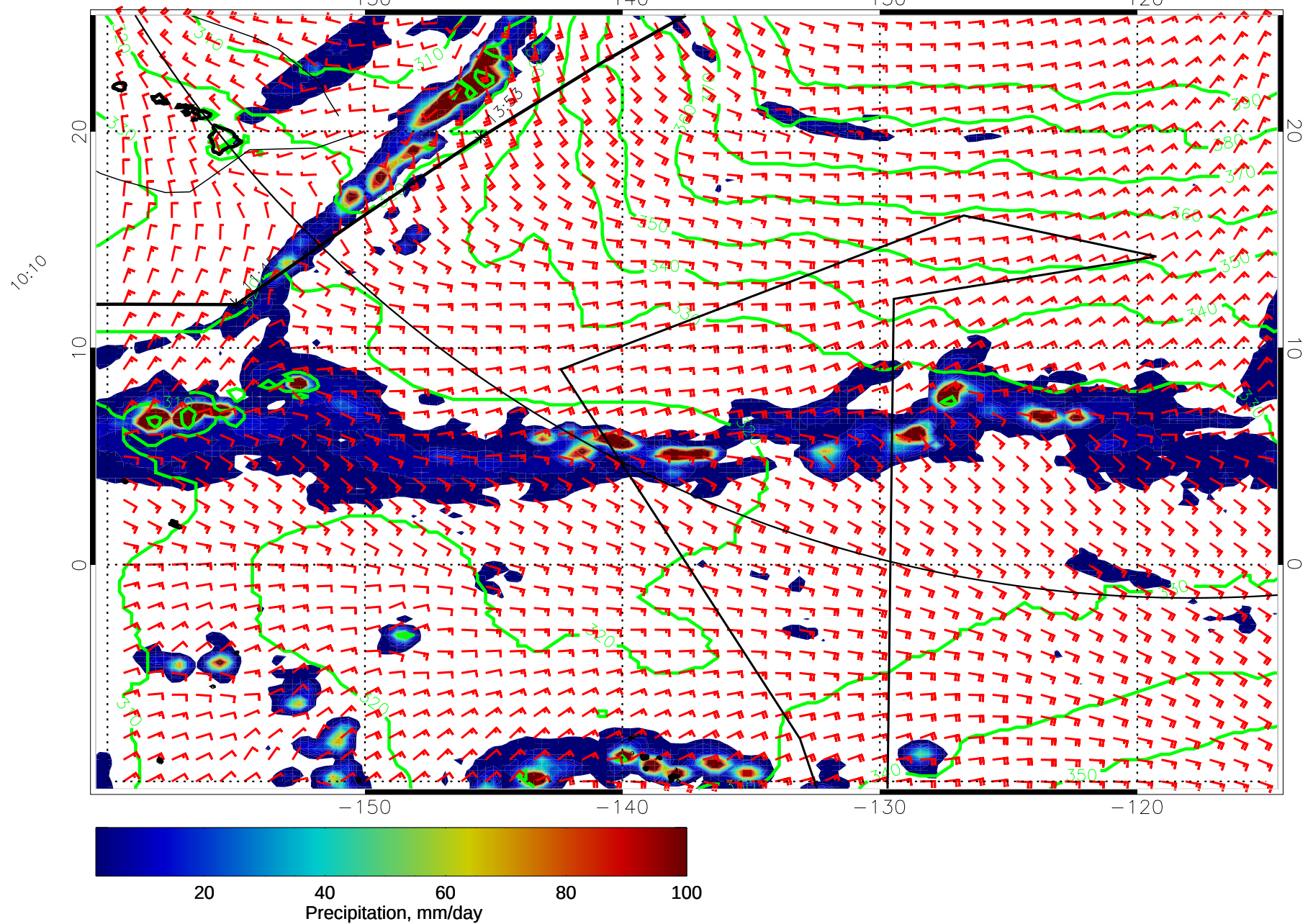
14122718, 18 hour forecast for 975mb Z, Precip., and Surface Winds (knots) -- NASA GEOS5
