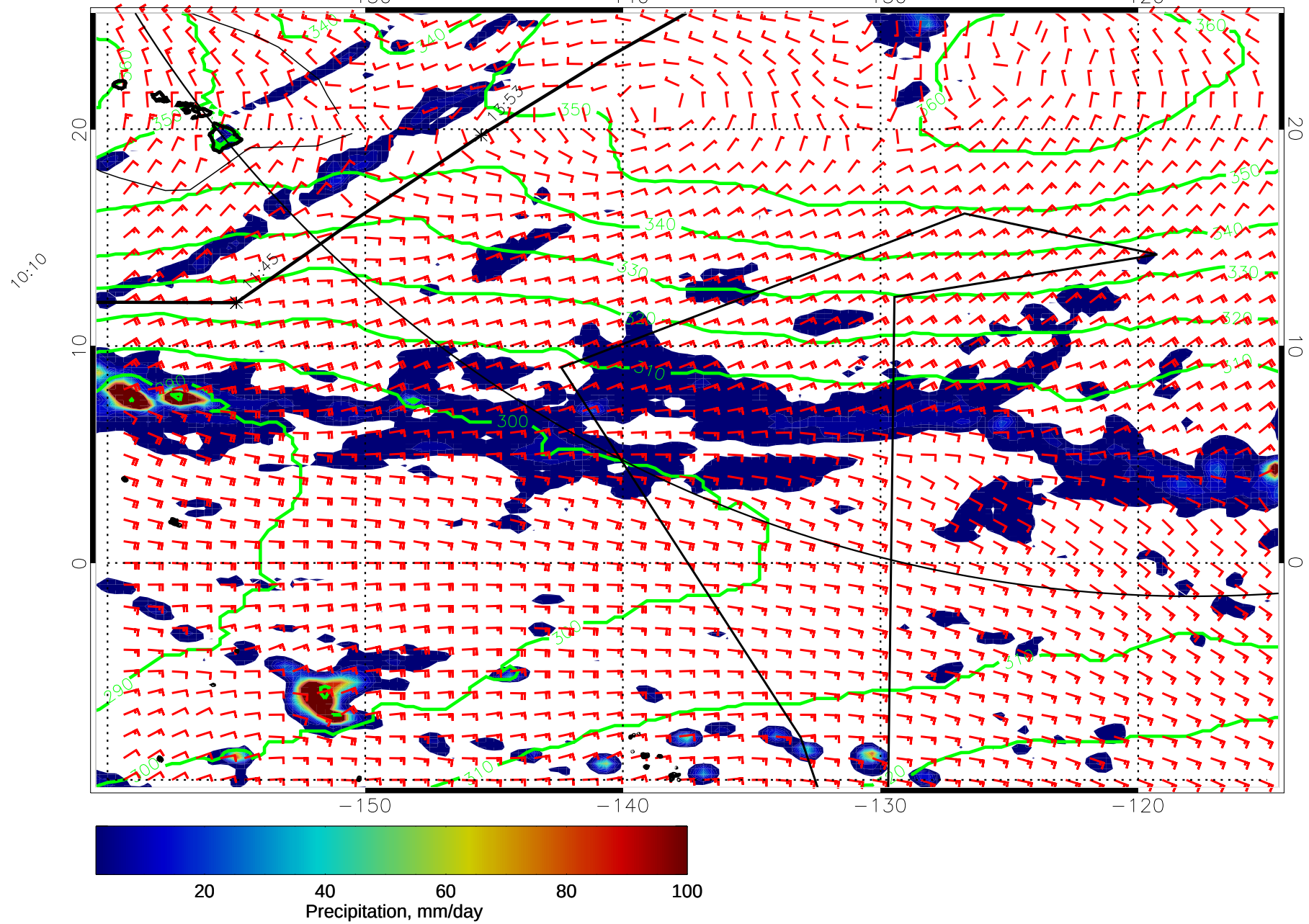
15010100, 120 hour forecast for 975mb Z, Precip., and Surface Winds (knots) -- NASA GEOS5
