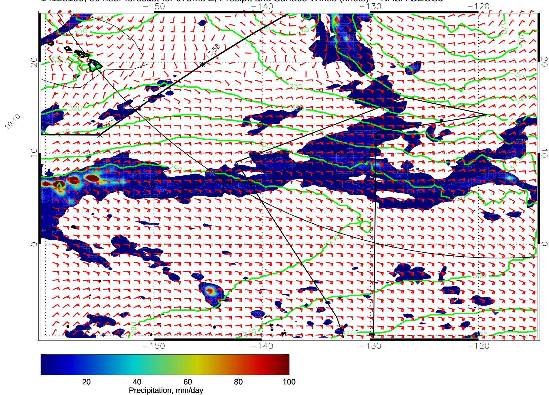
14123100, 96 hour forecast for 975mb Z, Precip., and Surface Winds (knots) -- NASA GEOS5
