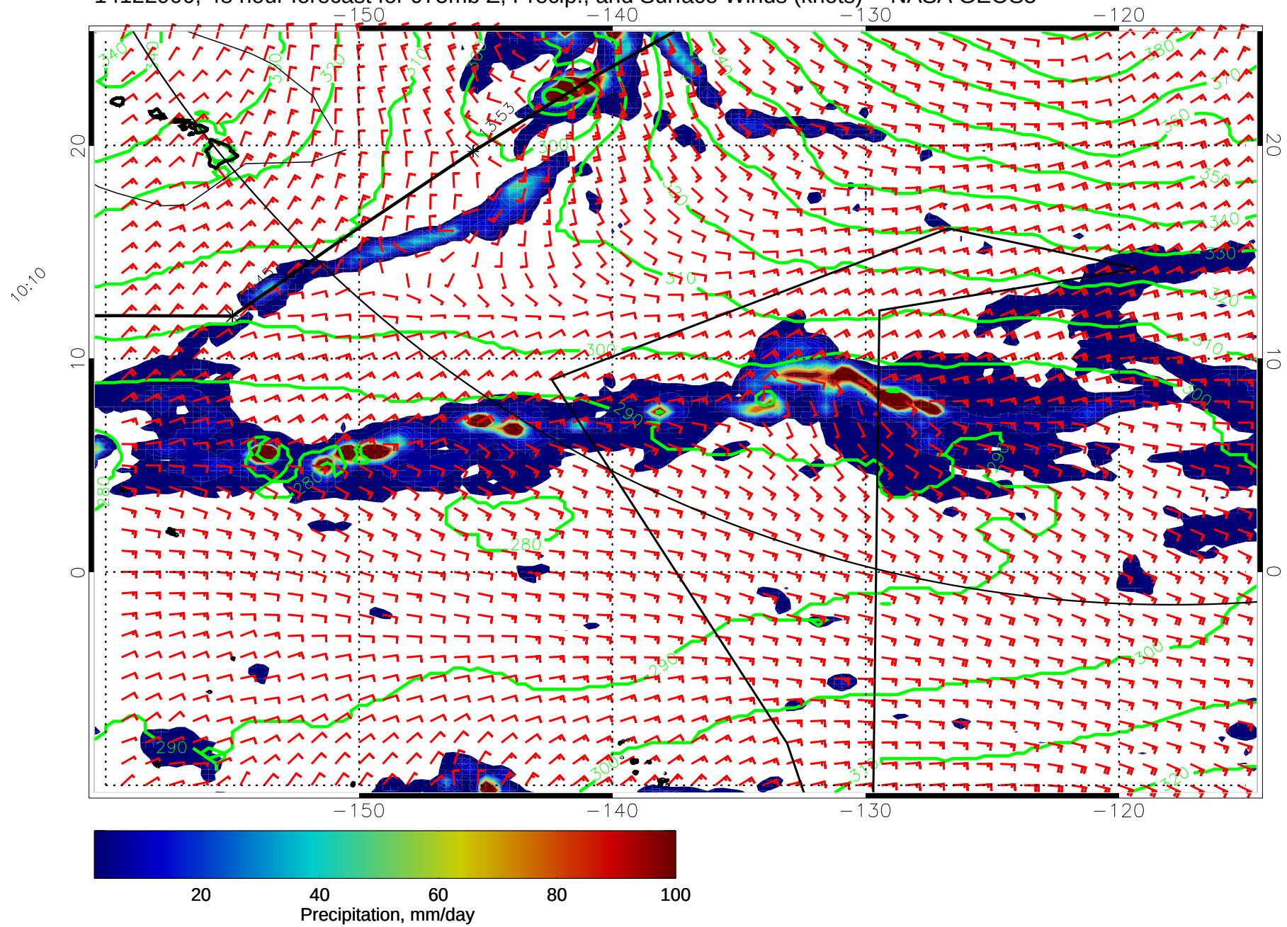
14122900, 48 hour forecast for 975mb Z, Precip., and Surface Winds (knots) -- NASA GEOS5
