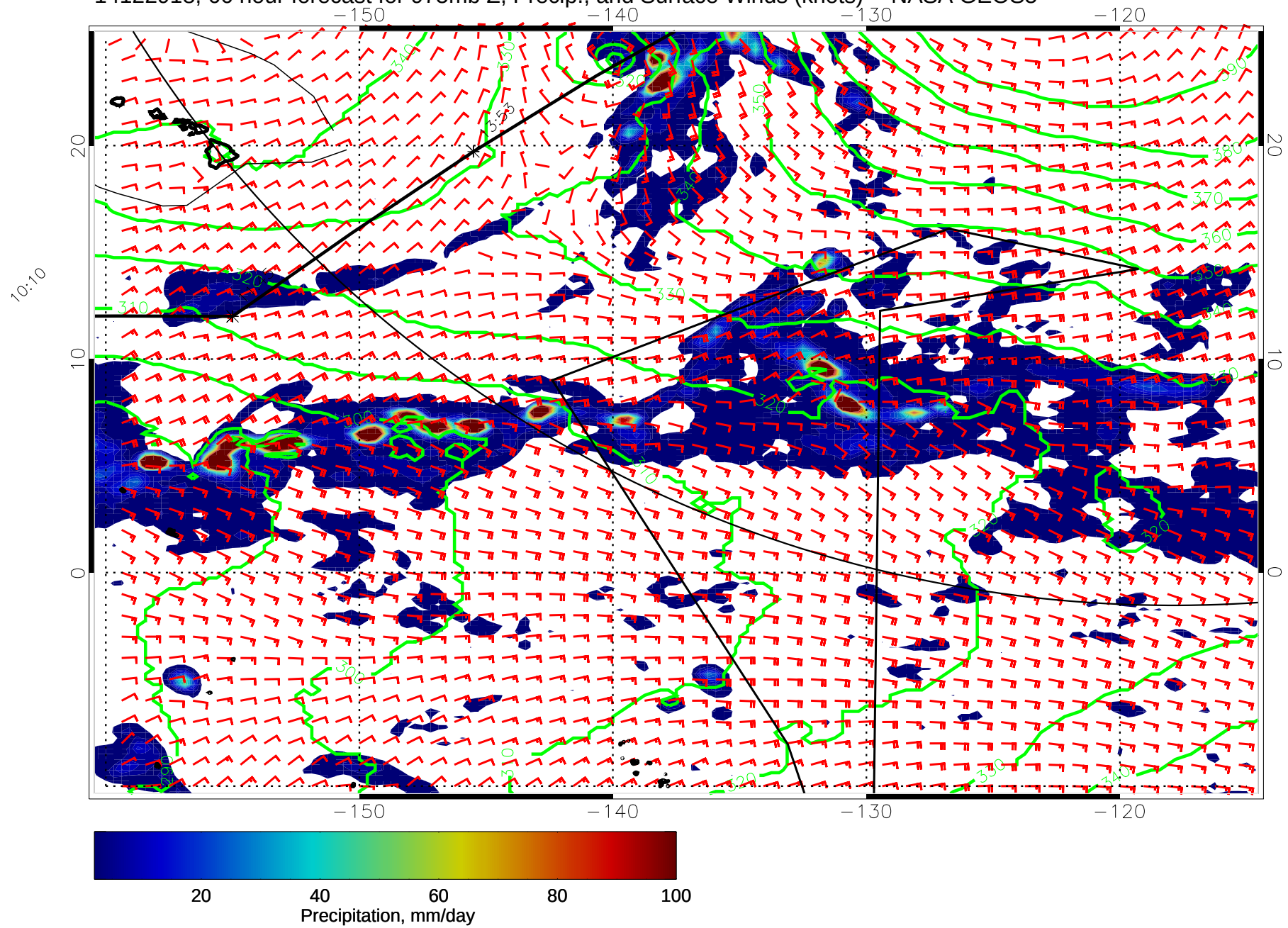
14122918, 66 hour forecast for 975mb Z, Precip., and Surface Winds (knots) -- NASA GEOS5
