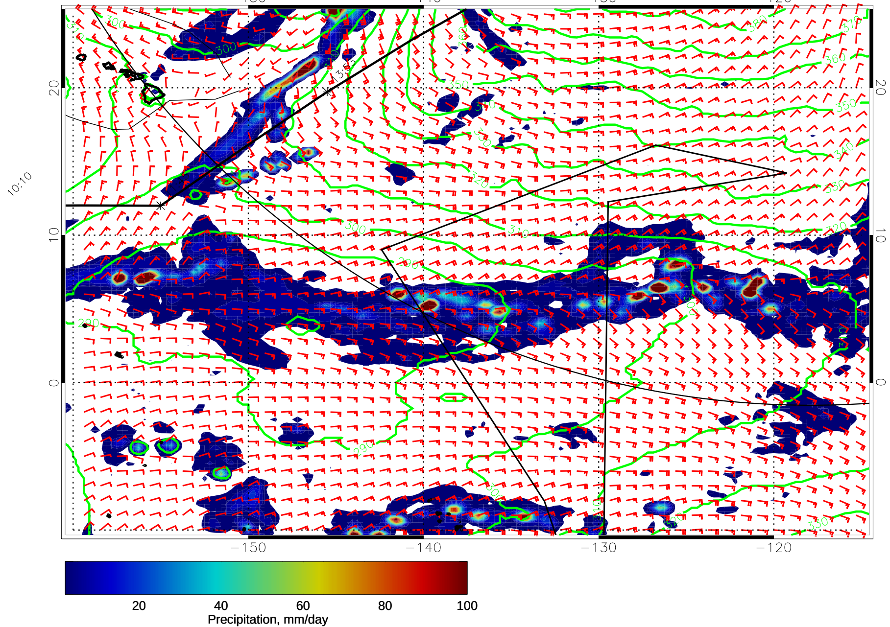
14122712, 12 hour forecast for 975mb Z, Precip., and Surface Winds (knots) -- NASA GEOS5
