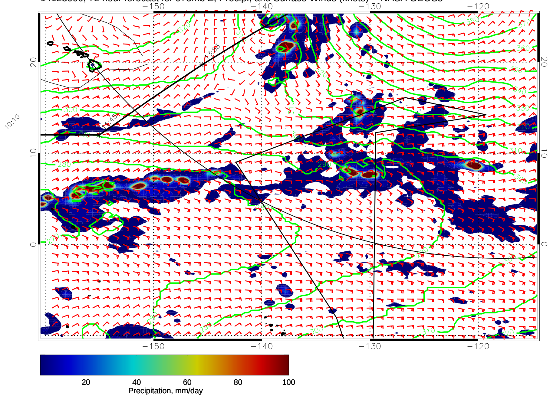
14123000, 72 hour forecast for 975mb Z, Precip., and Surface Winds (knots) -- NASA GEOS5
