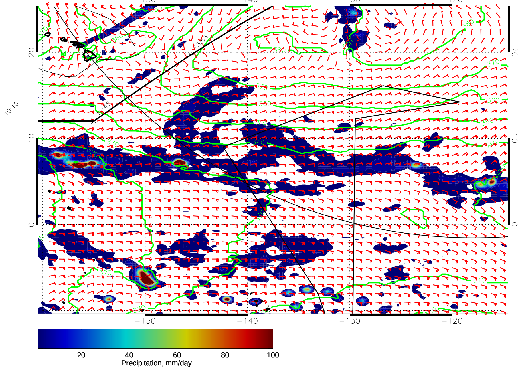
14123118, 114 hour forecast for 975mb Z, Precip., and Surface Winds (knots) -- NASA GEOS5
