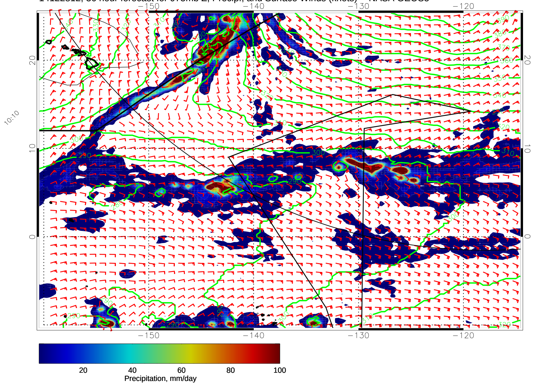
14122812, 36 hour forecast for 975mb Z, Precip., and Surface Winds (knots) -- NASA GEOS5
