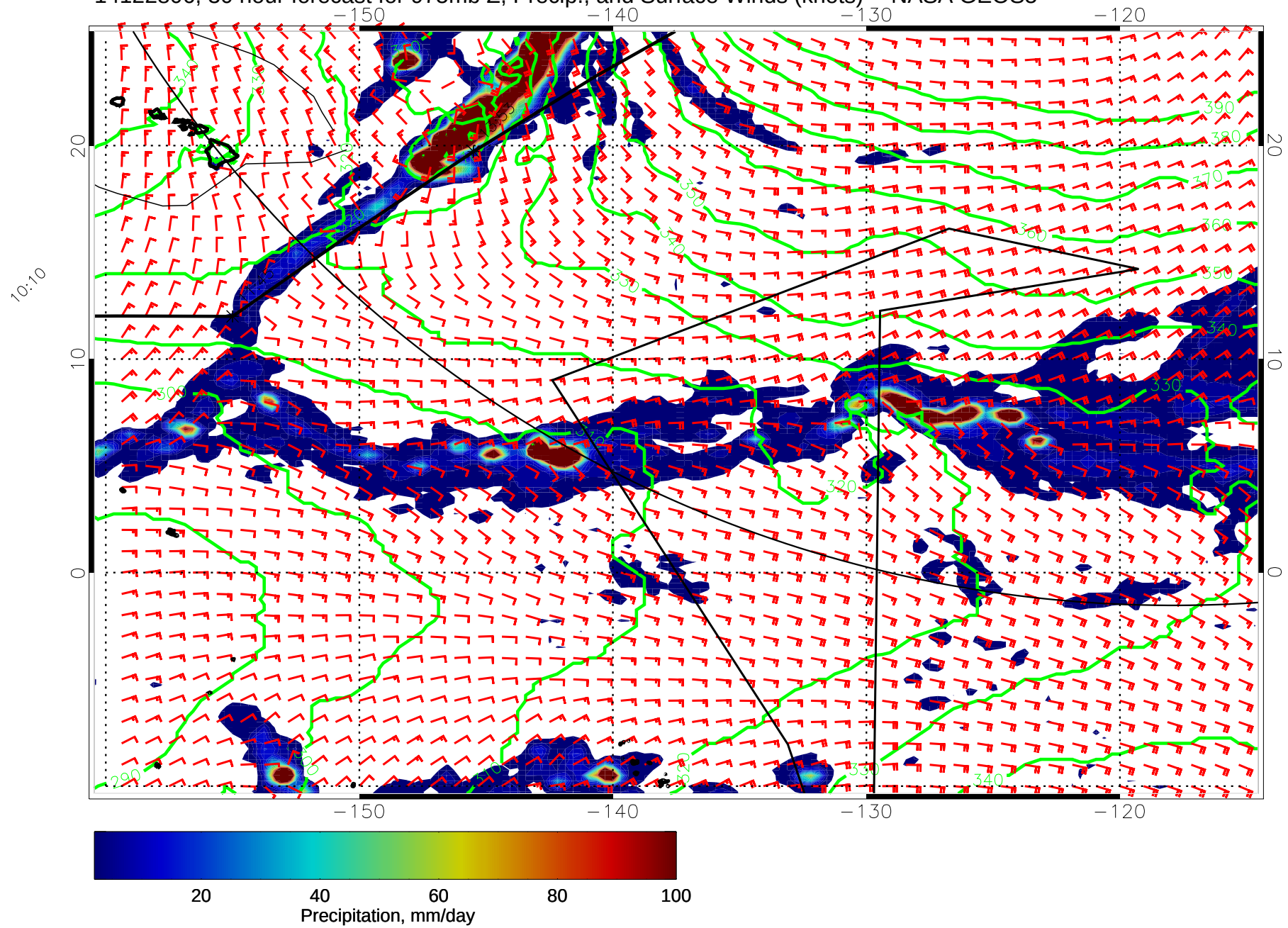
14122806, 30 hour forecast for 975mb Z, Precip., and Surface Winds (knots) -- NASA GEOS5
