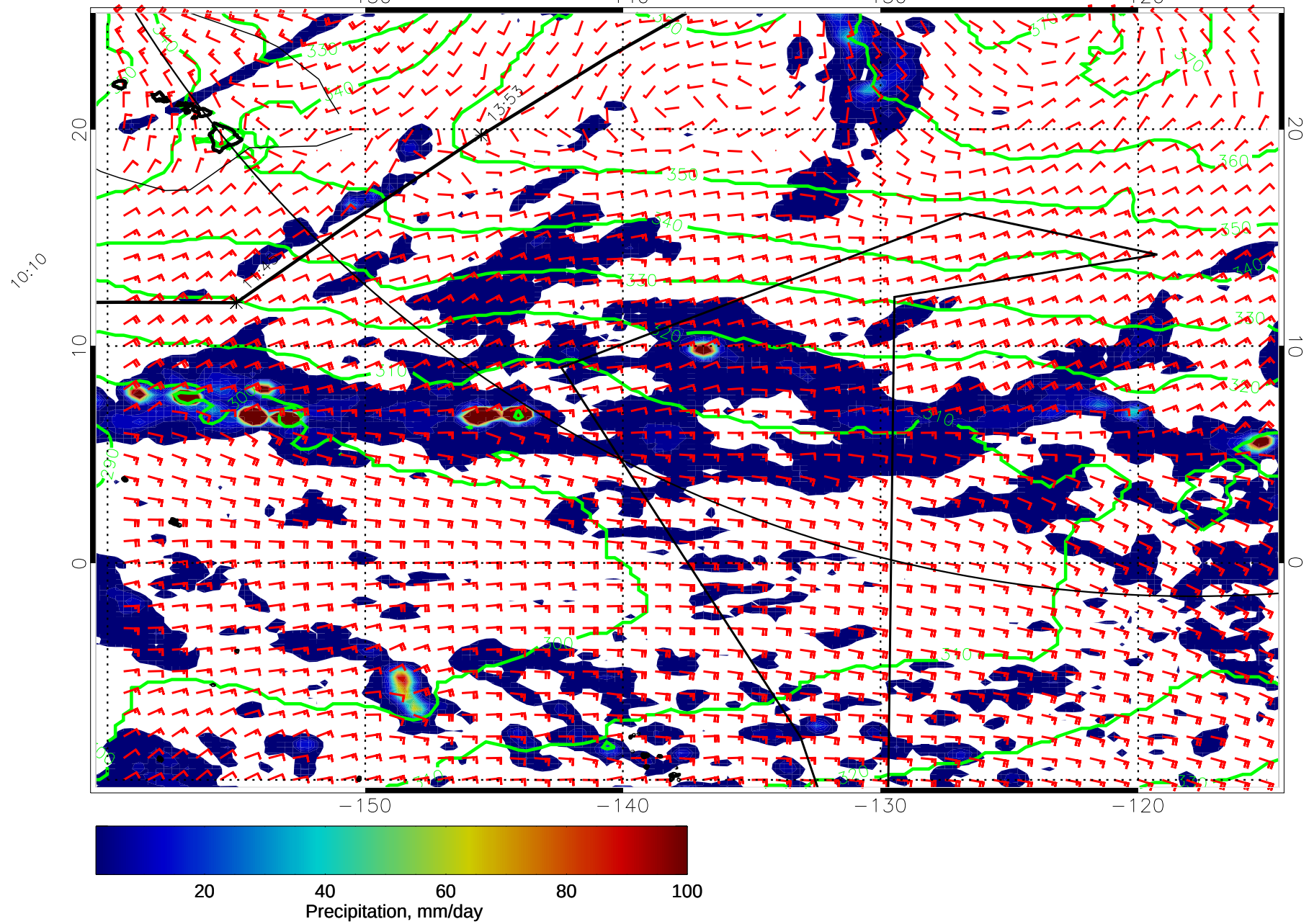
14123112, 108 hour forecast for 975mb Z, Precip., and Surface Winds (knots) -- NASA GEOS5
