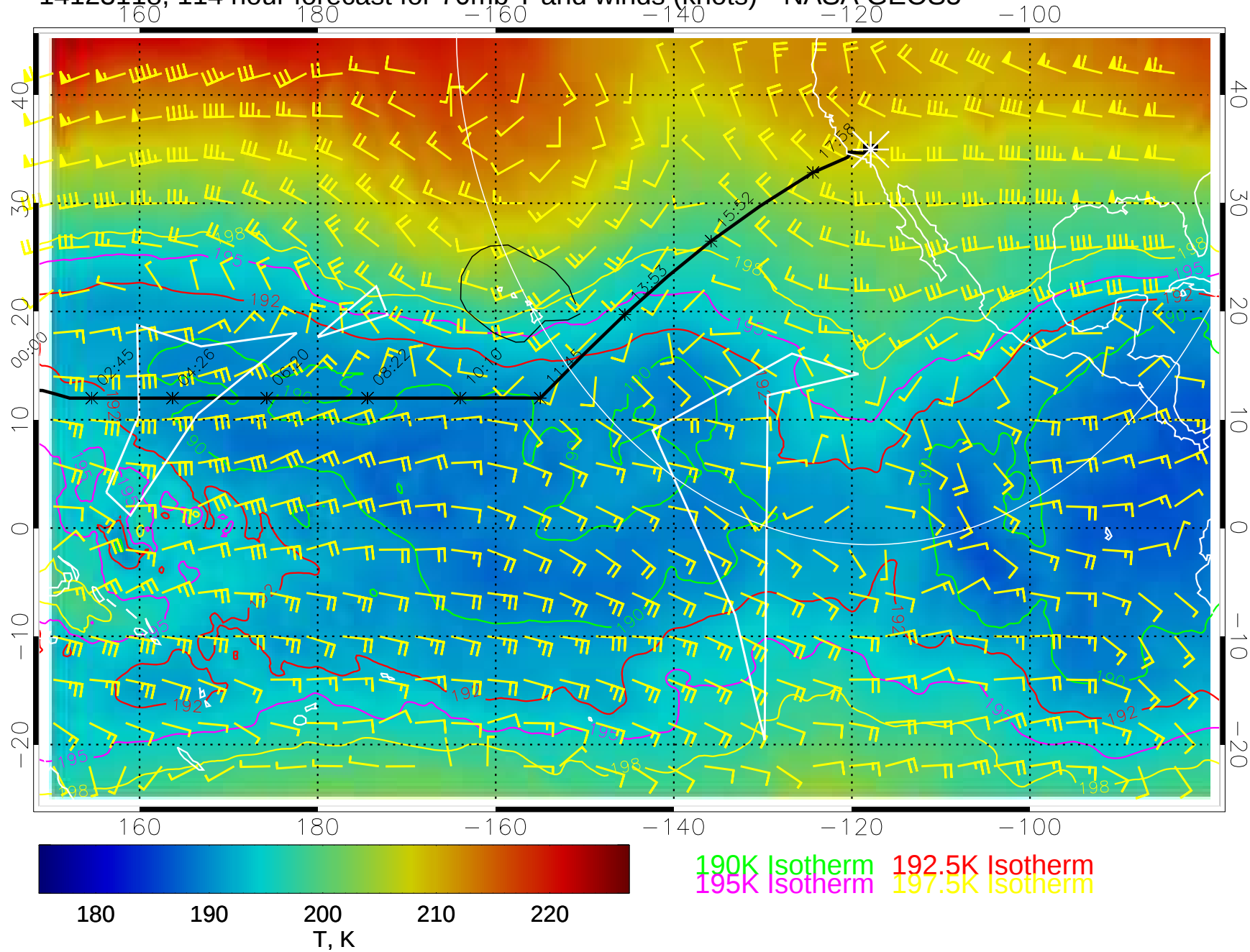
14123118, 114 hour forecast for 70mb T and winds (knots)-- NASA GEOS5
