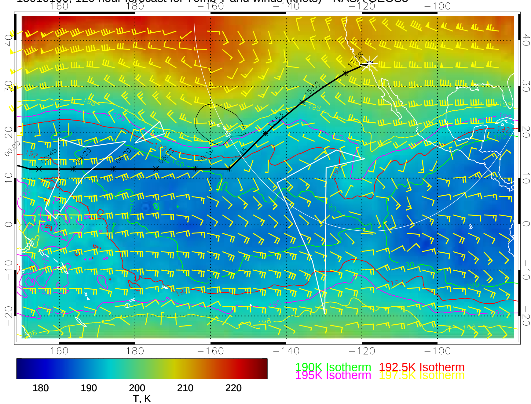
15010100, 120 hour forecast for 70mb T and winds (knots)-- NASA GEOS5
