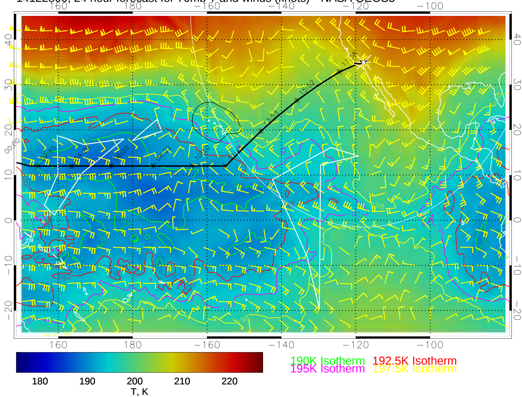
14122800, 24 hour forecast for 70mb T and winds (knots)-- NASA GEOS5
