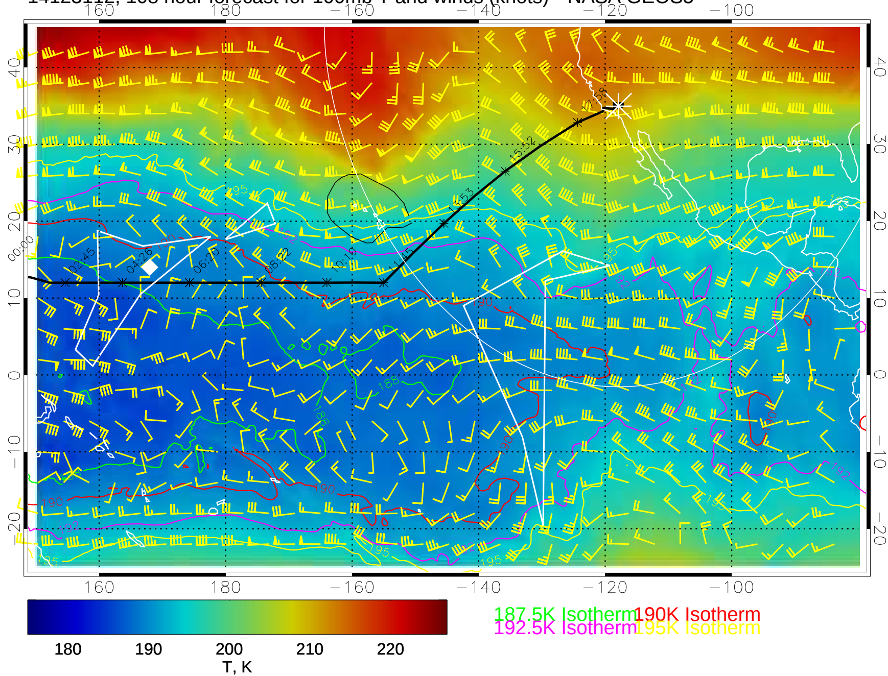
14123112, 108 hour forecast for 100mb T and winds (knots)-- NASA GEOS5
