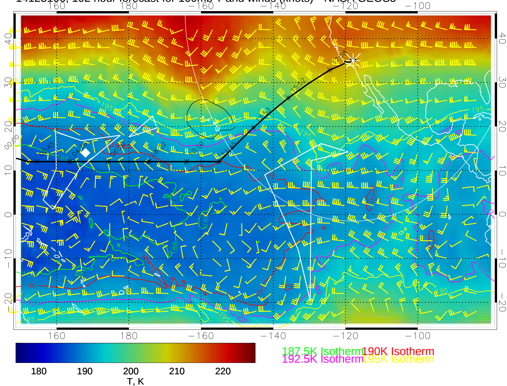
14123106, 102 hour forecast for 100mb T and winds (knots)-- NASA GEOS5
