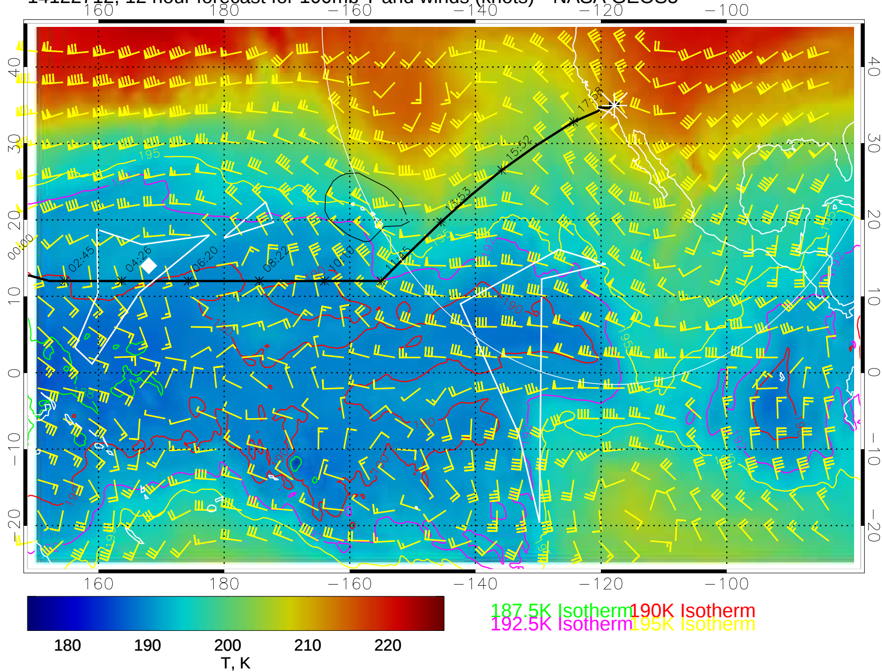
14122712, 12 hour forecast for 100mb T and winds (knots)-- NASA GEOS5
