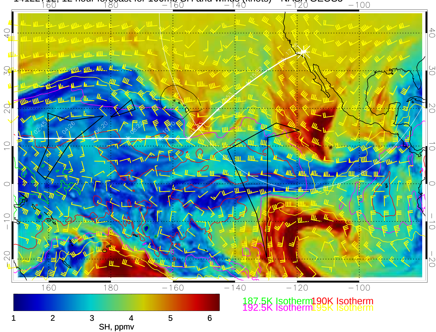
14122712, 12 hour forecast for 100mb SH and winds (knots)-- NASA GEOS5
