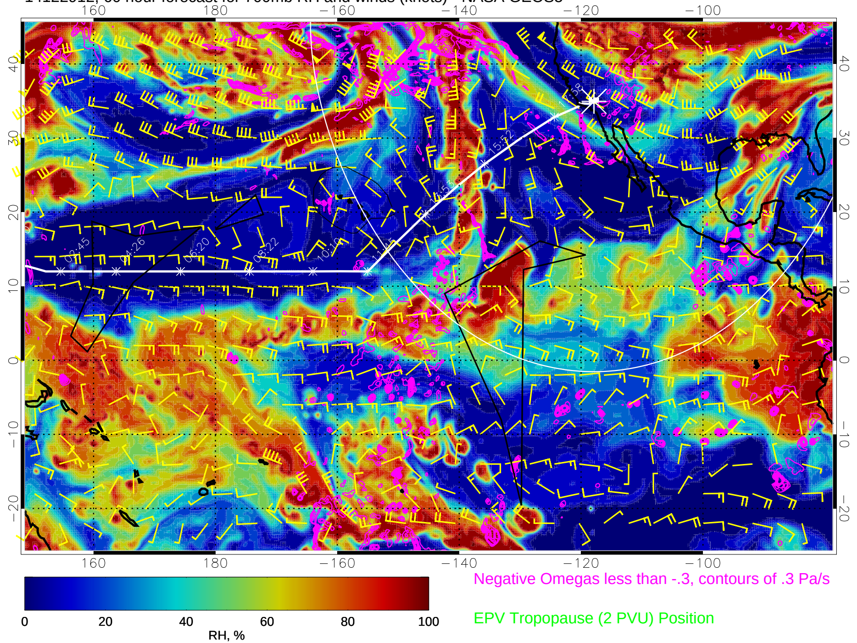
14122912, 60 hour forecast for 700mb RH and winds (knots) - NASA GEOS5
