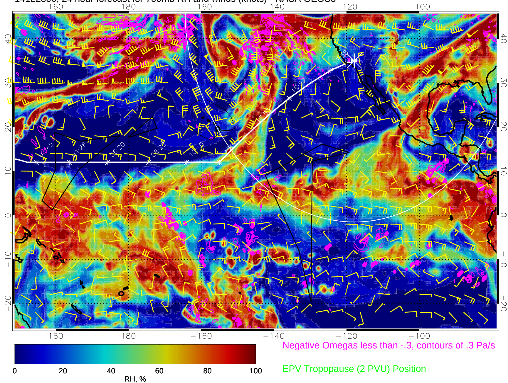
14122800, 24 hour forecast for 700mb RH and winds (knots) - NASA GEOS5
