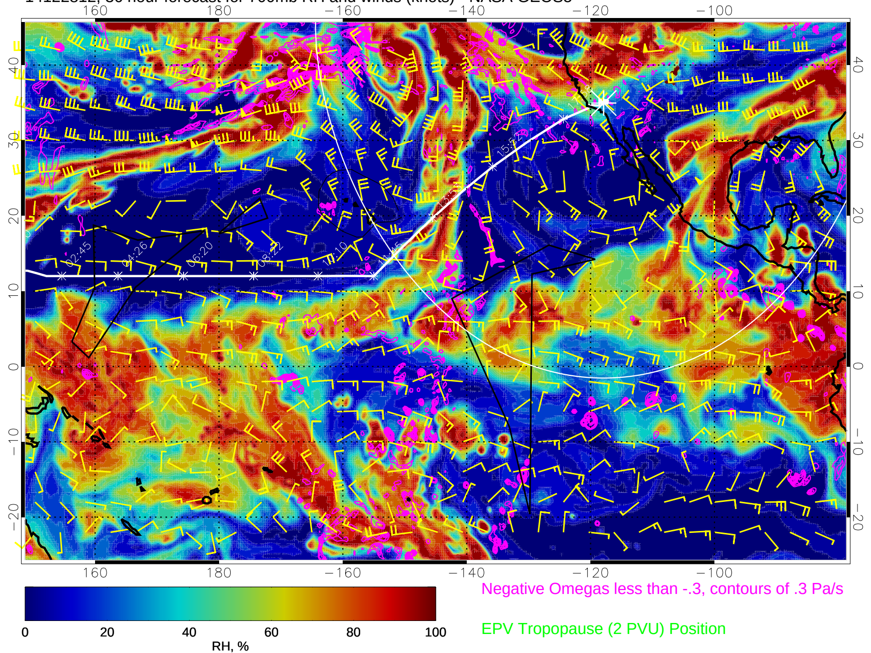
14122812, 36 hour forecast for 700mb RH and winds (knots) - NASA GEOS5
