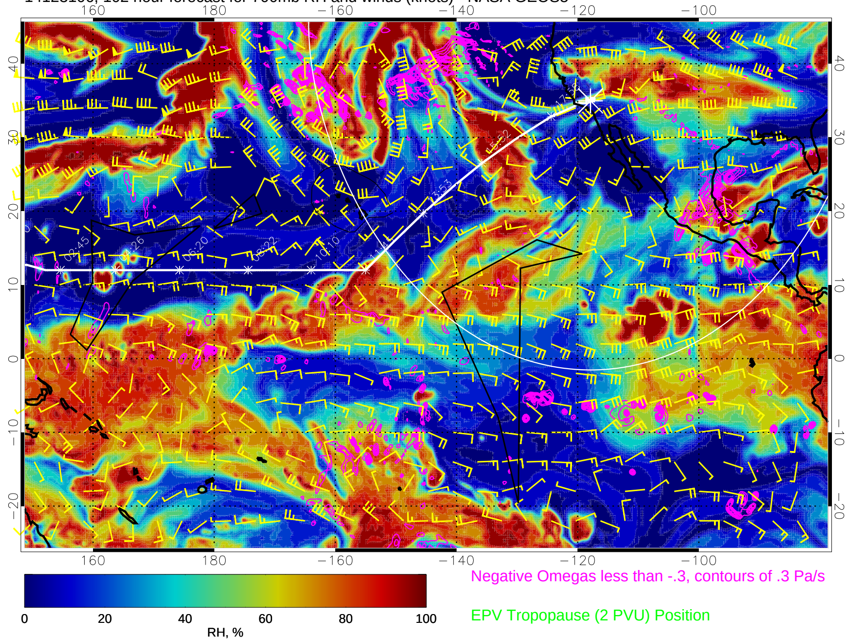
14123106, 102 hour forecast for 700mb RH and winds (knots) - NASA GEOS5
