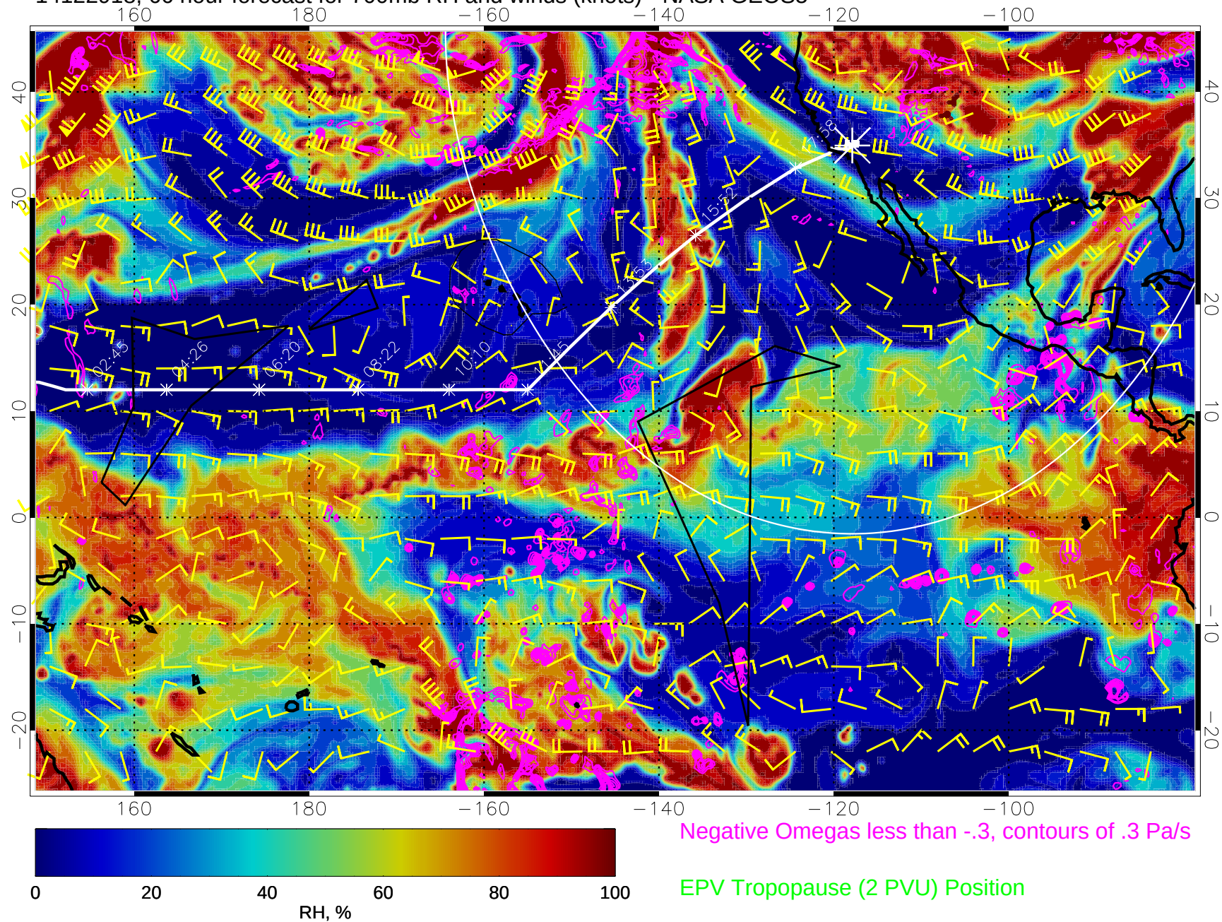
14122918, 66 hour forecast for 700mb RH and winds (knots) - NASA GEOS5
