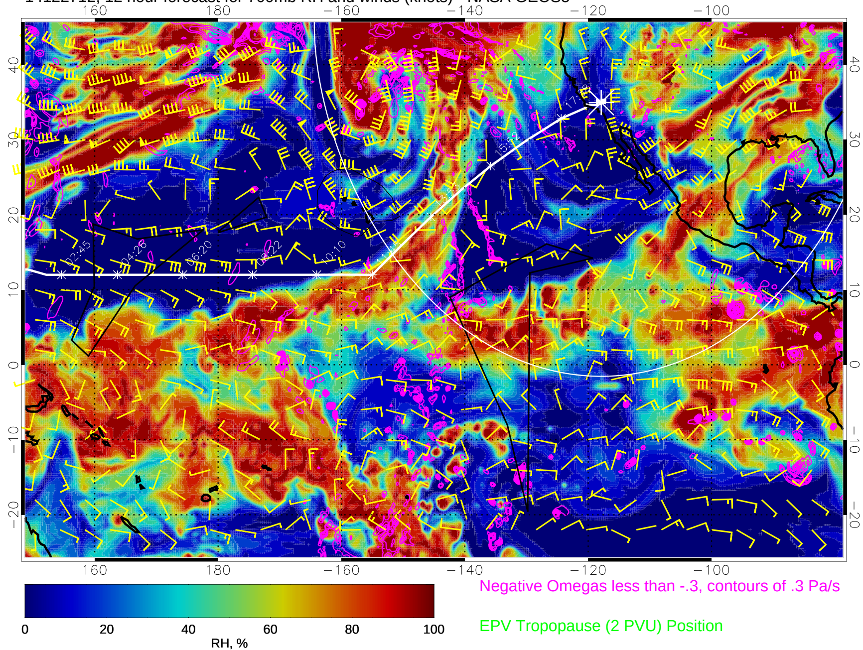
14122712, 12 hour forecast for 700mb RH and winds (knots) - NASA GEOS5
