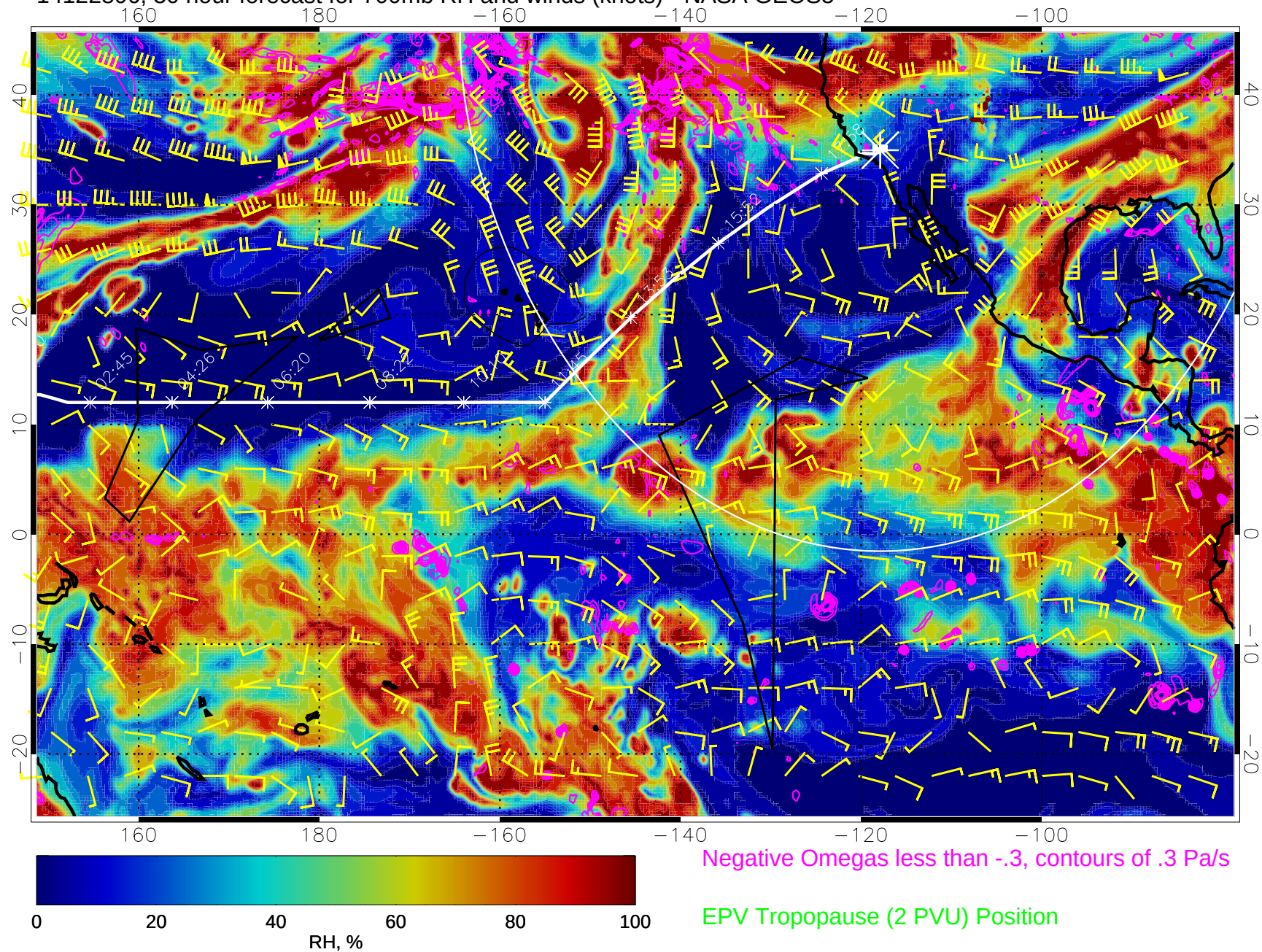
14122806, 30 hour forecast for 700mb RH and winds (knots) - NASA GEOS5
