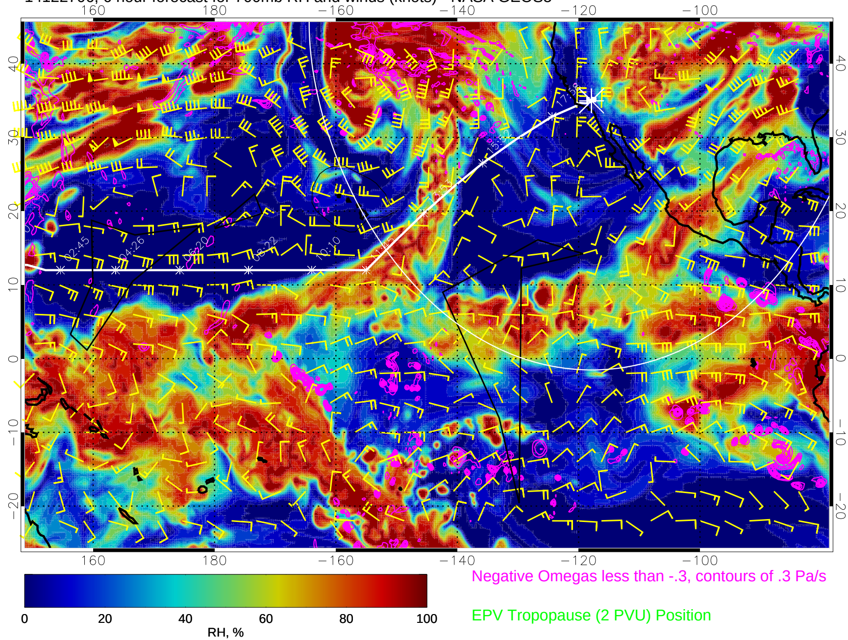
14122706, 6 hour forecast for 700mb RH and winds (knots) - NASA GEOS5
