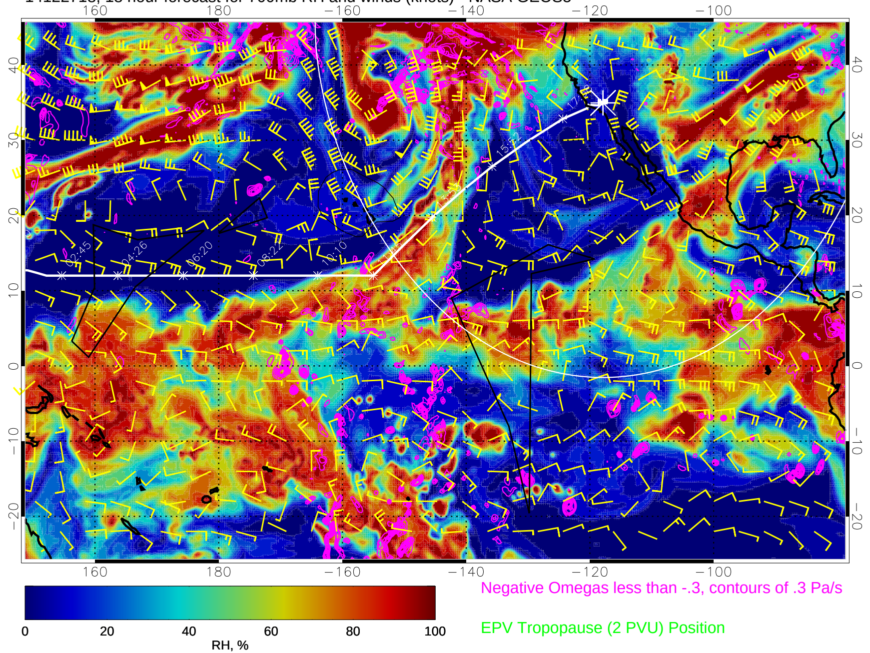
14122718, 18 hour forecast for 700mb RH and winds (knots) - NASA GEOS5
