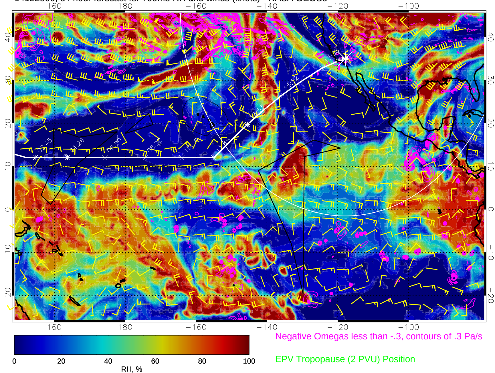
14122906, 54 hour forecast for 700mb RH and winds (knots) - NASA GEOS5
