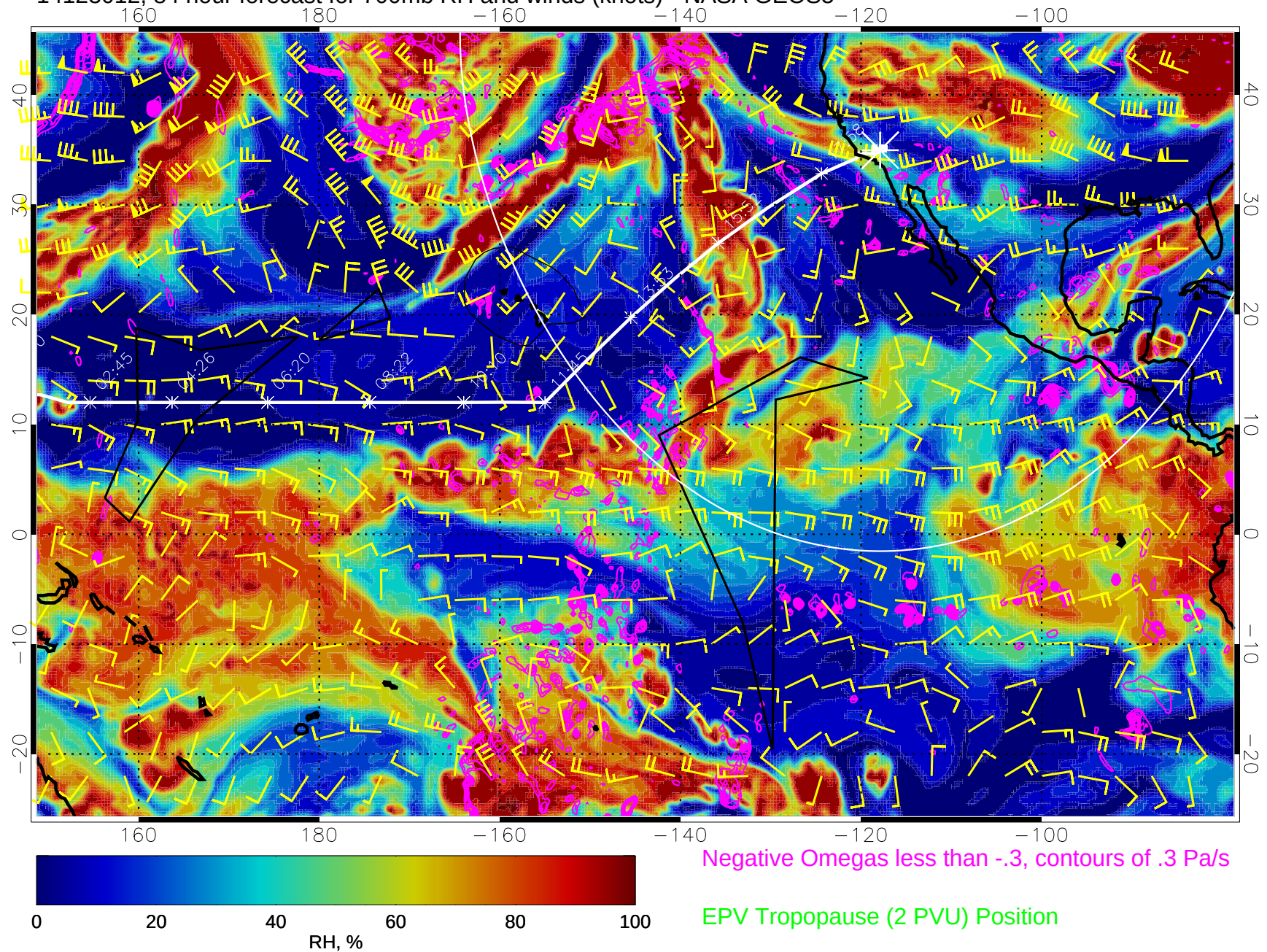
14123012, 84 hour forecast for 700mb RH and winds (knots) - NASA GEOS5
