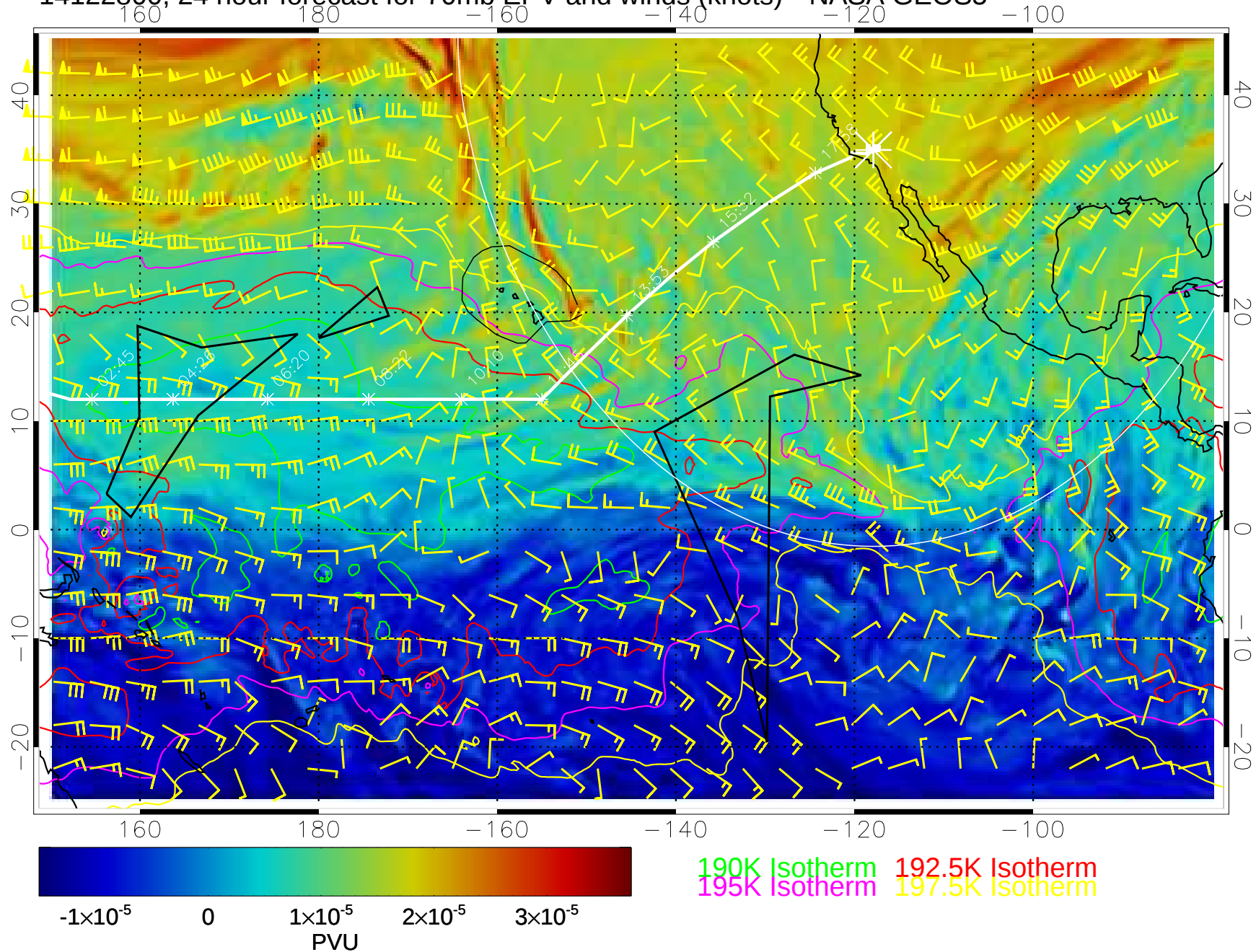
14122800, 24 hour forecast for 70mb EPV and winds (knots)-- NASA GEOS5
