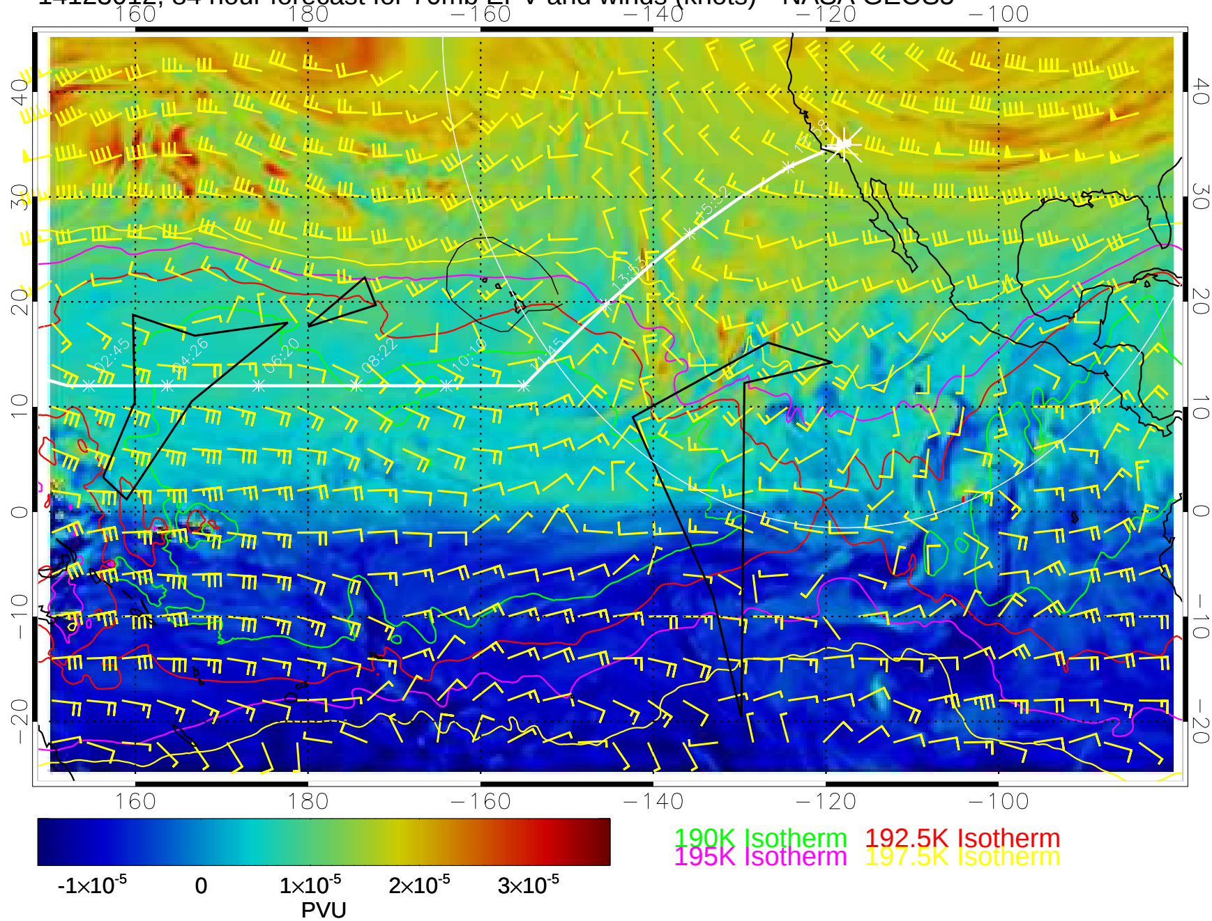
14123012, 84 hour forecast for 70mb EPV and winds (knots)-- NASA GEOS5
