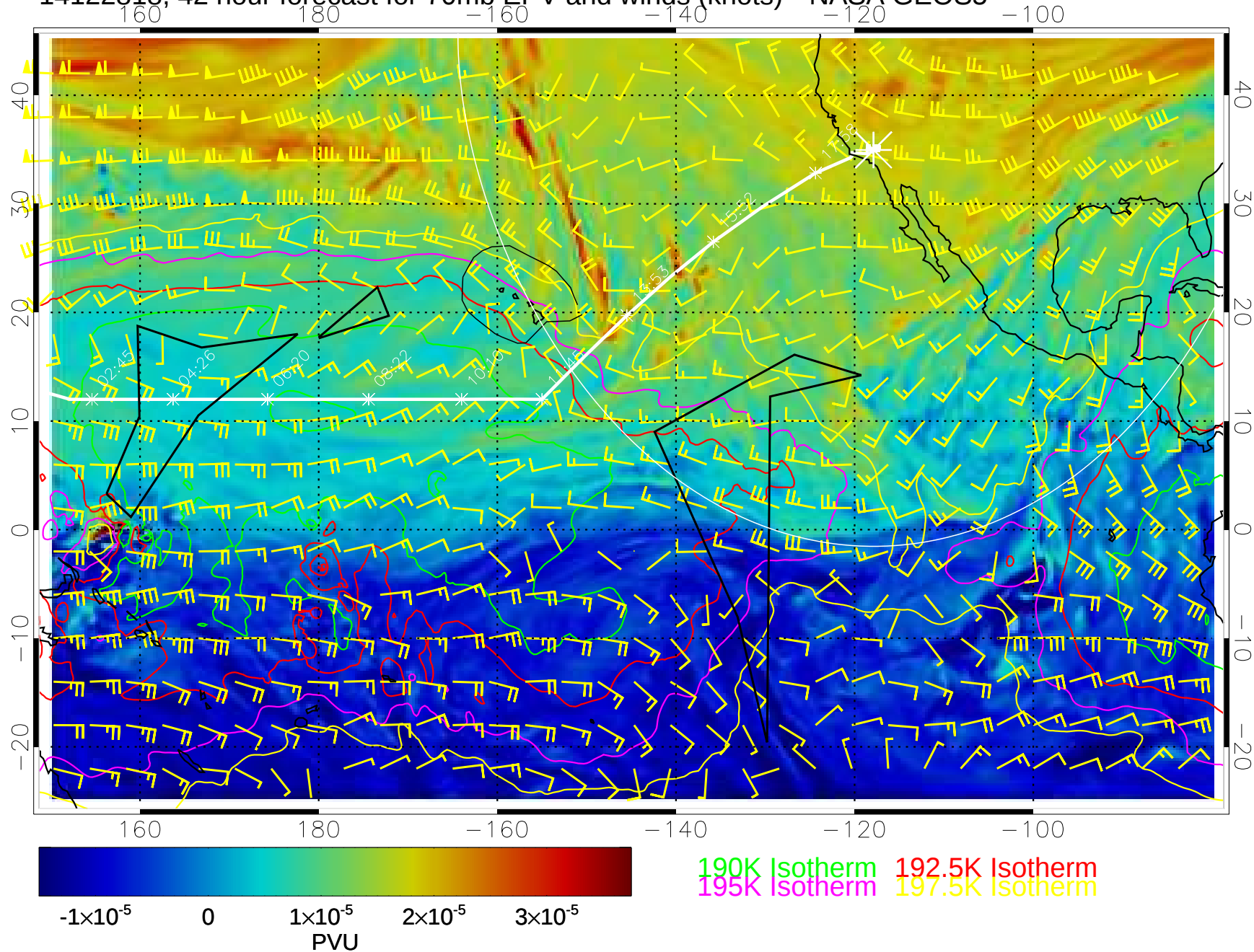
14122818, 42 hour forecast for 70mb EPV and winds (knots)-- NASA GEOS5
