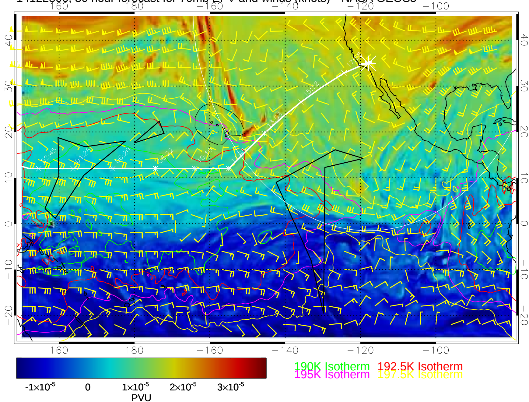
14122806, 30 hour forecast for 70mb EPV and winds (knots)-- NASA GEOS5
