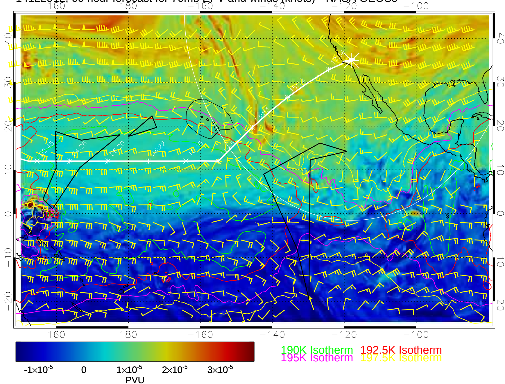
14122912, 60 hour forecast for 70mb EPV and winds (knots)-- NASA GEOS5
