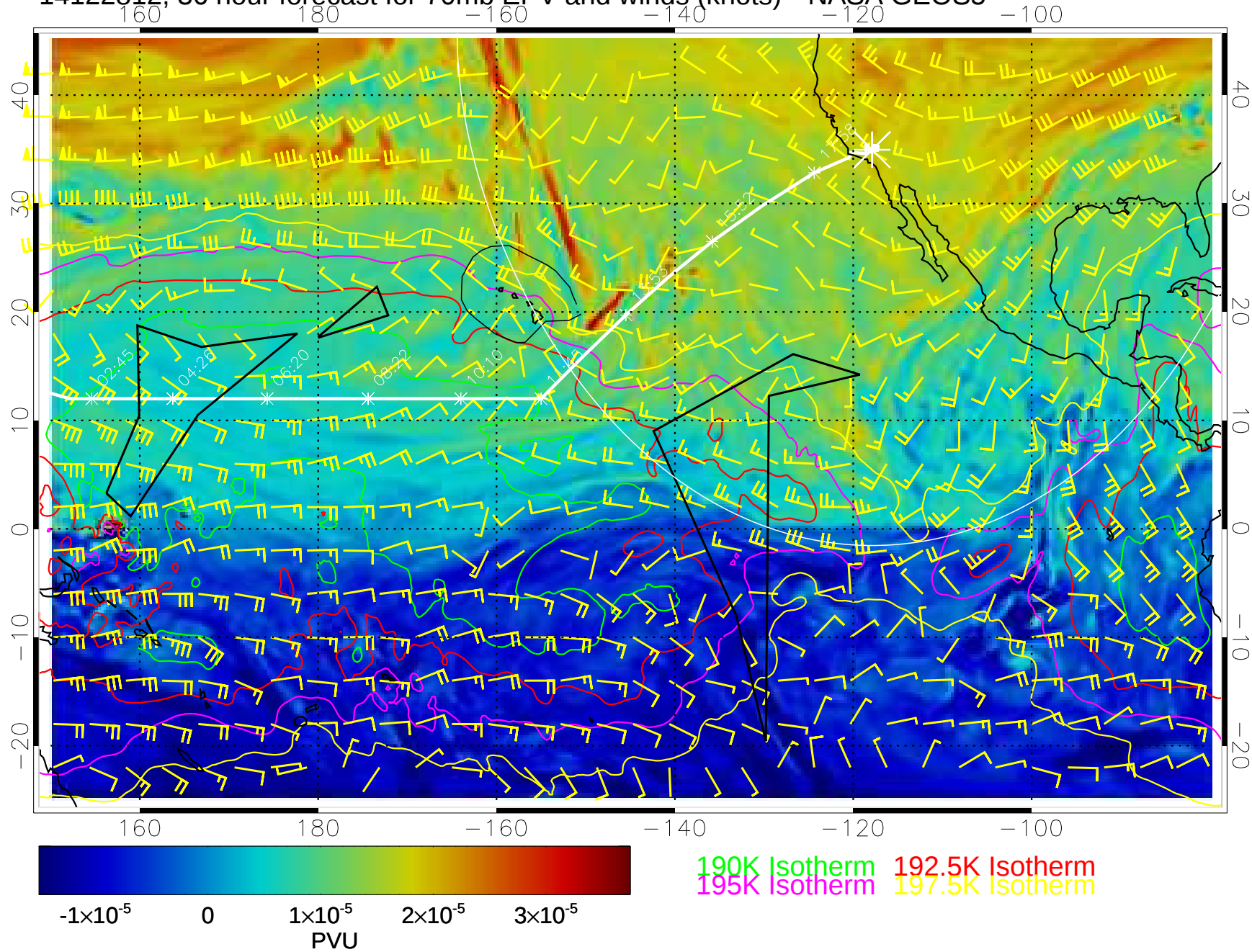
14122812, 36 hour forecast for 70mb EPV and winds (knots)-- NASA GEOS5
