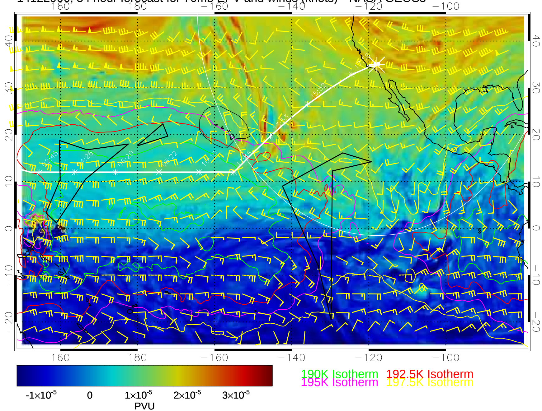
14122906, 54 hour forecast for 70mb EPV and winds (knots)-- NASA GEOS5
