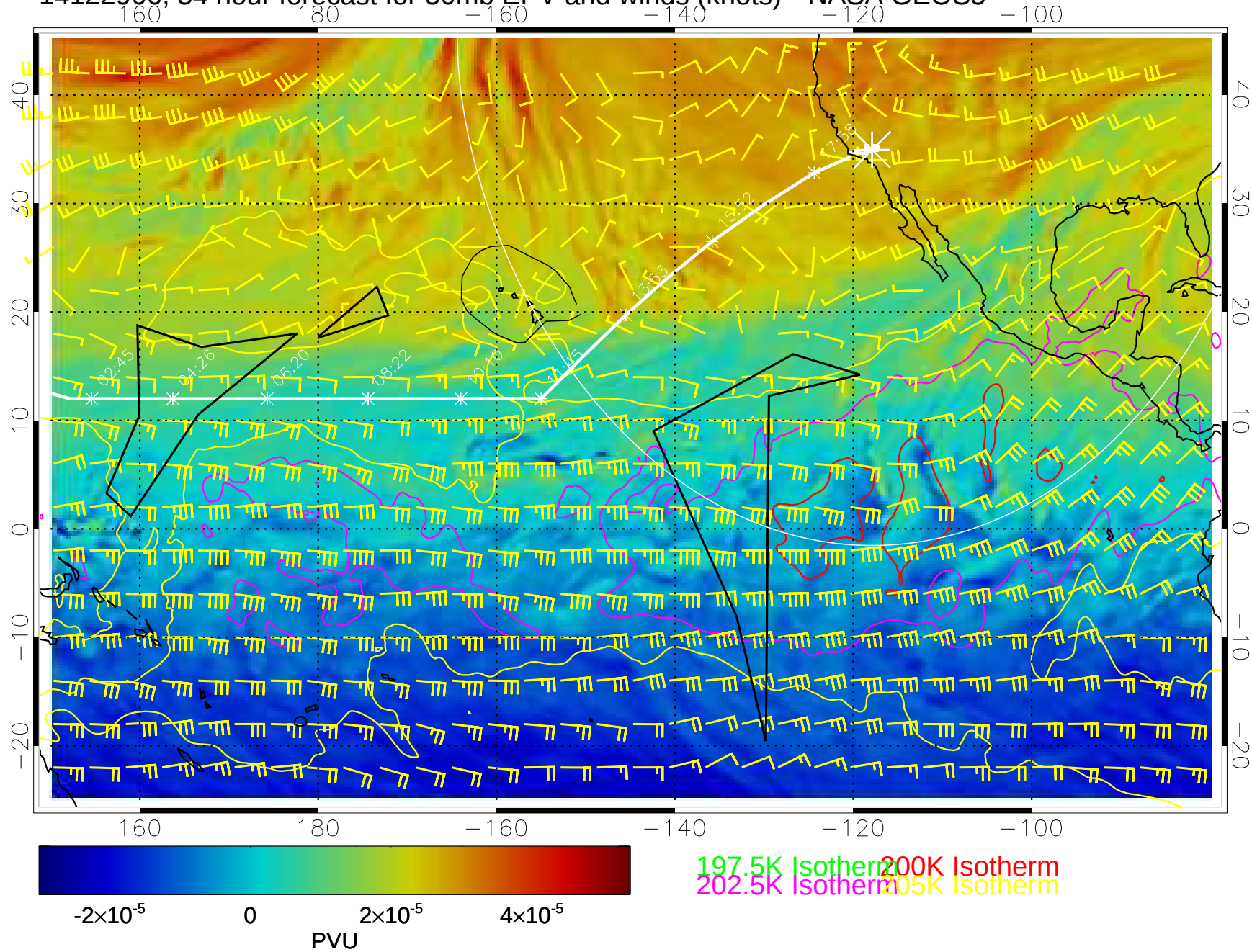
14122906, 54 hour forecast for 50mb EPV and winds (knots)-- NASA GEOS5
