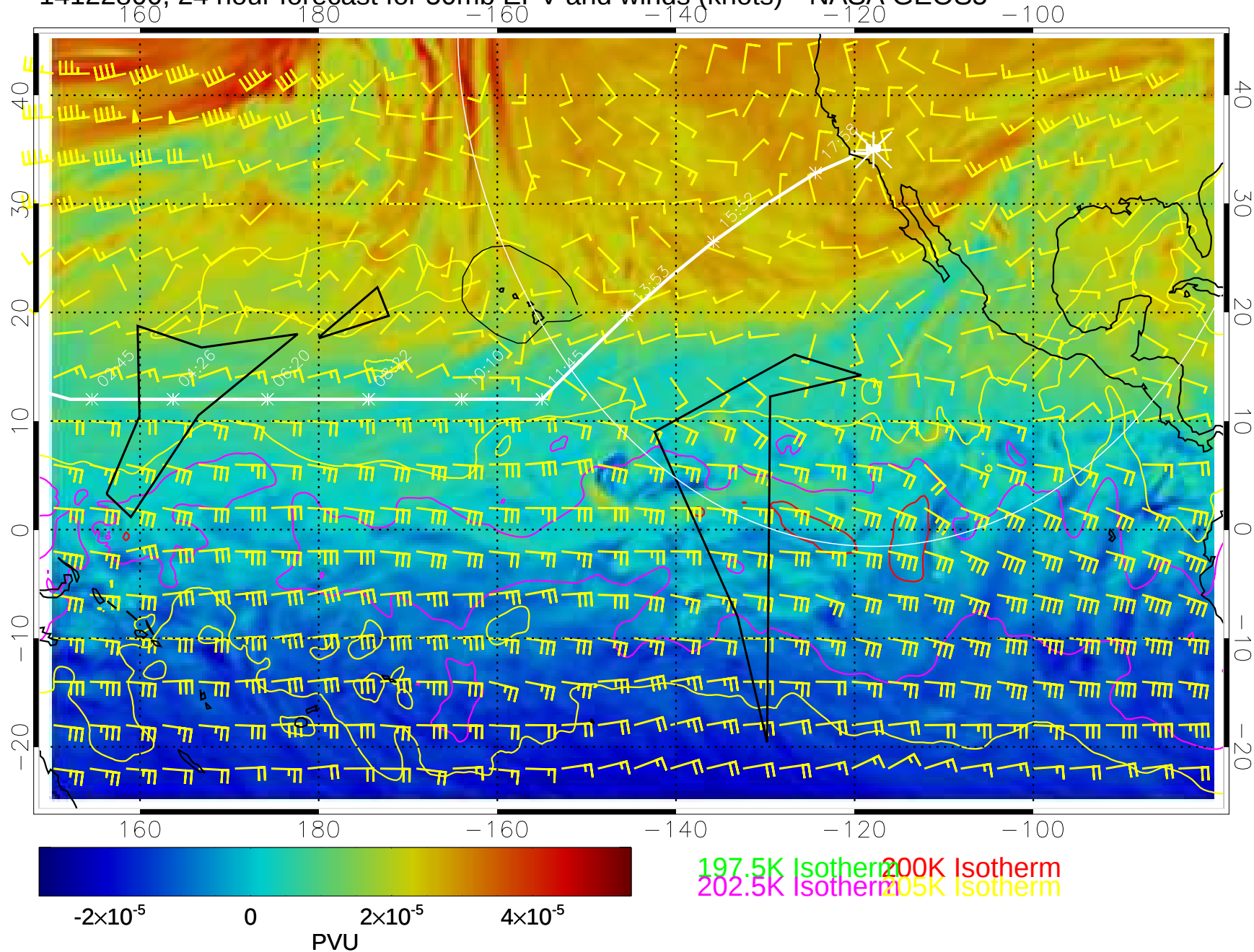
14122800, 24 hour forecast for 50mb EPV and winds (knots)-- NASA GEOS5
