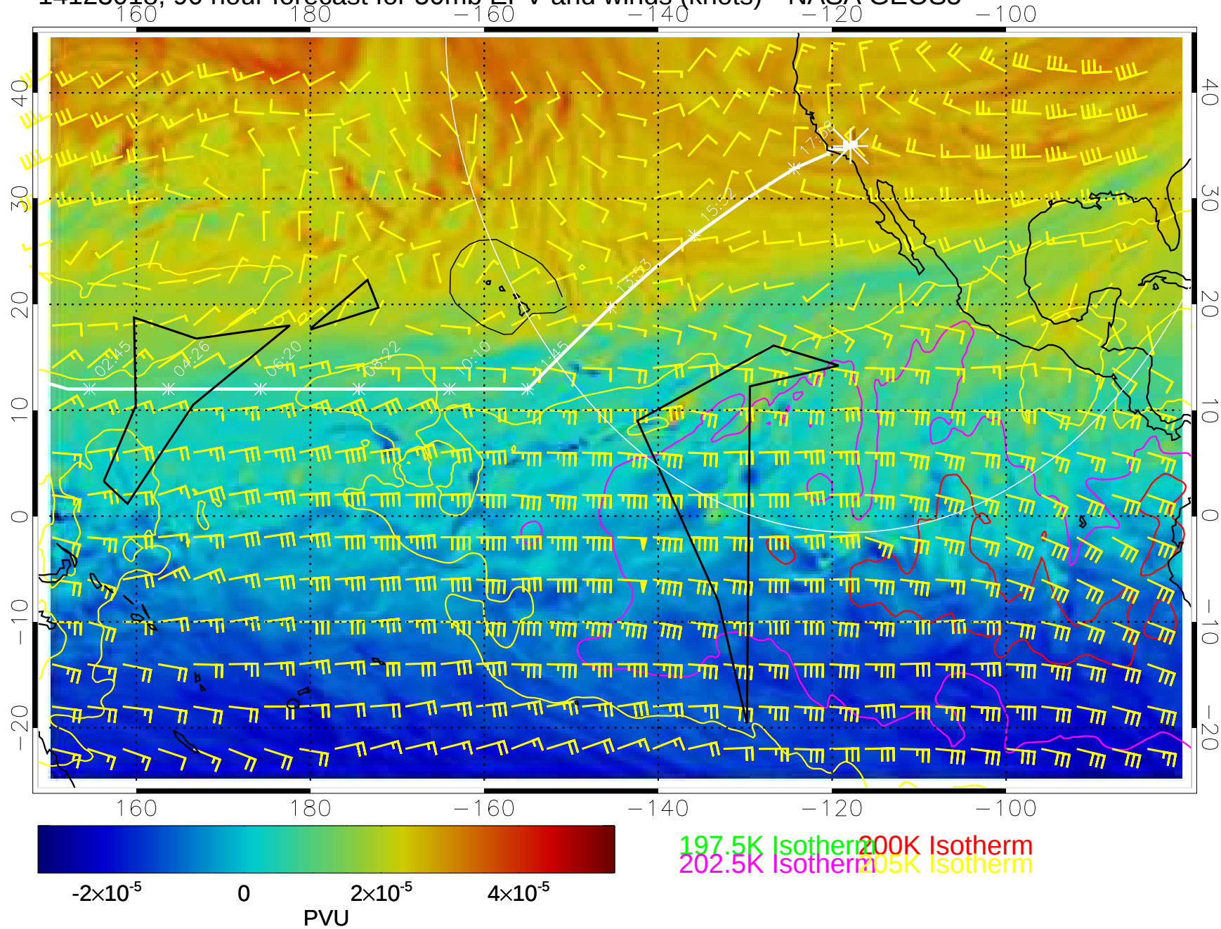
14123018, 90 hour forecast for 50mb EPV and winds (knots)-- NASA GEOS5
