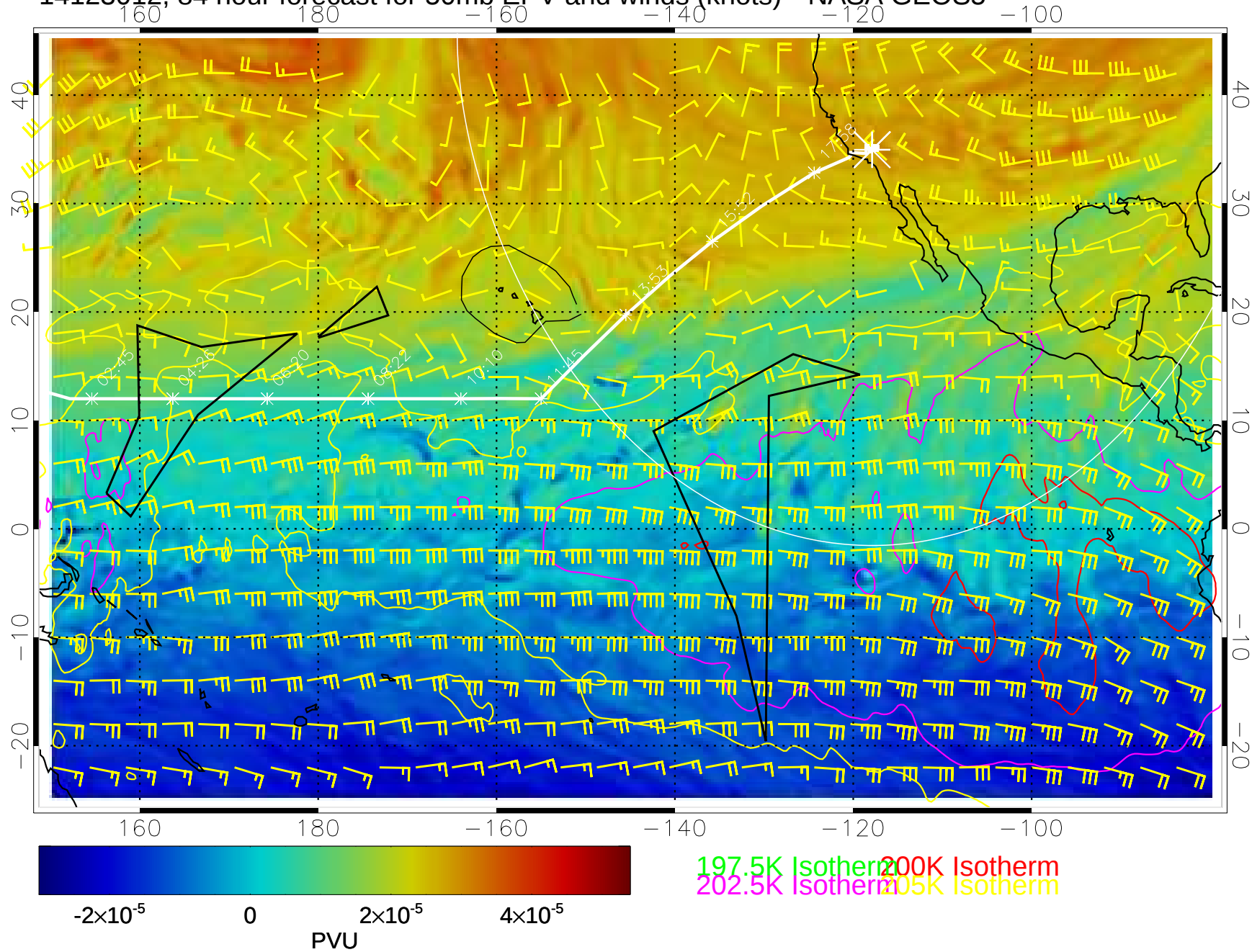
14123012, 84 hour forecast for 50mb EPV and winds (knots)-- NASA GEOS5
