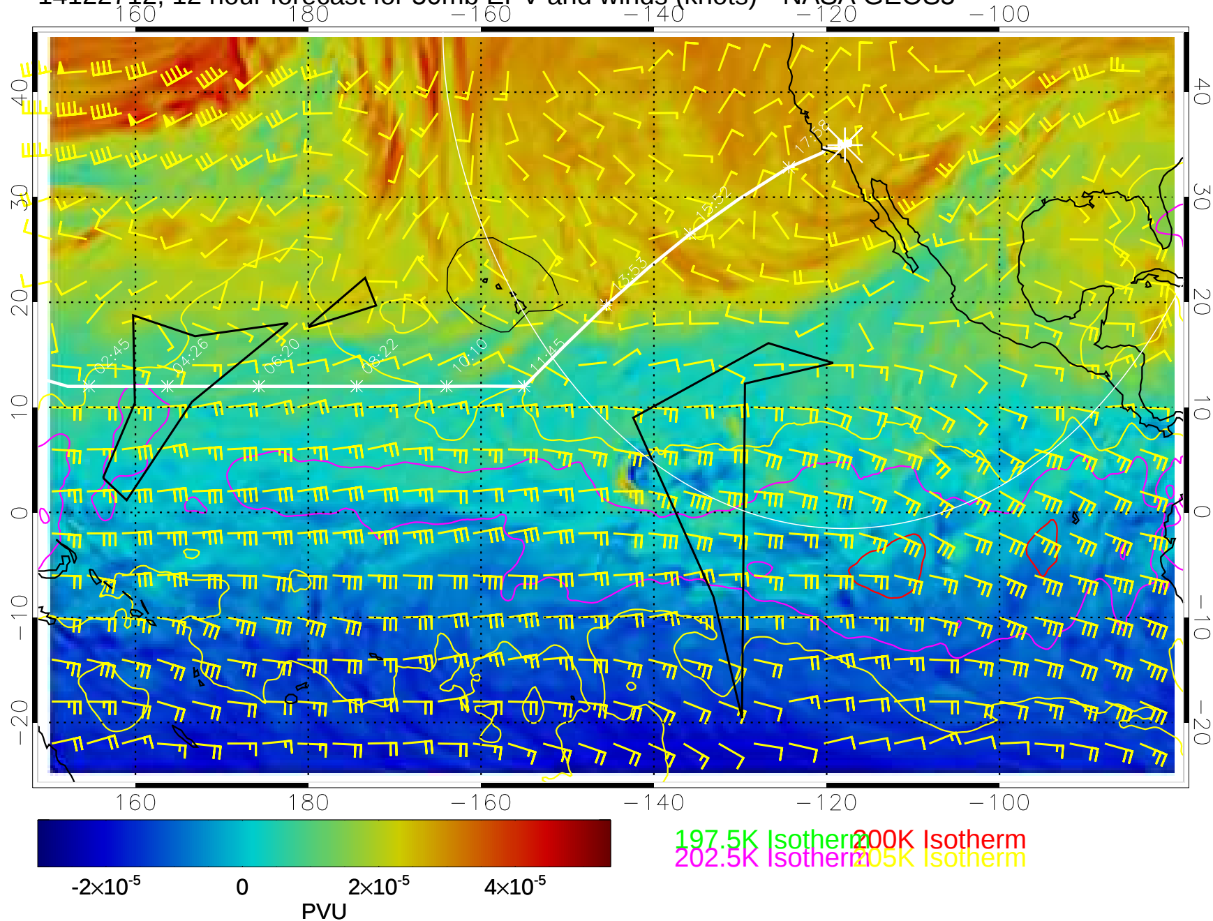
14122712, 12 hour forecast for 50mb EPV and winds (knots)-- NASA GEOS5
