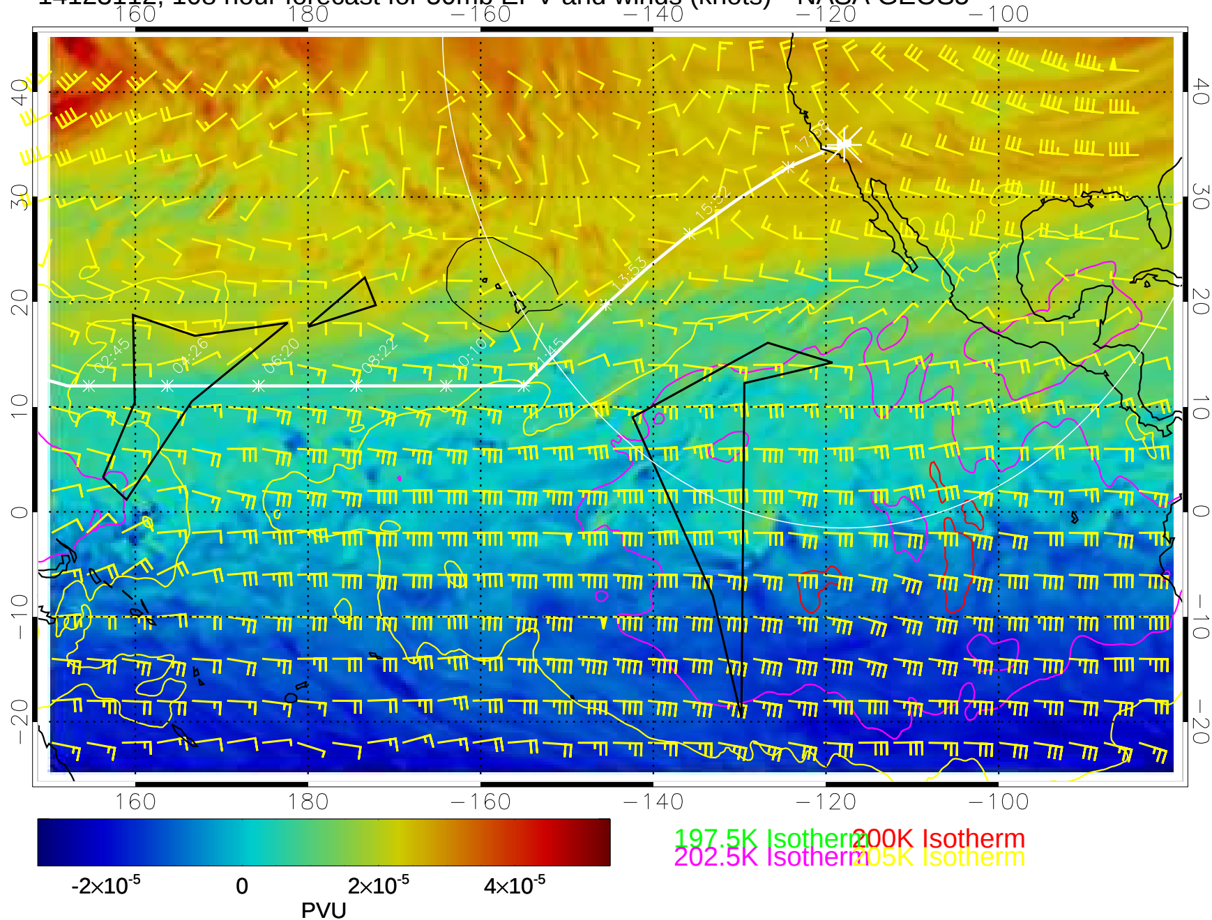
14123112, 108 hour forecast for 50mb EPV and winds (knots)-- NASA GEOS5
