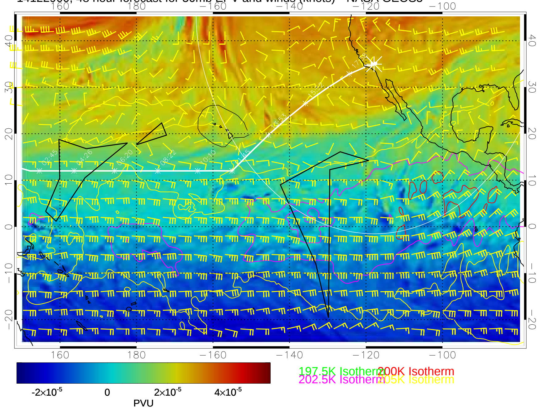
14122900, 48 hour forecast for 50mb EPV and winds (knots)-- NASA GEOS5
