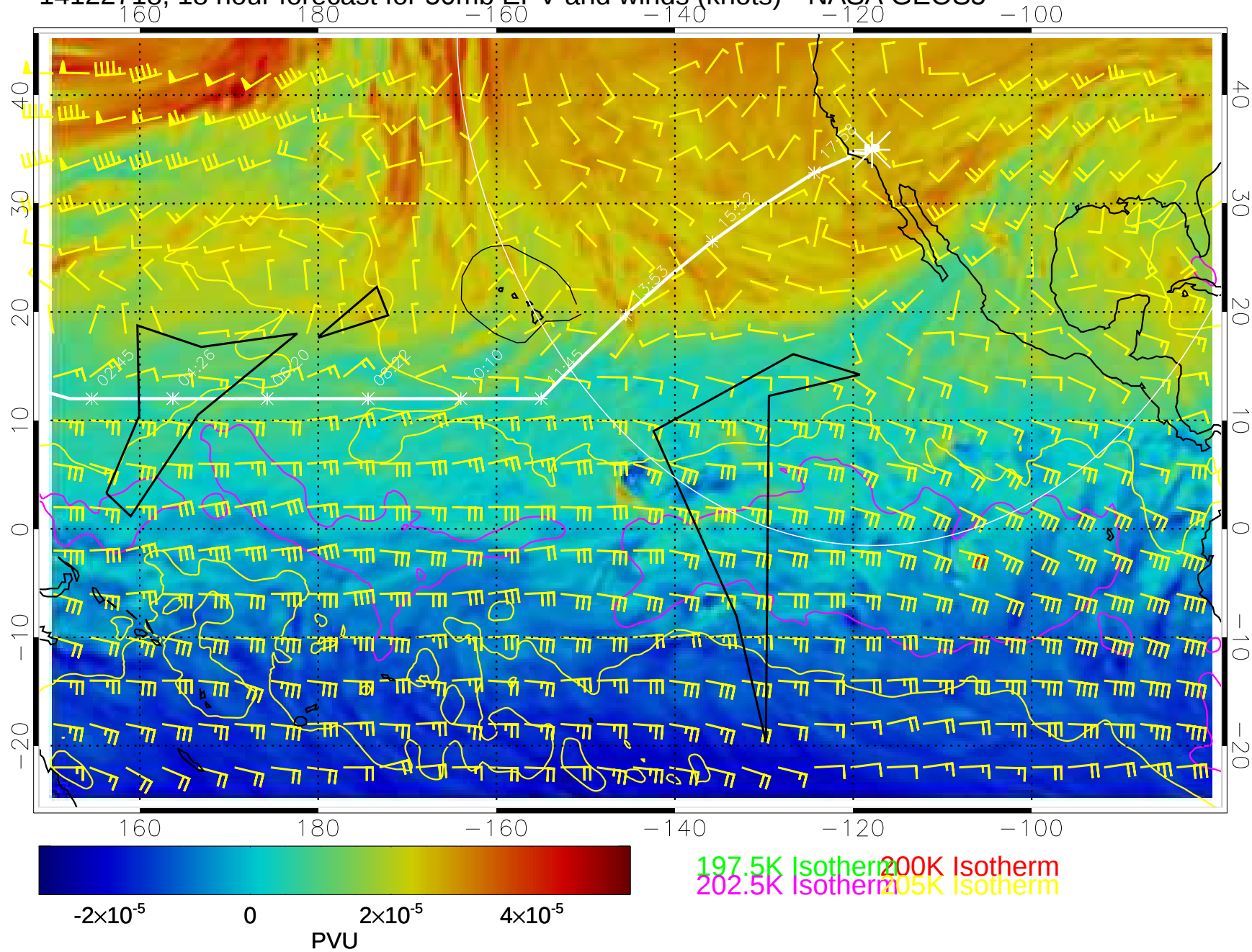
14122718, 18 hour forecast for 50mb EPV and winds (knots)-- NASA GEOS5
