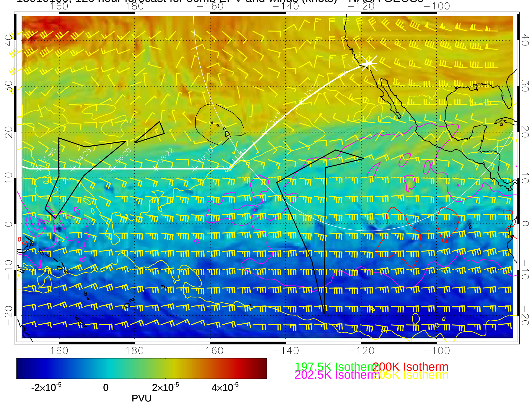
15010100, 120 hour forecast for 50mb EPV and winds (knots)-- NASA GEOS5
