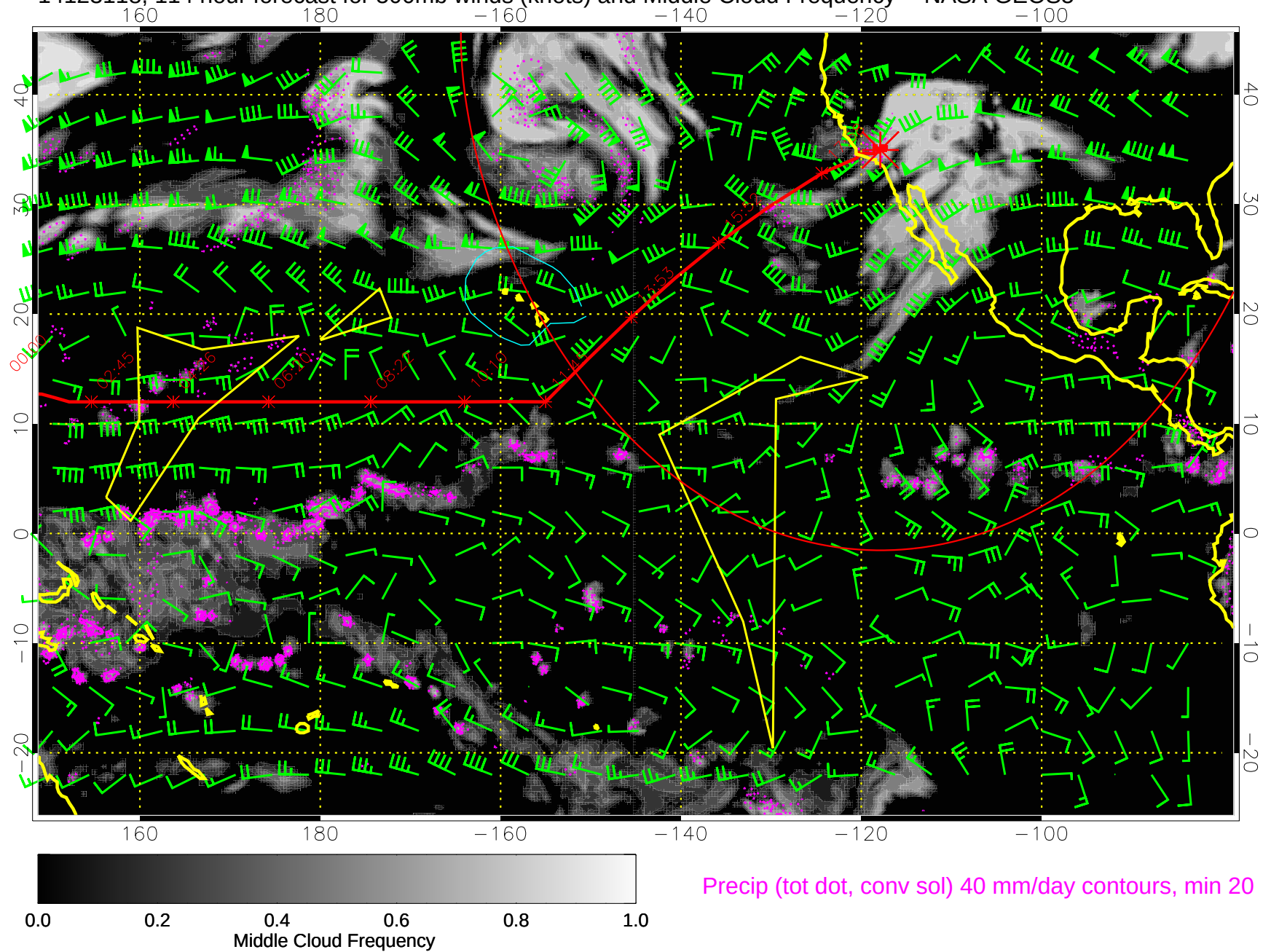
14123118, 114 hour forecast for 500mb winds (knots) and Middle Cloud Frequency -- NASA GEOS5
