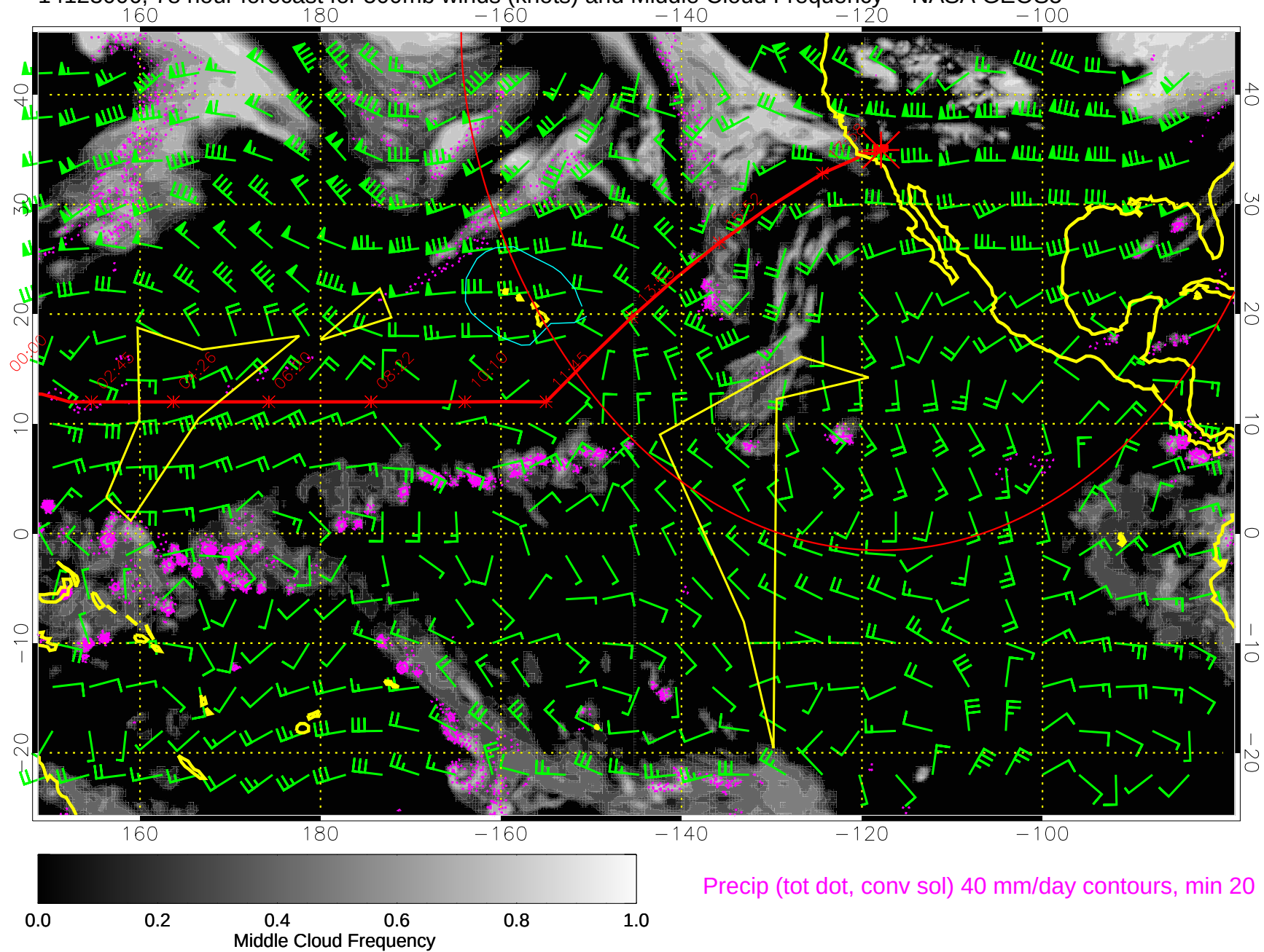
14123006, 78 hour forecast for 500mb winds (knots) and Middle Cloud Frequency -- NASA GEOS5
