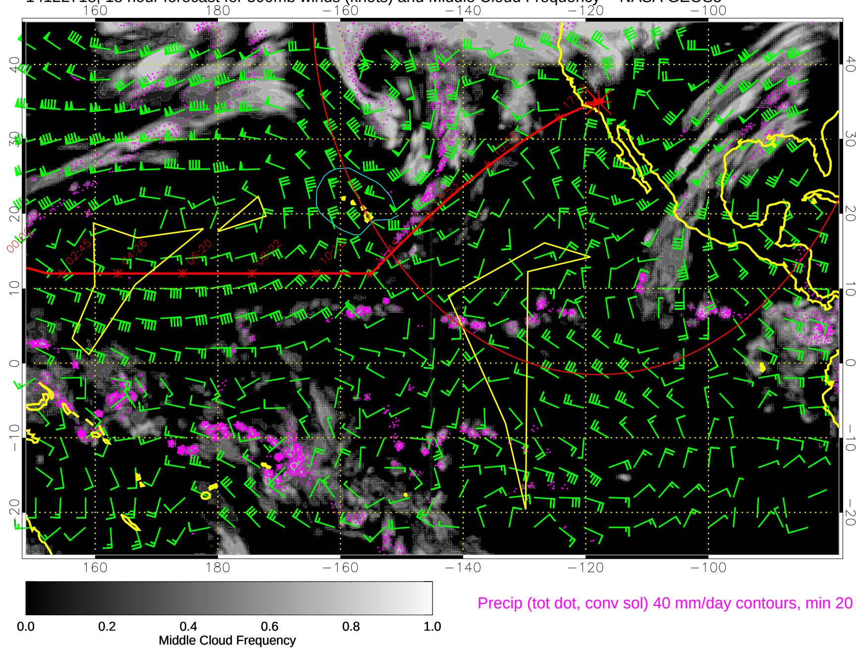
14122718, 18 hour forecast for 500mb winds (knots) and Middle Cloud Frequency -- NASA GEOS5
