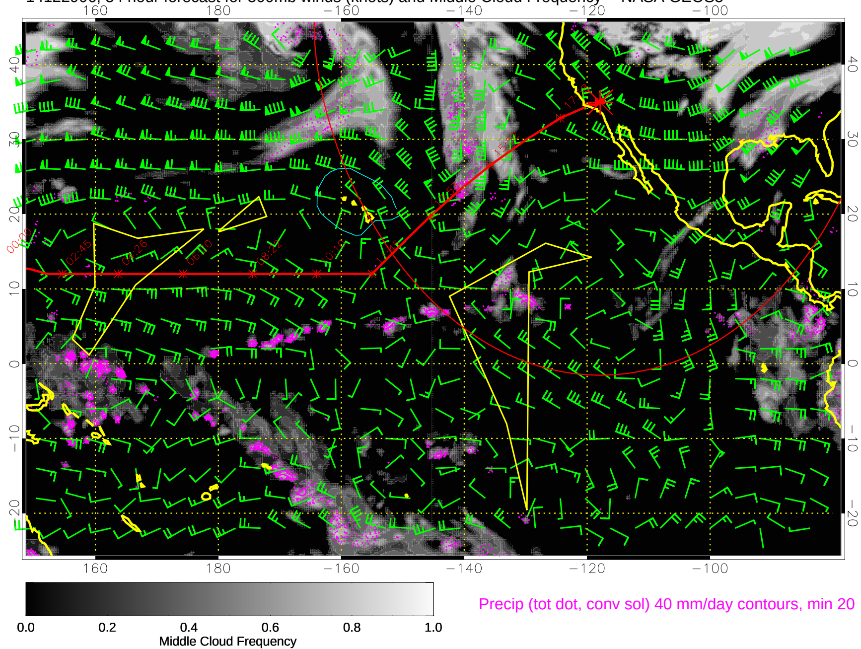
14122906, 54 hour forecast for 500mb winds (knots) and Middle Cloud Frequency -- NASA GEOS5
