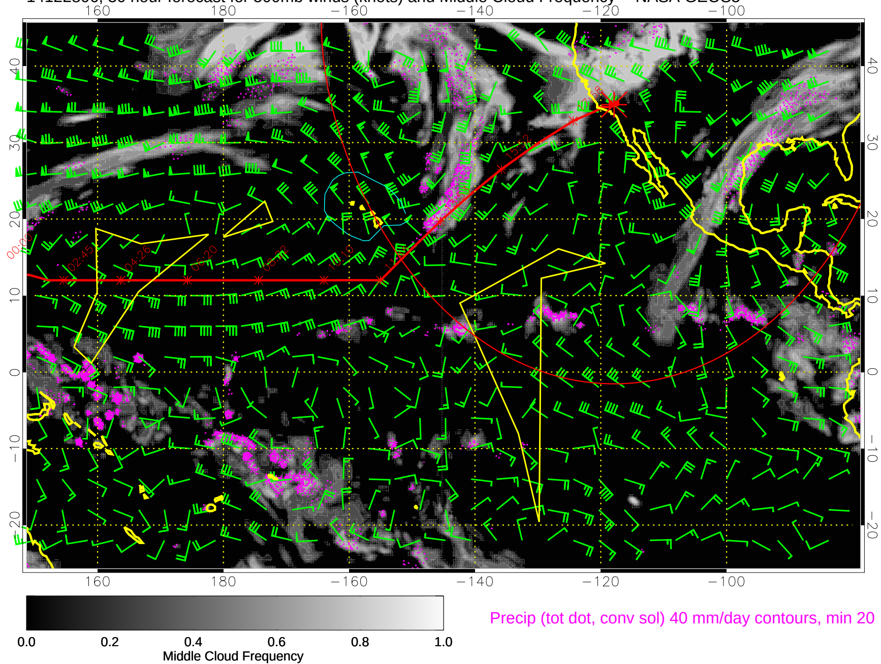
14122806, 30 hour forecast for 500mb winds (knots) and Middle Cloud Frequency -- NASA GEOS5
