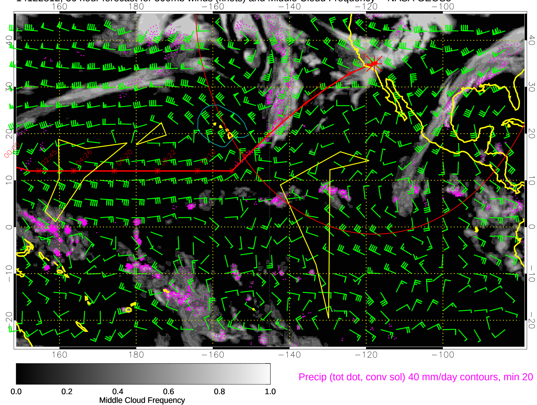
14122812, 36 hour forecast for 500mb winds (knots) and Middle Cloud Frequency -- NASA GEOS5
