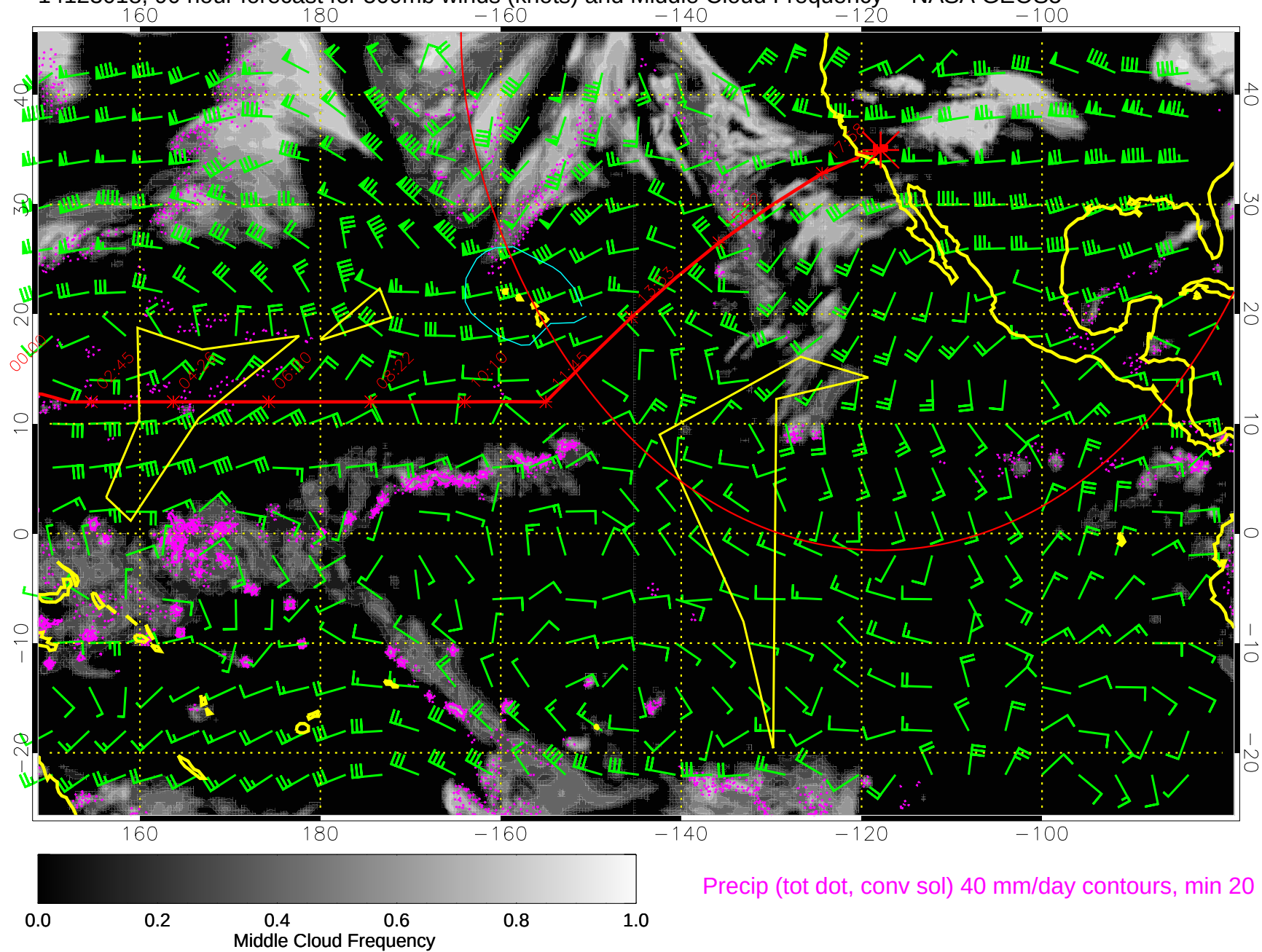
14123018, 90 hour forecast for 500mb winds (knots) and Middle Cloud Frequency -- NASA GEOS5
