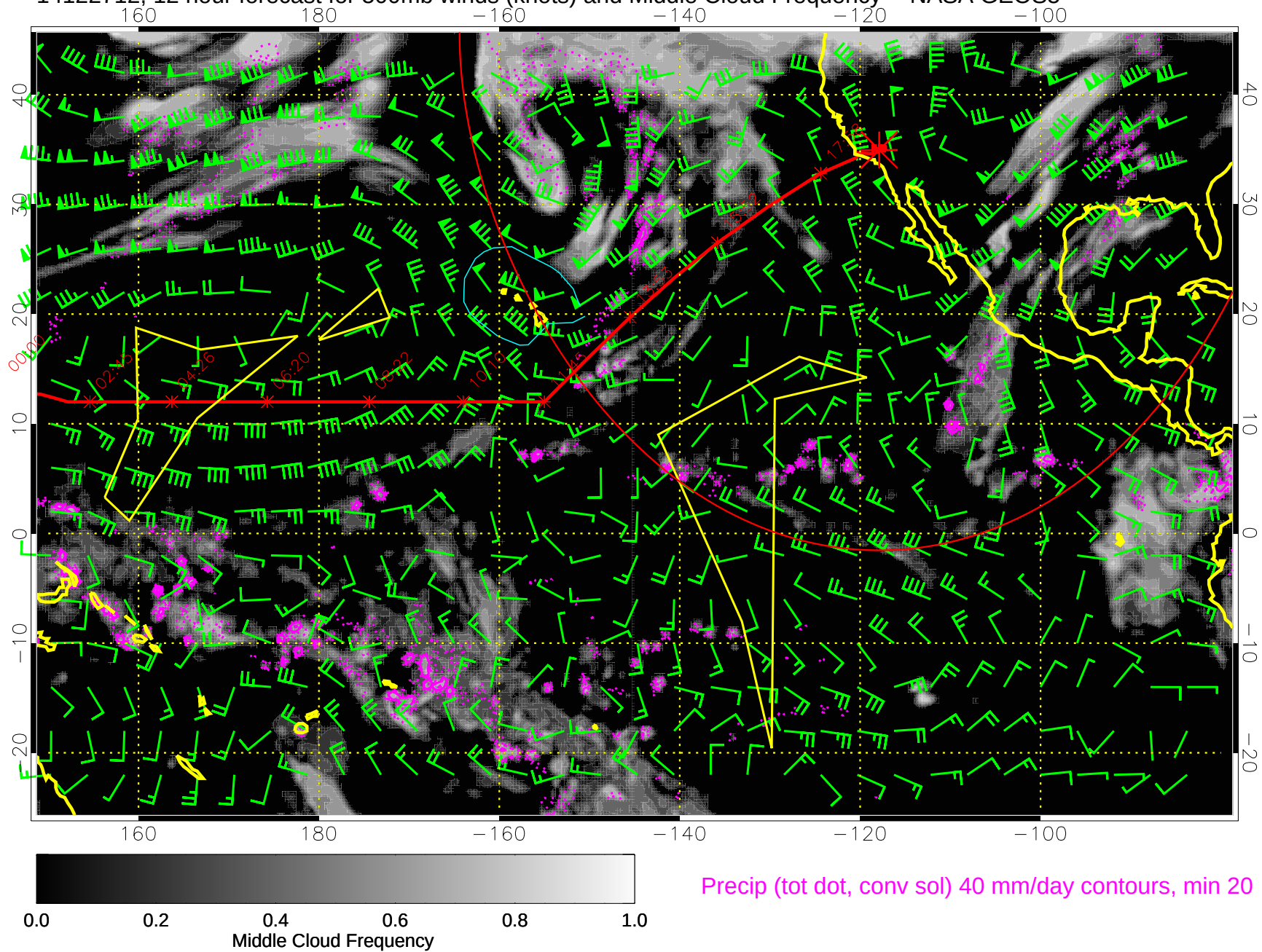
14122712, 12 hour forecast for 500mb winds (knots) and Middle Cloud Frequency -- NASA GEOS5
