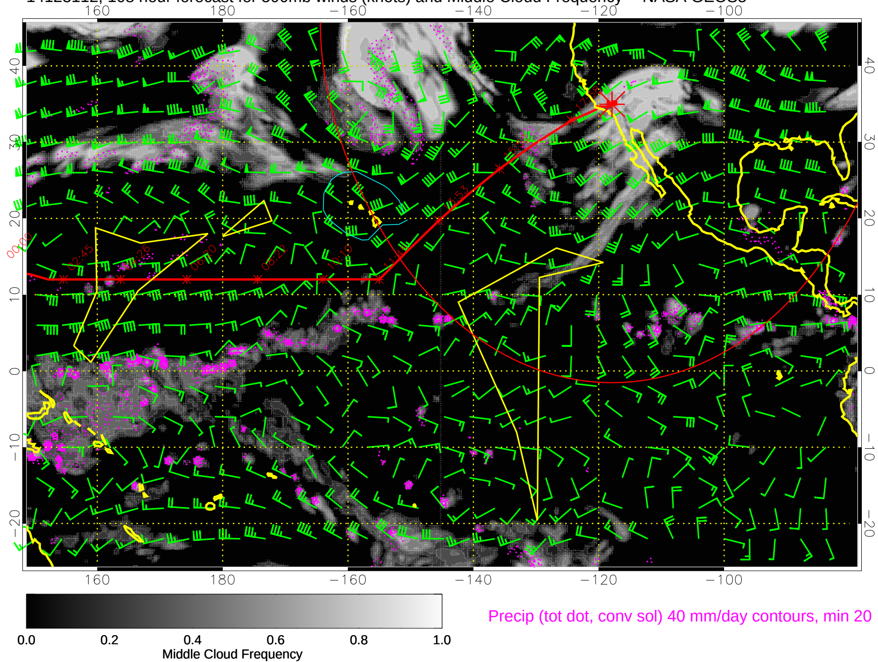
14123112, 108 hour forecast for 500mb winds (knots) and Middle Cloud Frequency -- NASA GEOS5
