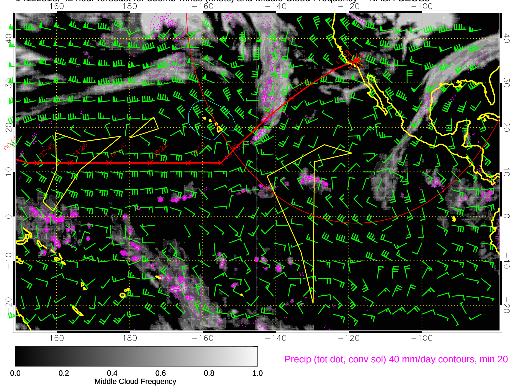
14122818, 42 hour forecast for 500mb winds (knots) and Middle Cloud Frequency -- NASA GEOS5
