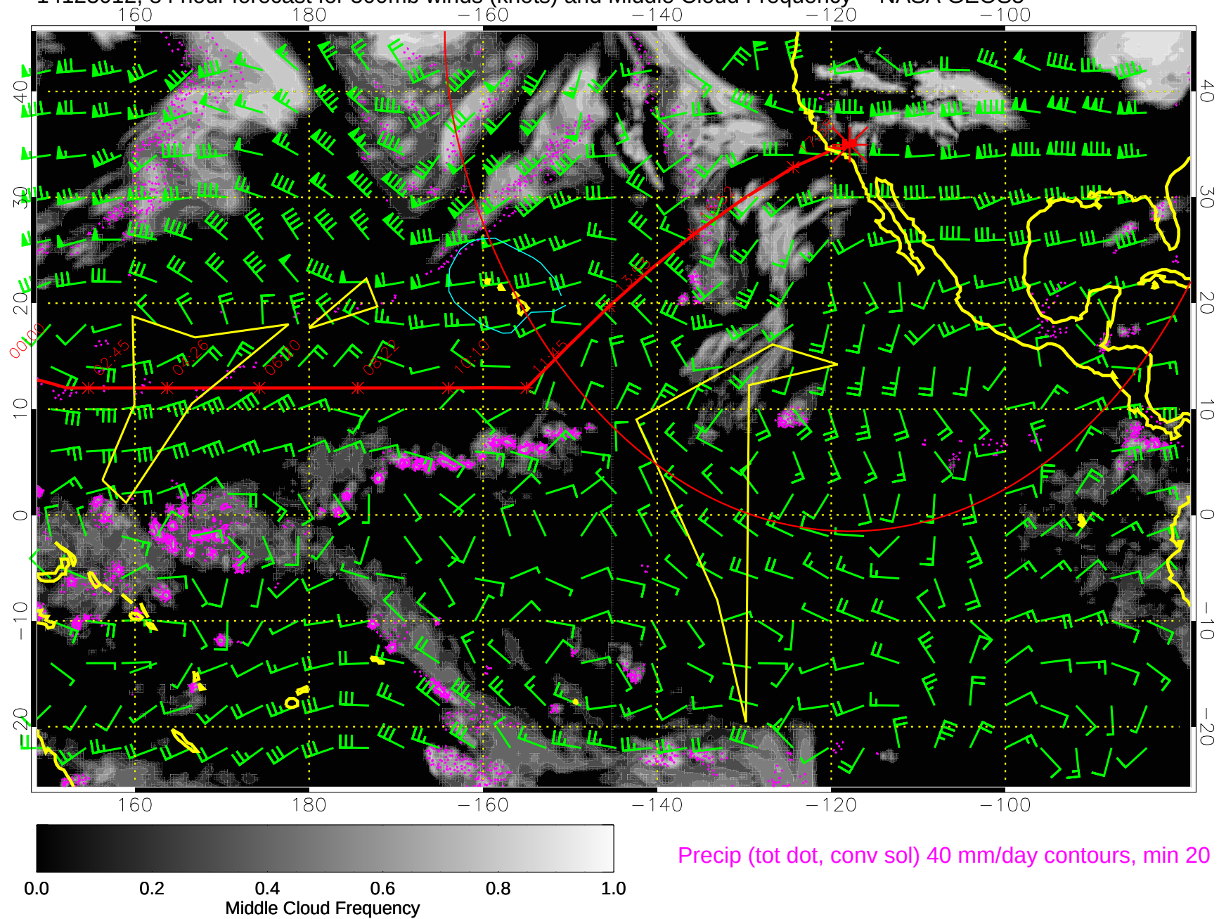
14123012, 84 hour forecast for 500mb winds (knots) and Middle Cloud Frequency -- NASA GEOS5
