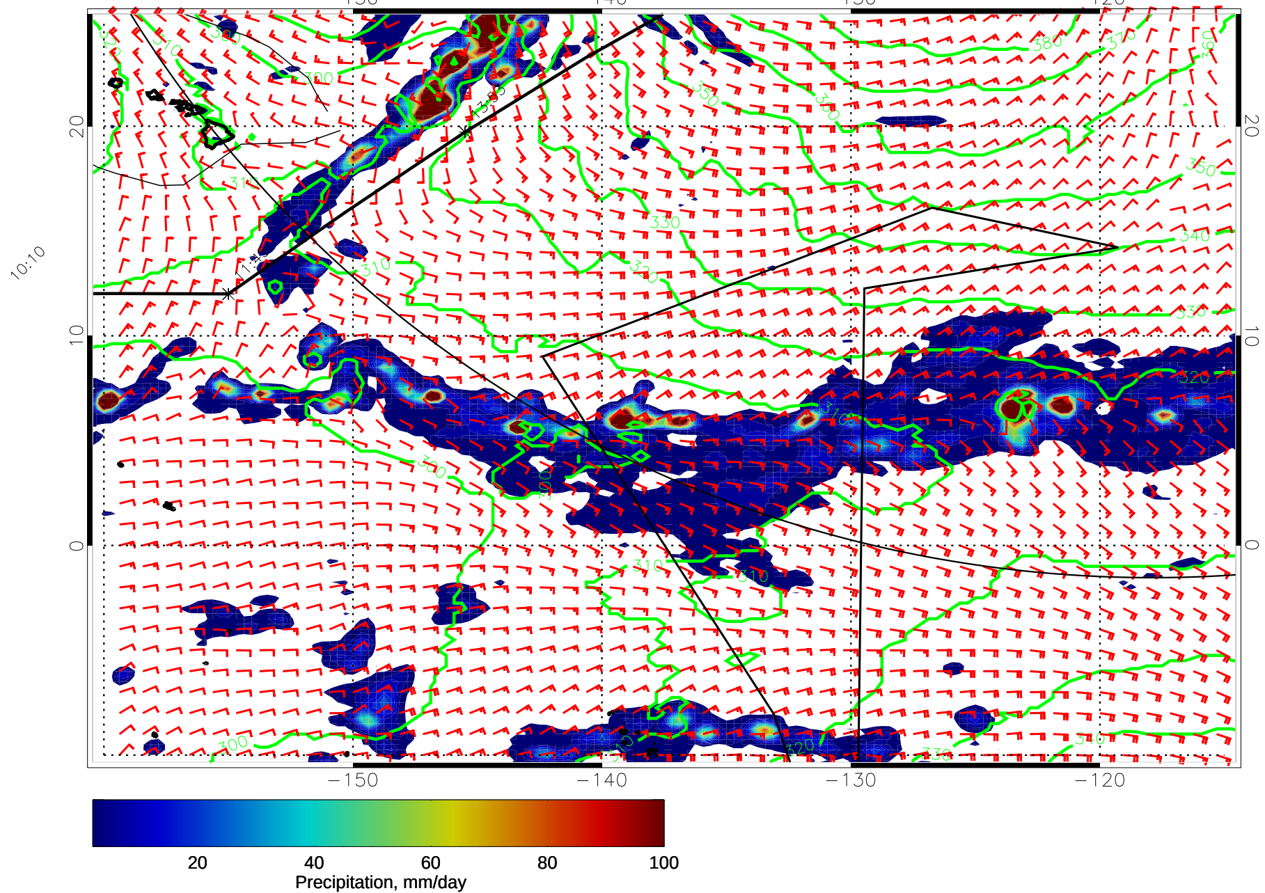
14122706, 30 hour forecast for 975mb Z, Precip., and Surface Winds (knots) -- NASA GEOS5
