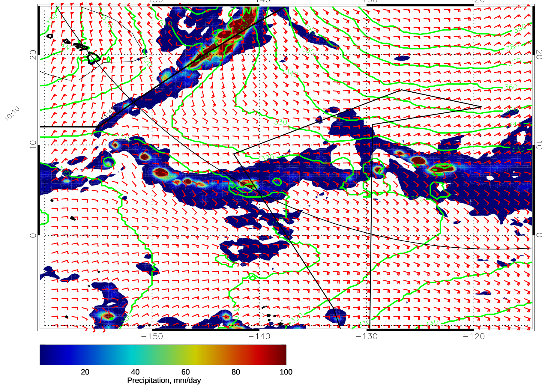
14122806, 54 hour forecast for 975mb Z, Precip., and Surface Winds (knots) -- NASA GEOS5
