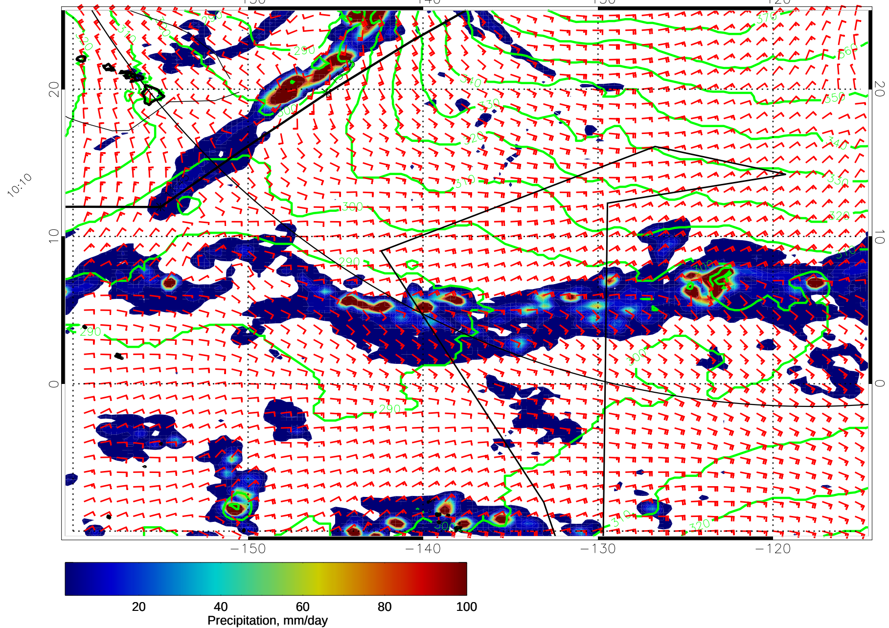
14122712, 36 hour forecast for 975mb Z, Precip., and Surface Winds (knots) -- NASA GEOS5
