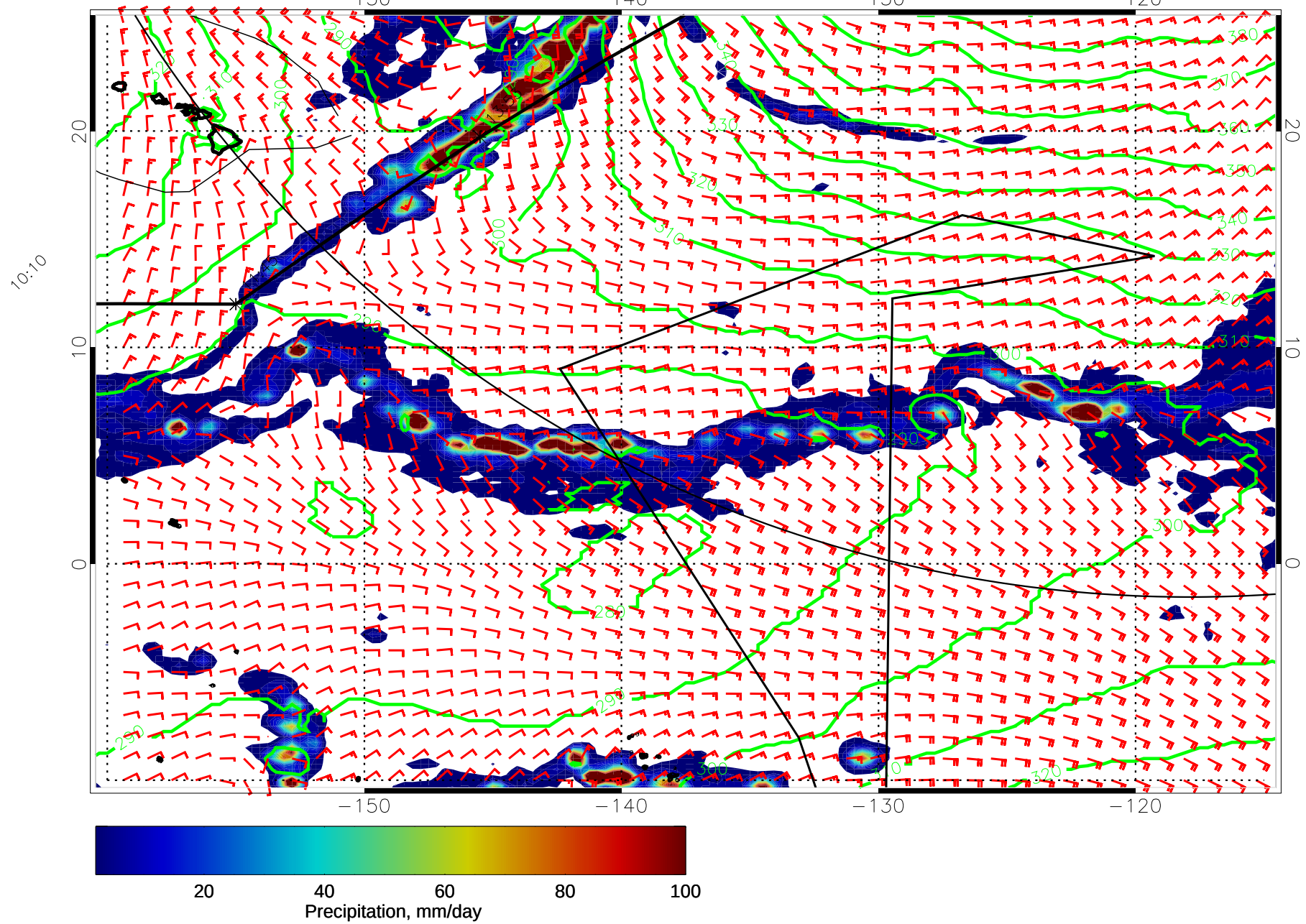
14122800, 48 hour forecast for 975mb Z, Precip., and Surface Winds (knots) -- NASA GEOS5
