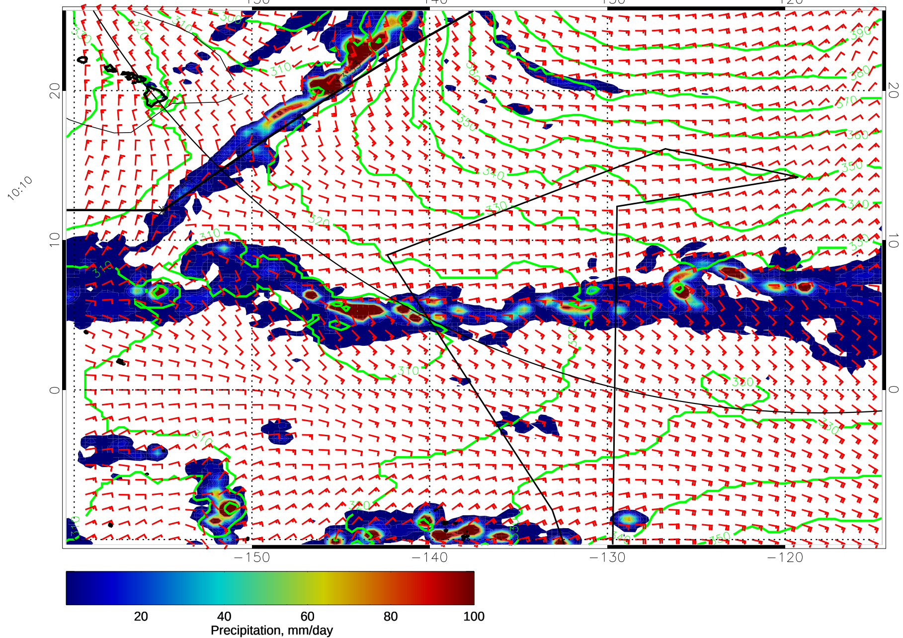
14122718, 42 hour forecast for 975mb Z, Precip., and Surface Winds (knots) -- NASA GEOS5
