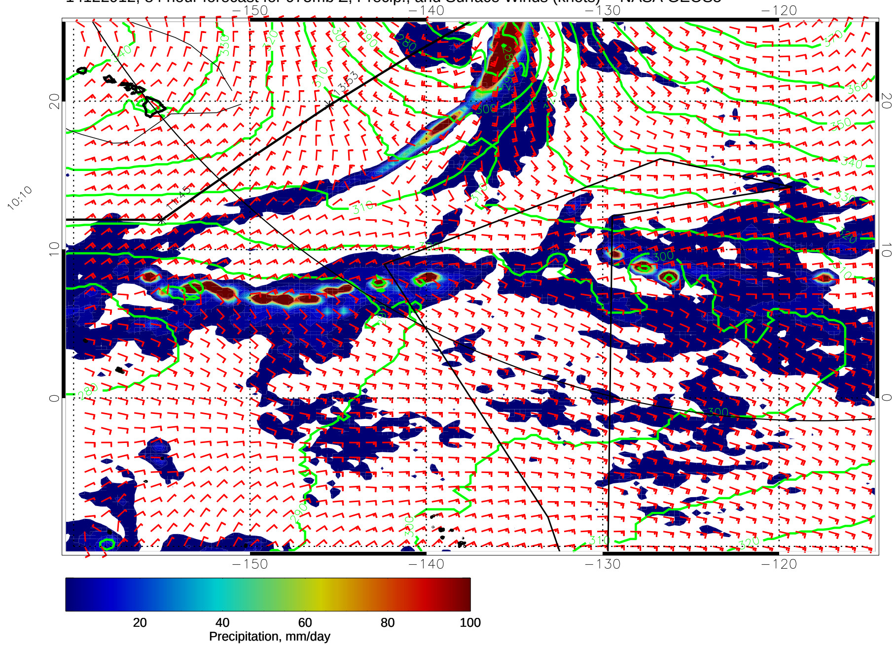
14122912, 84 hour forecast for 975mb Z, Precip., and Surface Winds (knots) -- NASA GEOS5
