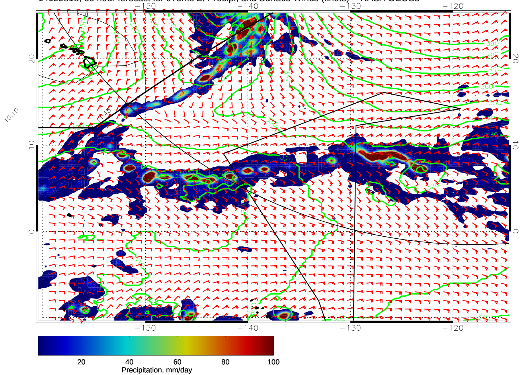
14122818, 66 hour forecast for 975mb Z, Precip., and Surface Winds (knots) -- NASA GEOS5
