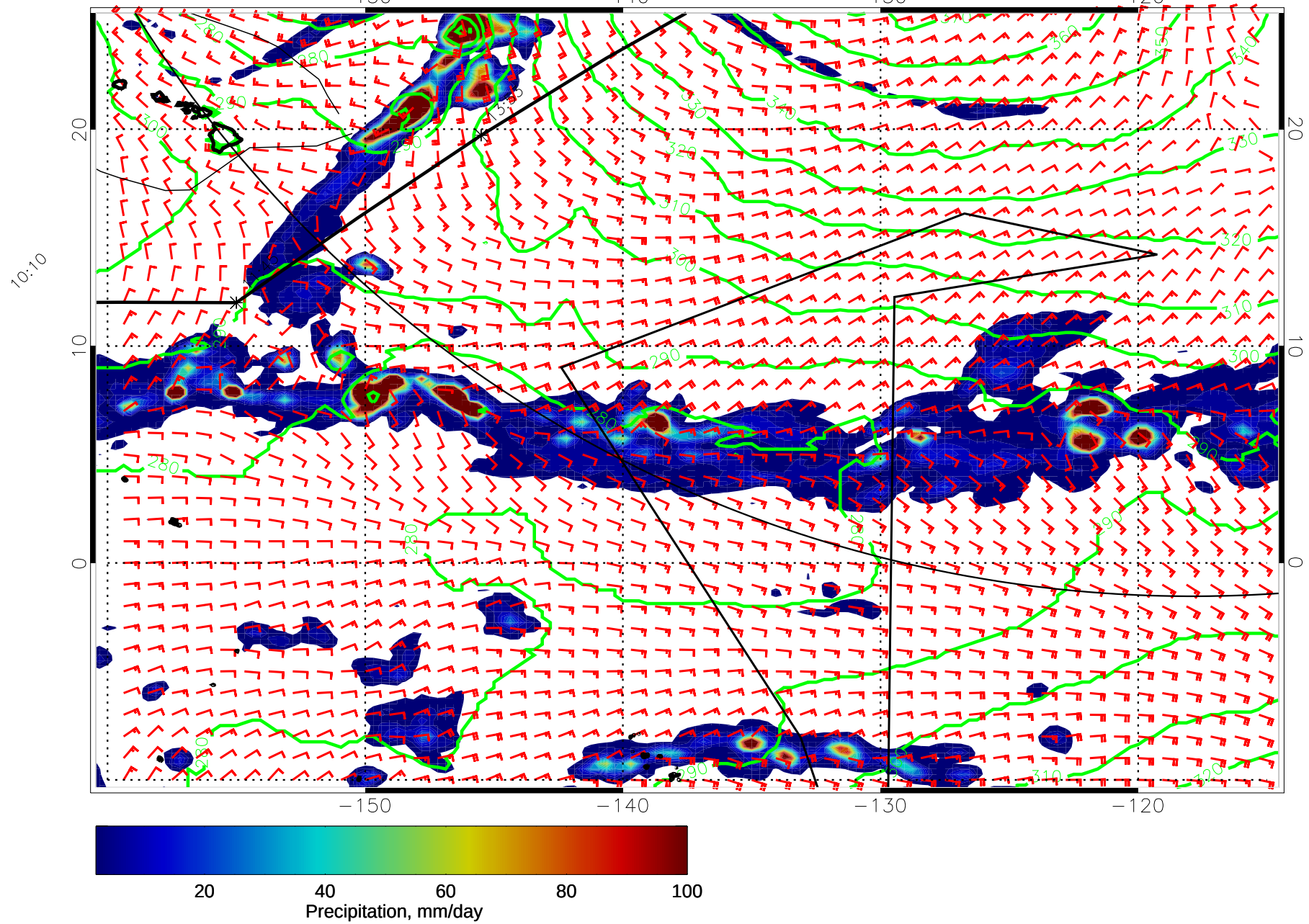
14122700, 24 hour forecast for 975mb Z, Precip., and Surface Winds (knots) -- NASA GEOS5
