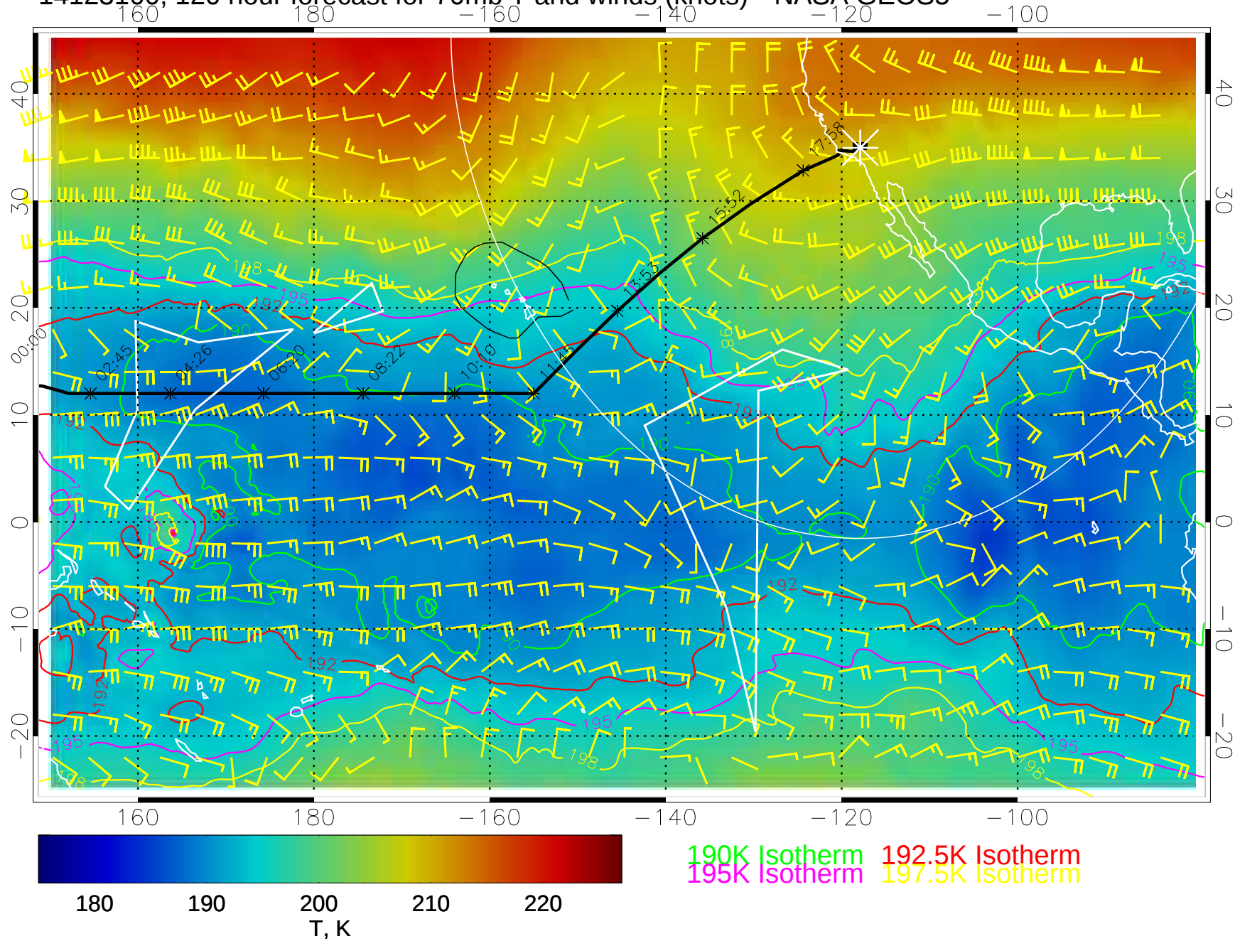
14123100, 120 hour forecast for 70mb T and winds (knots)-- NASA GEOS5
