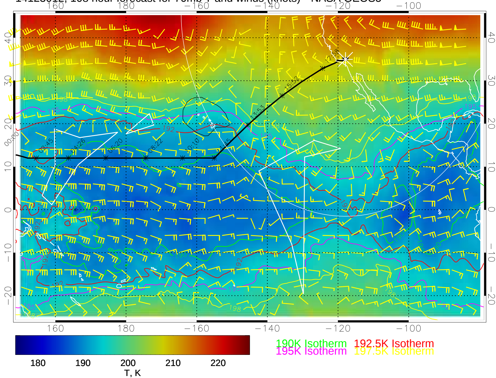
14123012, 108 hour forecast for 70mb T and winds (knots)-- NASA GEOS5
