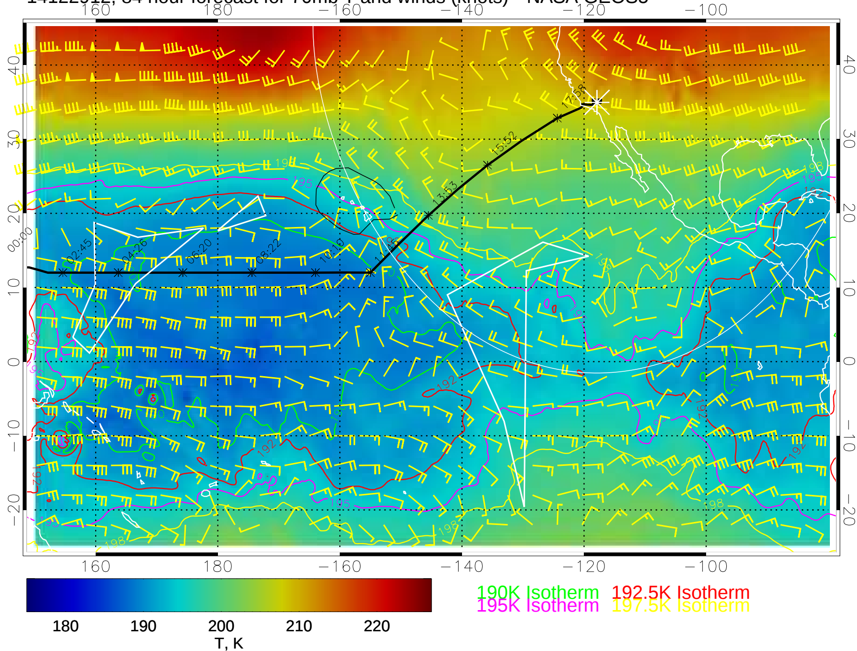
14122912, 84 hour forecast for 70mb T and winds (knots)-- NASA GEOS5
