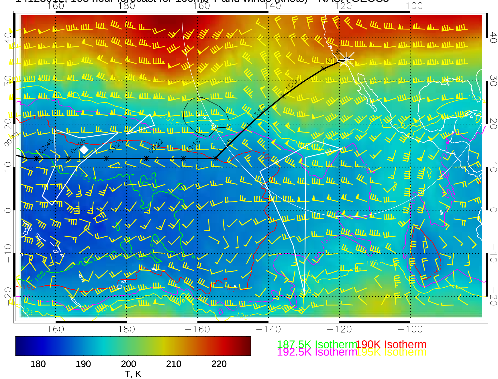
14123012, 108 hour forecast for 100mb T and winds (knots)-- NASA GEOS5
