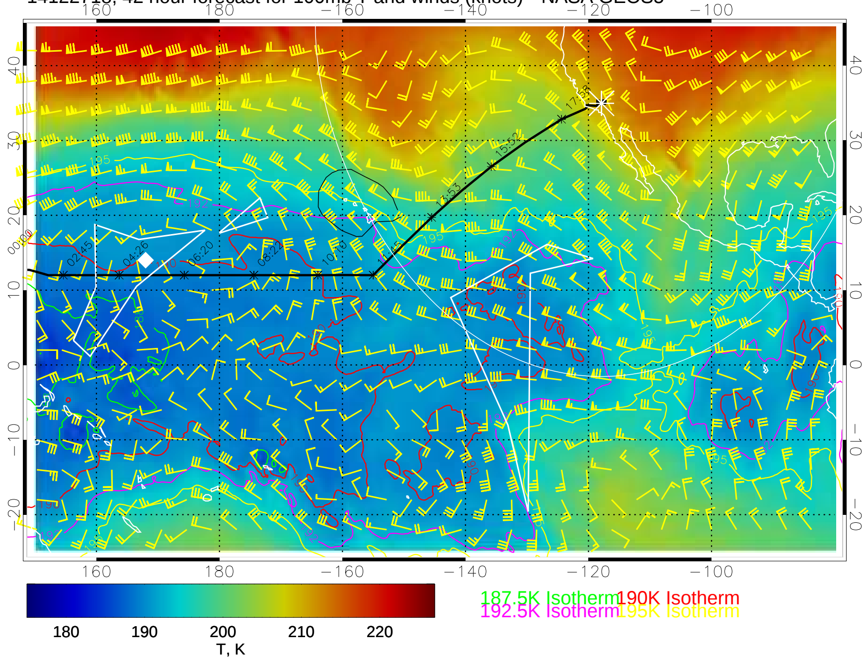
14122718, 42 hour forecast for 100mb T and winds (knots)-- NASA GEOS5
