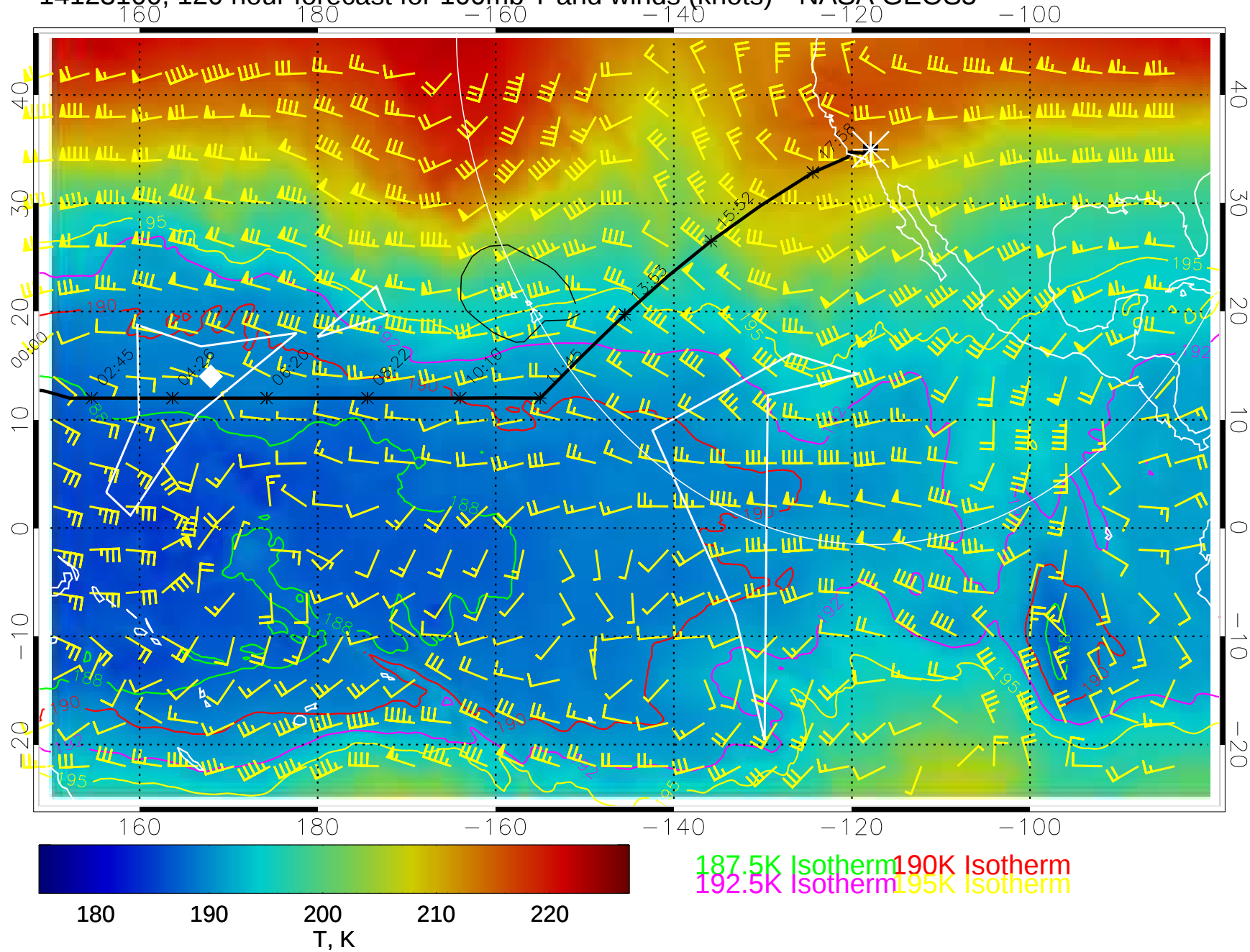
14123100, 120 hour forecast for 100mb T and winds (knots)-- NASA GEOS5
